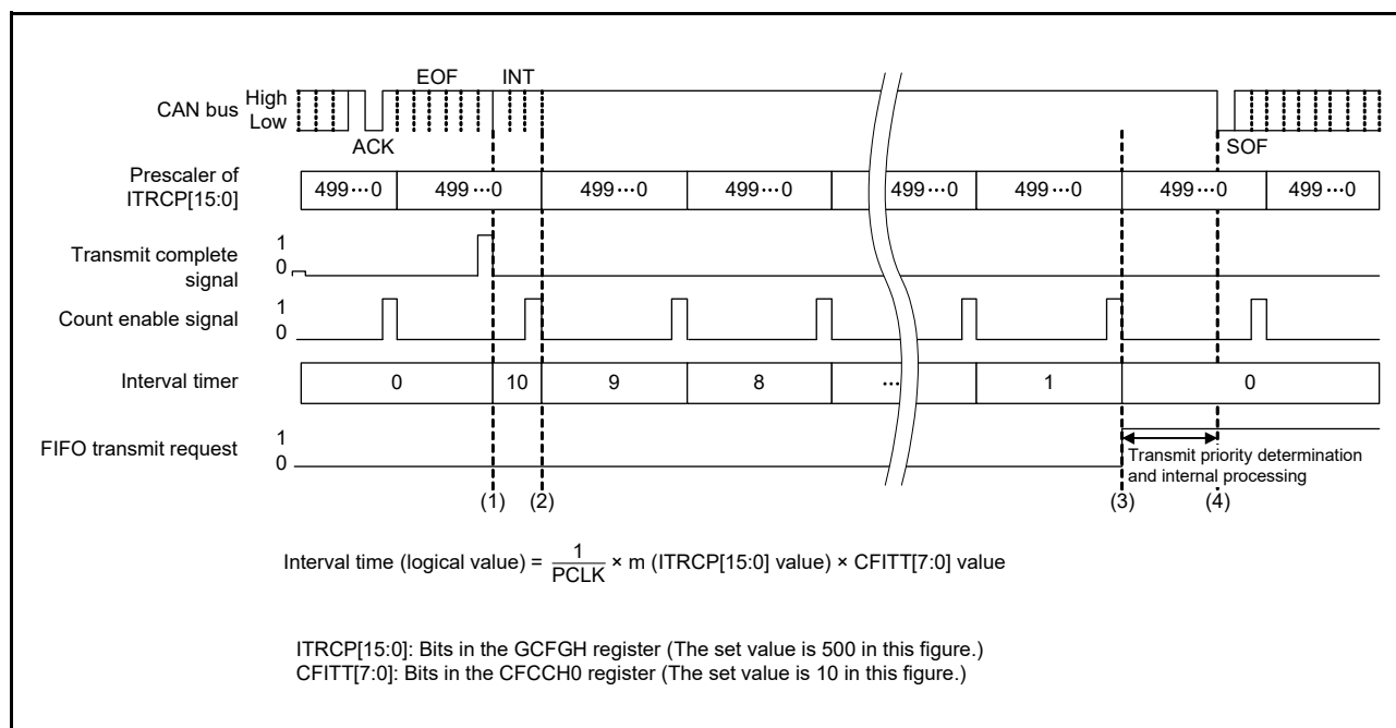
Figure 28.9 Interval Timer Timing Chart
