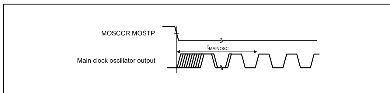
Figure 37.23 Main Clock Oscillation Start Timing
