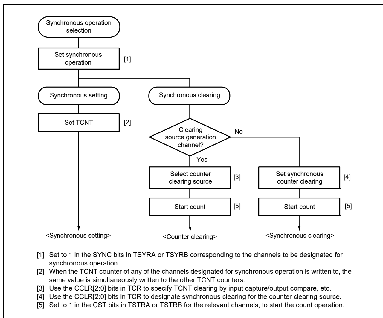
Figure 20.13 Example of Synchronous Operation Setting Procedure
