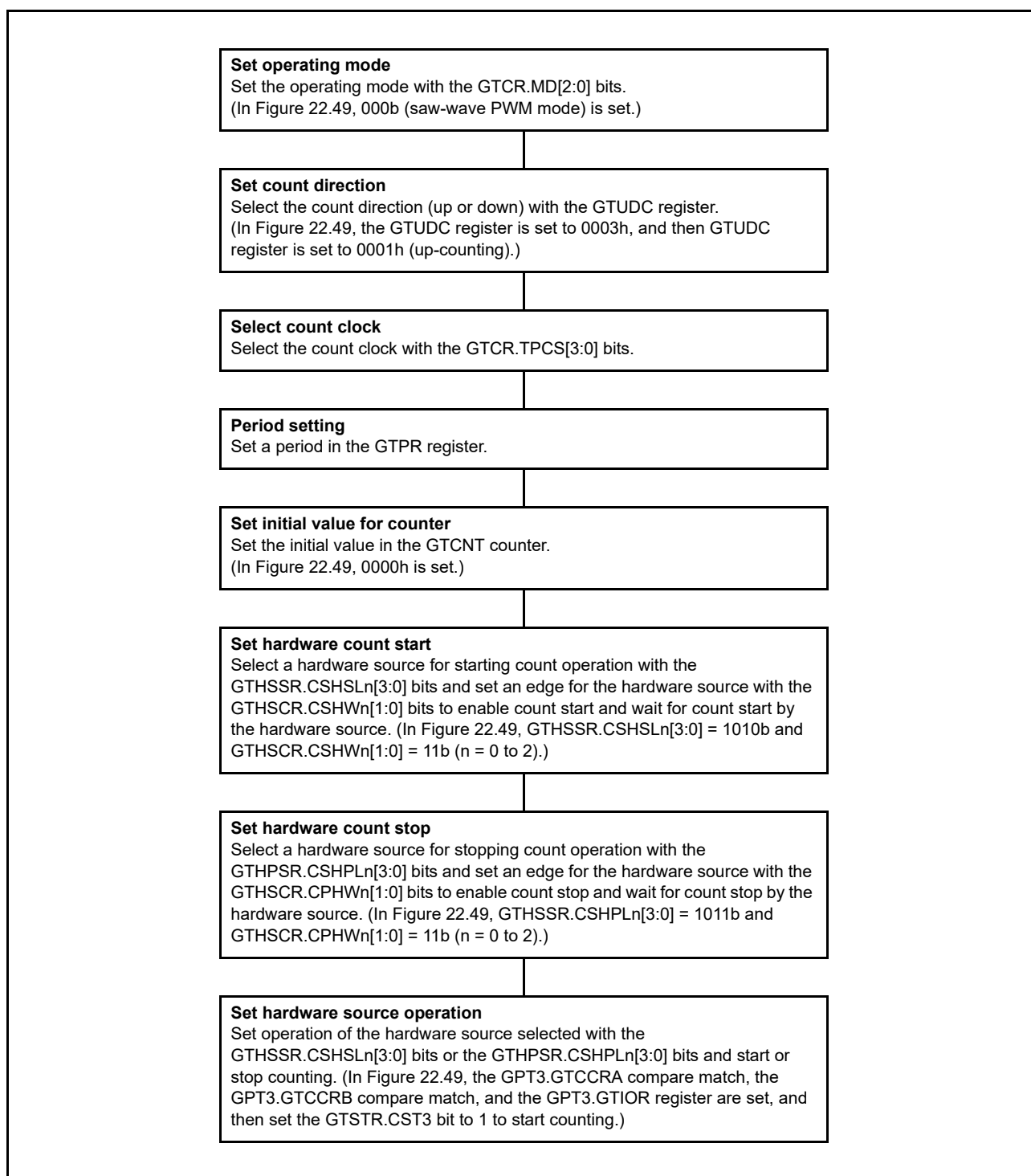
Figure 22.50 Example for Setting Count Stop Operation by Hardware Source
