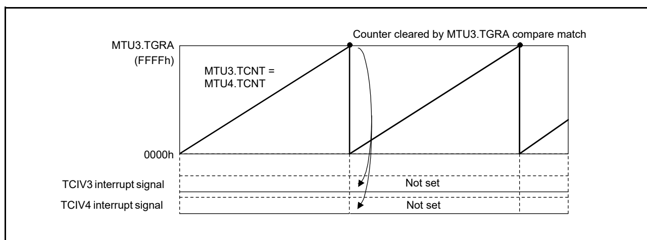
Figure 20.146 Overflow in Reset-Synchronized PWM Mode
