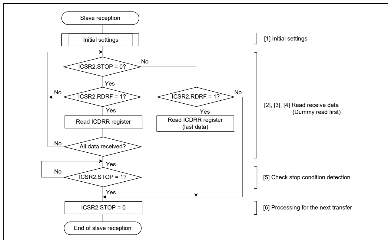
Figure 27.18 Example of Slave Reception Flowchart
