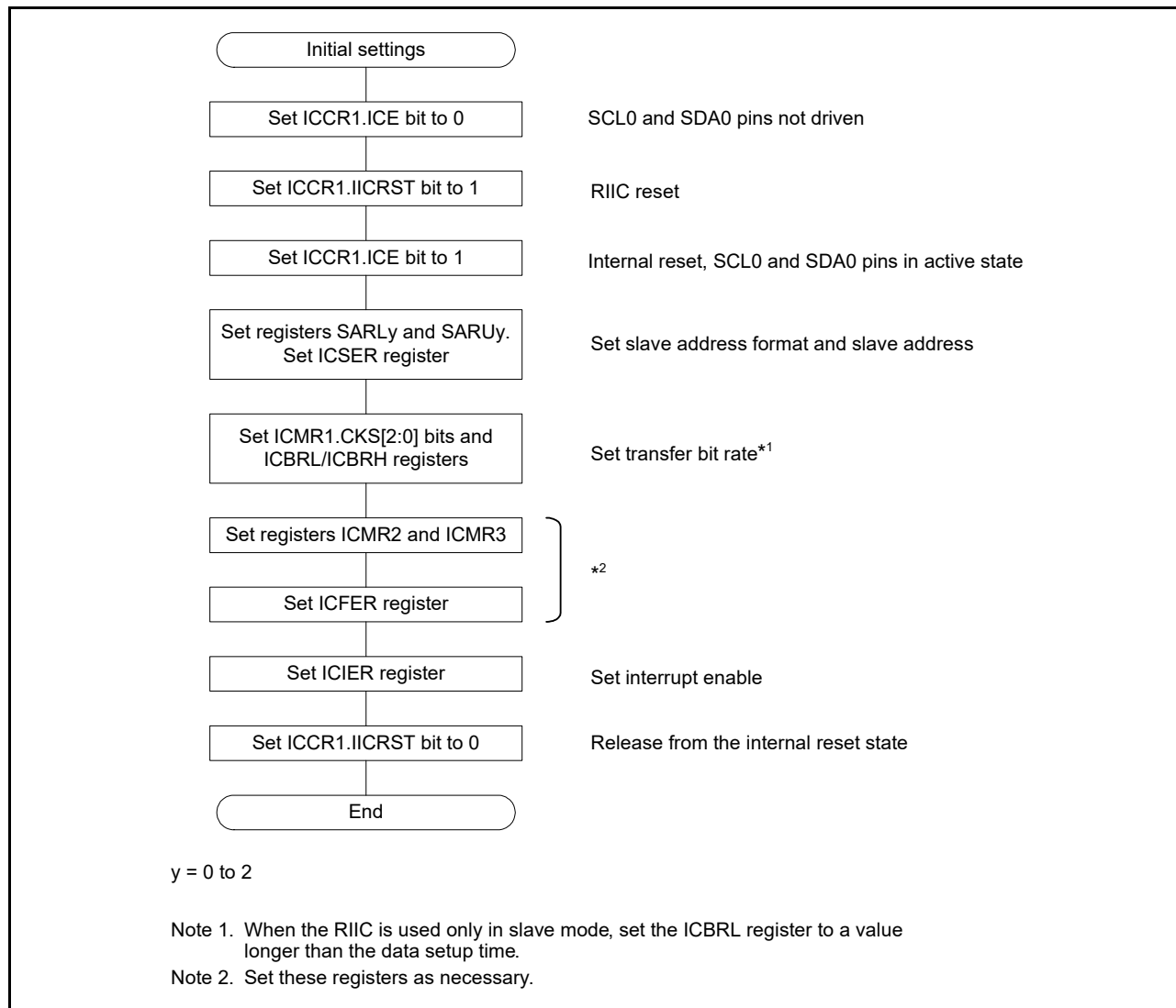
Figure 27.5 Example of RIIC Initialization Flowchart
