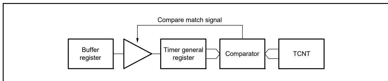
Figure 20.15 Compare Match Buffer Operation
