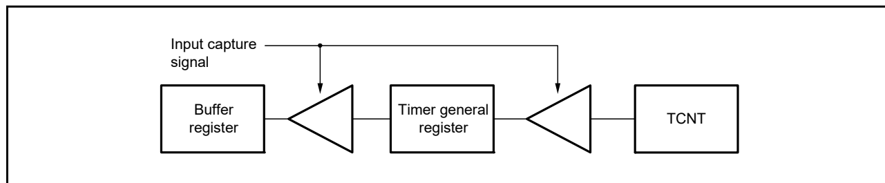
Figure 20.16 Input Capture Buffer Operation
