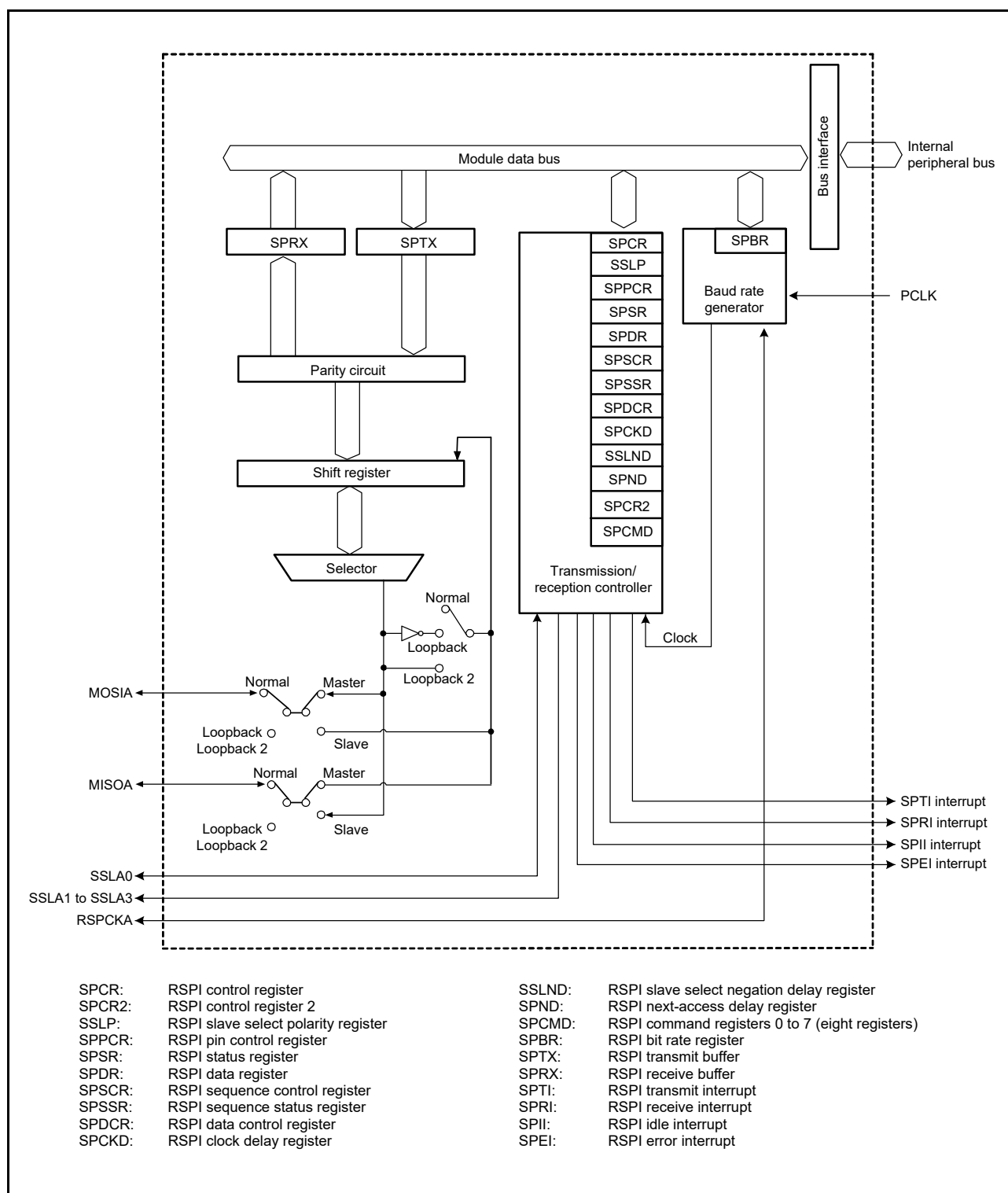
Figure 29.1 RSPI Block Diagram
