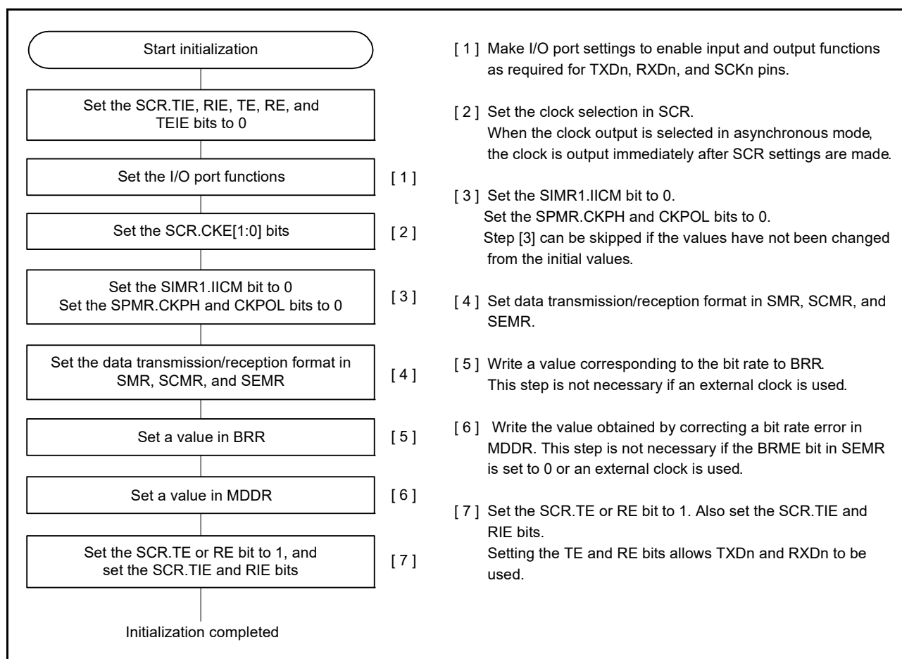
Figure 26.7 Sample SCI Initialization Flowchart (Asynchronous Mode)
