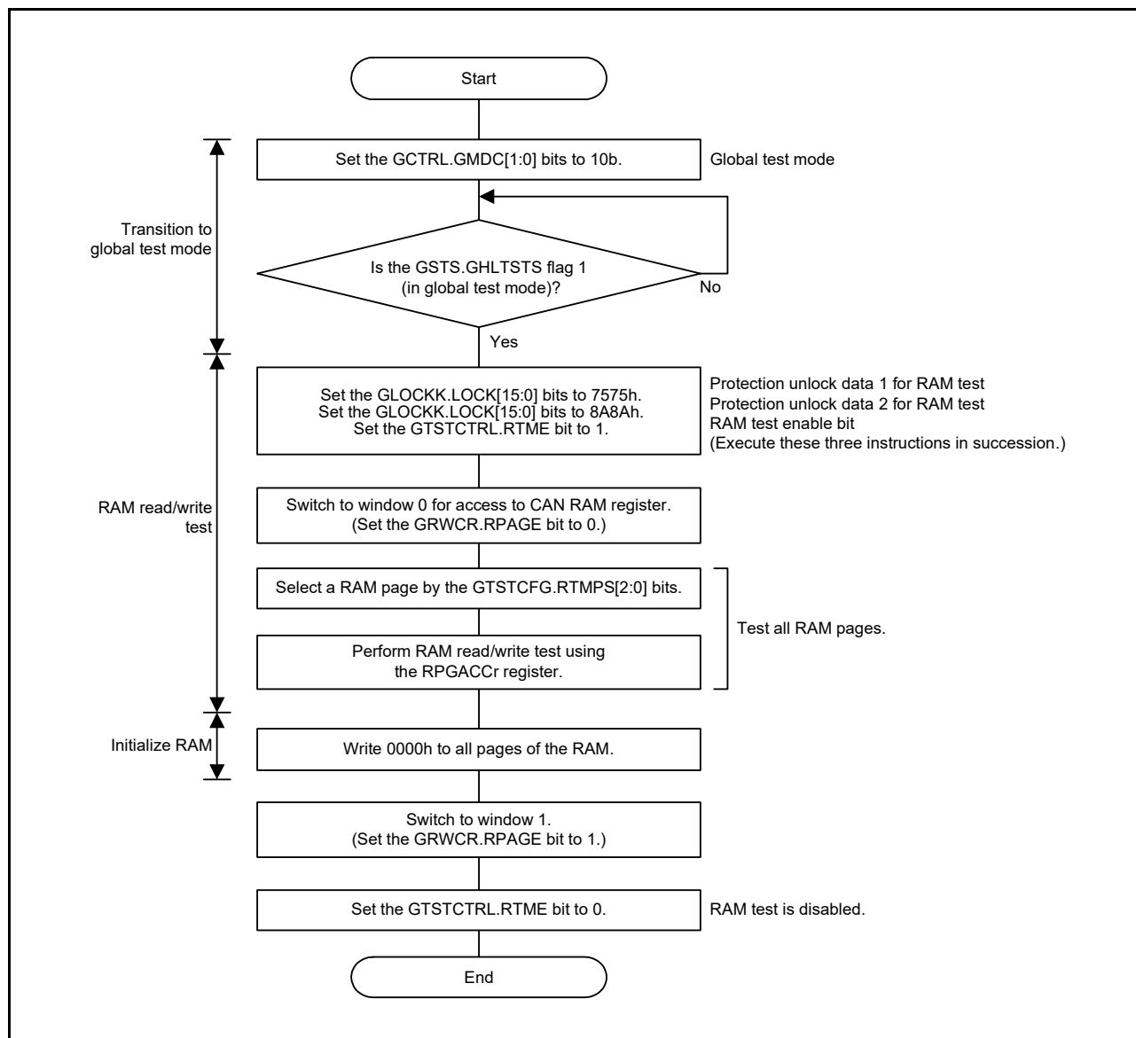
Figure 28.35 RAM Test Setting Procedure
