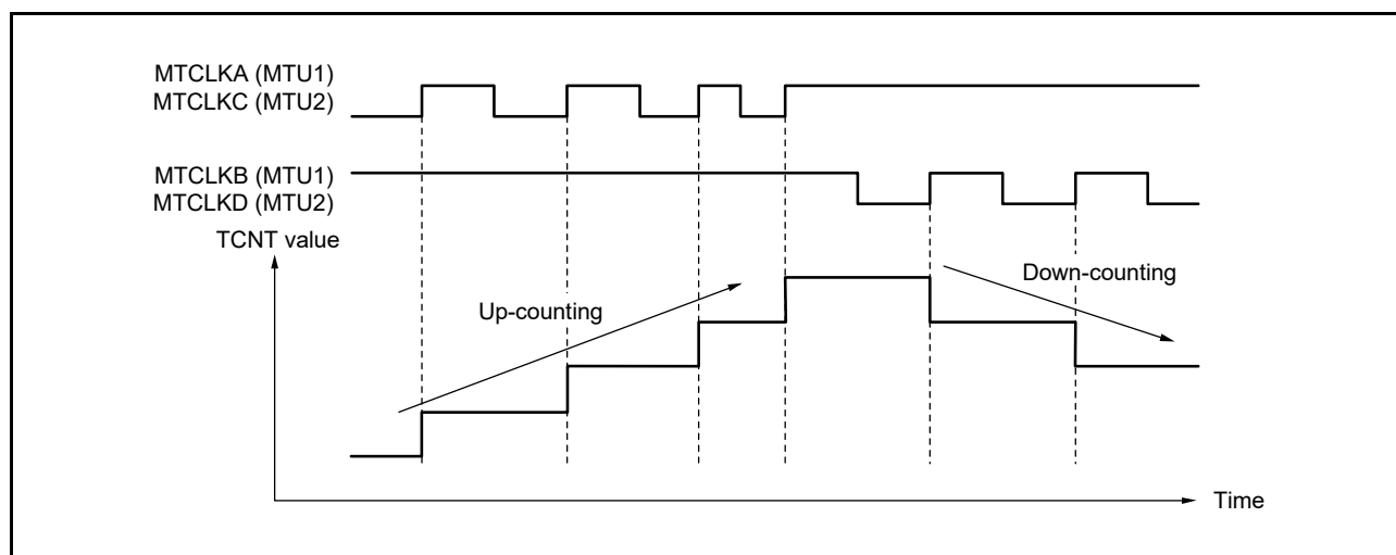
Figure 20.36 Example of Operation in Phase Counting Mode 3 (When MTUn.TCR2.PCB[1:0] = 01b ( n = 1, 2 ))
