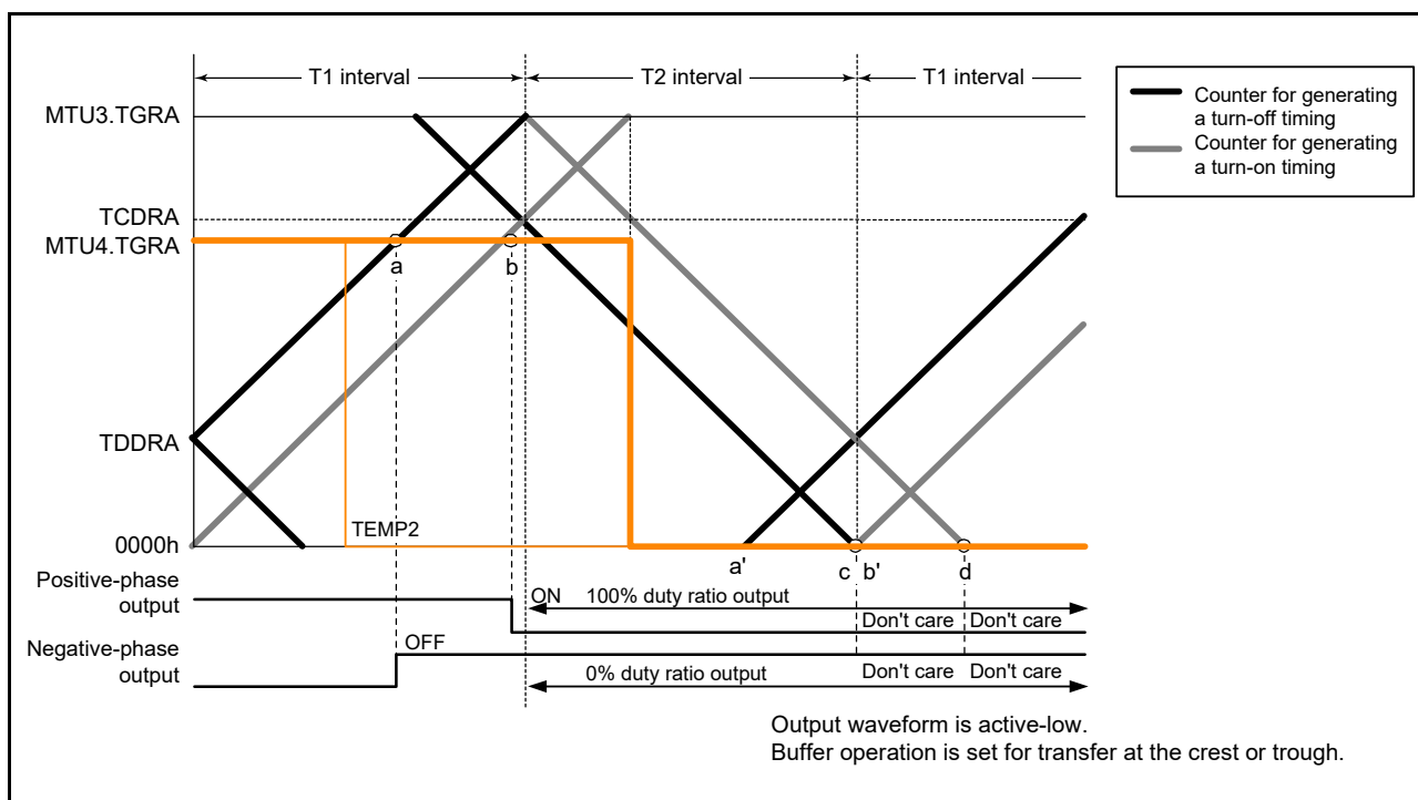
Figure 20.61 Example of 0% and 100% Waveform Output in Complementary PWM Mode (MTU3 and MTU4) (4)
