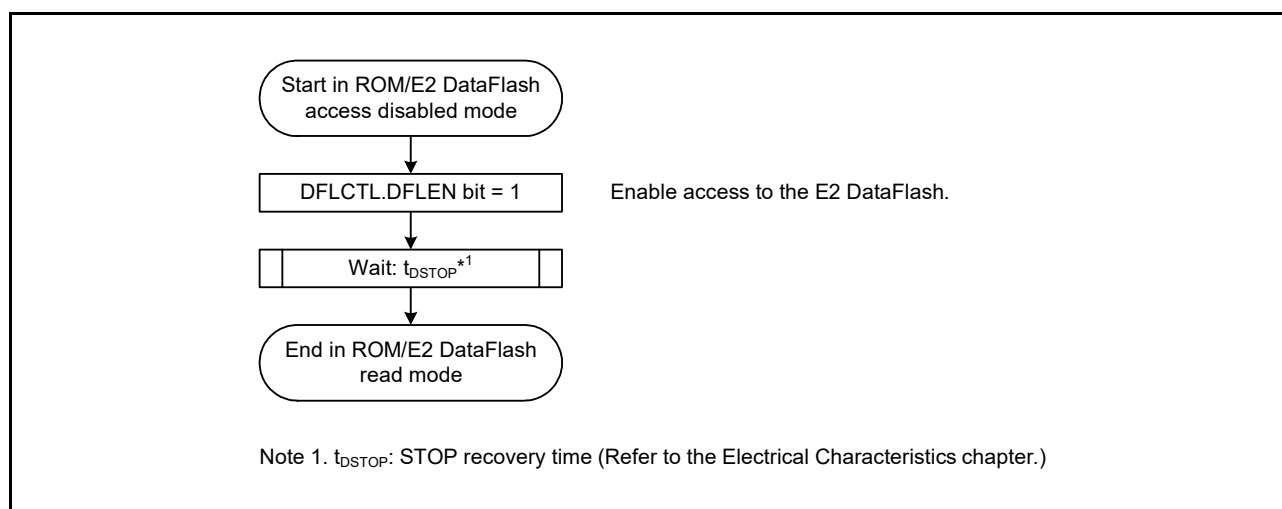
Figure 36.7 Procedure for Transition from E2 DataFlash Access Disabled Mode to ROM/E2 DataFlash Read Mode
