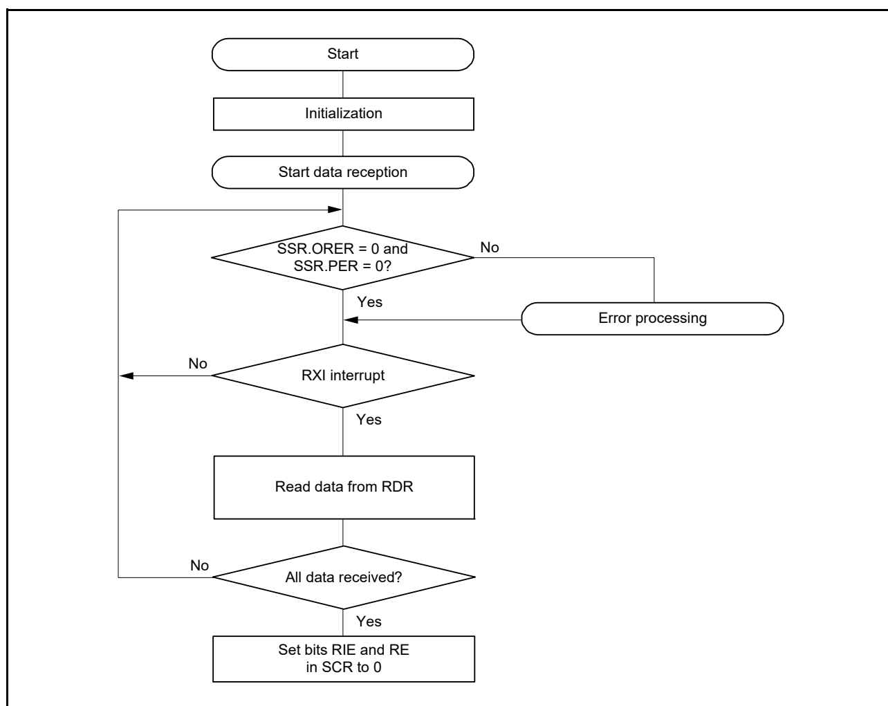
Figure 26.41 Sample Smart Card Interface Reception Flowchart
