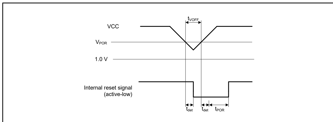
Figure 37.55 Voltage Detection Reset Timing
