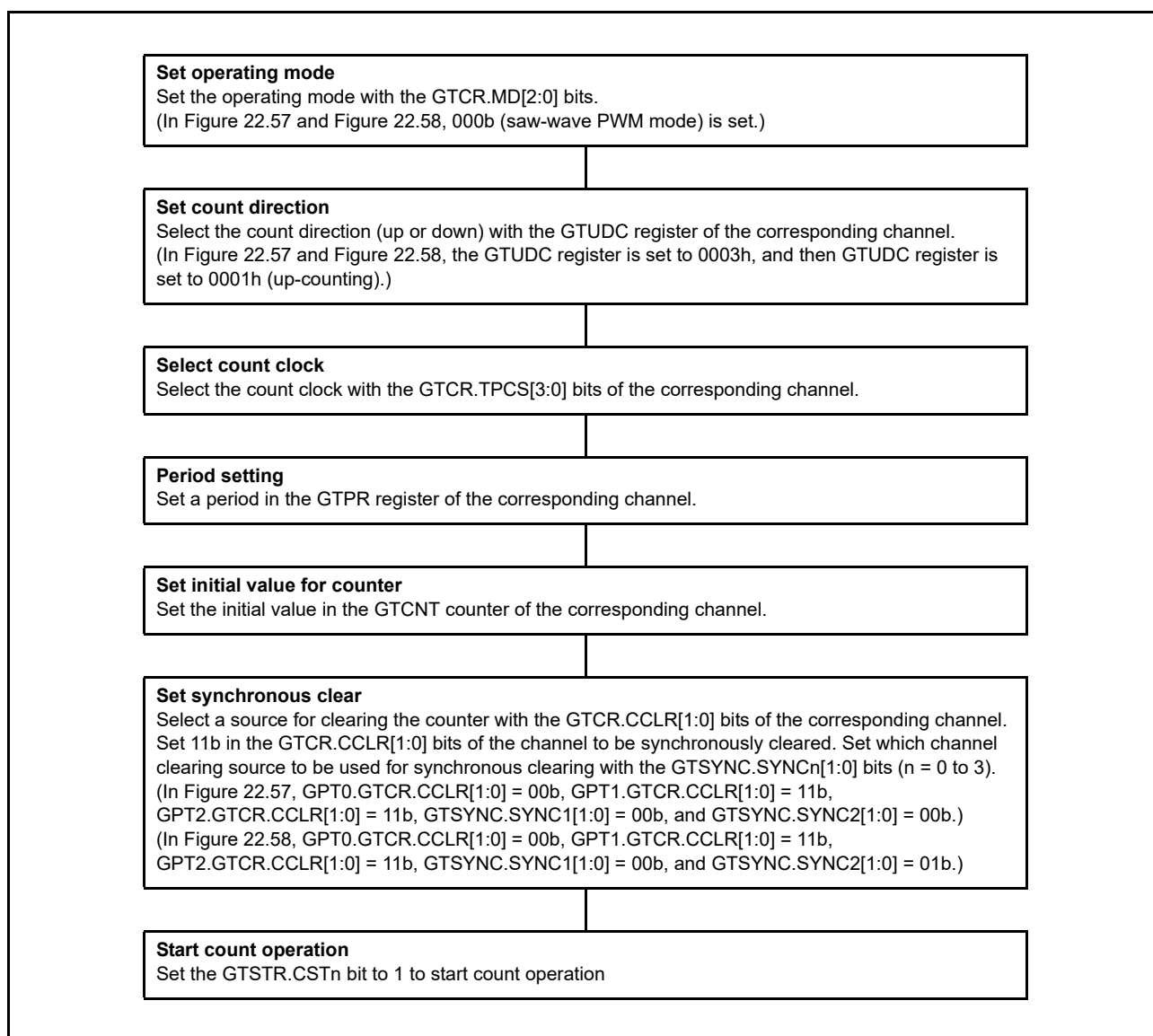
Figure 22.59 Example for Setting Synchronous Clear Operation
