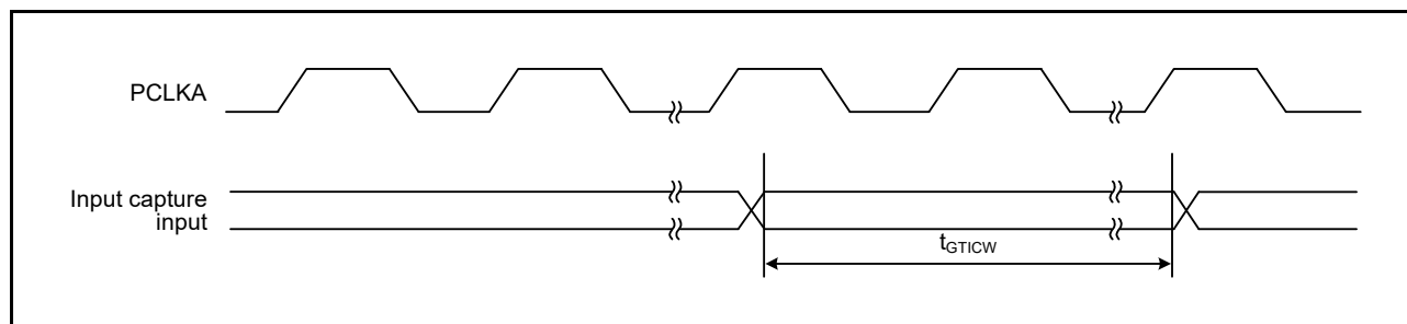
Figure 37.40 Input Timing of GPT Input Capture
