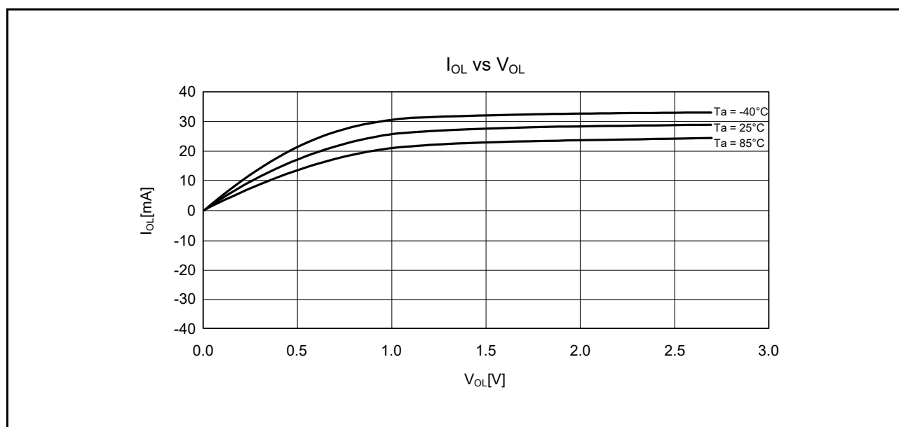
Figure 37.19 V_{OL} and I_{OL} Temperature Characteristics of RIIC Output Pin at V_{CC} = 2.7\text{ V} (Reference Data)
