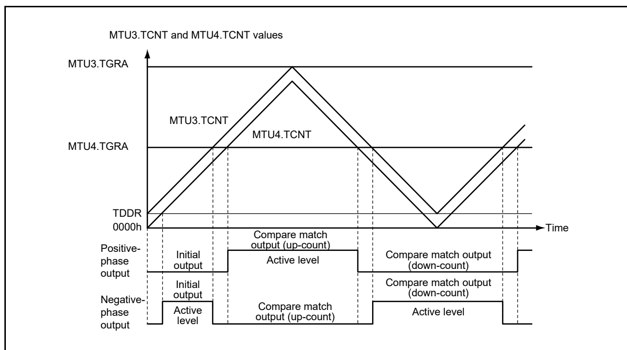
Figure 20.3 Example of Output in Complementary PWM Mode
