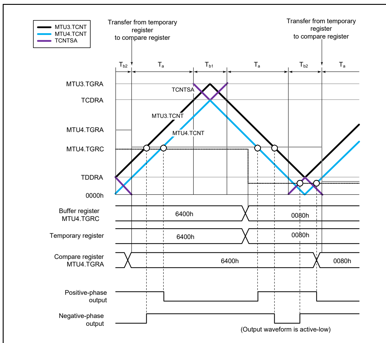
Figure 20.49 Example of Operation in Complementary PWM Mode (MTU3 and MTU4)
