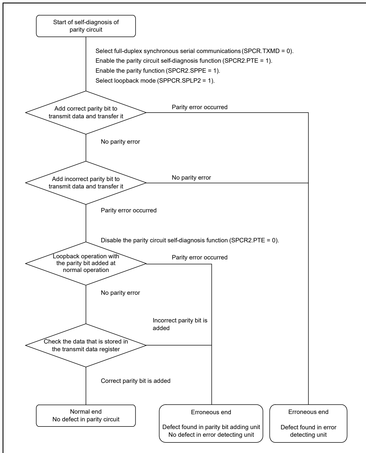
Figure 29.49 Flowchart for Self-Diagnosis of Parity Circuit
