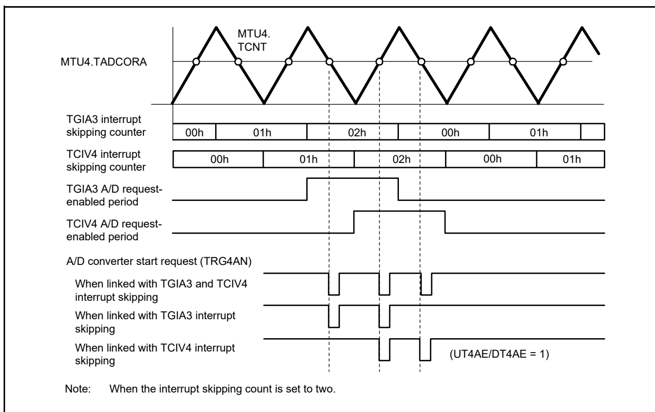
Figure 20.94 Example of A/D Converter Start Request Signal (TRG4AN) Operation Linked with Interrupt Skipping Function 1 (UT4AE and DT4AE = 1)
