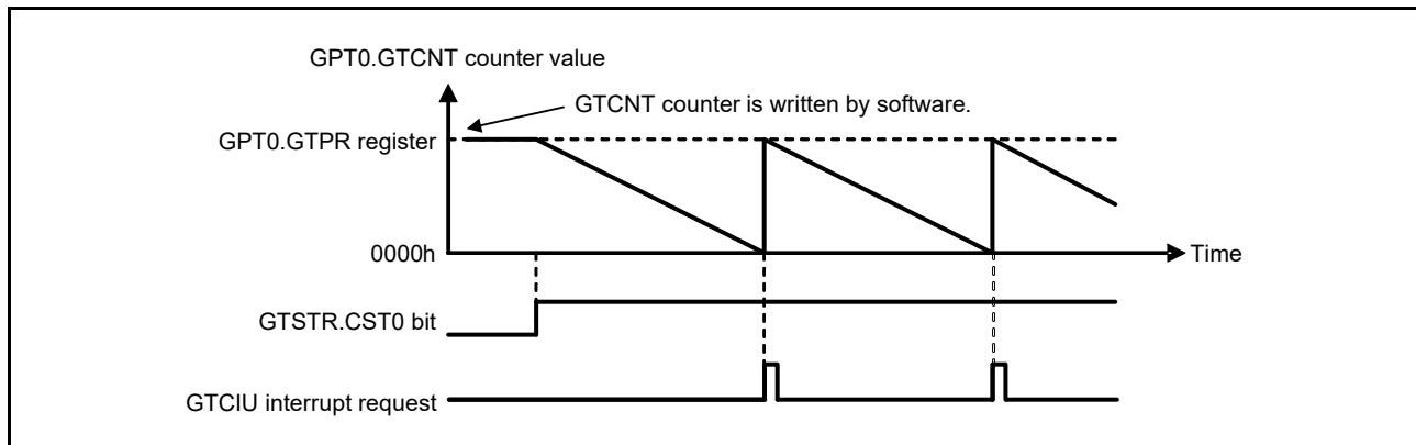
Figure 22.5 Example of Periodic Count Operation (in Down-Counting)
