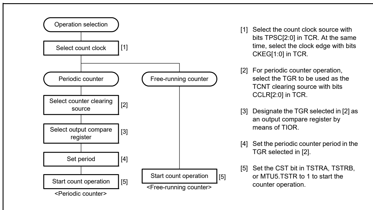
Figure 20.5 Example of Counter Operation Setting Procedure
