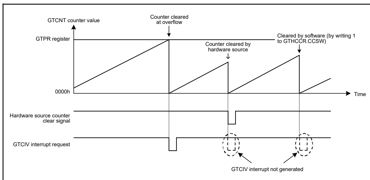
Figure 22.56 Relationship between Counter Clearing by Hardware Source and GTCIV Interrupt
