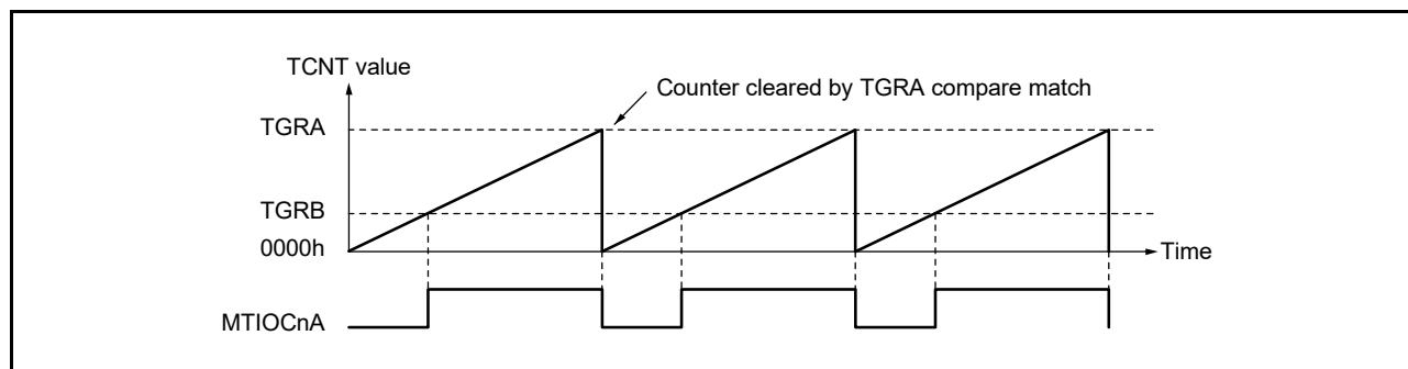
Figure 20.27 Example of PWM Mode 1 Operation (n = 0 to 4, 6, 7, 9)
