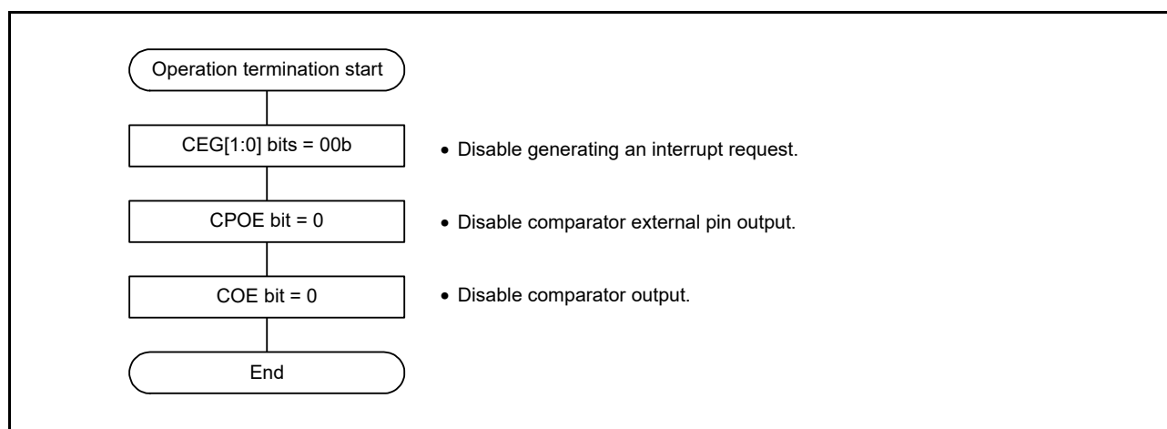
Figure 33.7 Comparator Operation Termination Flowchart
