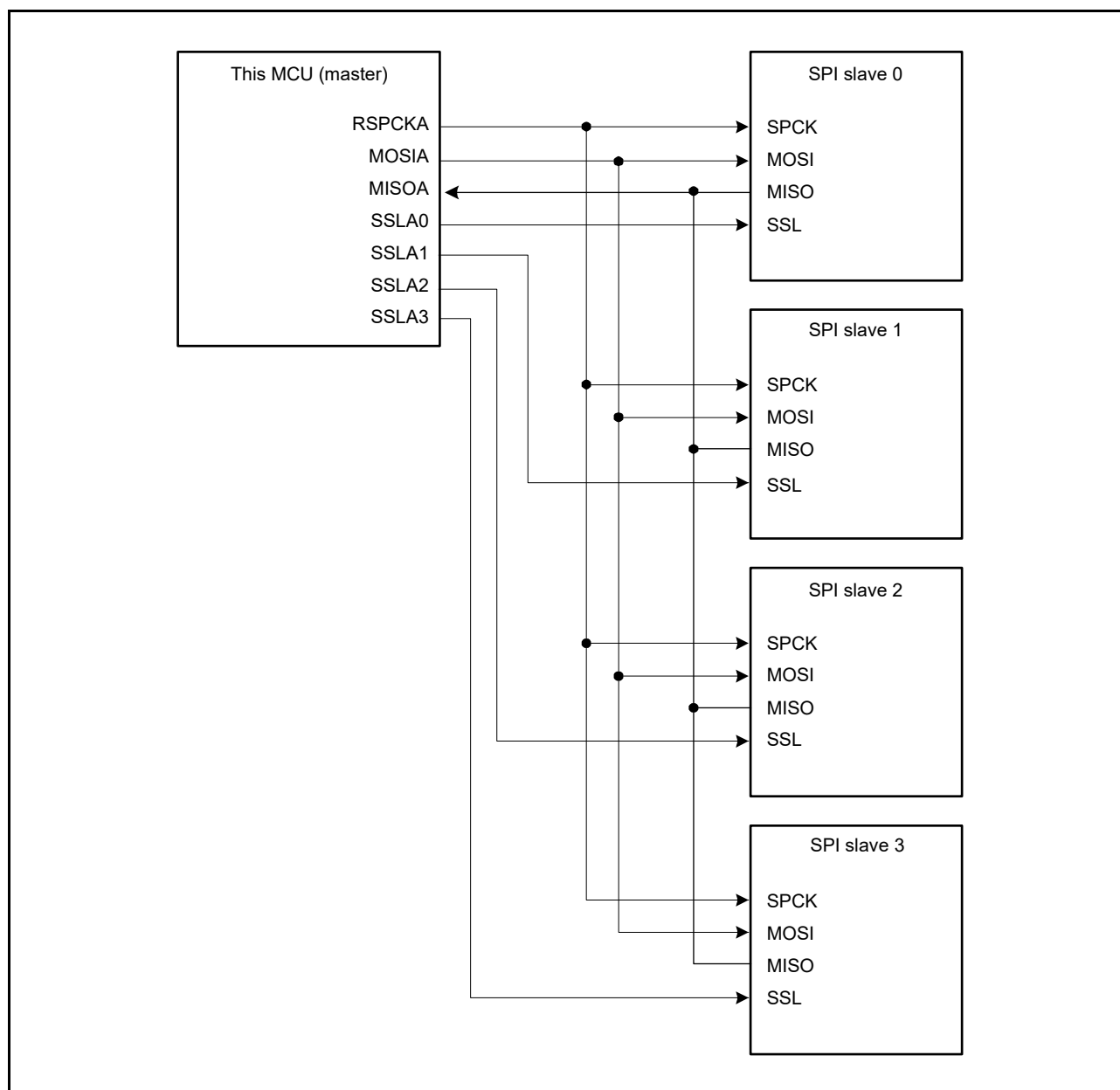
Figure 29.8 Single-Master/Multi-Slave Configuration Example (This MCU = Master)
