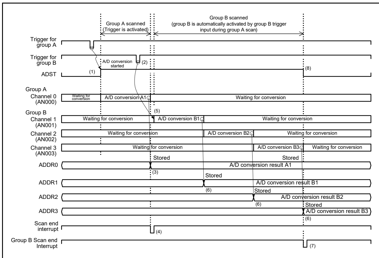
Figure 31.21 Example 3 of Group Priority Operation: Group B Trigger Input during Group A Scan, With Rescan Setting (ADGPSCR.GBRSCN = 1, ADGPSCR.GBRP = 0, ADGPSCR.LGRRS = 0)
