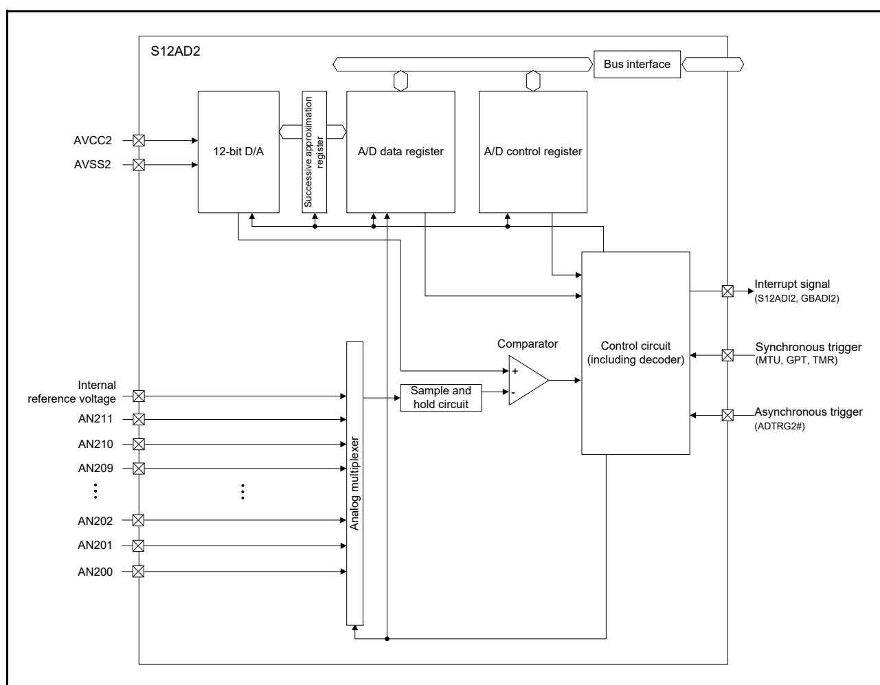
Figure 31.3 Block Diagram of 12-Bit A/D Converter (Unit 2)
