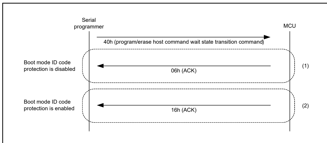
Figure 36.34 Procedure to Enter the Program/Erase Host Command Wait State
