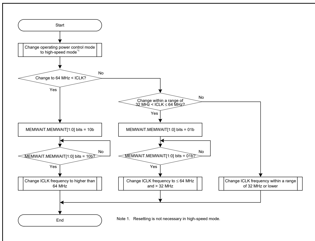
Figure 9.2 Example of Setting Procedure When Changing the Current ICLK Frequency to a Higher Frequency
