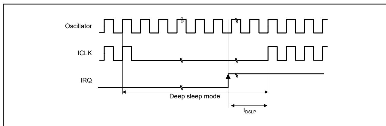
Figure 37.33 Deep Sleep Mode Recovery Timing
