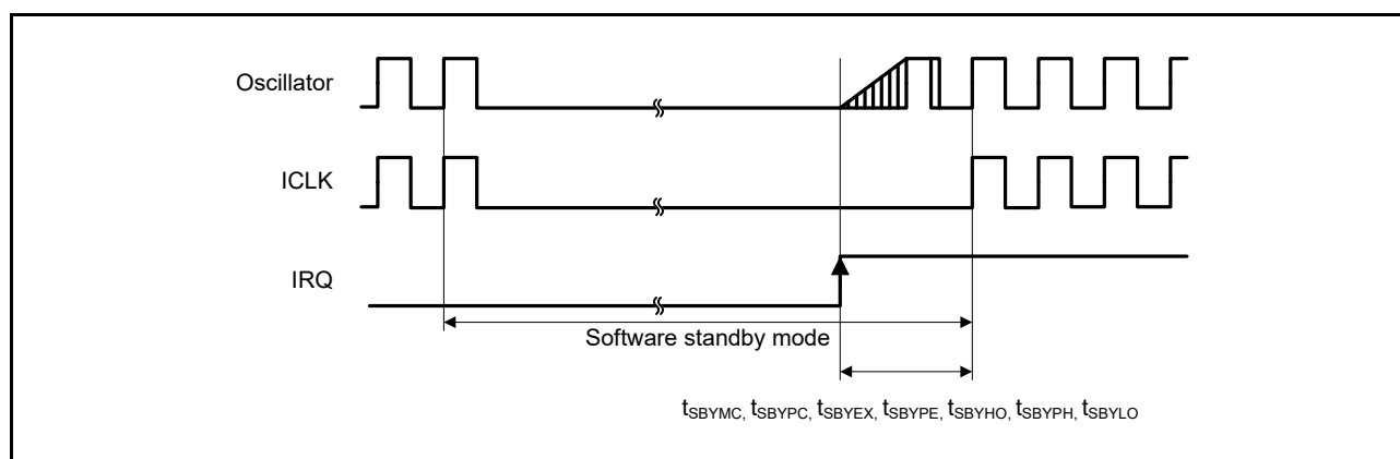
Figure 37.32 Software Standby Mode Recovery Timing
