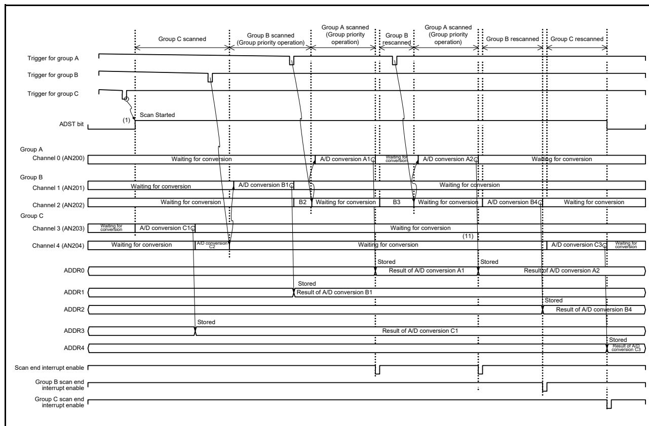
Figure 31.25 Example 2 of Group Priority Operation: Priority Group Trigger Input during Low-Priority Group Rescan, With Rescan Setting (ADGSPCR.GBRSCN = 1, ADGSPCR.GBRP = 0, ADGSPCR.LGRRS = 1)
