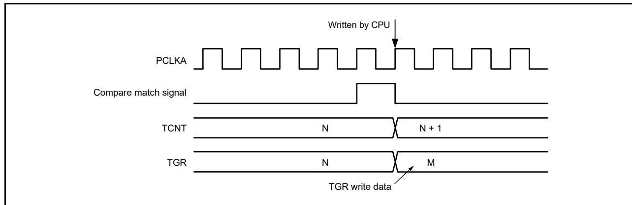
Figure 20.136 Contention between TGR Write Operation and Compare Match
