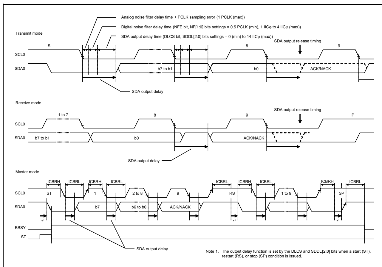
Figure 27.22 SDA Output Delay Function
