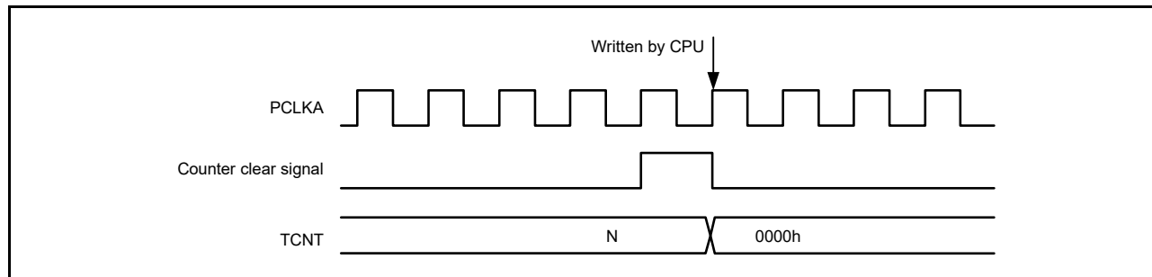
Figure 20.134 Contention between TCNT Write and Clear Operations
