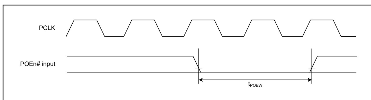
Figure 37.39 POE# Input Timing
