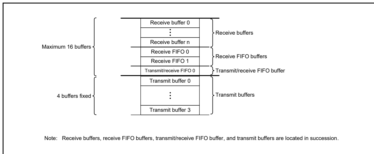
Figure 28.20 Buffer Configuration
