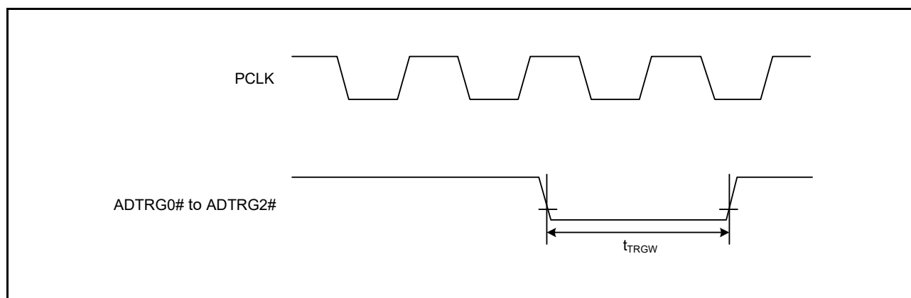
Figure 37.46 A/D Converter External Trigger Input Timing
