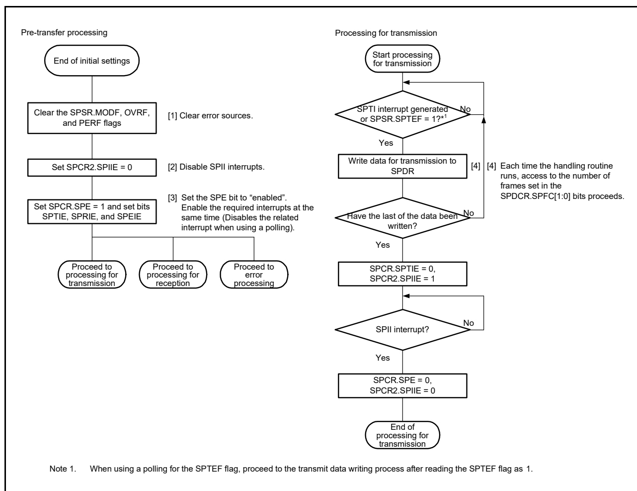
Figure 29.36 Flowchart in Master Mode (Transmission)
