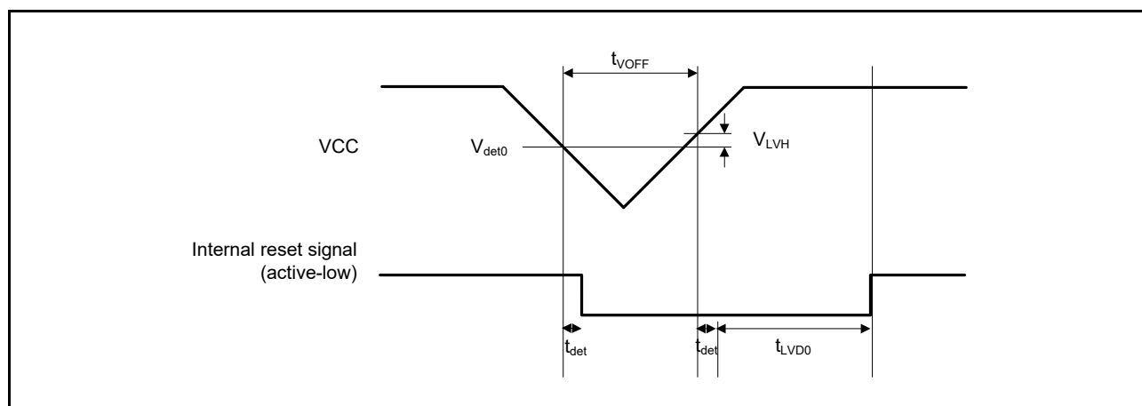
Figure 37.57 Voltage Detection Circuit Timing (Vdet0)
