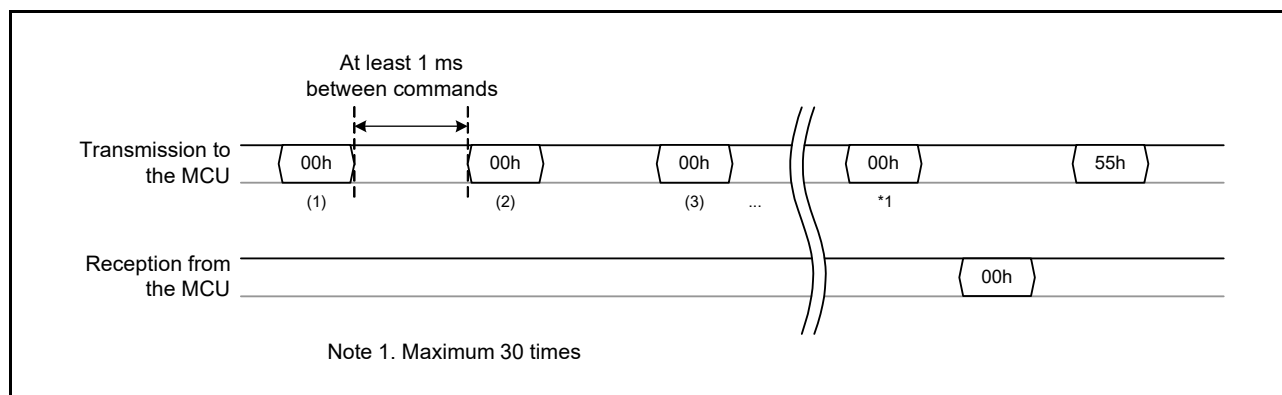
Figure 36.30 Transmit/Receive Data for Bit Rate Automatic Adjustment
