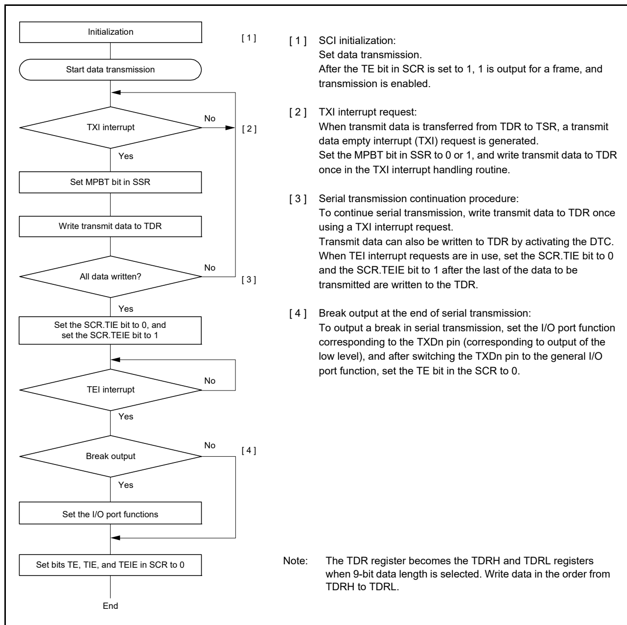
Figure 26.17 Example of Multi-Processor Serial Transmission Flowchart
