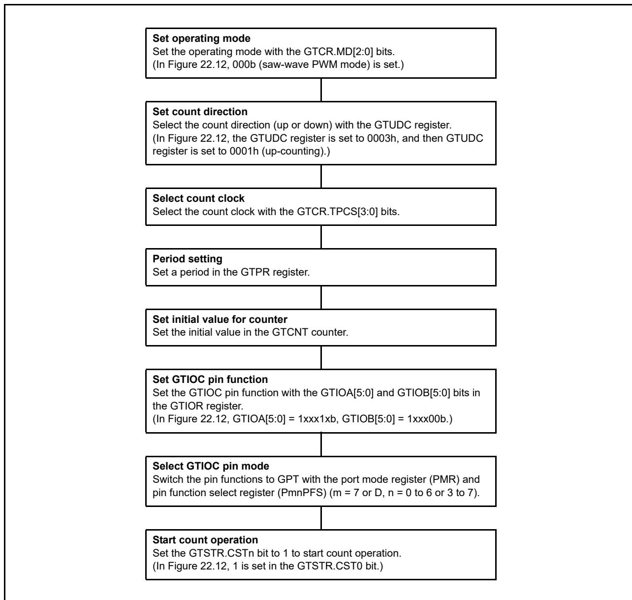
Figure 22.13 Example for Setting Input Capture Operation
