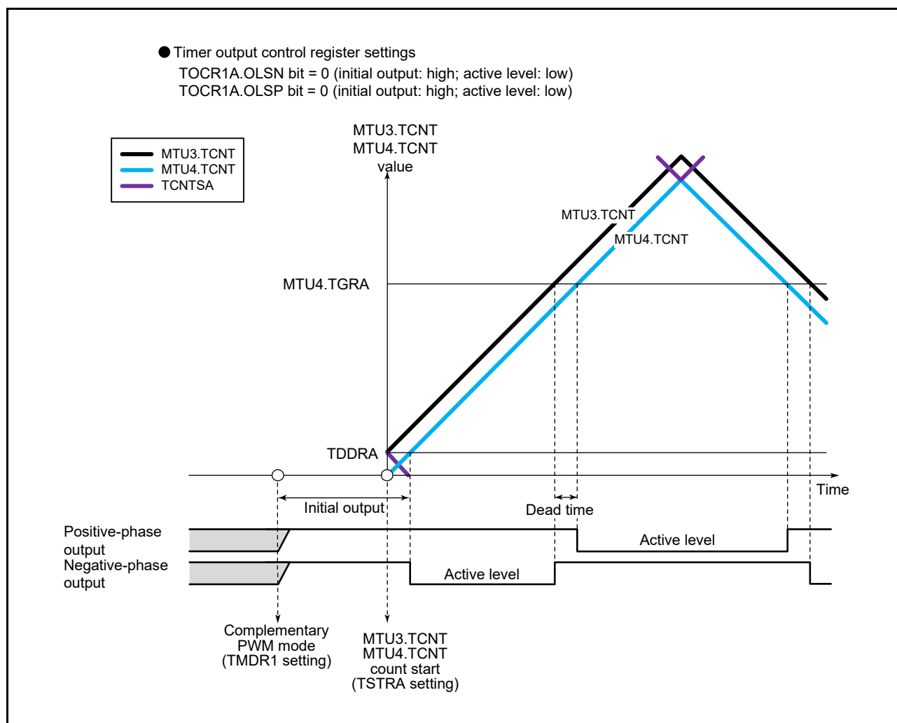
Figure 20.53 Example of Initial Output in Complementary PWM Mode (MTU3 and MTU4) (1))
