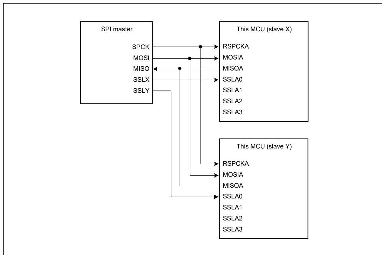
Figure 29.9 Single-Master/Multi-Slave Configuration Example (This MCU = Slave)
