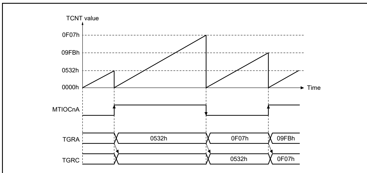
Figure 20.19 Example of Buffer Operation (2) (n = 0 to 4, 6, 7, 9)
