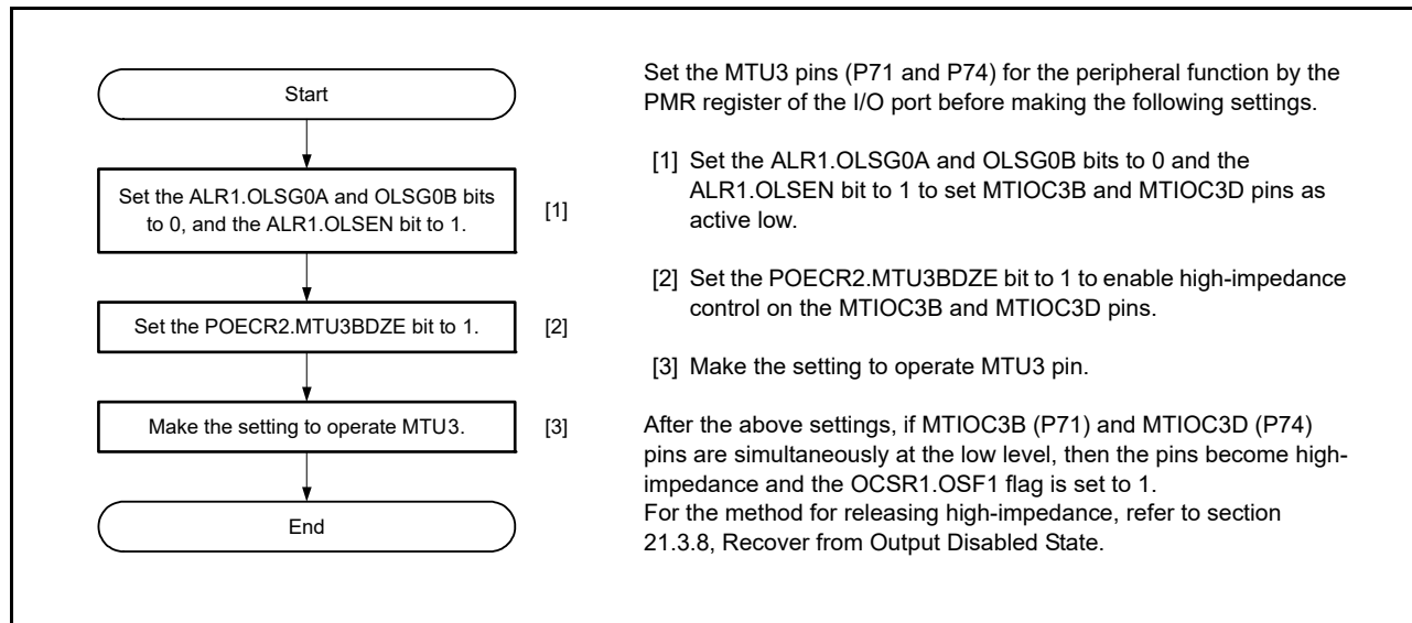
Figure 21.13 Procedure for Setting the POE
