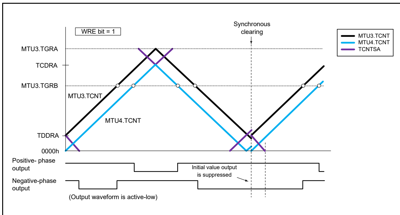
Figure 20.70 Example of Synchronous Clearing in Tb2 interval (Timing (11) in Figure 20.65; TWCRA.WRE Bit is 1)
