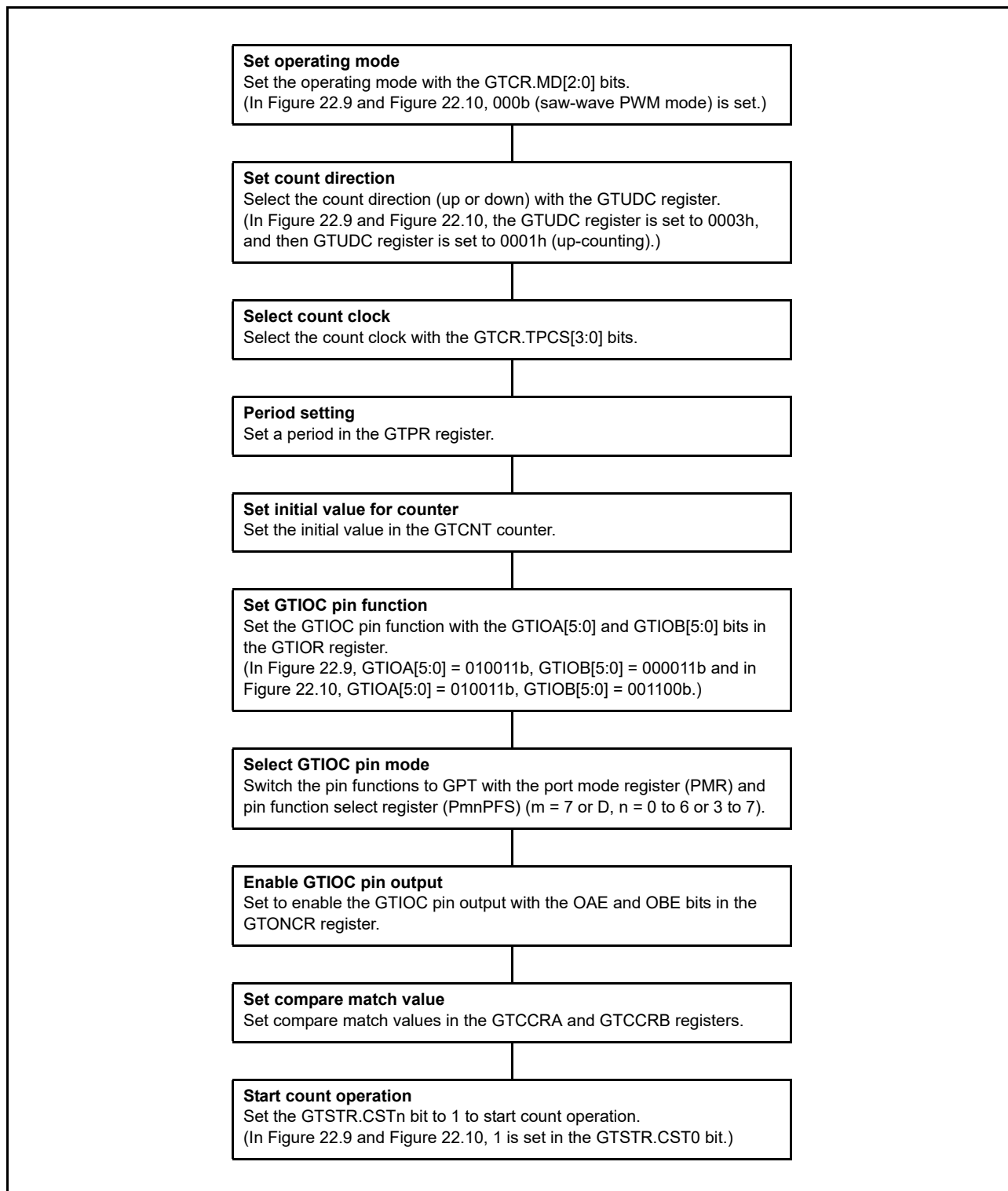
Figure 22.11 Example for Setting Toggled Output Operation
