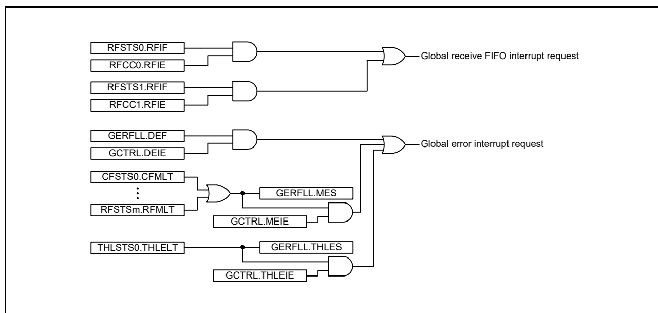
Figure 28.13 CAN Global Interrupt Block Diagram
