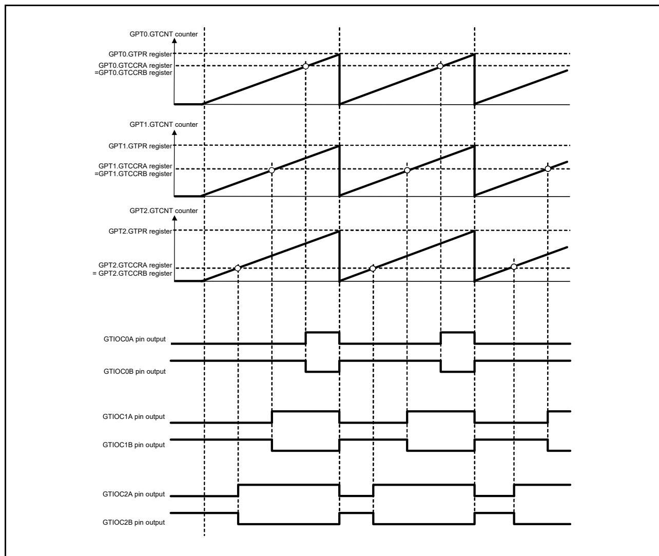
Figure 22.67 Example of Three-Phase Saw-Wave Complementary PWM Output
