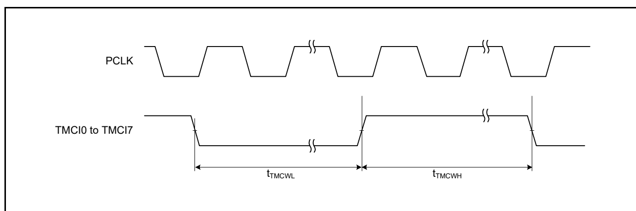
Figure 37.43 TMR Clock Input Timing
