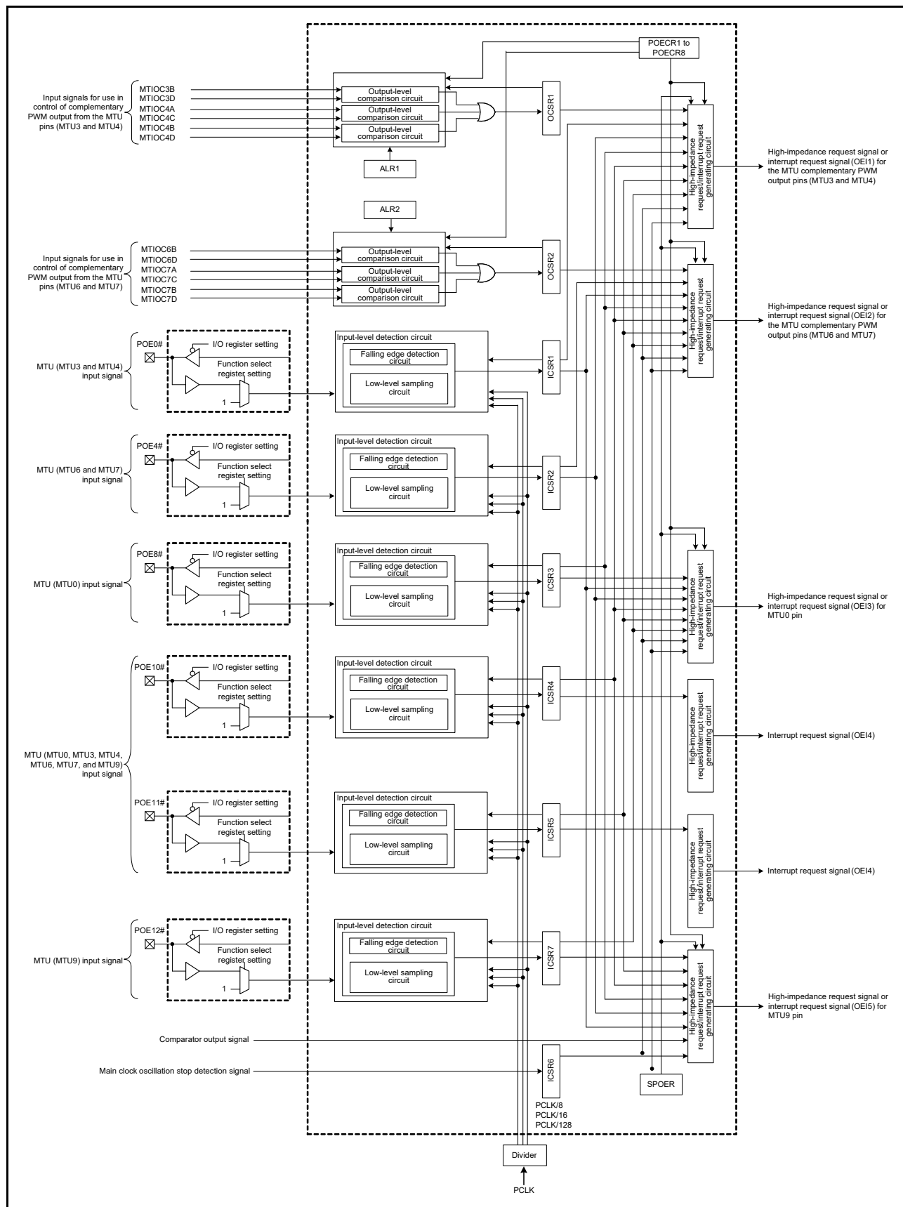
Figure 21.1 POE Block Diagram (Chip Version A)
