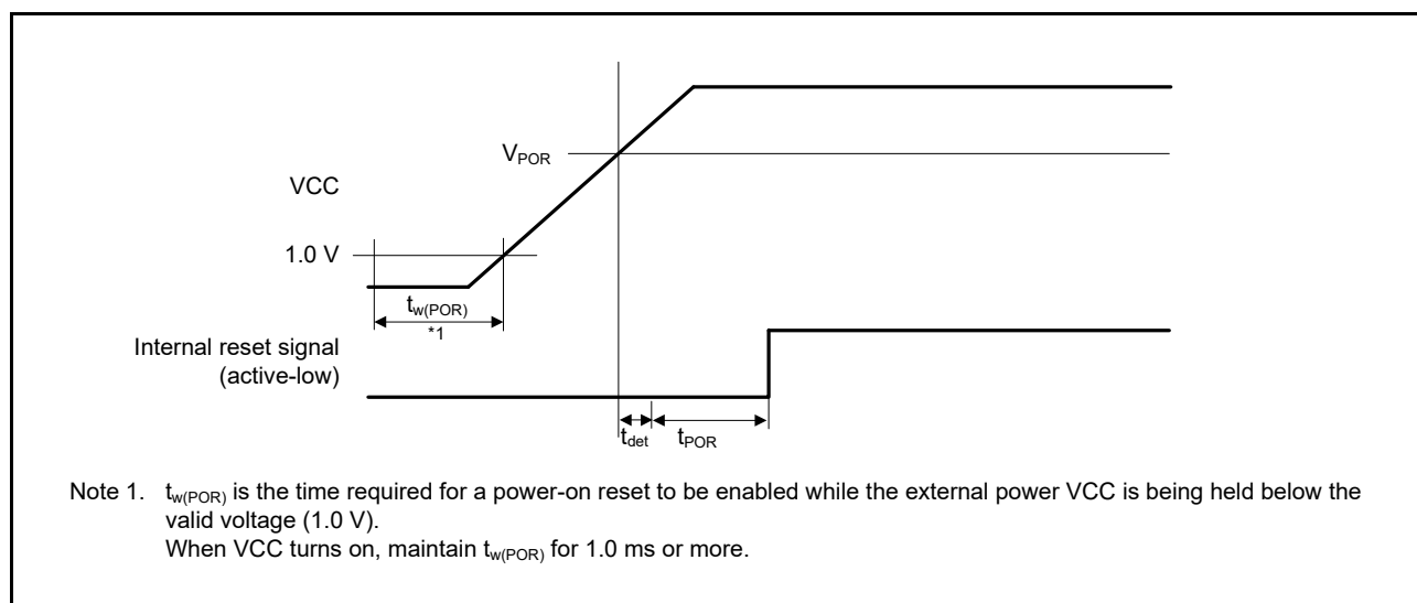
Figure 37.56 Power-On Reset Timing
