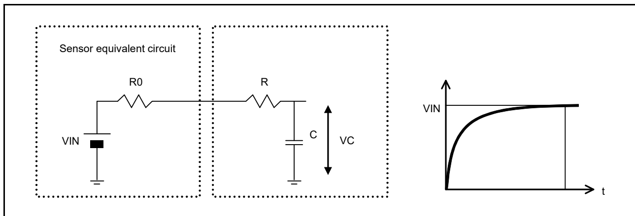
Figure 31.35 Equivalent Circuit of Analog Input Pin and External Sensor
