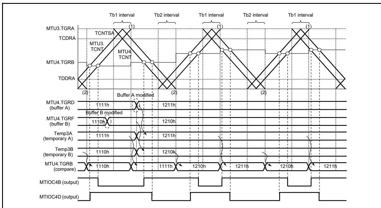
Figure 20.82 Example of Double Buffer Operation
