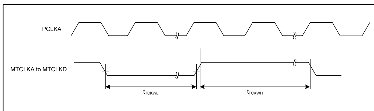
Figure 37.38 MTU3 Clock Input Timing
