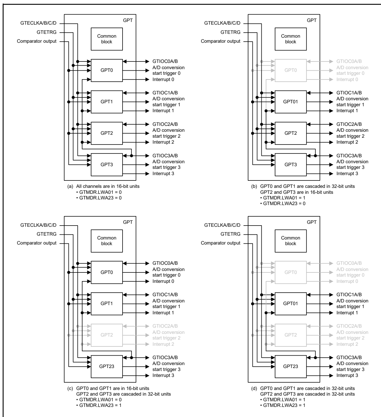
Figure 22.2 Timer Configurations
