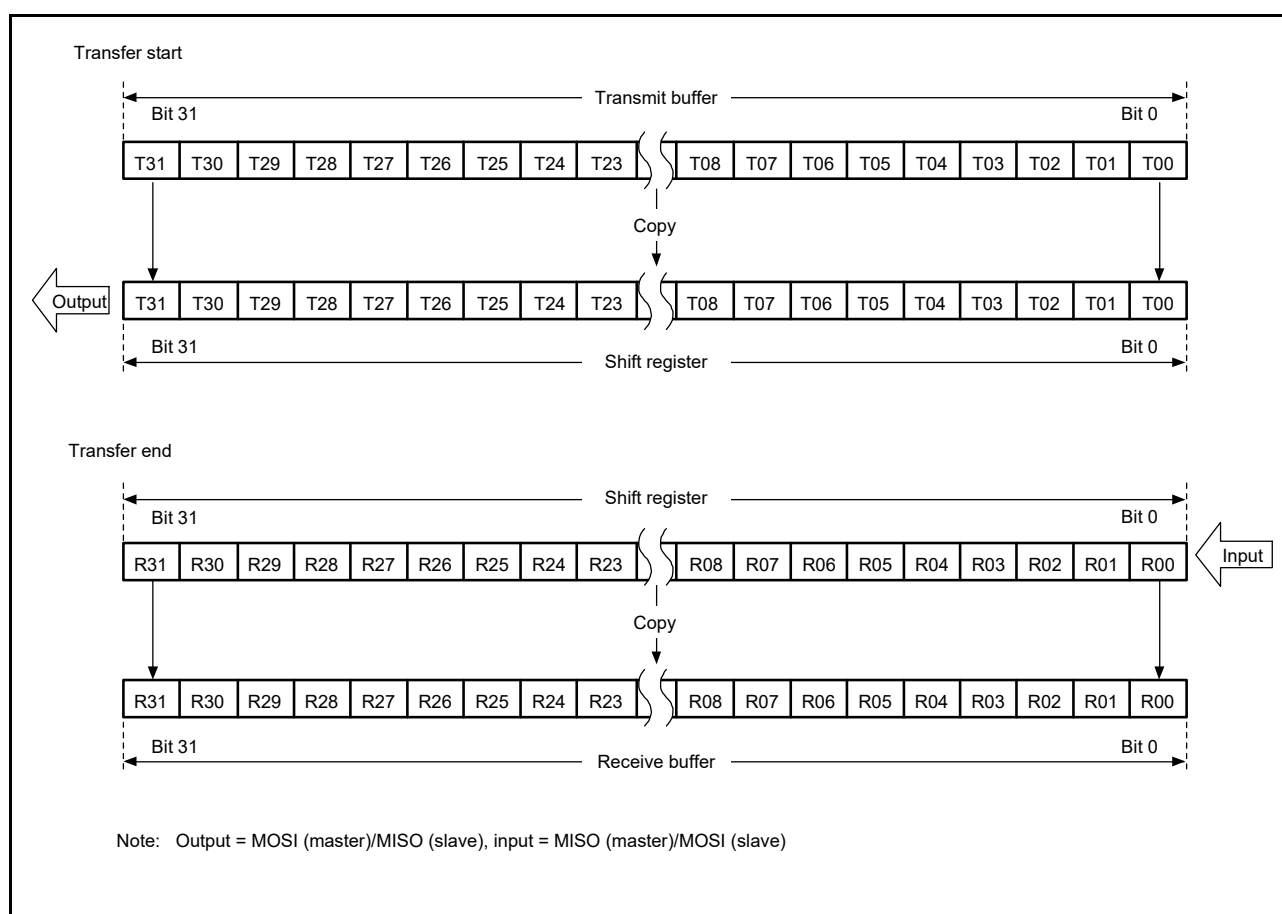
Figure 29.14 MSB First Transfer (32-Bit Data, Parity Disabled)
