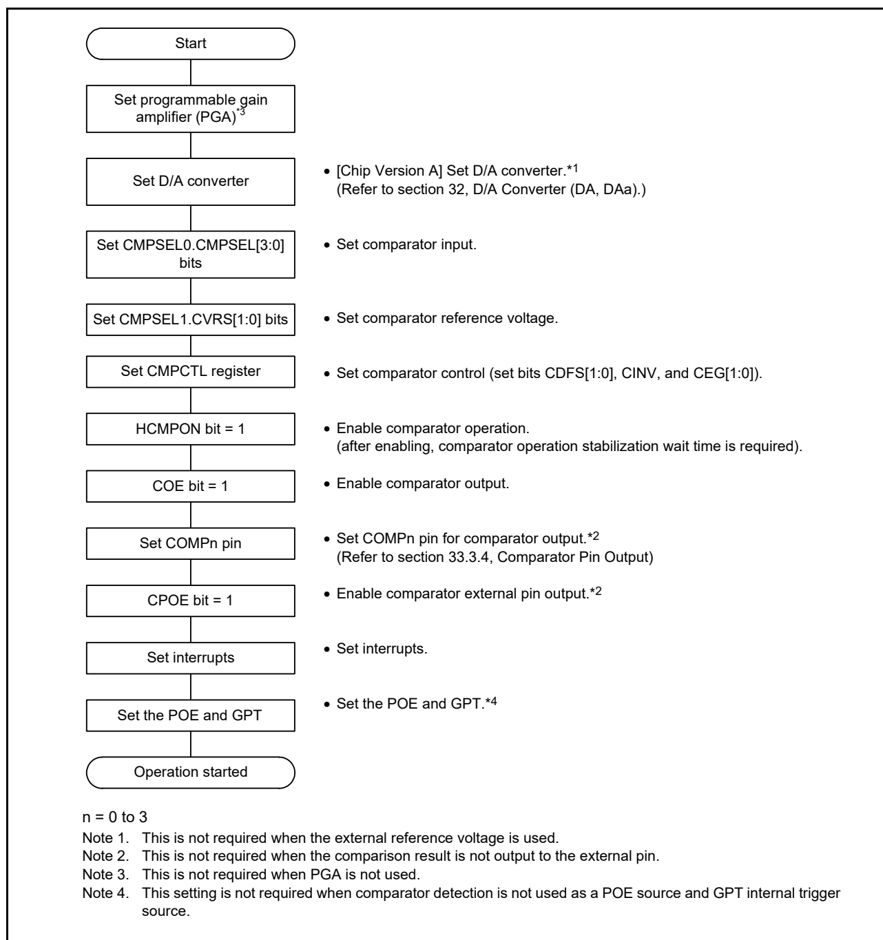
Figure 33.6 Comparator Operation Setting Flowchart
