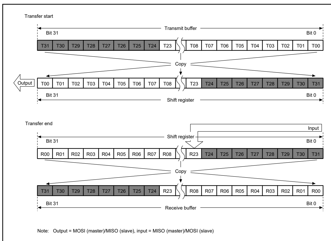
Figure 29.17 LSB First Transfer (24-Bit Data, Parity Disabled)
