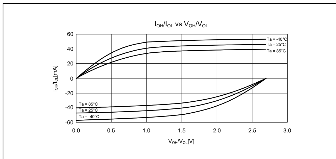
Figure 37.15 V_{OH}/V_{OL} and I_{OH}/I_{OL} Temperature Characteristics of Large Current Ports at V_{CC} = 2.7\text{ V} (Reference Data)
