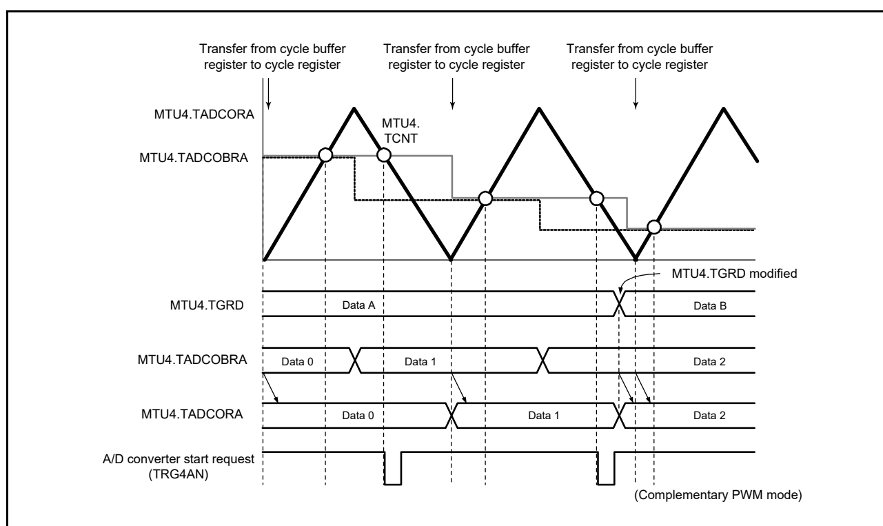
Figure 20.93 Example of A/D Converter Start Request Signal (TRG4AN) and Buffer Transfer Operation
