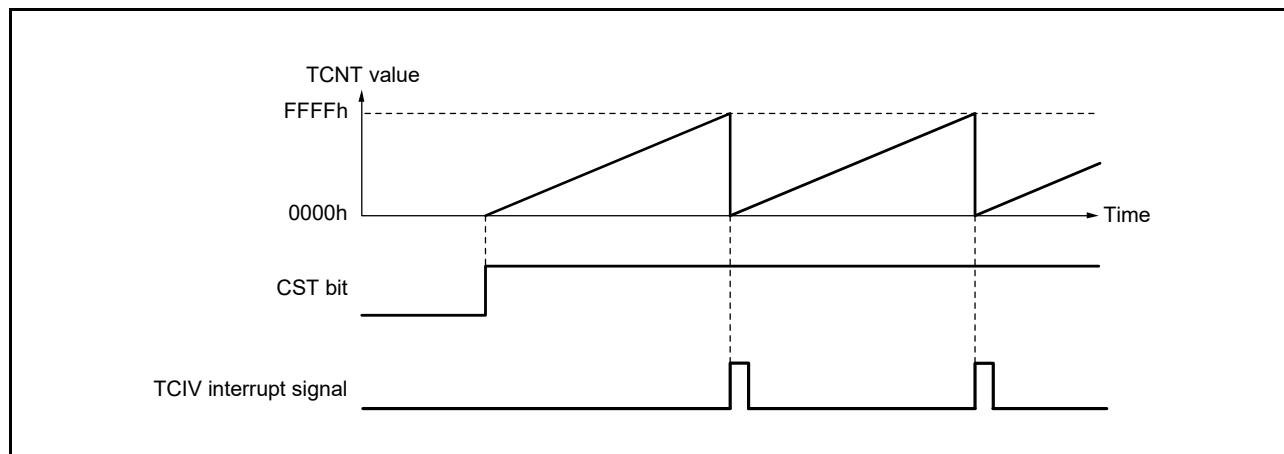
Figure 20.6 Free-Running Counter Operation
