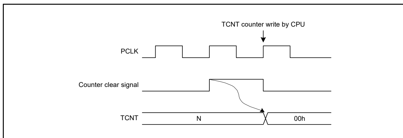
Figure 23.15 Conflict between TCNT Write and Counter Clear
