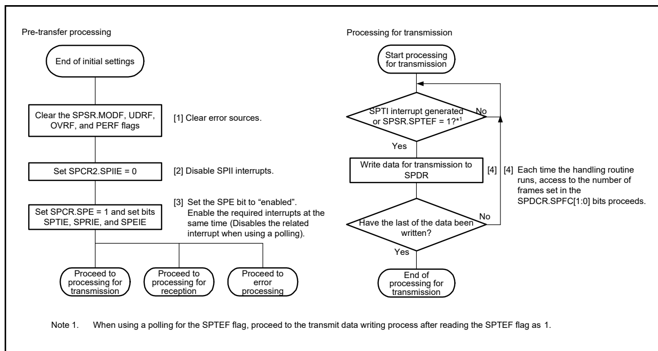
Figure 29.40 Flowchart in Slave Mode (Transmission)
