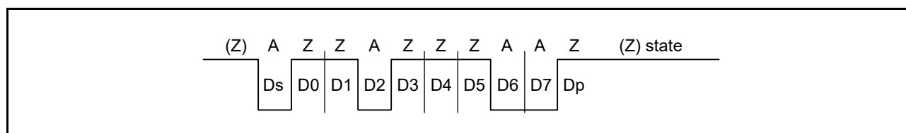
Figure 26.33 Direct Convention (SDIR in SCMR = 0, SINV in SCMR = 0, PM in SMR = 0)
