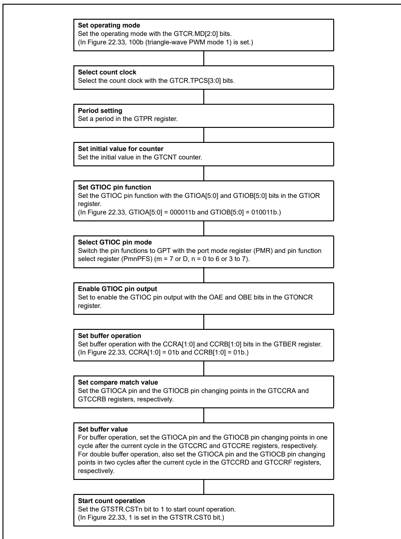
Figure 22.34 Example for Setting Triangle-Wave PWM Mode 1
