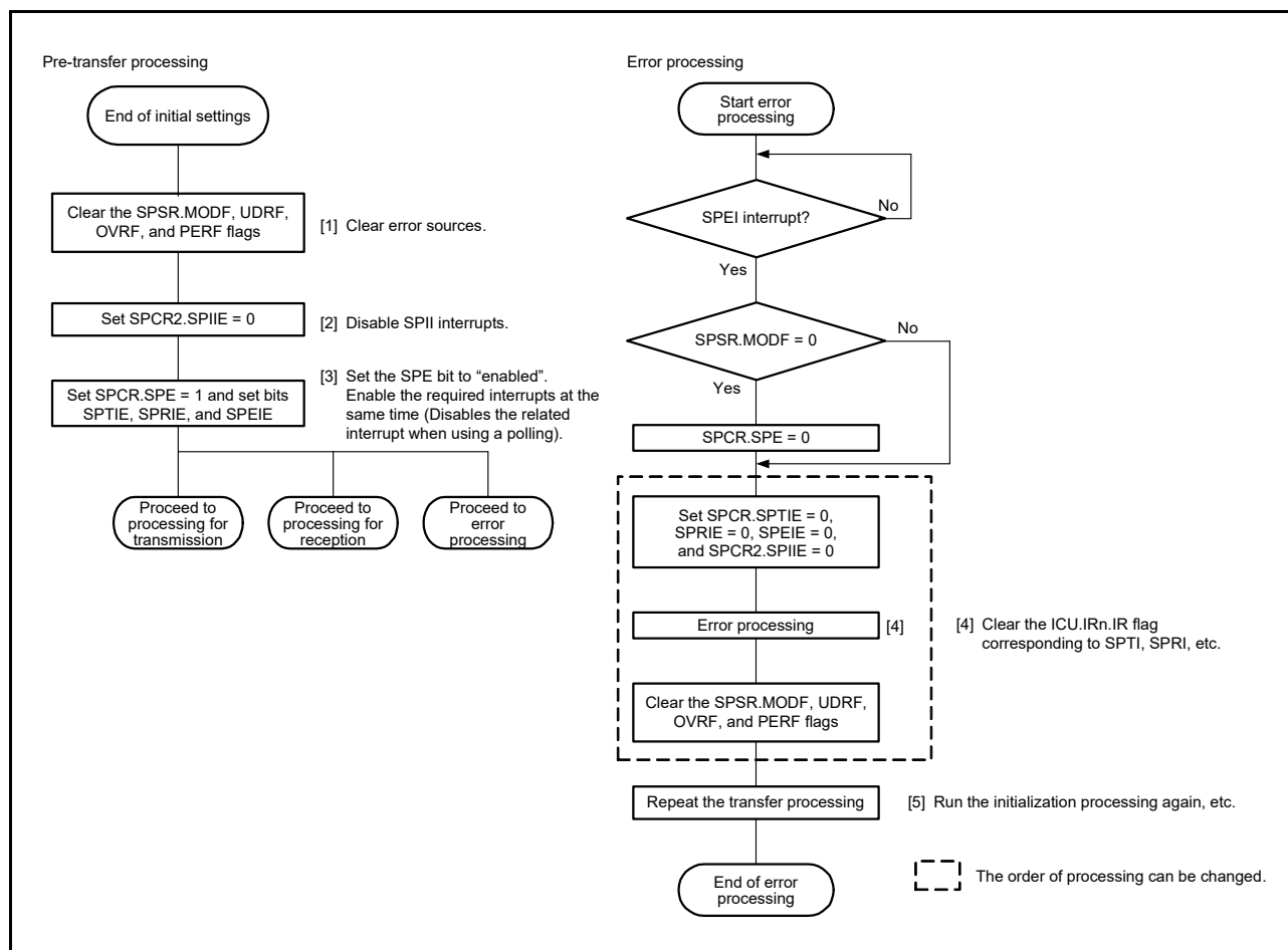
Figure 29.42 Flowchart for Slave Mode (Error Processing)
