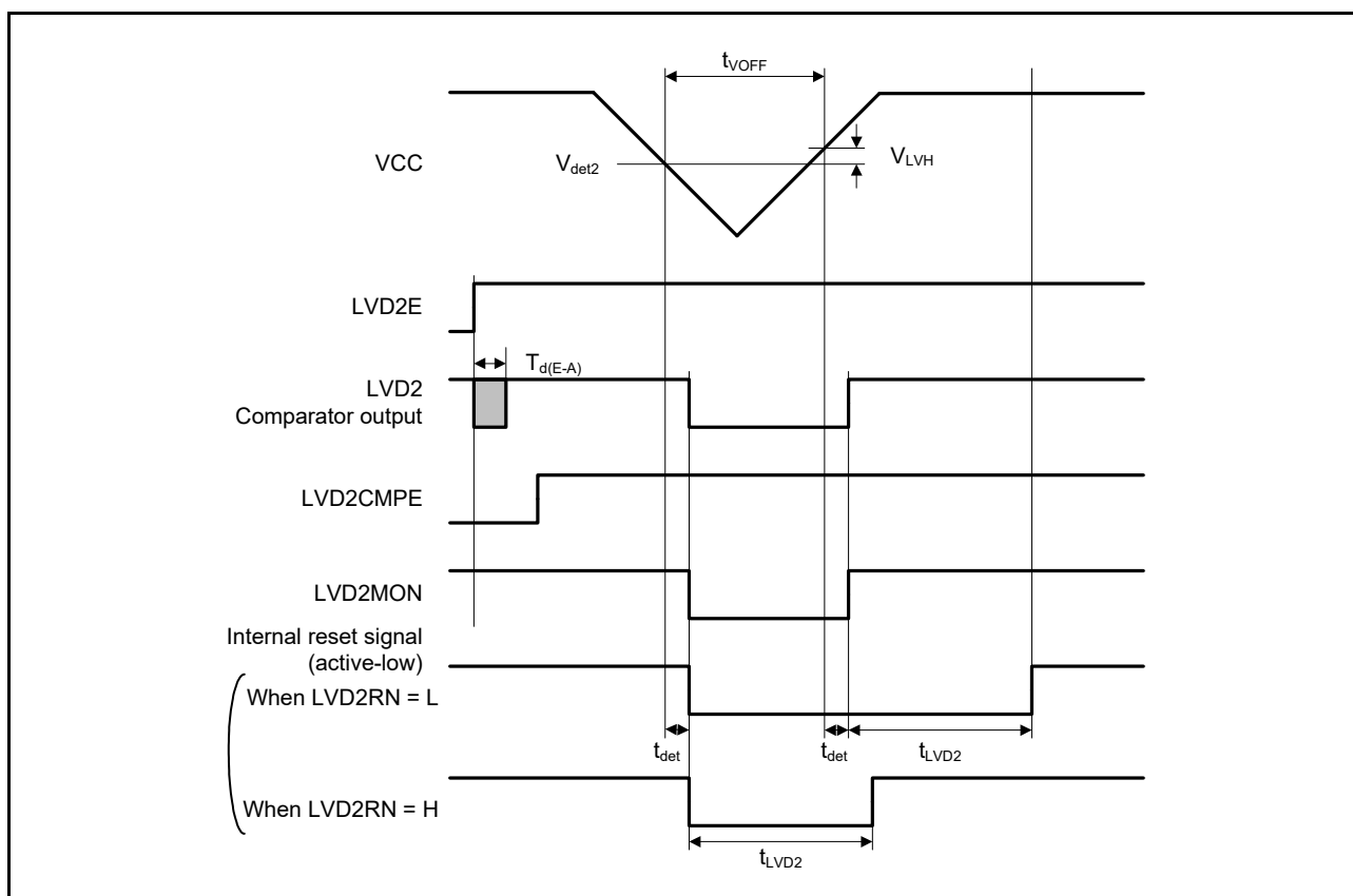
Figure 37.59 Voltage Detection Circuit Timing ( V_{det2} )
