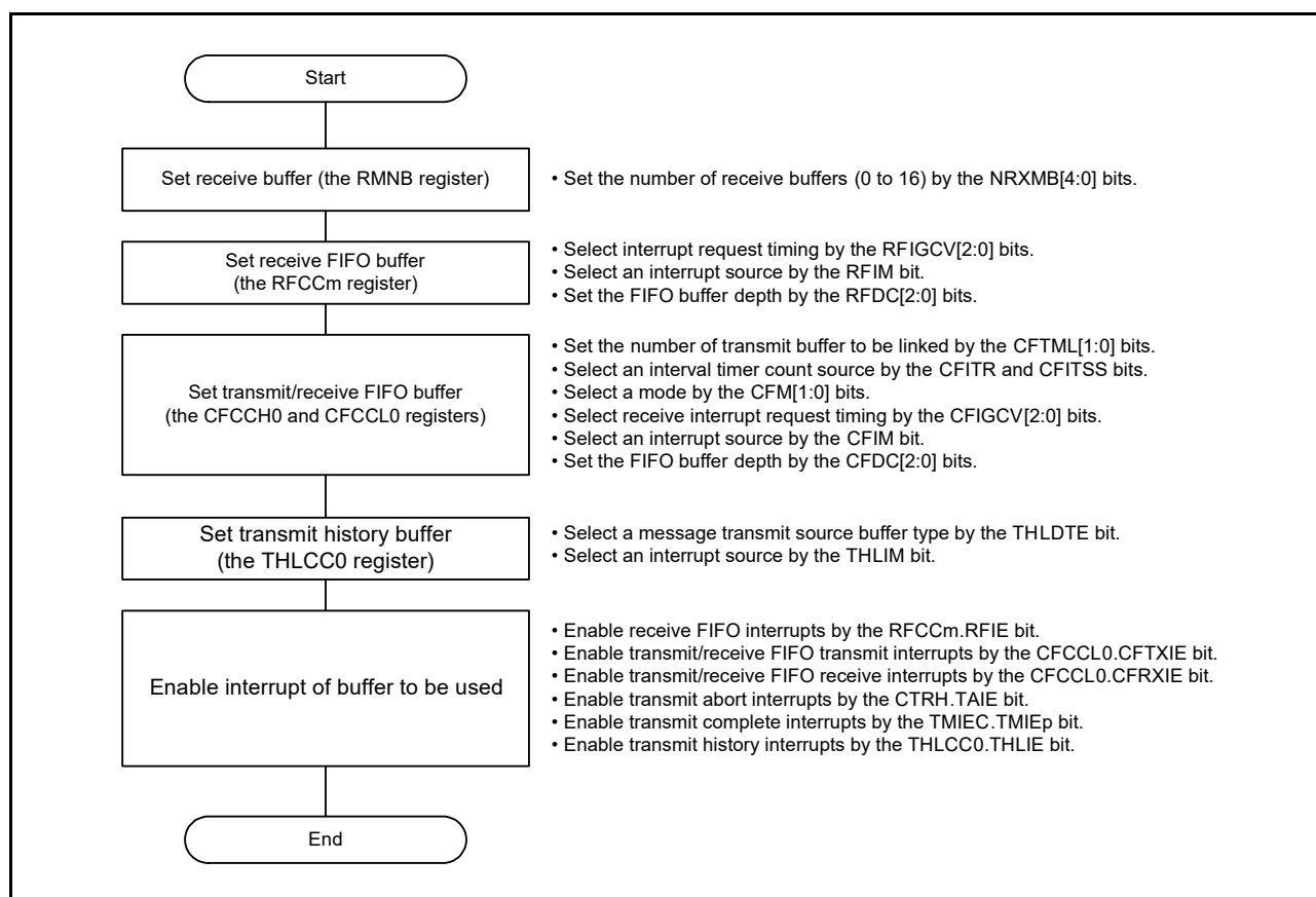
Figure 28.21 Buffer Setting Procedure
