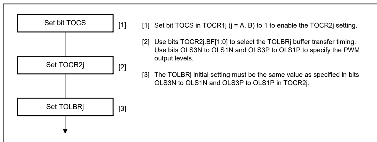
Figure 20.4 Example of PWM Output Level Setting Procedure in Buffer Operation
