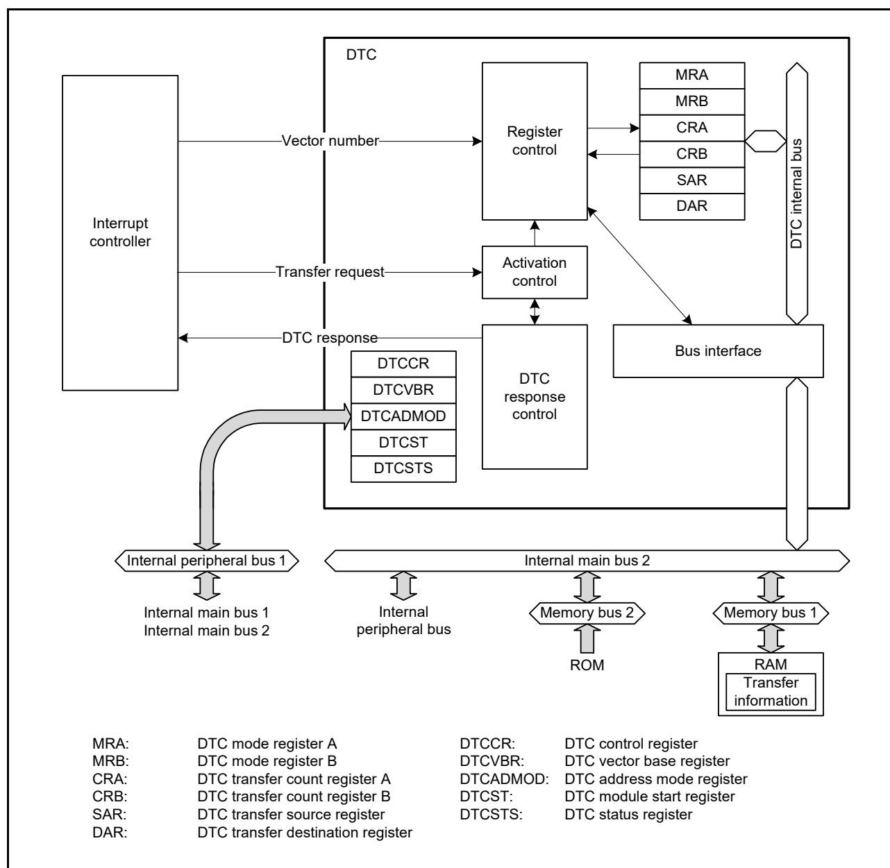
Figure 17.1 DTC Block Diagram
