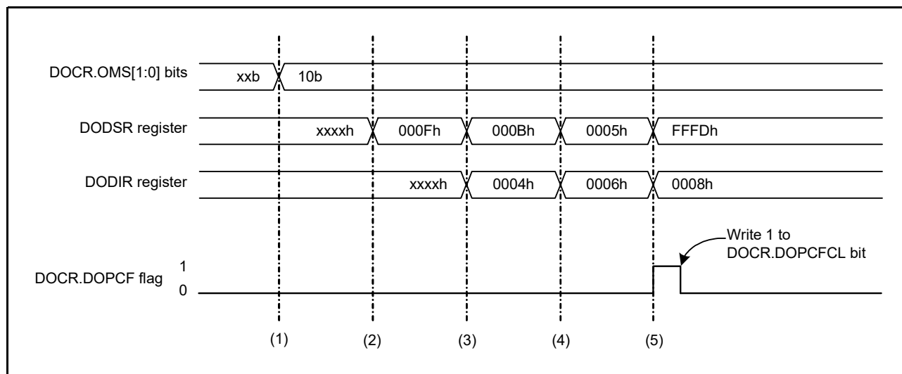
Figure 34.4 Example of Operation in Data Subtraction Mode
