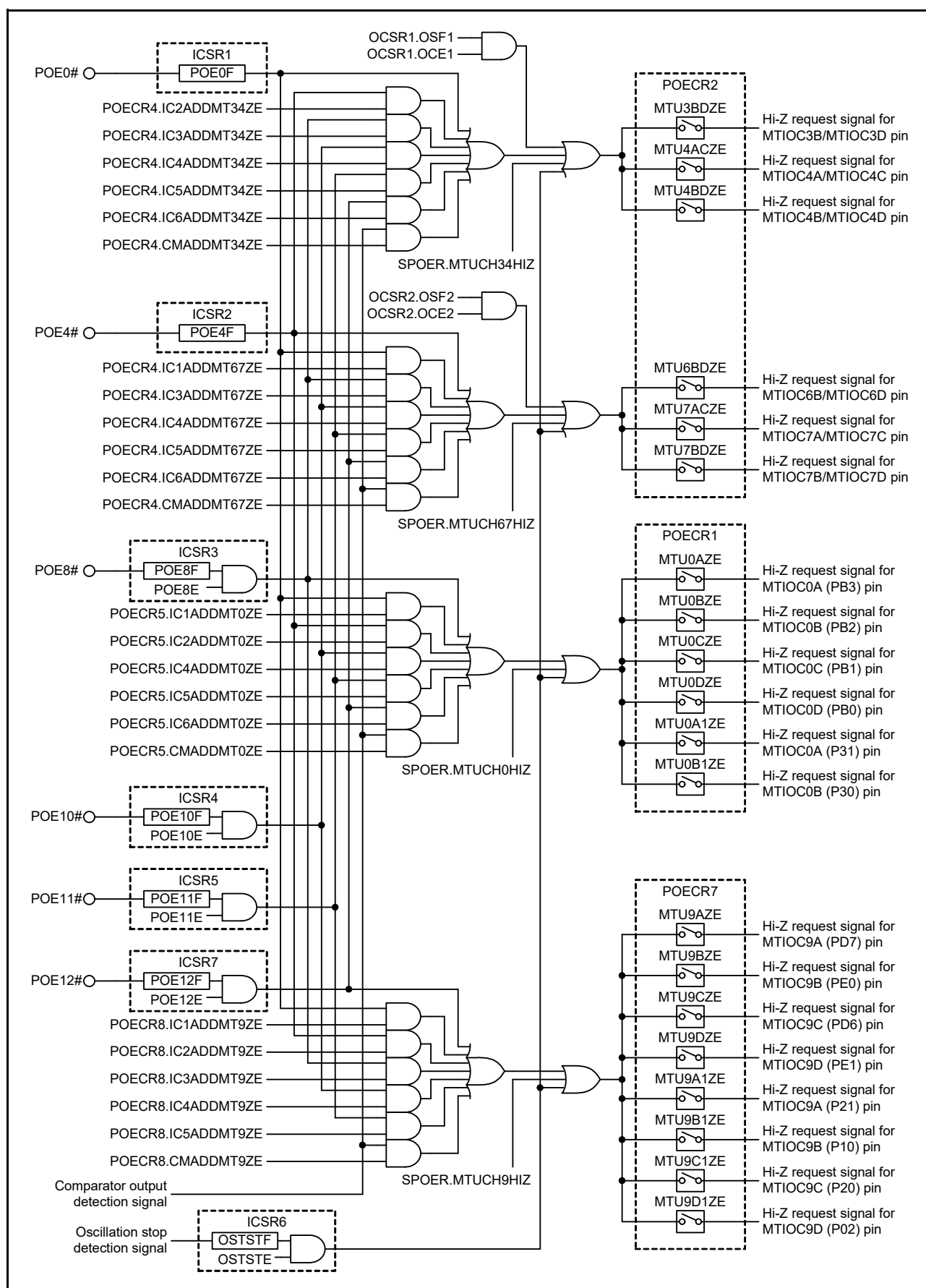
Figure 21.3 Target Pins and Conditions for High-Impedance Control (Chip Version A)
