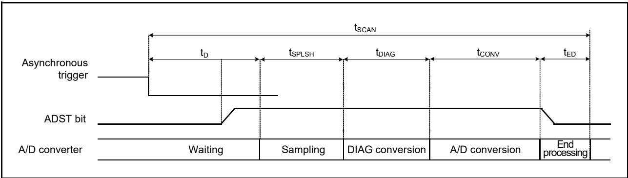
Figure 31.30 Scan Conversion Timing (Activated by Asynchronous Trigger)
