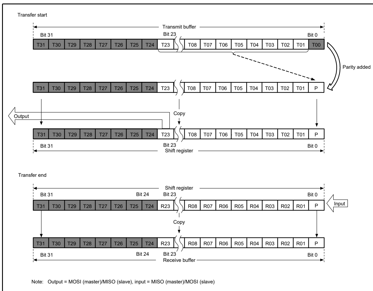
Figure 29.19 MSB First Transfer (24-Bit Data, Parity Enabled)
