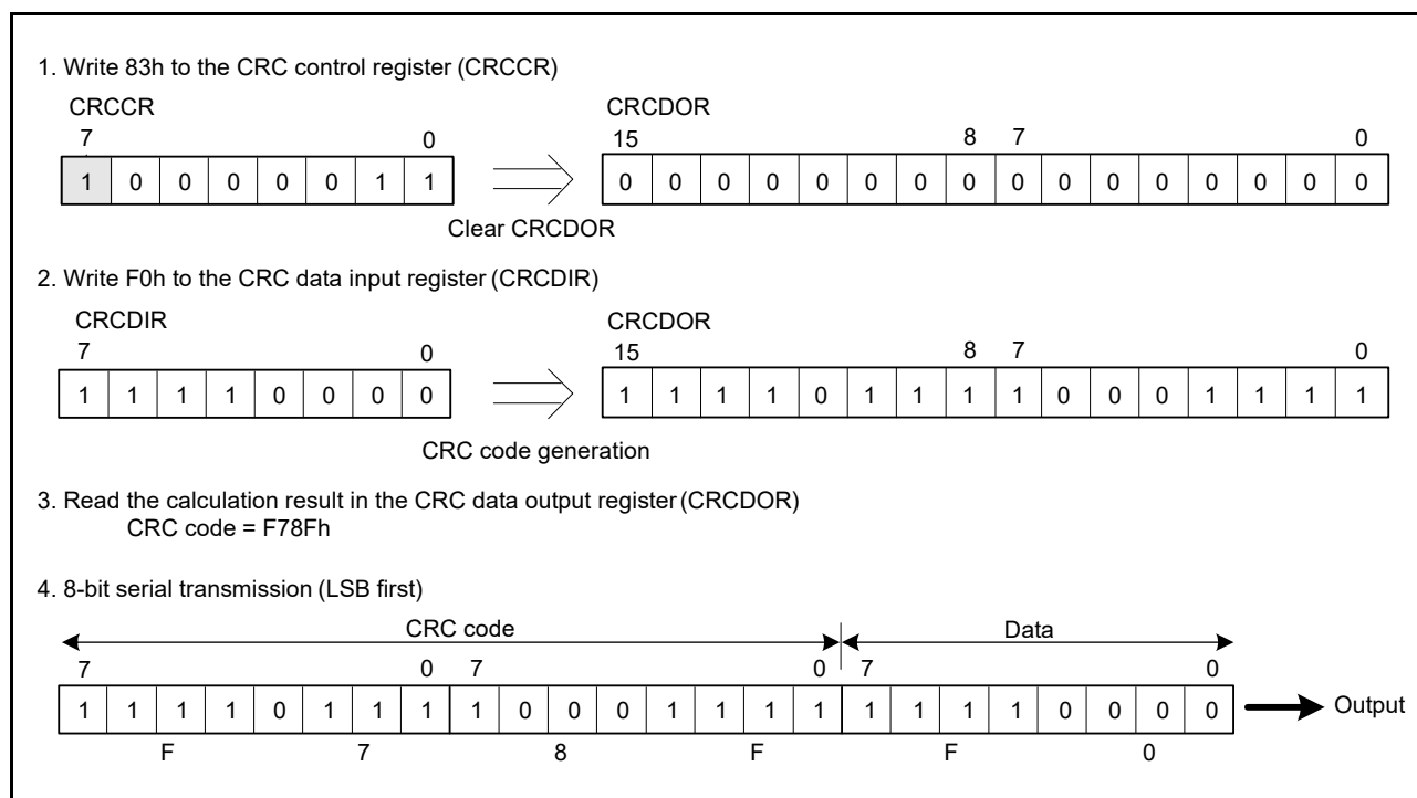
Figure 30.2 LSB First Data Transmission
