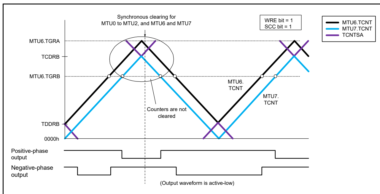
Figure 20.74 Example of Synchronous Clearing in Tb1 interval (Timing (6) in Figure 20.65; TWCRB.WRE Bit is 1 and SCC Bit is 1 in MTU6 and MTU7)
