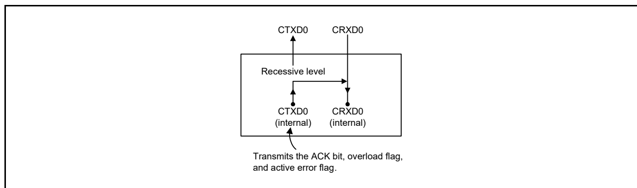
Figure 28.10 Connection When Listen-Only Mode is Selected
