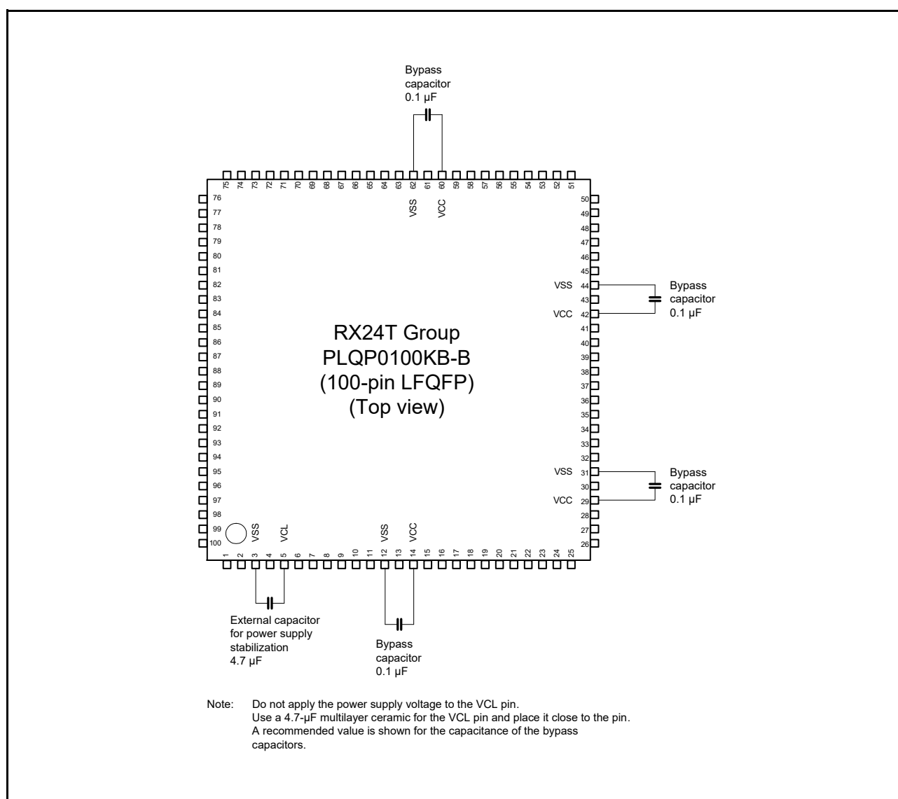
Figure 37.61 Connecting Capacitors (100 Pins)
