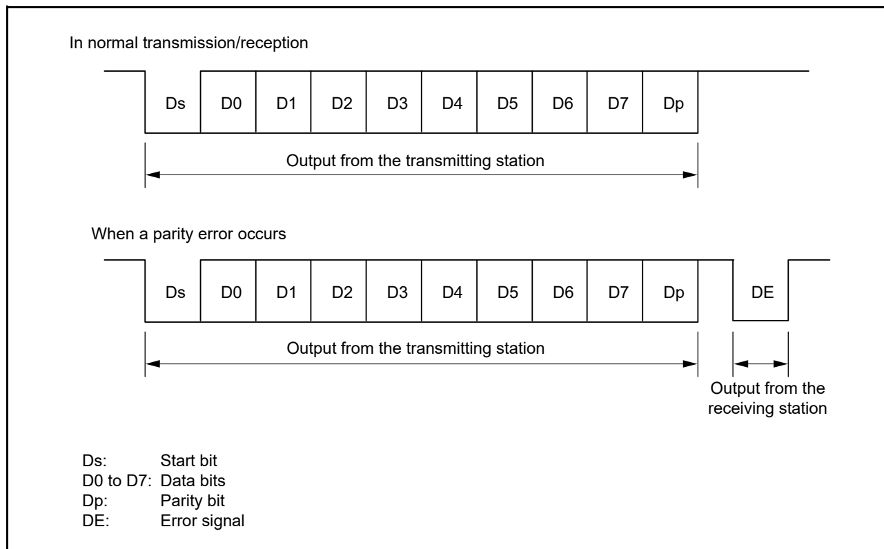
Figure 26.32 Data Formats in Smart Card Interface Mode
