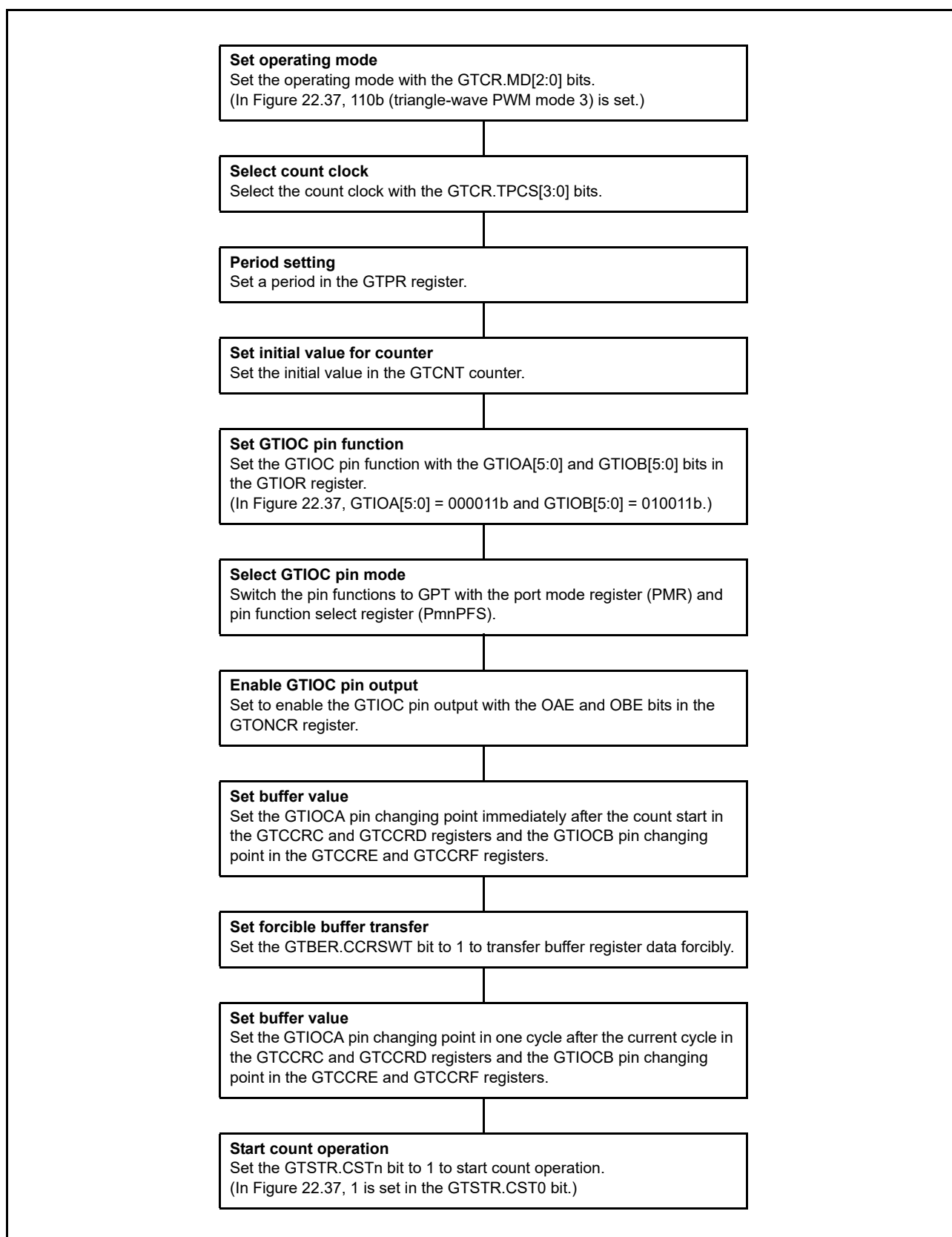
Figure 22.38 Example for Setting Triangle-Wave PWM Mode 3
