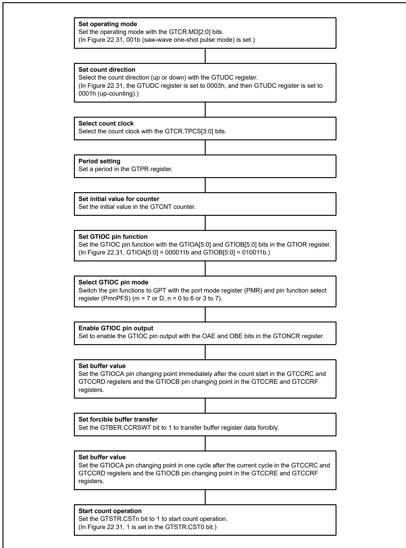
Figure 22.32 Example for Setting Saw-Wave One-Shot Pulse Mode
