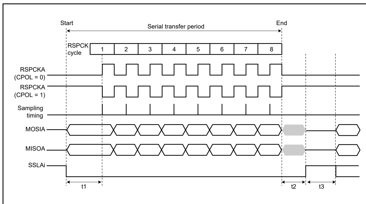
Figure 29.22 RSPI Transfer Format (CPHA = 0)
