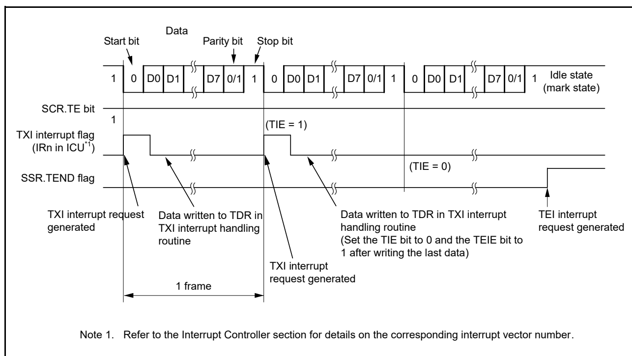
Figure 26.10 Example of Operation for Serial Transmission in Asynchronous Mode (3) (with 8-Bit Data, Parity, 1 Stop Bit, CTS Function Not Used, from the Middle of Transmission until Transmission Completion)
