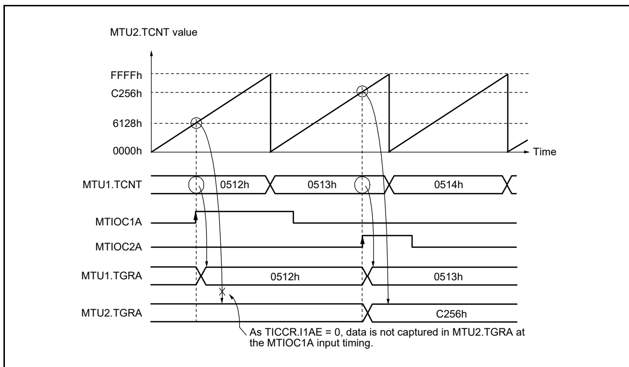
Figure 20.23 Cascaded Operation Example (b)
