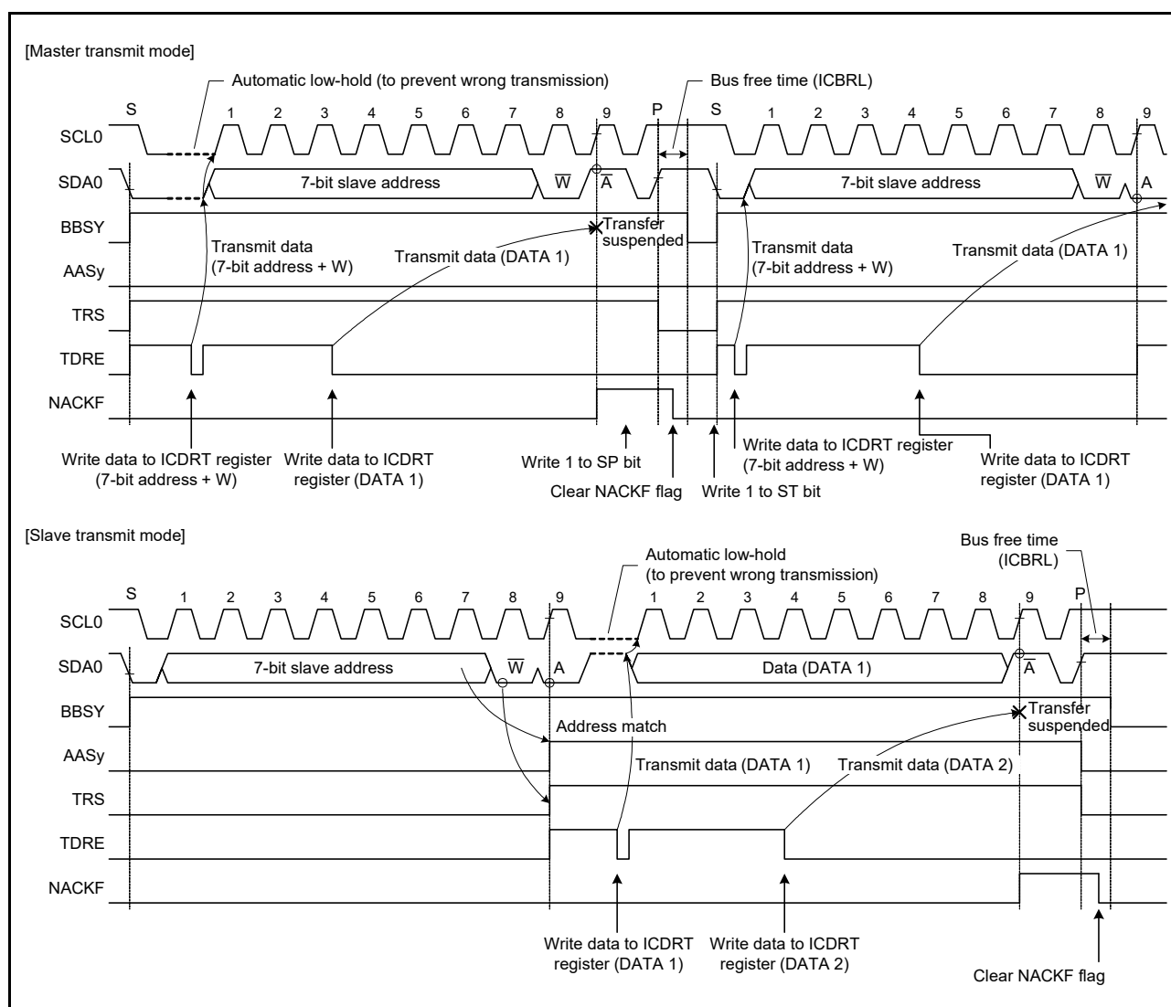
Figure 27.31 Suspension of Data Transfer When NACK is Received (NACKEN = 1)
