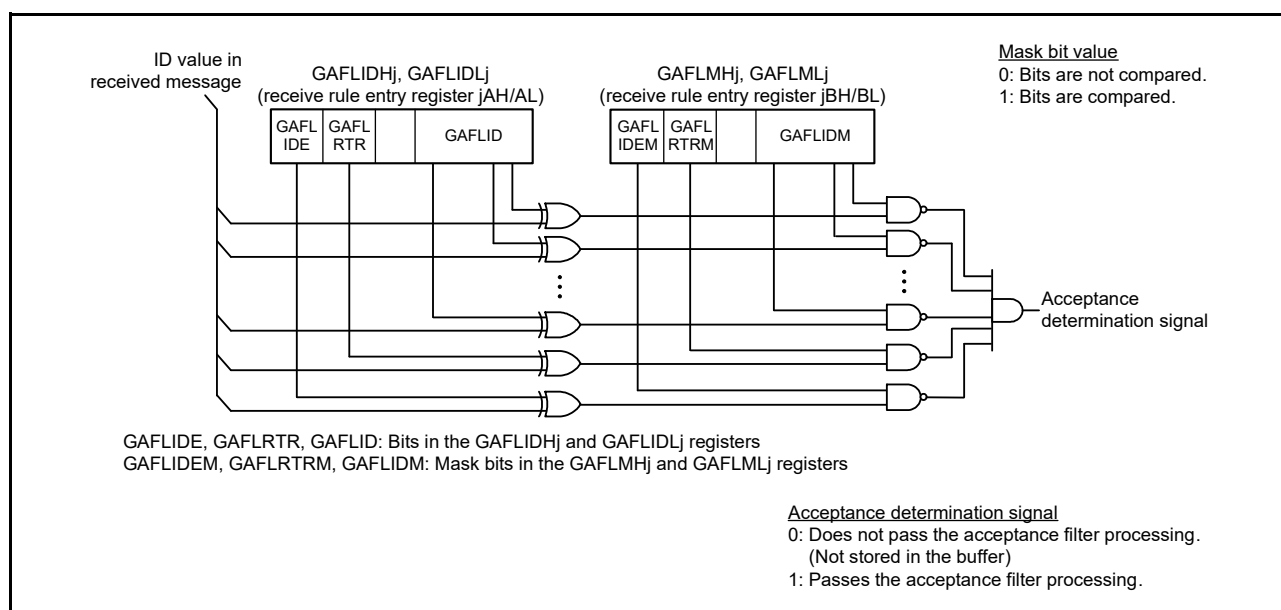
Figure 28.5 Acceptance Filter Function
