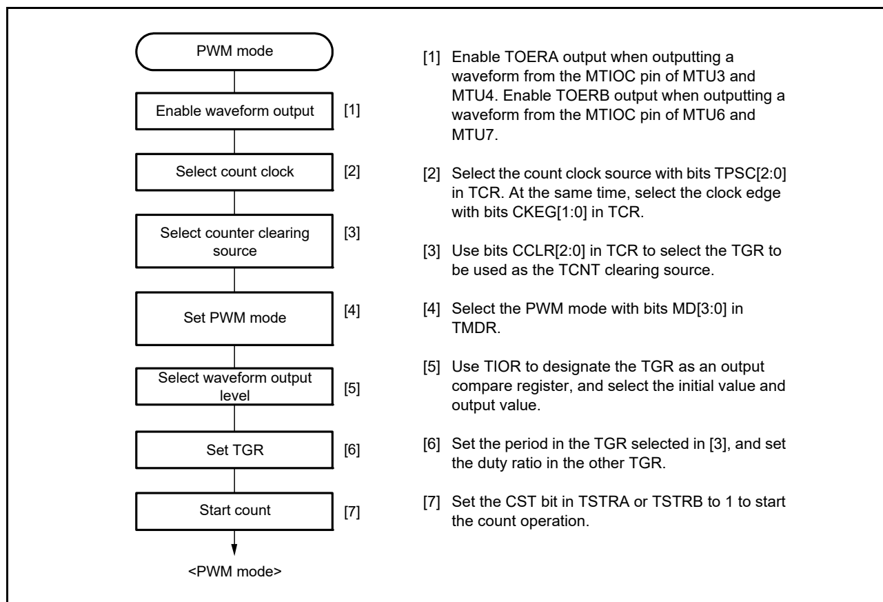
Figure 20.26 Example of PWM Mode Setting Procedure
