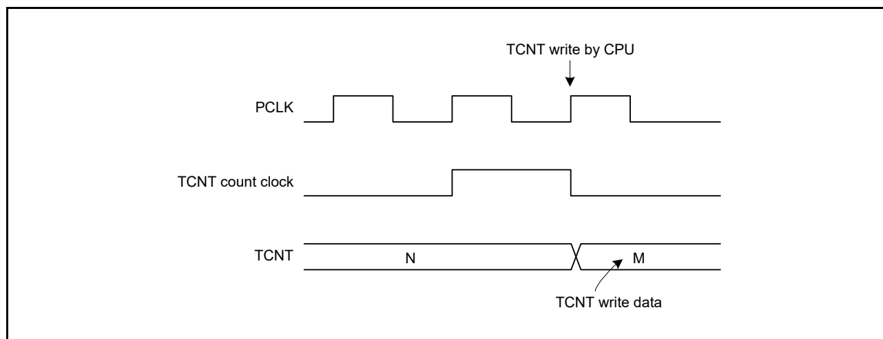
Figure 23.16 Conflict between TCNT Write and Increment
