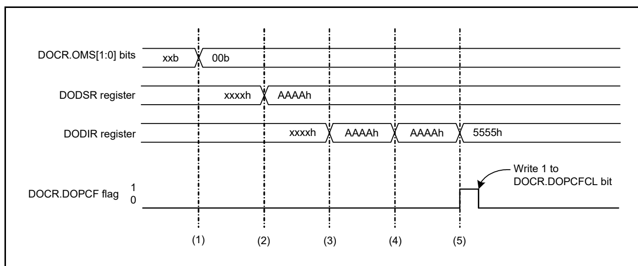
Figure 34.2 Example of Operation in Data Comparison Mode
