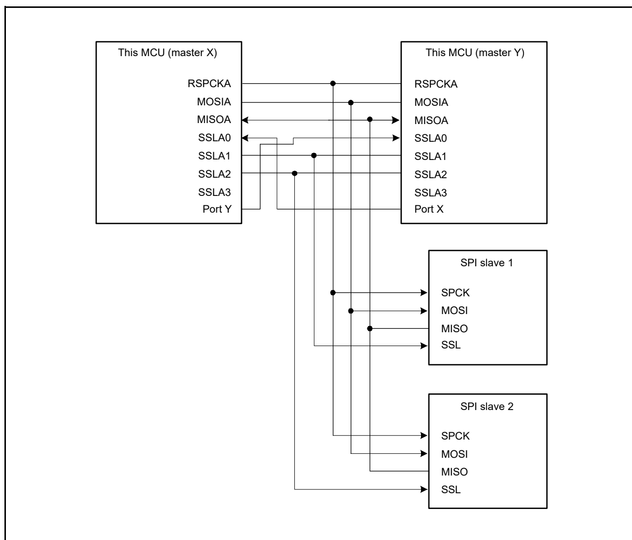
Figure 29.10 Multi-Master/Multi-Slave Configuration Example (This MCU = Master)
