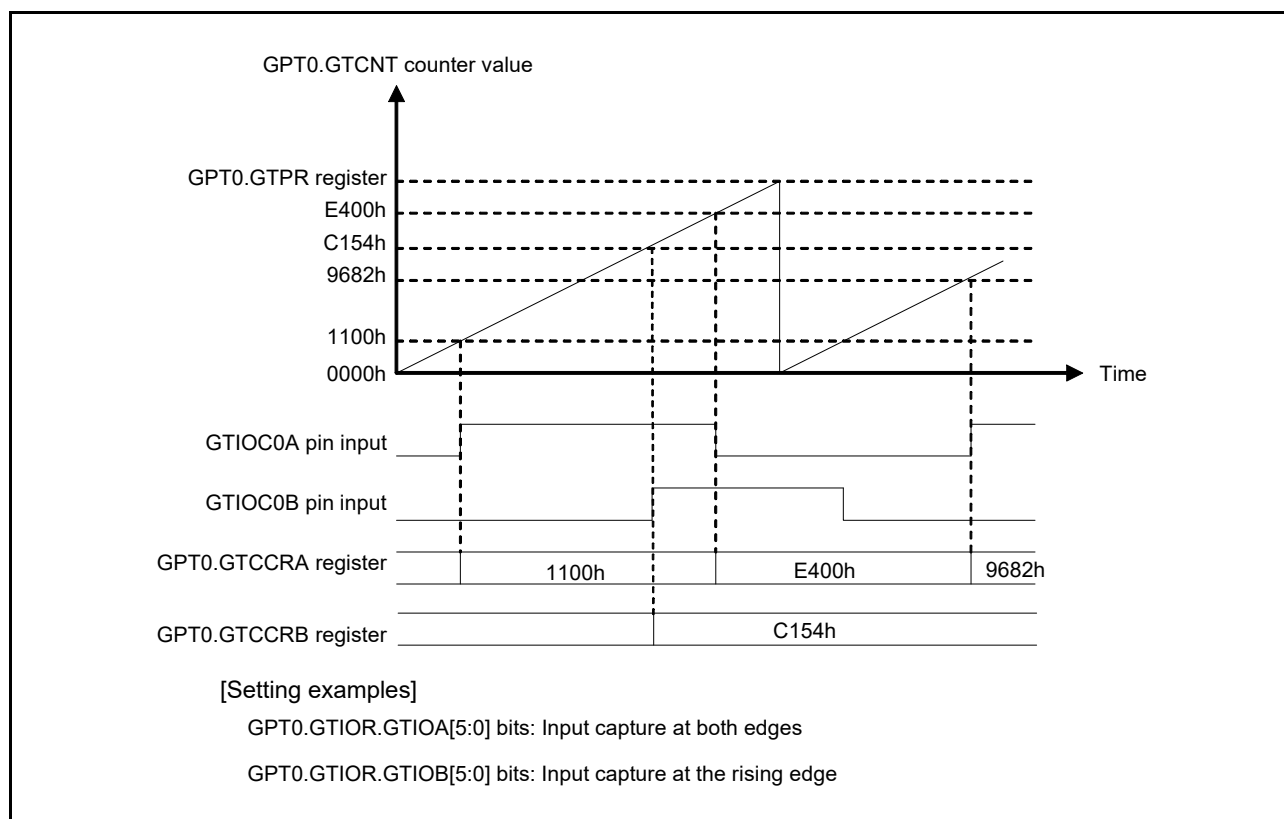
Figure 22.12 Example of Input Capture Operation
