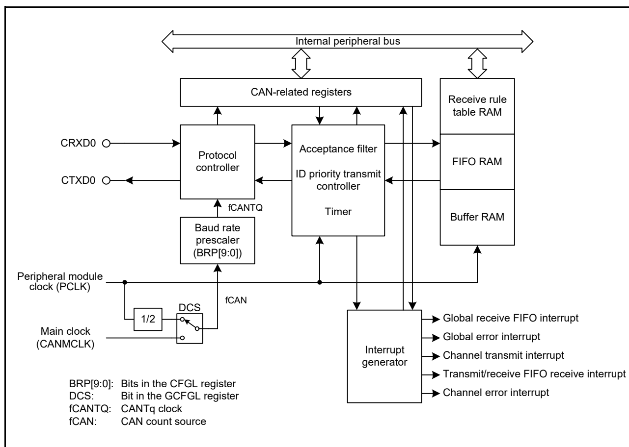
Figure 28.1 CAN Module Block Diagram
