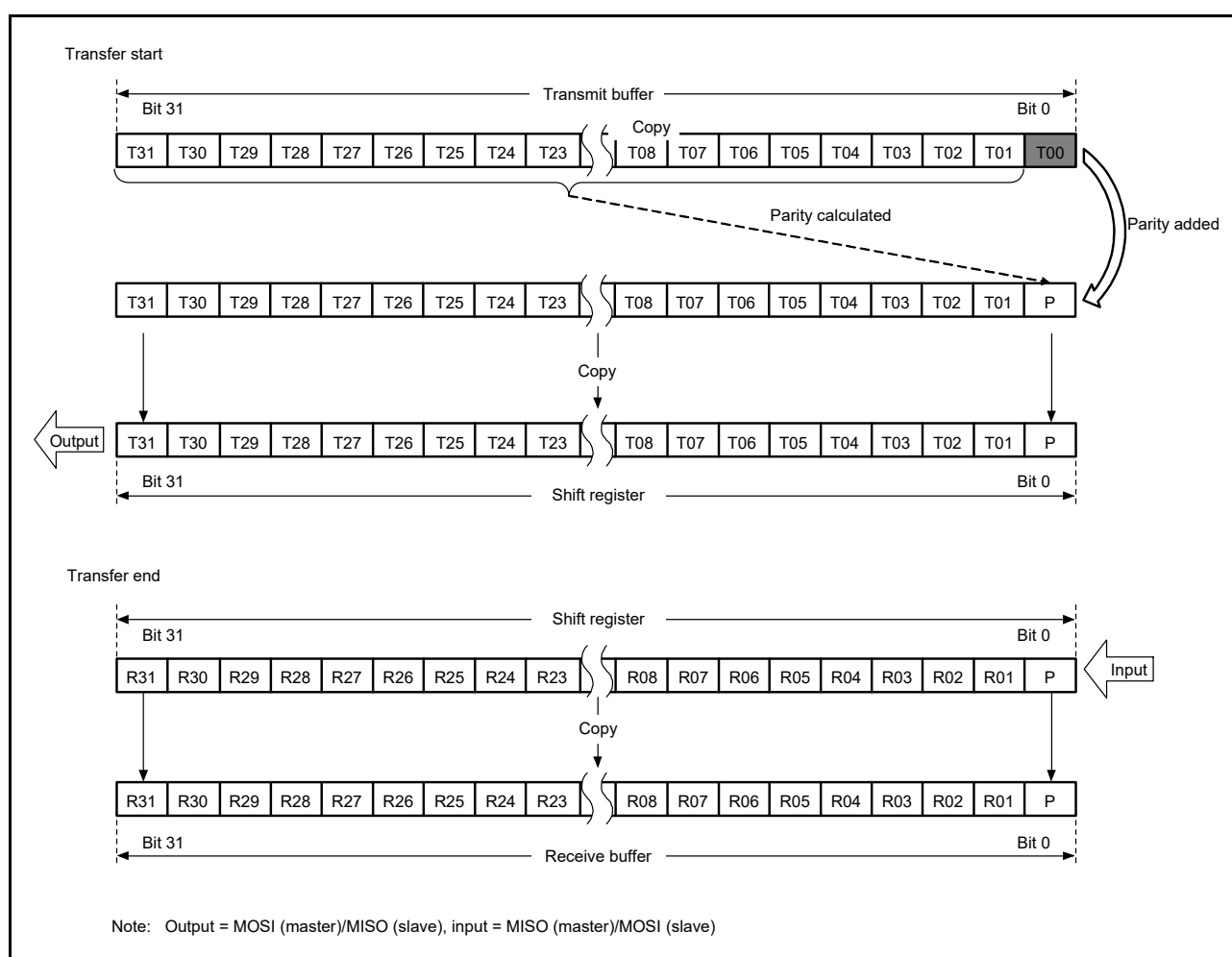
Figure 29.18 MSB First Transfer (32-Bit Data, Parity Enabled)
