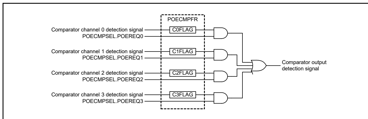
Figure 21.8 Comparator Output Detection Signal Generator Block Diagram (Chip Version A)
