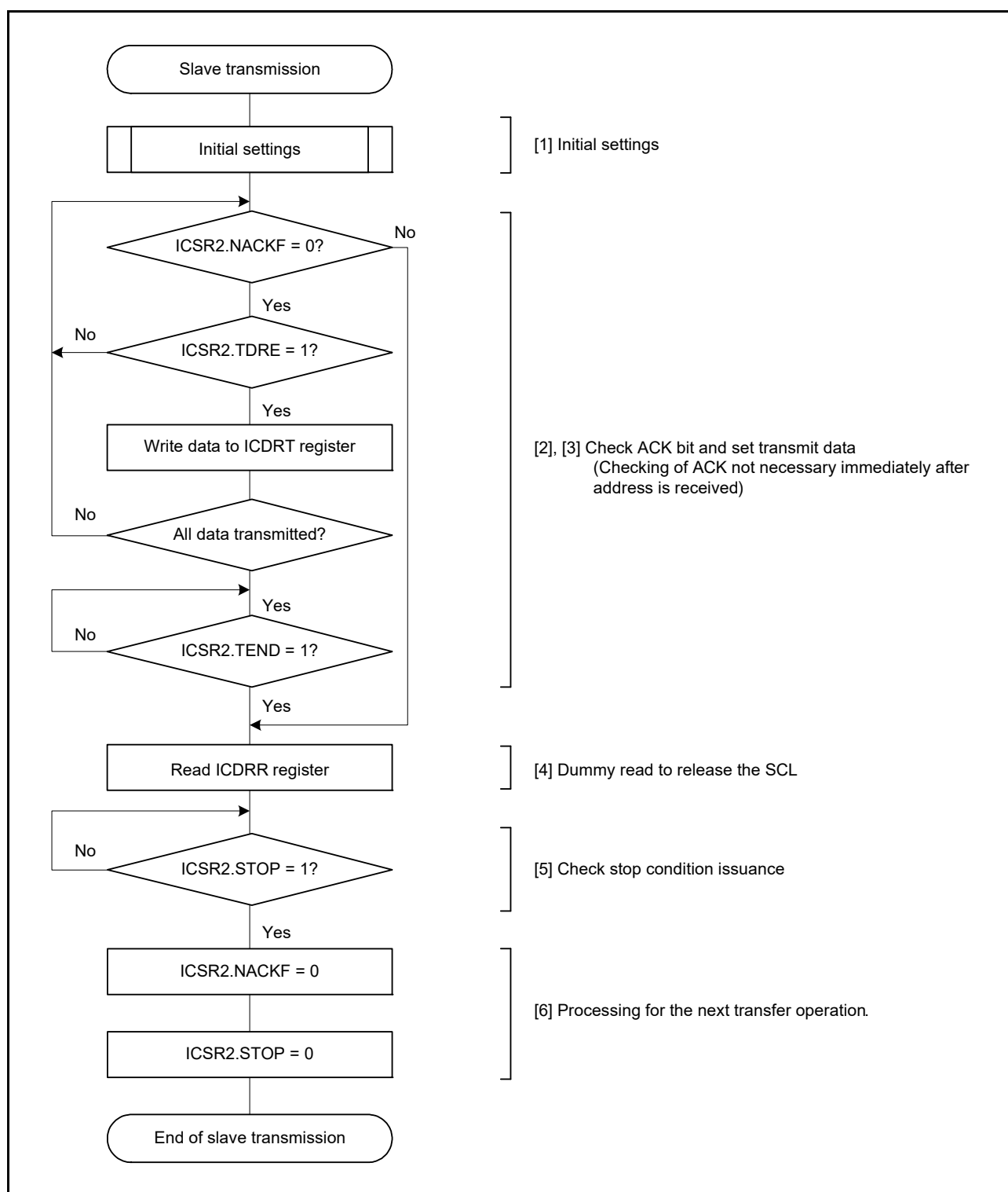
Figure 27.15 Example of Slave Transmission Flowchart
