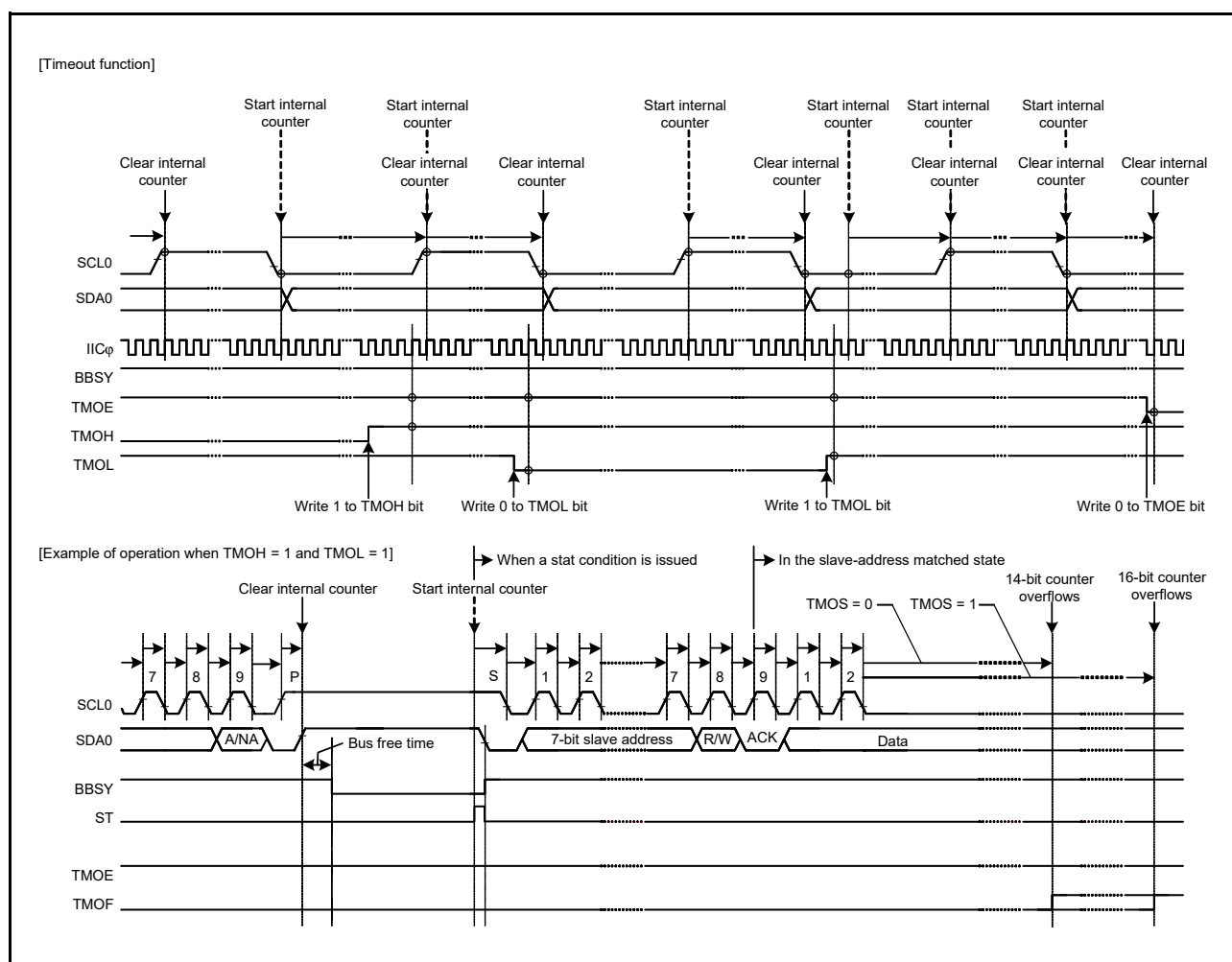
Figure 27.39 Timeout Function
