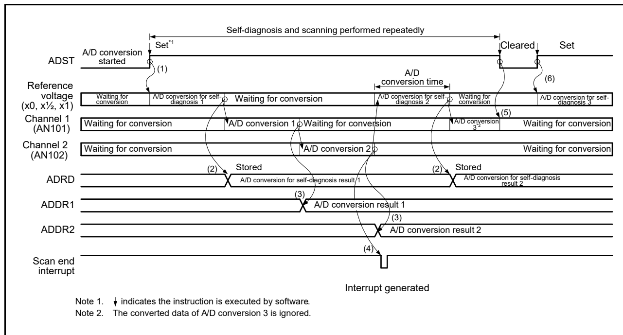
Figure 31.14 Example of Operation in Continuous Scan Mode (Basic Operation; AN101 and AN102 Selected + Self-Diagnosis)
