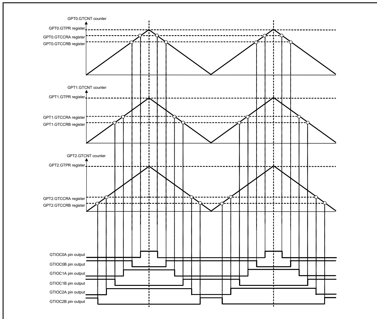
Figure 22.69 Example of Three-Phase Triangle-Wave Complementary PWM Output
