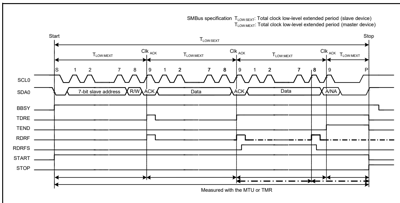
Figure 27.41 SMBus Timeout Measurement
