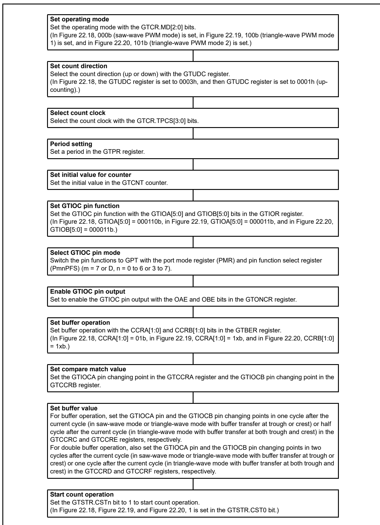
Figure 22.21 Example for Setting GTCCRA and GTCCRB Buffer Operation (for Output Compare)
