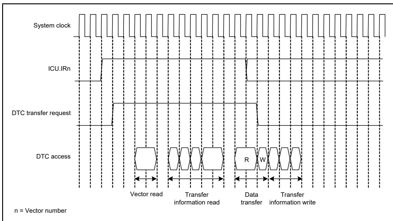
Figure 17.12 Example (4) of DTC Operation Timing (Full-Address Mode, Normal Transfer Mode, Repeat Transfer Mode)
