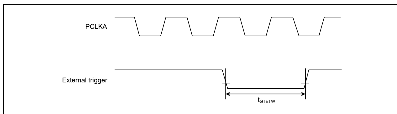
Figure 37.41 Timing of the GPT External Trigger Input
