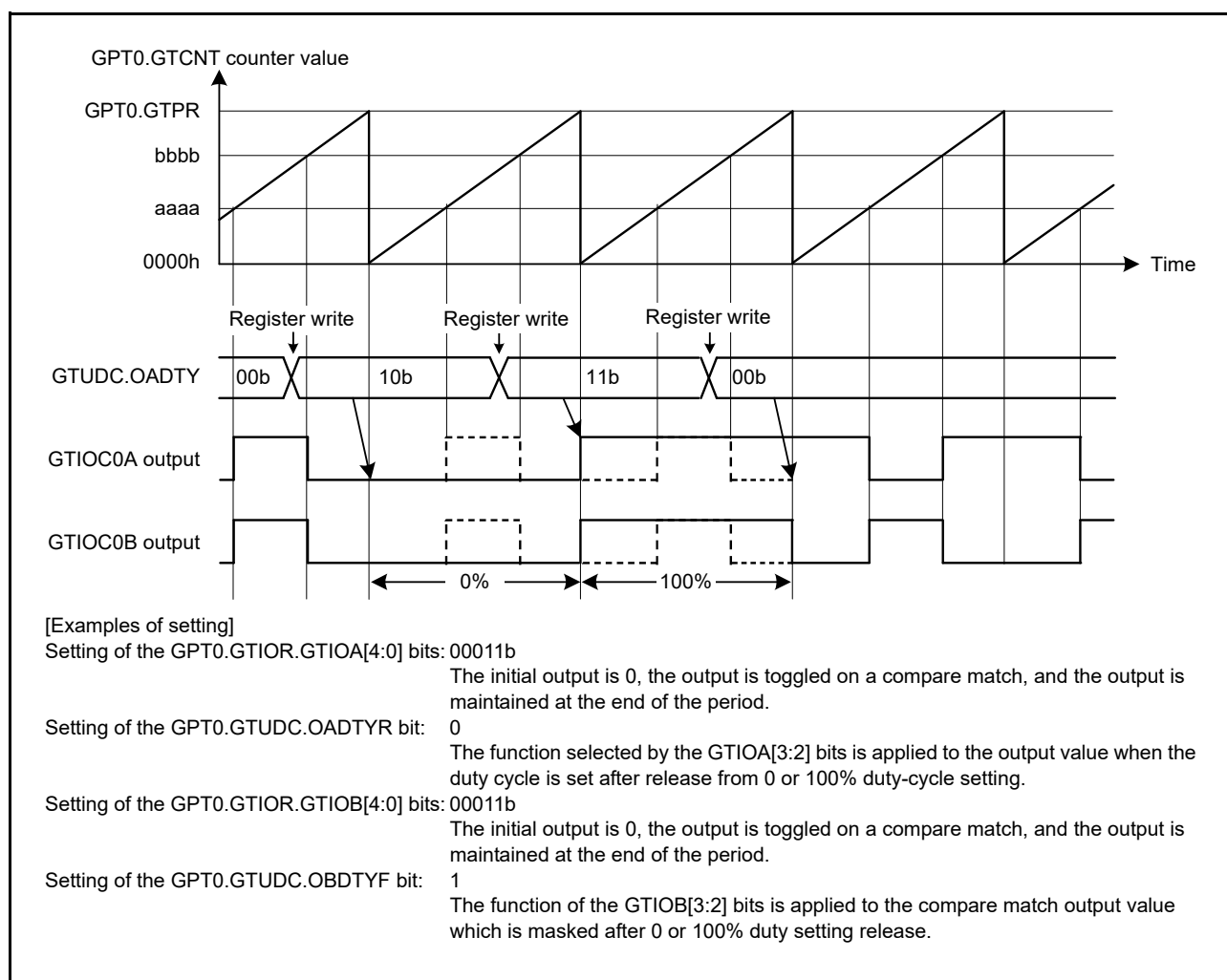
Figure 22.46 Example of Operation of Output of Duty Cycle 0% or 100%
