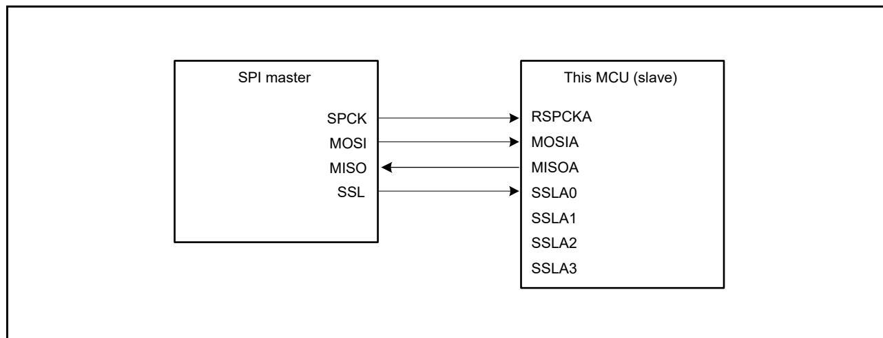
Figure 29.6 Single-Master/Single-Slave Configuration Example (This MCU = Slave, CPHA = 0)
