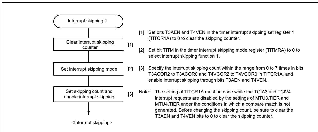
Figure 20.85 Example of Interrupt Skipping Function 1 Setting Procedure
