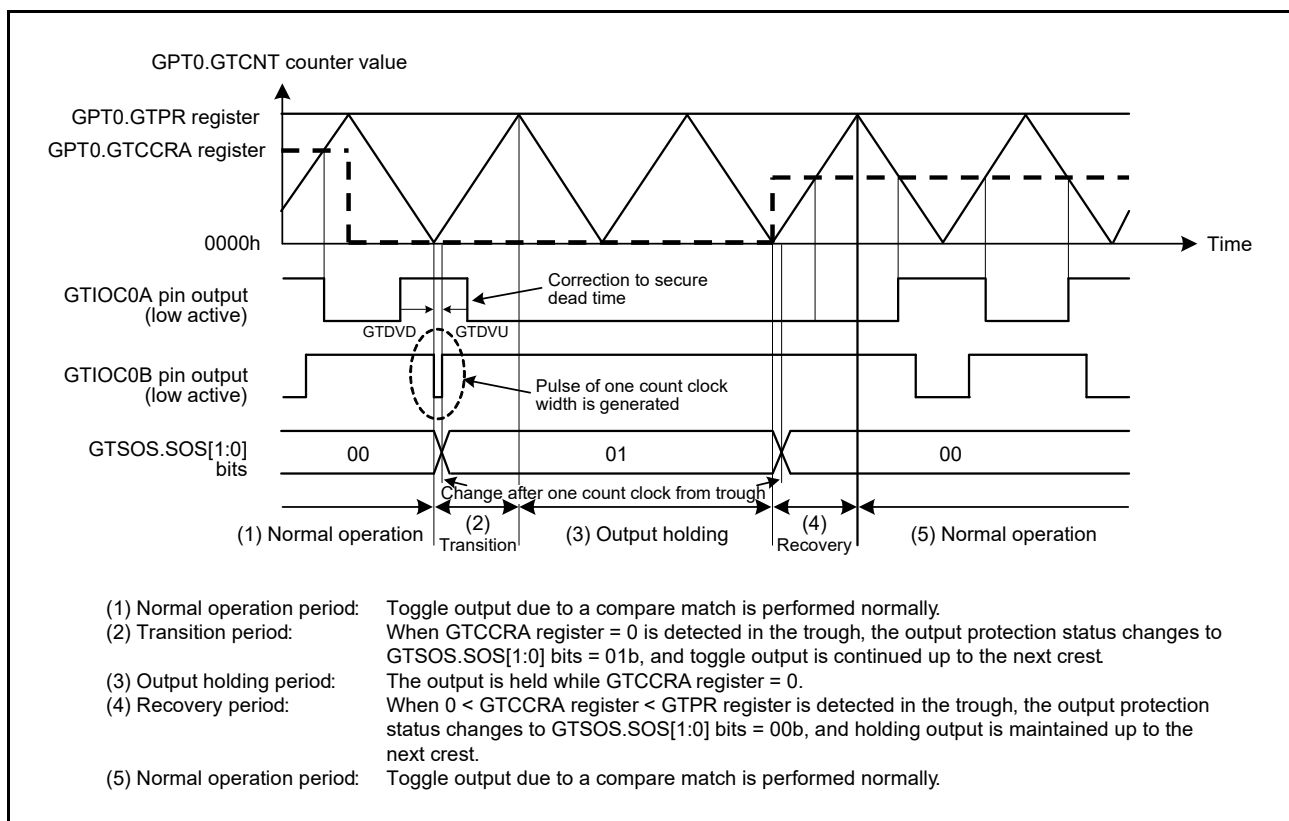
Figure 22.86 Example of Output Protection Function Operation When the GTCCRA Register is Set to 0000h during Buffer Transfer at Crests (Restored to 0 < \text{GTCCRA} < \text{GTPR} during Buffer Transfer at Troughs, Active Level: Low)
