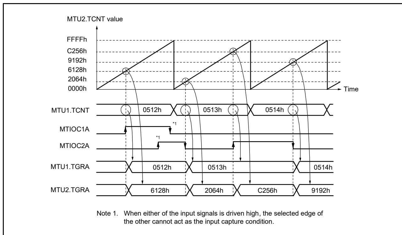
Figure 20.24 Cascaded Operation Example (c)
