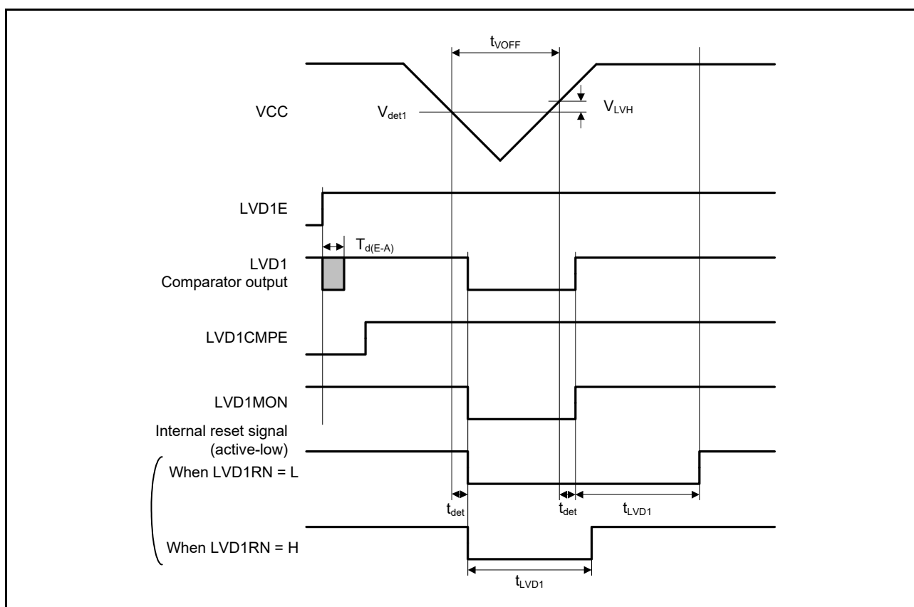
Figure 37.58 Voltage Detection Circuit Timing ( V_{det1} )
