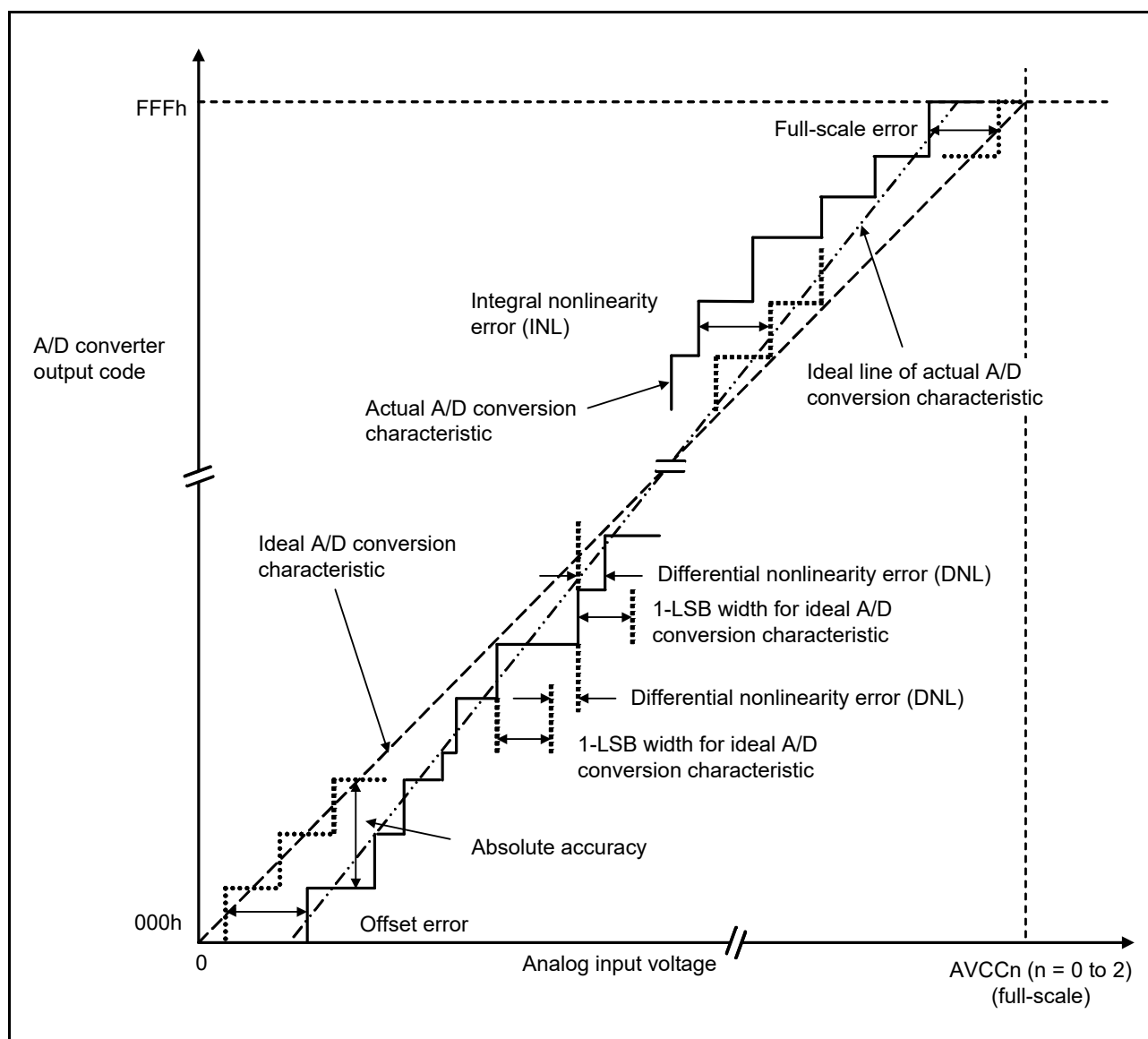
Figure 37.53 Illustration of A/D Converter Characteristic Terms
