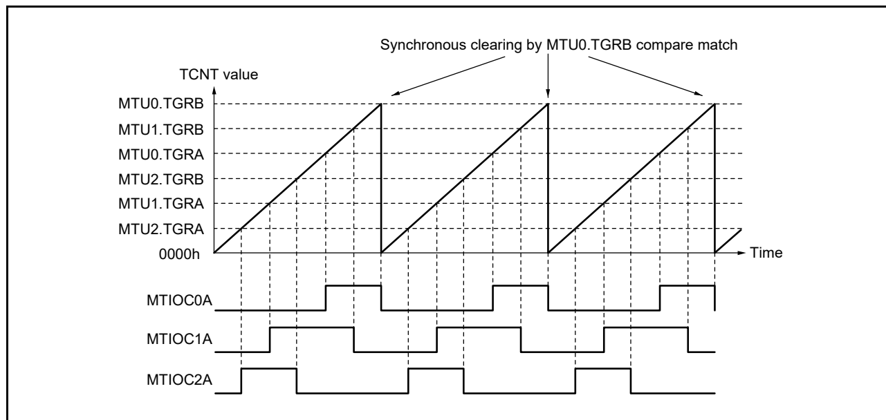
Figure 20.14 Example of Synchronous Operation
