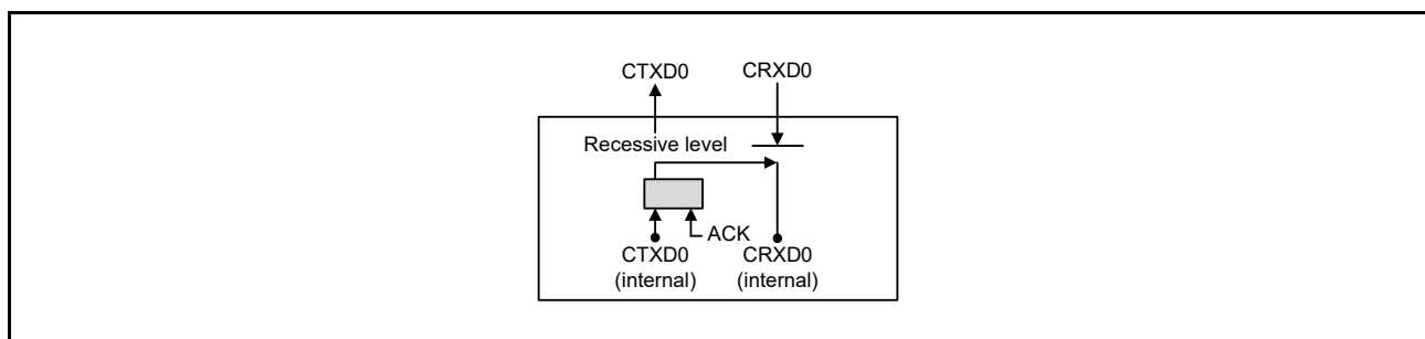
Figure 28.12 Connection When Self-Test Mode 1 is Selected
