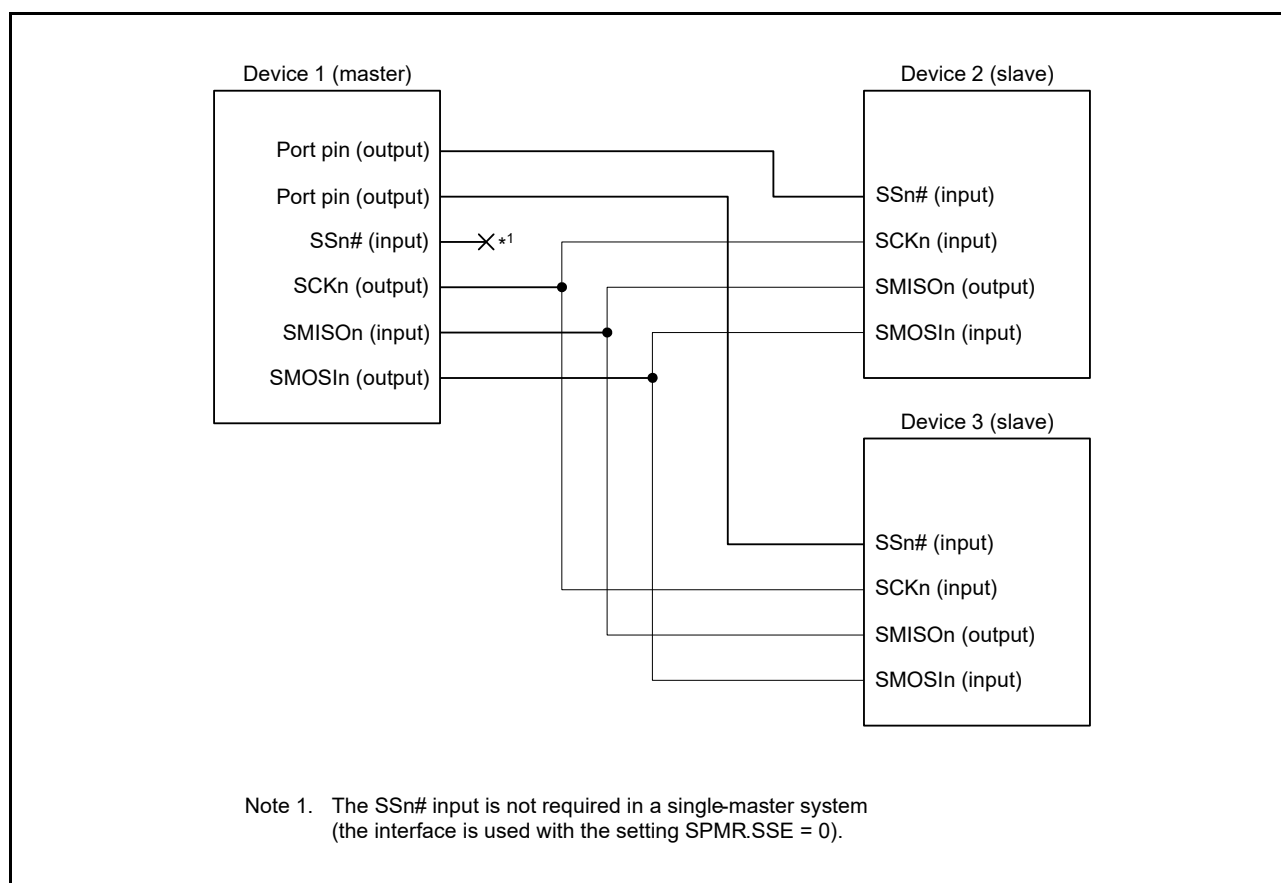
Figure 26.54 Example of Connections via a Simple SPI Mode (In Single Master Mode, SPMR.SSE Bit = 0)
