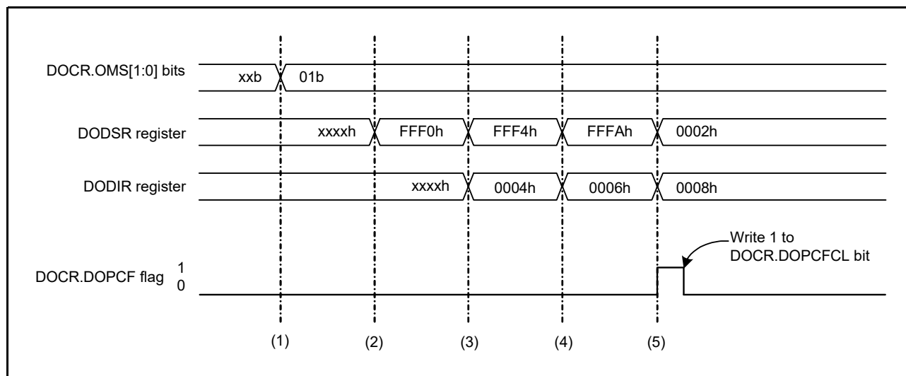
Figure 34.3 Example of Operation in Data Addition Mode
