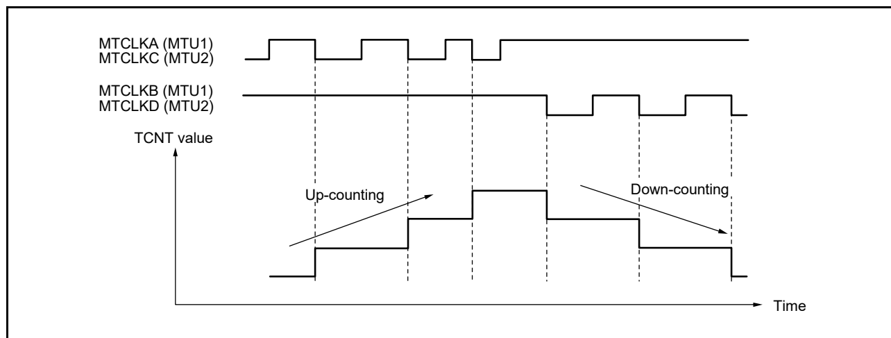
Figure 20.35 Example of Operation in Phase Counting Mode 3 (When MTUn.TCR2.PCB[1:0] = 00b ( n = 1, 2 ))
