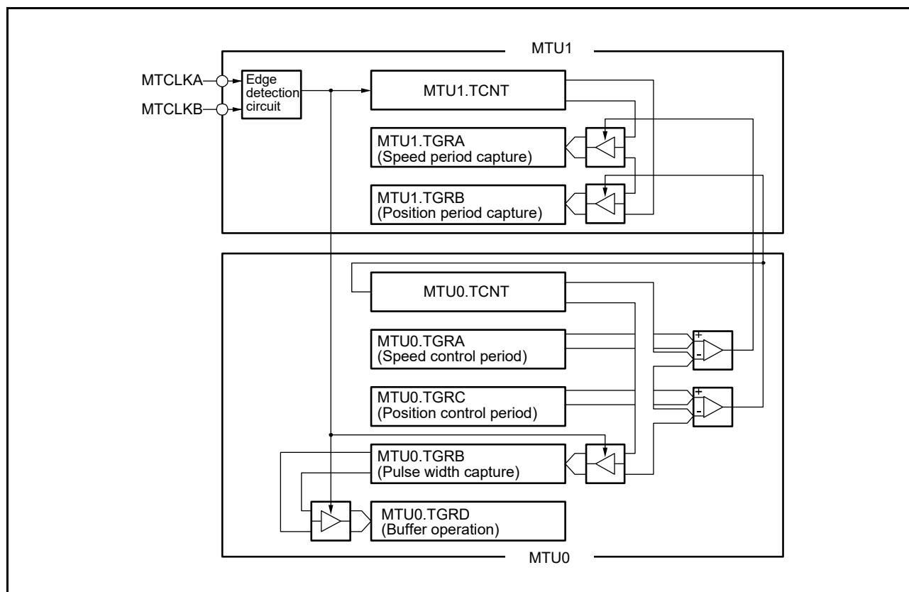
Figure 20.41 16-Bit Phase Counting Mode Application Example
