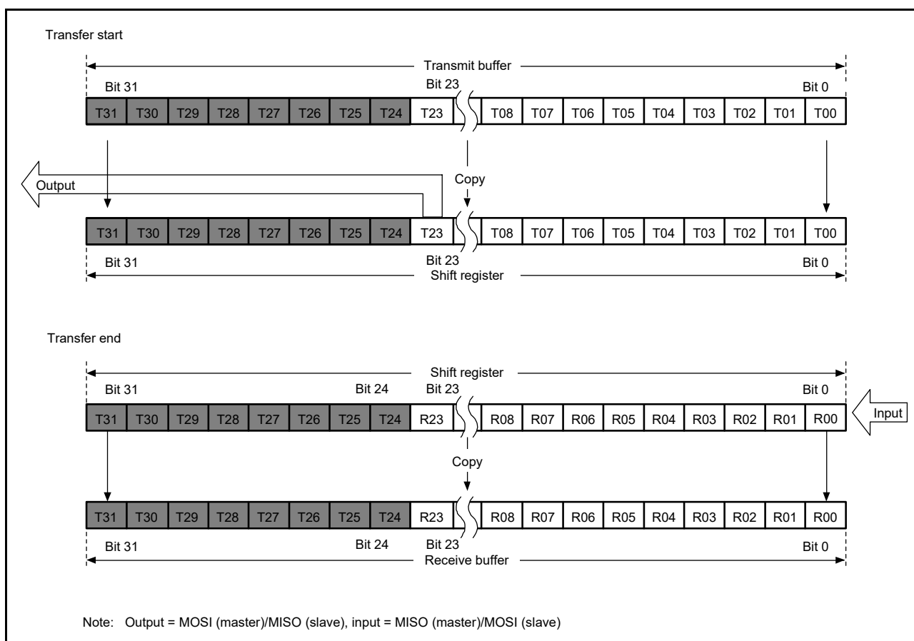
Figure 29.15 MSB First Transfer (24-Bit Data, Parity Disabled)
