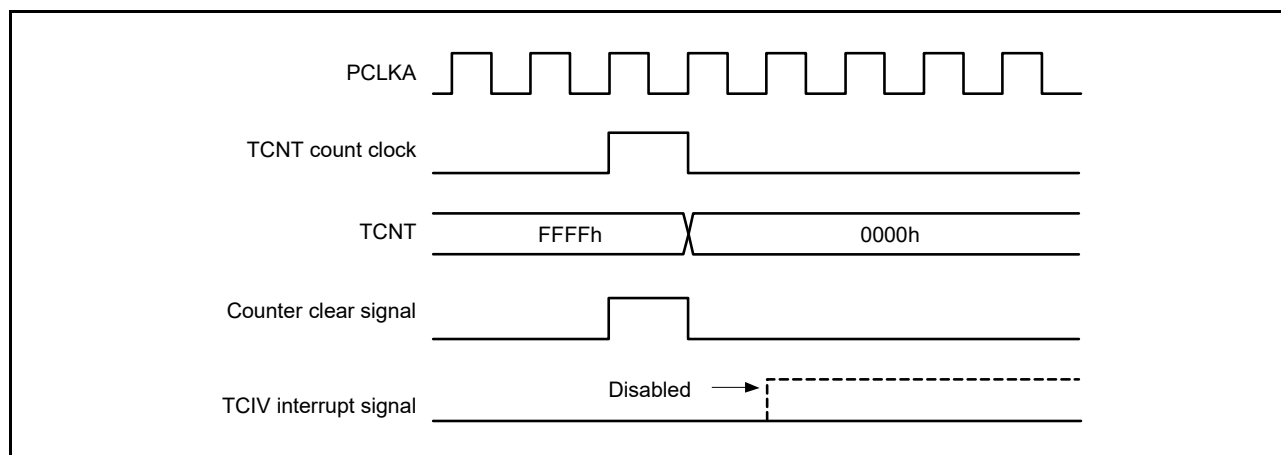
Figure 20.147 Contention between Overflow and Counter Clearing
