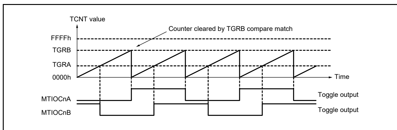
Figure 20.10 Example of Toggle Output Operation (n = 0 to 4, 6, 7, 9)
