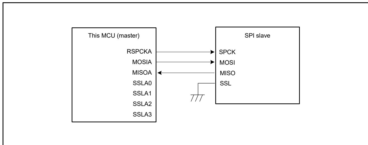
Figure 29.5 Single-Master/Single-Slave Configuration Example (This MCU = Master)
