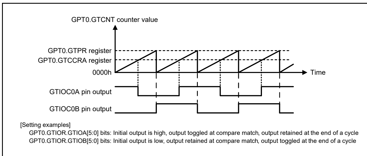
Figure 22.10 Example of Toggled Output Operation (2)
