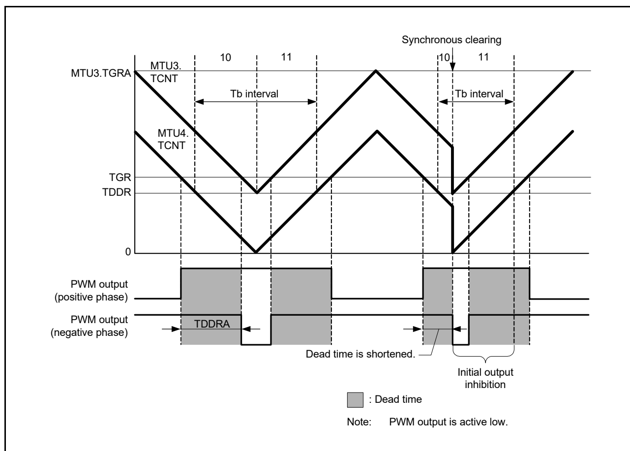
Figure 20.149 Example of Synchronous Clearing (When Condition 1 Applies)
