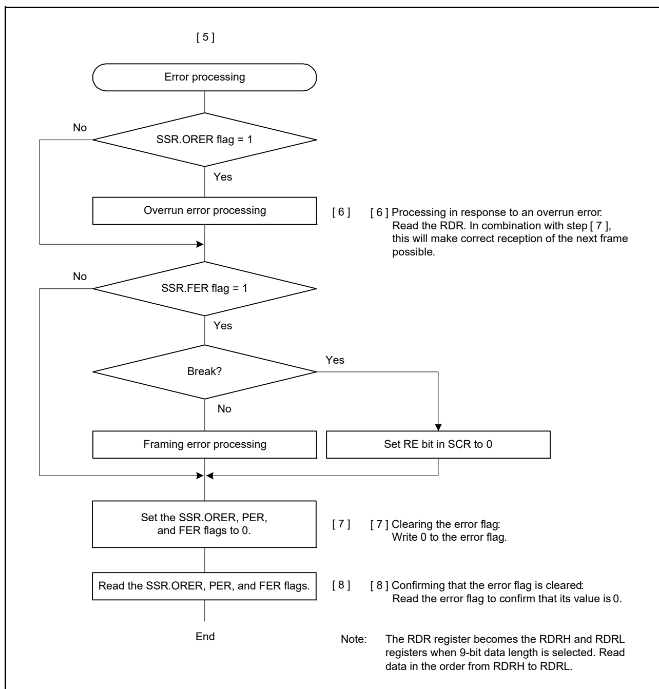
Figure 26.20 Example of Multi-Processor Serial Reception Flowchart (2)
