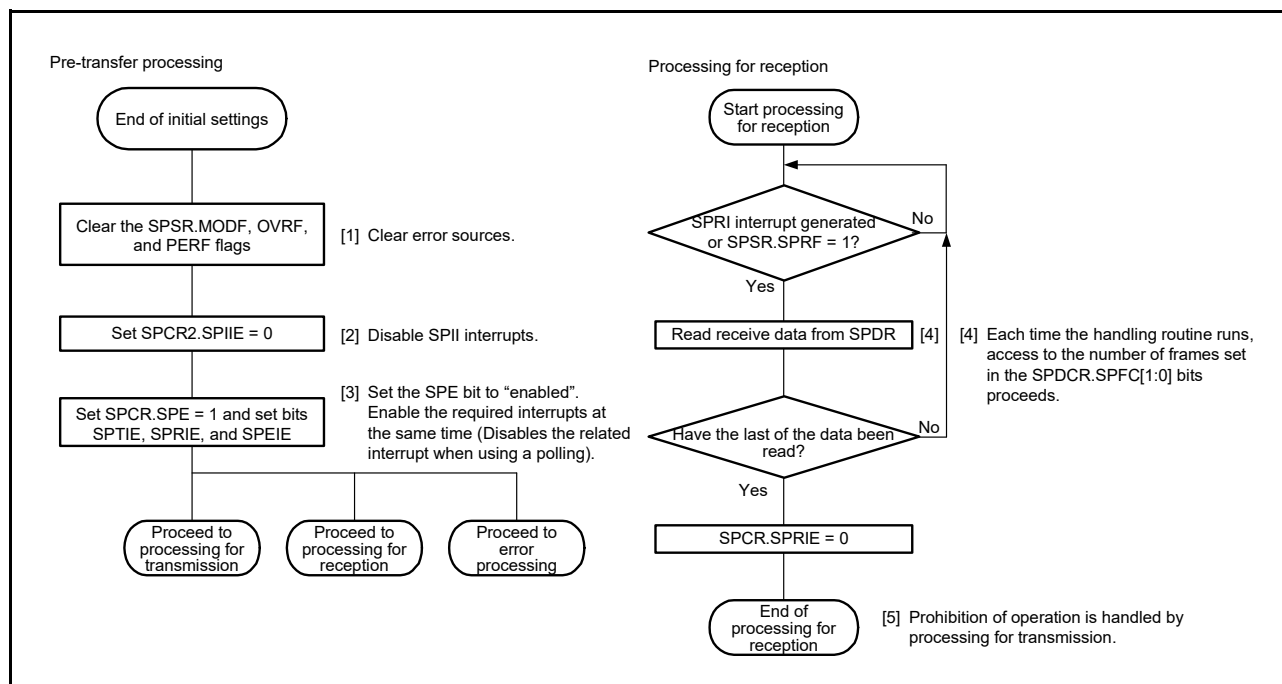
Figure 29.37 Flowchart in Master Mode (Reception)
