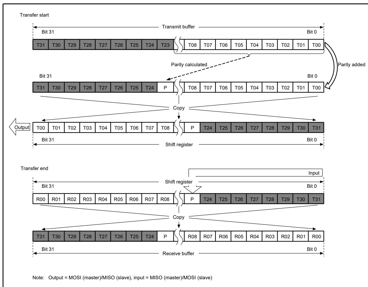
Figure 29.21 LSB First Transfer (24-Bit Data, Parity Enabled)
