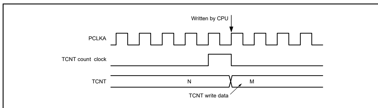
Figure 20.135 Contention between TCNT Write and Increment Operations
