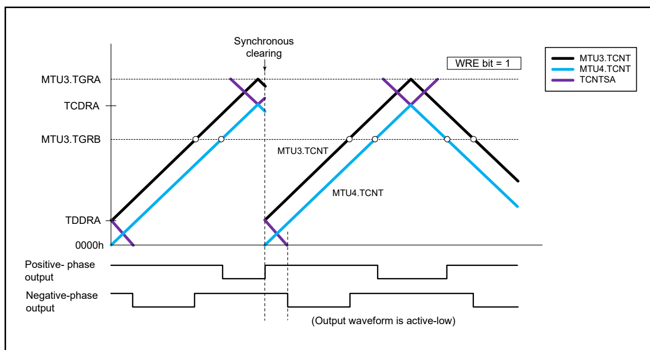
Figure 20.68 Example of Synchronous Clearing in Tb1 interval (Timing (6) in Figure 20.65; TWCRA.WRE Bit is 1)
