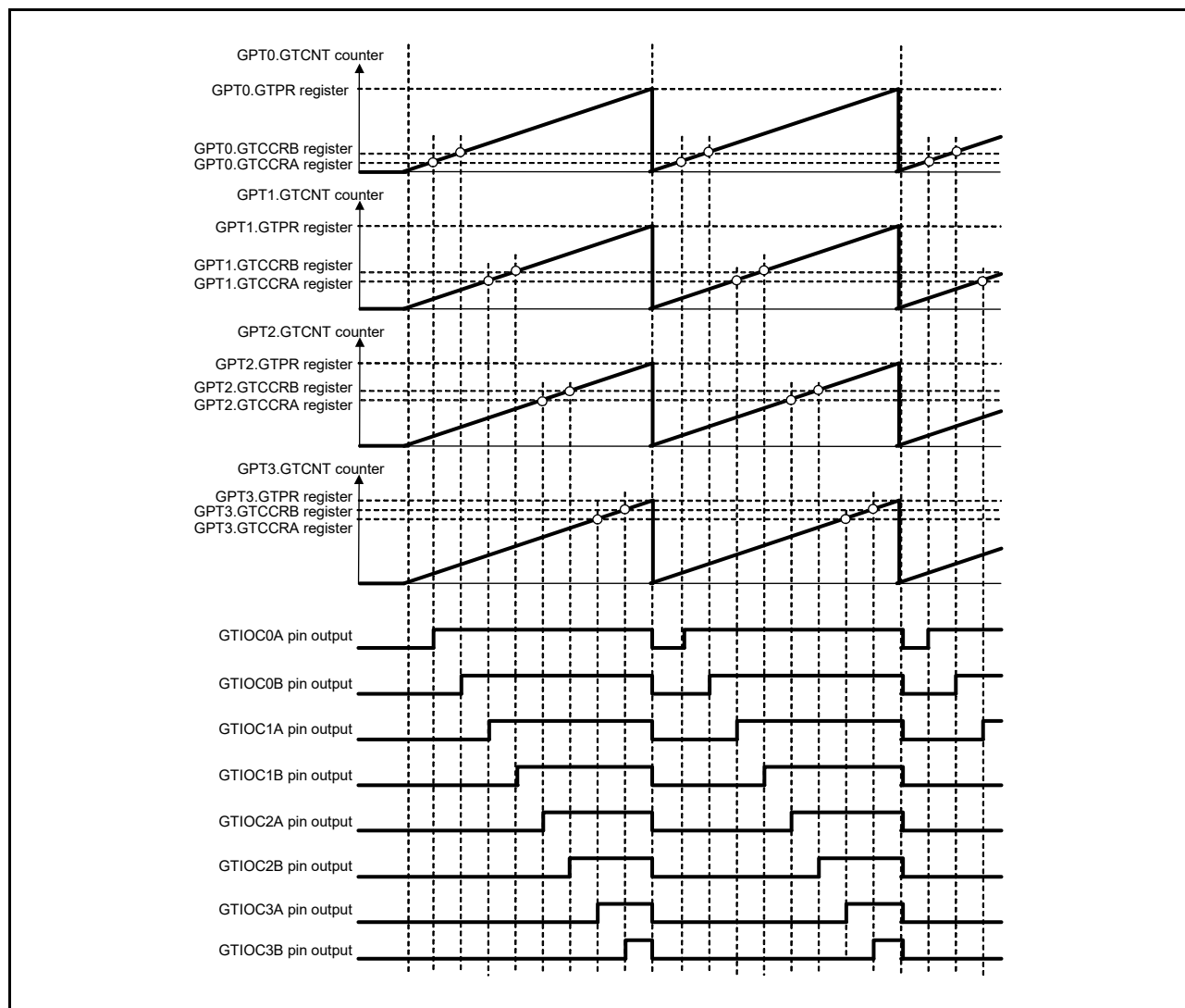
Figure 22.66 Example of Synchronous PWM Output
