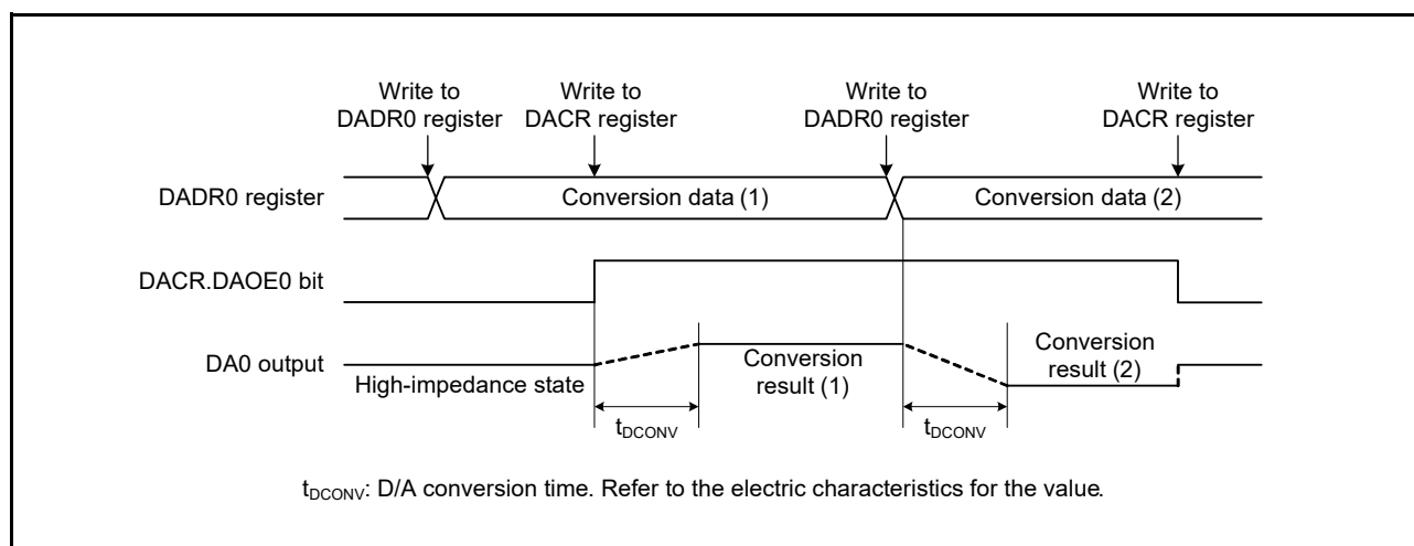
Figure 32.3 Example of 8-Bit D/A Converter Operation
