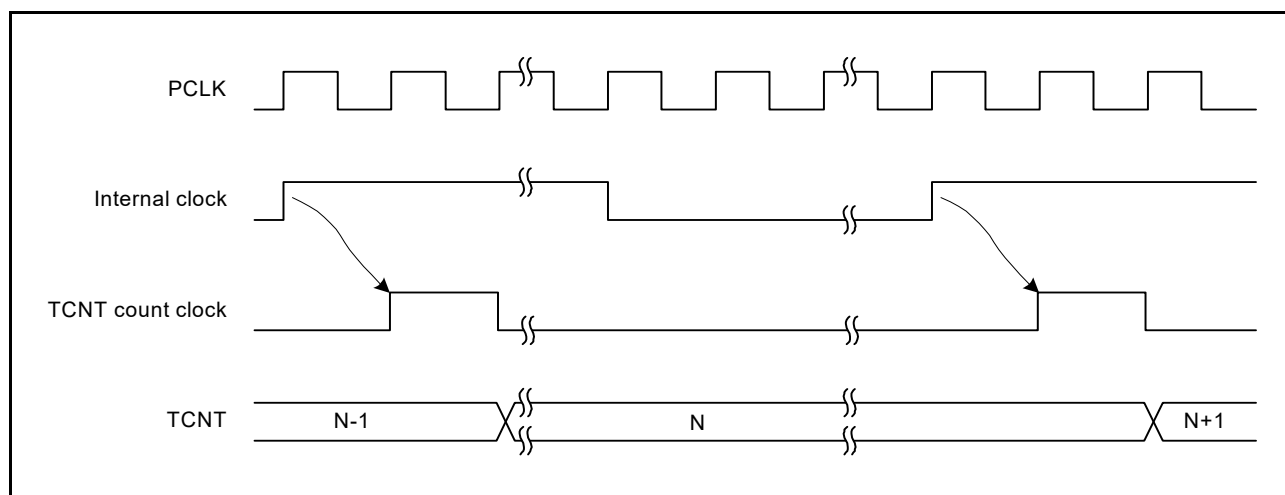
Figure 23.7 Count Timing for Internal Clock
