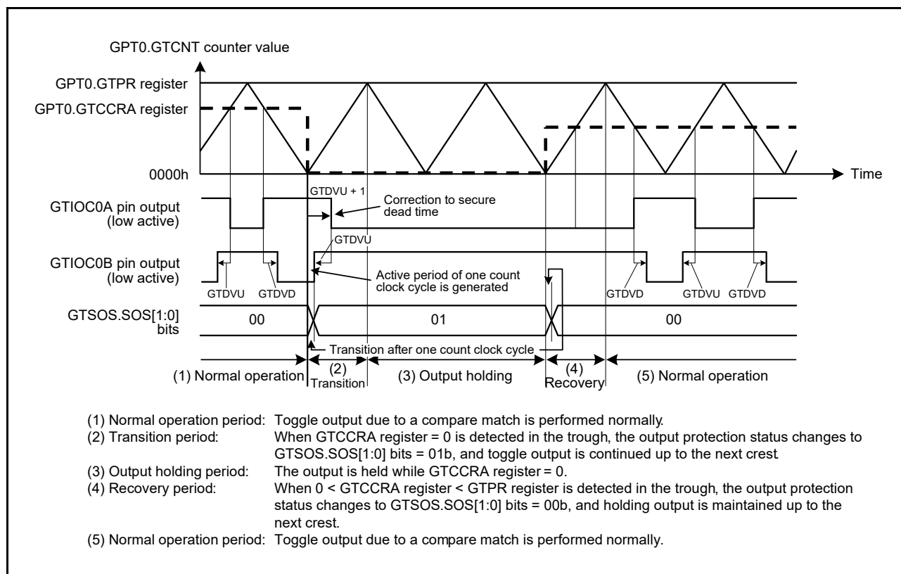
Figure 22.84 Example of Output Protection Function Operation When the GTCCRA Register is Set to 0000h during Buffer Transfer at Troughs (Restored to 0 < \text{GTCCRA} < \text{GTPR} during Buffer Transfer at Troughs, Active Level: Low)
