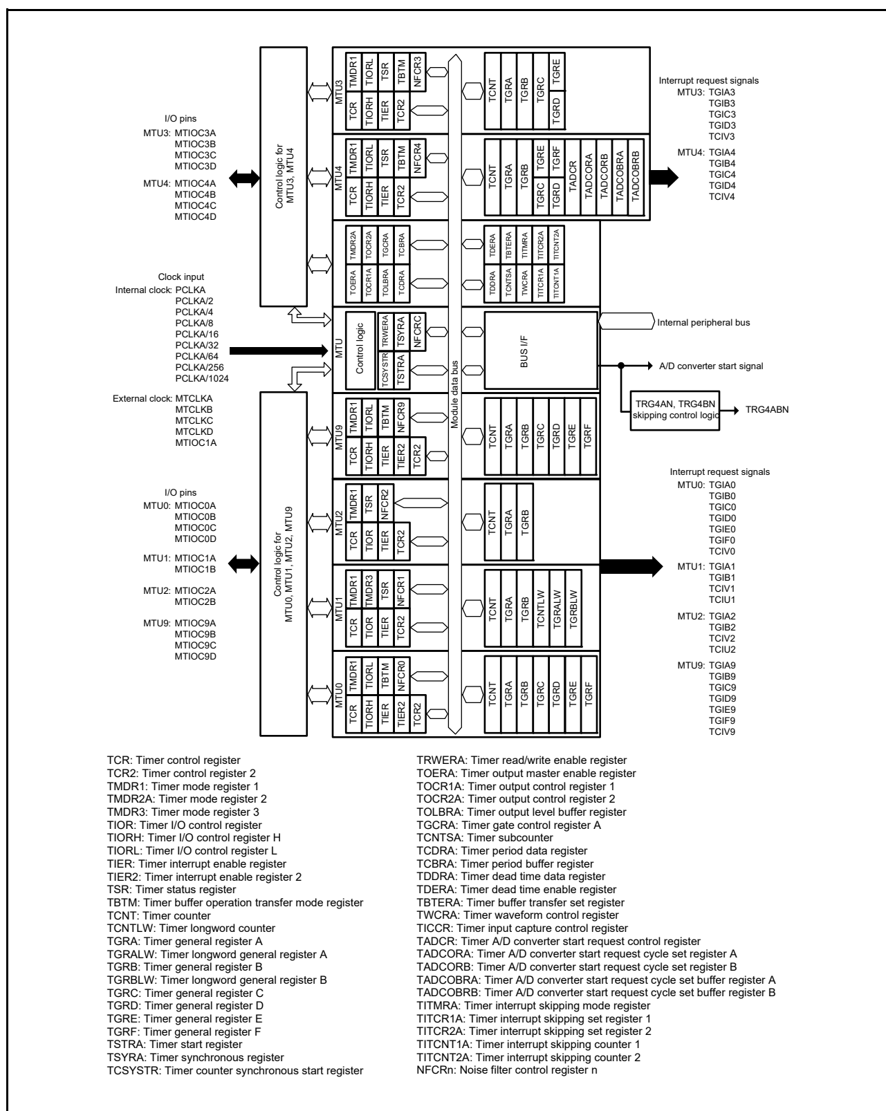
Figure 20.1 Block Diagram of MTU (MTU0 to MTU4, MTU9)
