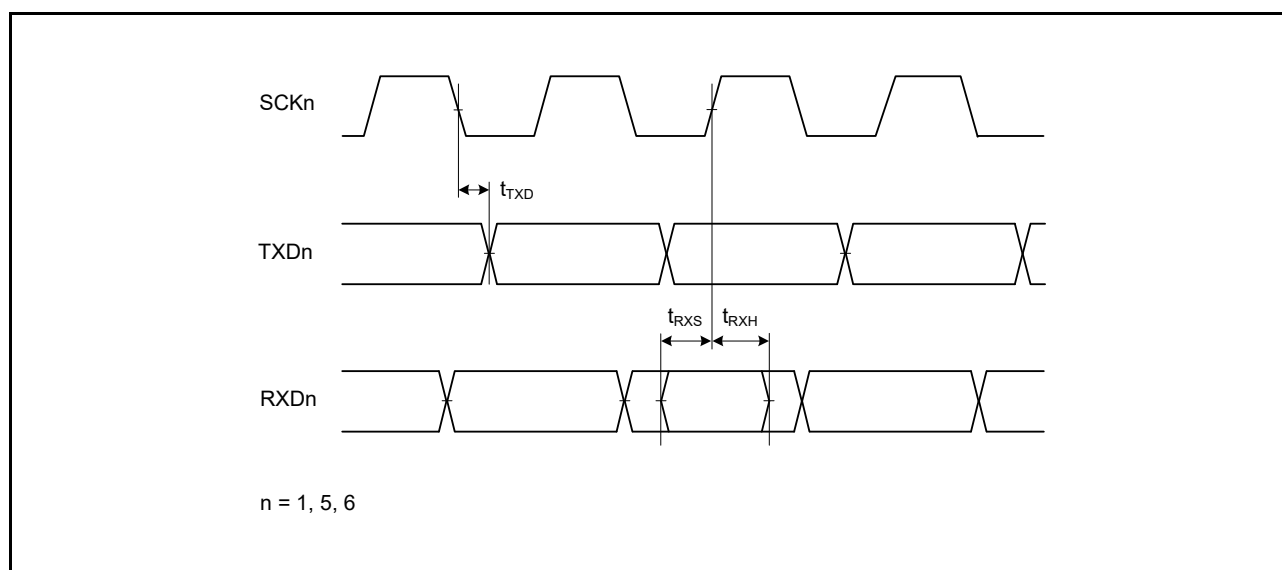
Figure 37.45 SCI Input/Output Timing: Clock Synchronous Mode
