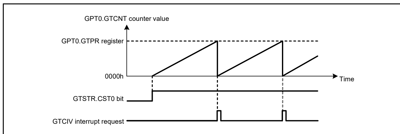
Figure 22.3 Example of Periodic Count Operation (in Up-Counting)
