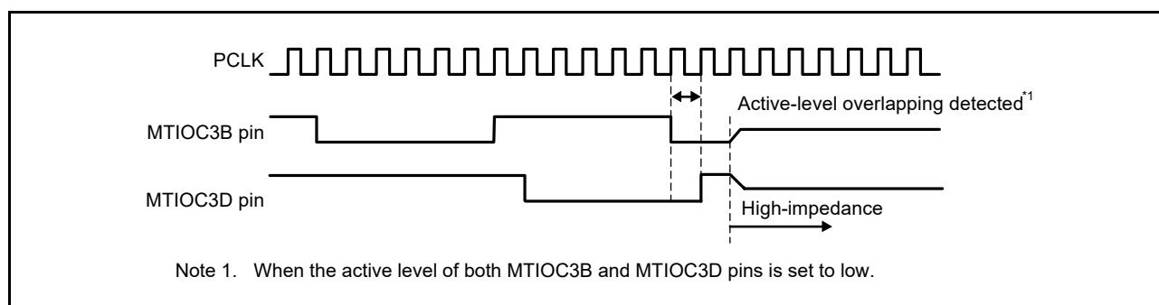
Figure 21.12 Output-Level Compare Operation
