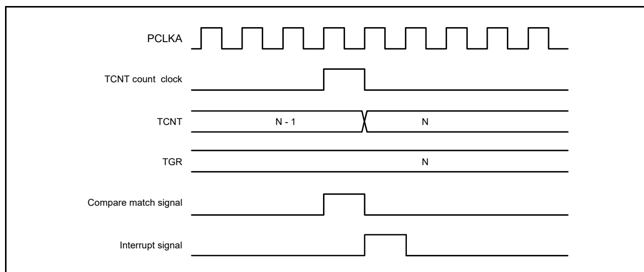
Figure 20.128 TGI Interrupt Timing (Compare Match) (MTU5)
