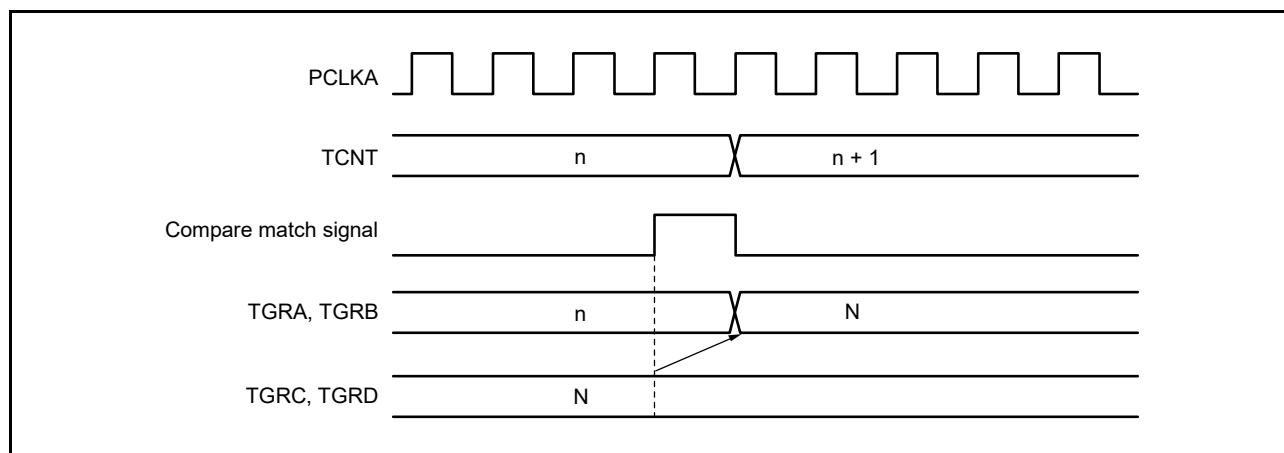
Figure 20.121 Buffer Operation Timing (Compare Match)
