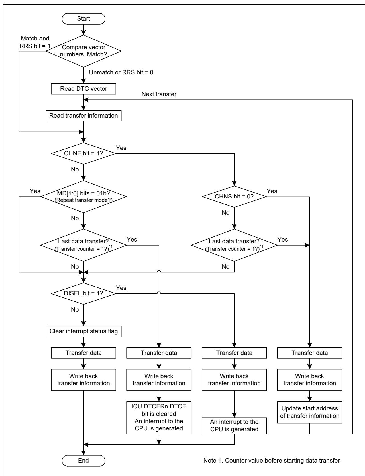
Figure 17.4 Operation Flowchart of the DTC
