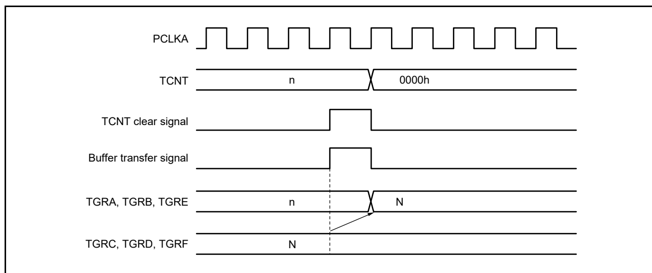
Figure 20.123 Buffer Operation Timing (When TCNT Cleared)
