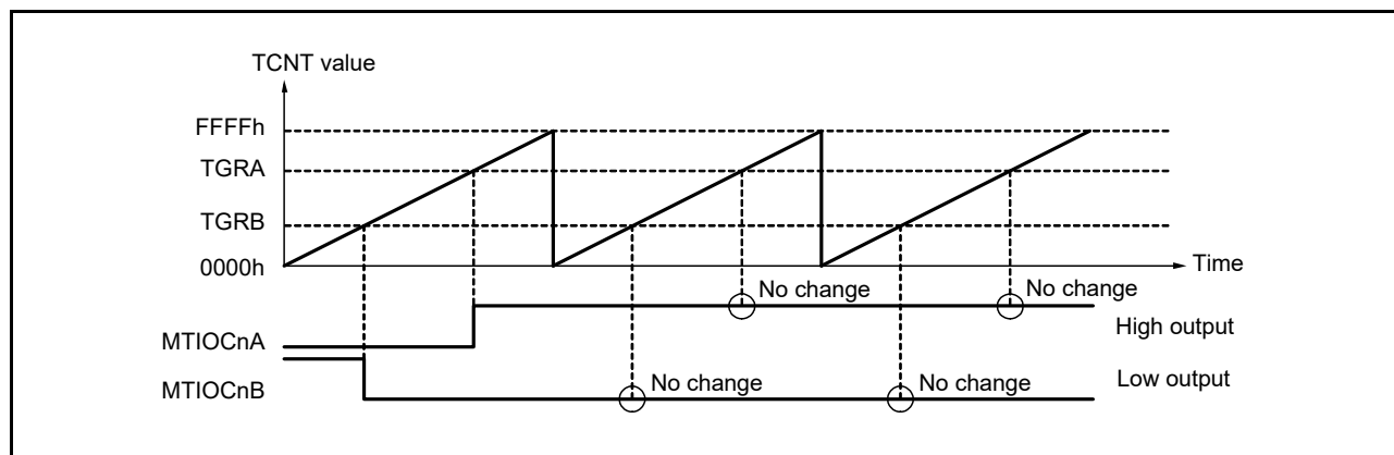
Figure 20.9 Example of low output and high output Operation (n = 0 to 4, 6, 7, 9)
