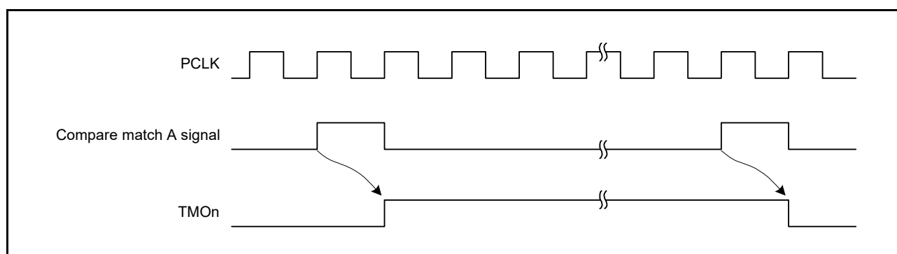
Figure 23.10 Timing of Timer Output Signal at Compare Match A Signal ( n = 0 to 7)
