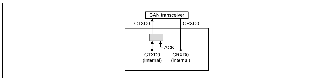
Figure 28.11 Connection When Self-Test Mode 0 is Selected
