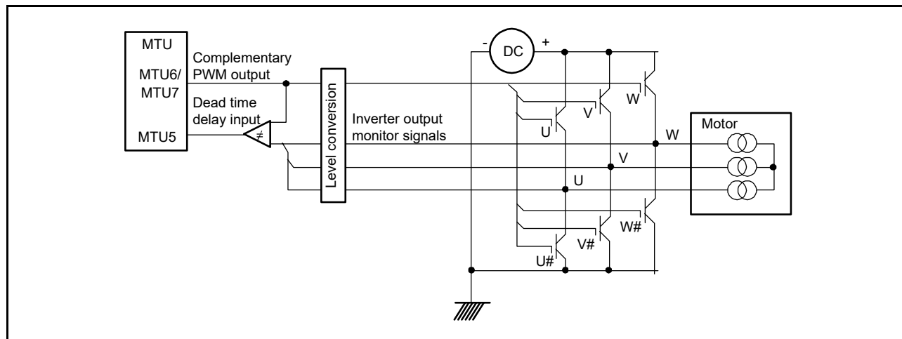
Figure 20.105 Motor Control Circuit Example
