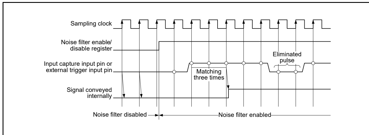
Figure 22.72 Timing of Noise Filtering
