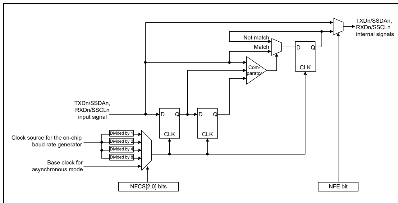
Figure 26.57 Block Diagram of Digital Noise Filter Circuit
