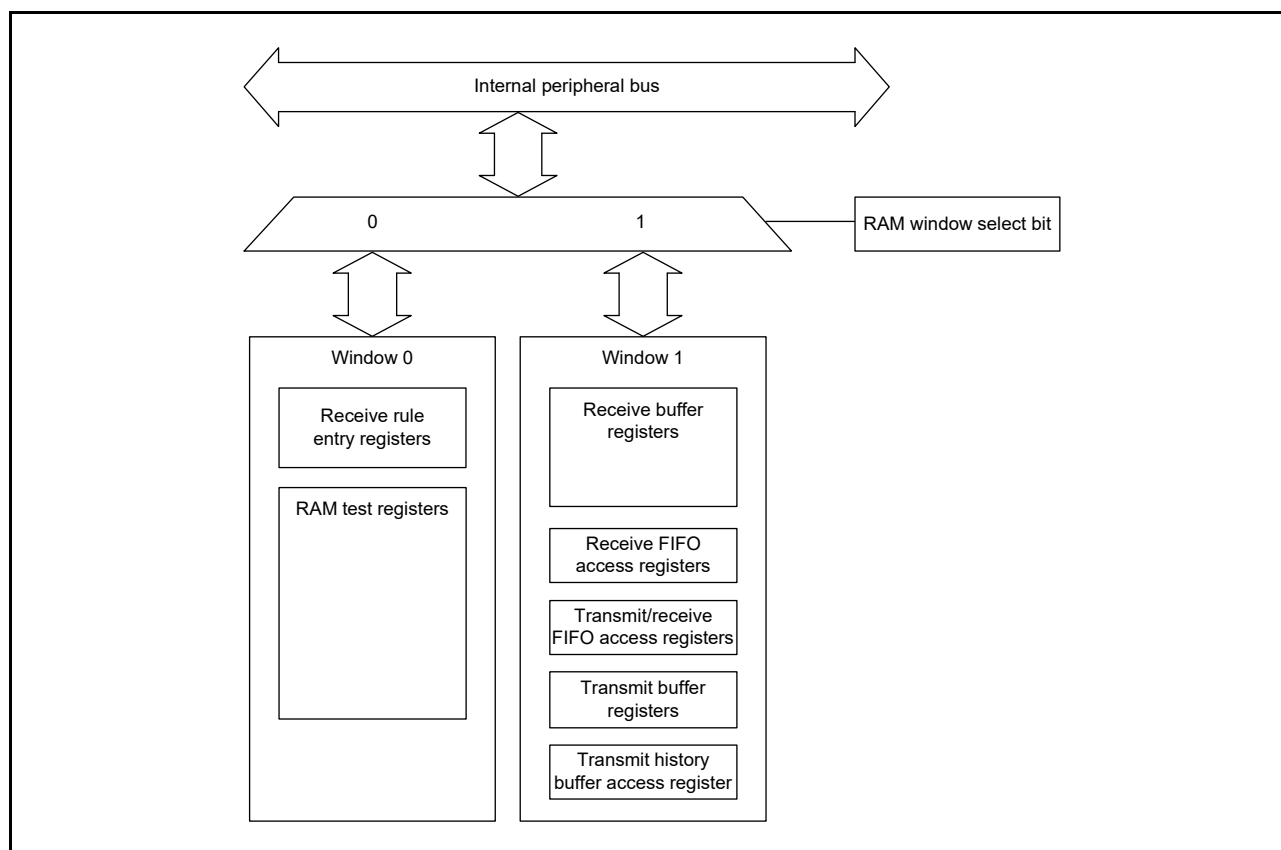
Figure 28.15 RAM Window
