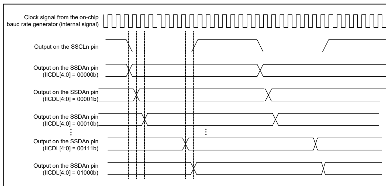
Figure 26.47 Timing of Delays in SSDA Output
