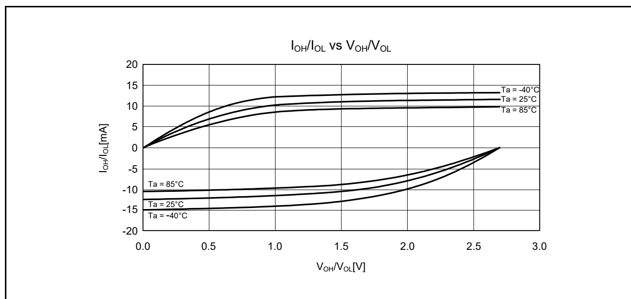
Figure 37.7 V_{OH}/V_{OL} and I_{OH}/I_{OL} Temperature Characteristics at V_{CC} = 2.7 V when Normal Output is Selected (Reference Data)
