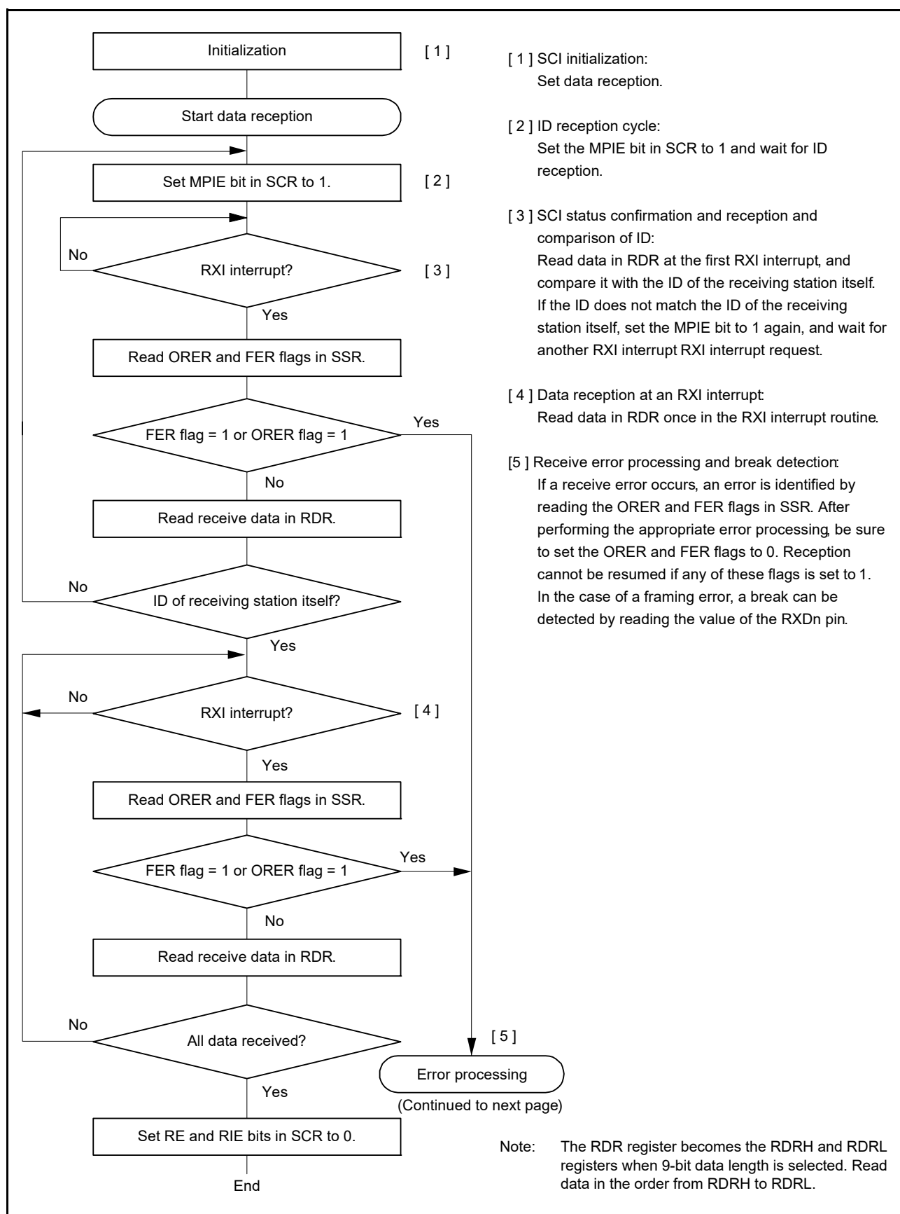
Figure 26.19 Example of Multi-Processor Serial Reception Flowchart (1)
