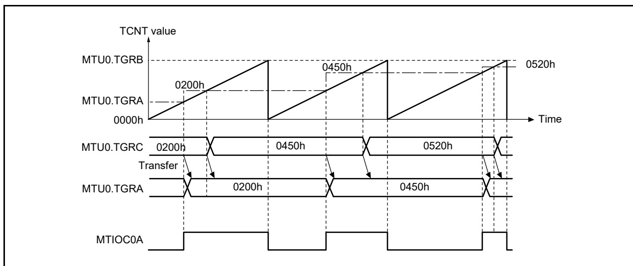
Figure 20.18 Example of Buffer Operation (1)
