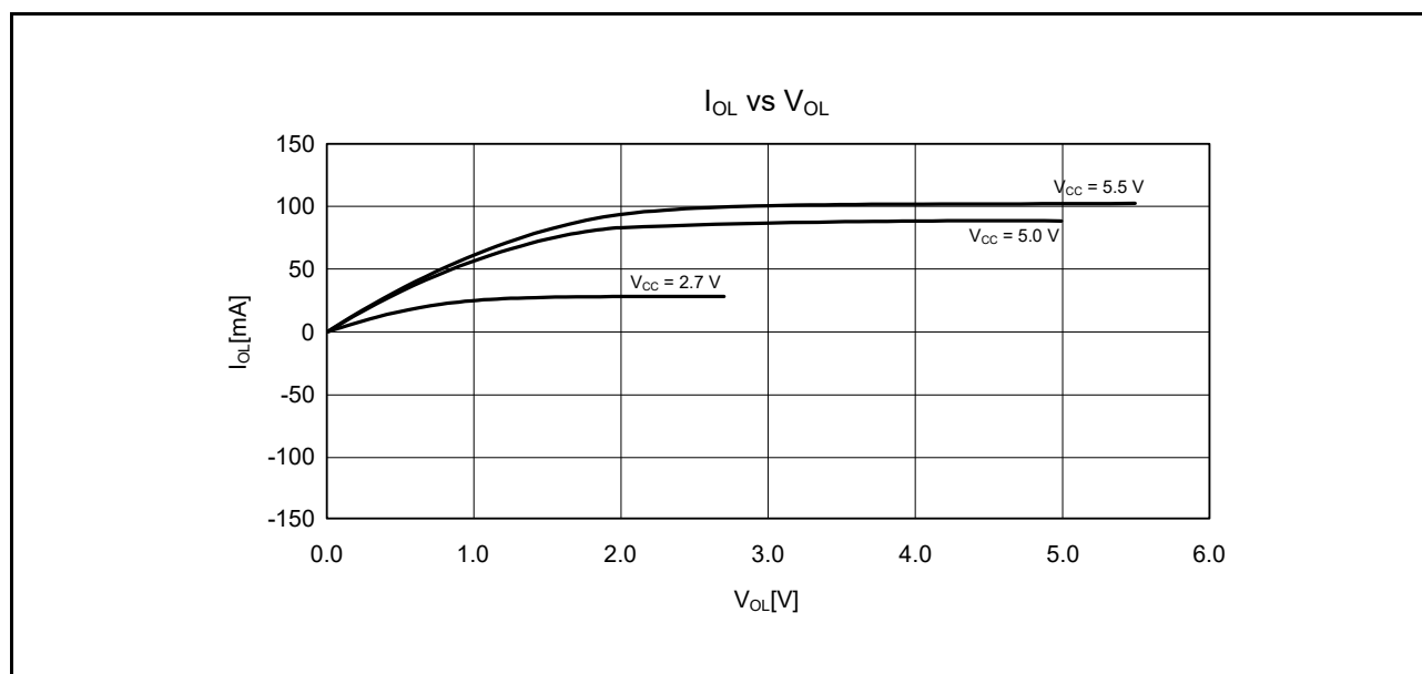
Figure 37.18 V_{OL} and I_{OL} Voltage Characteristics of RIIC Output Pin at T_a = 25^\circ\text{C} (Reference Data)
