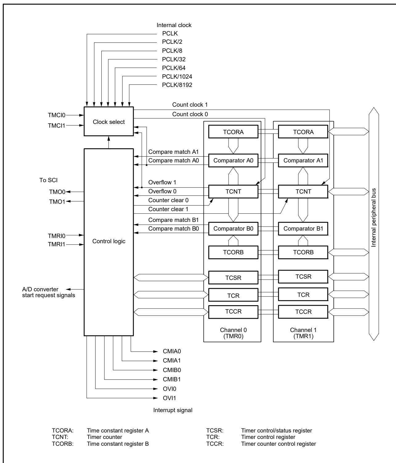
Figure 23.1 Block Diagram of TMR (Unit 0)
