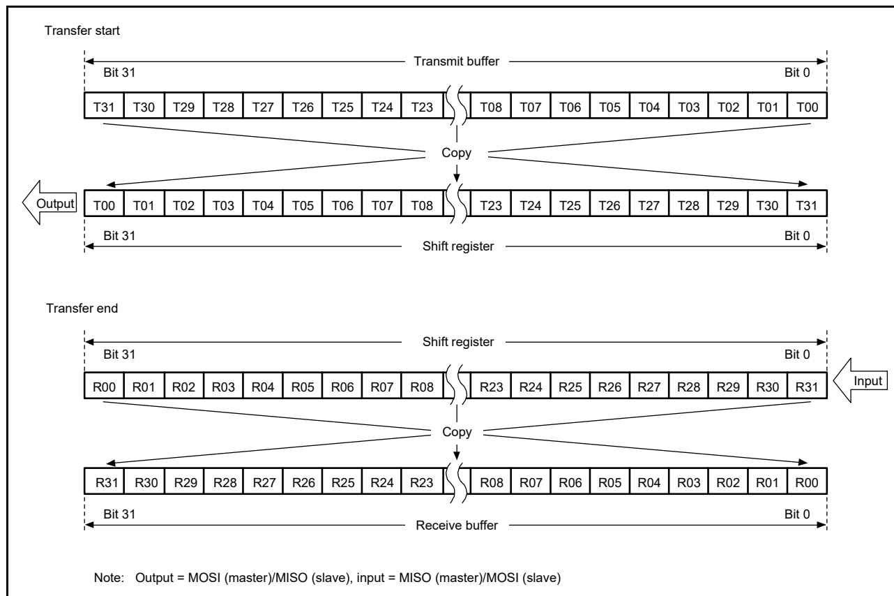
Figure 29.16 LSB First Transfer (32-Bit Data, Parity Disabled)
