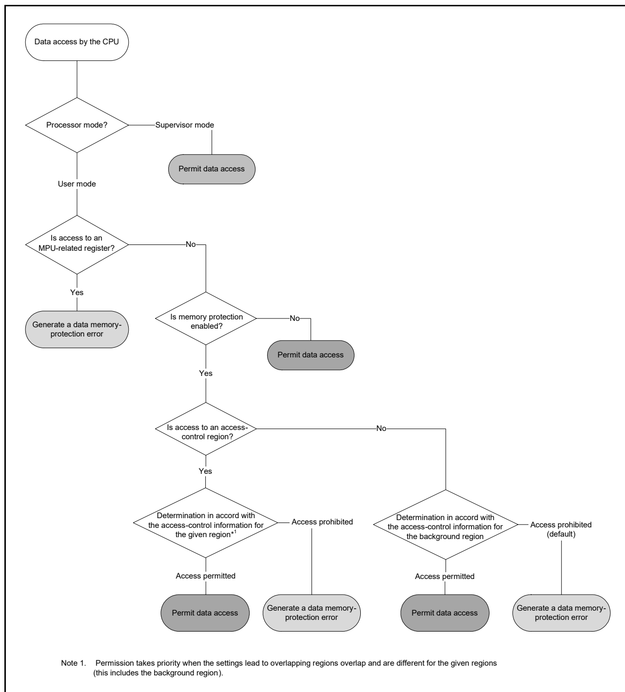
Figure 16.2 Flow of Determination for Data Access
