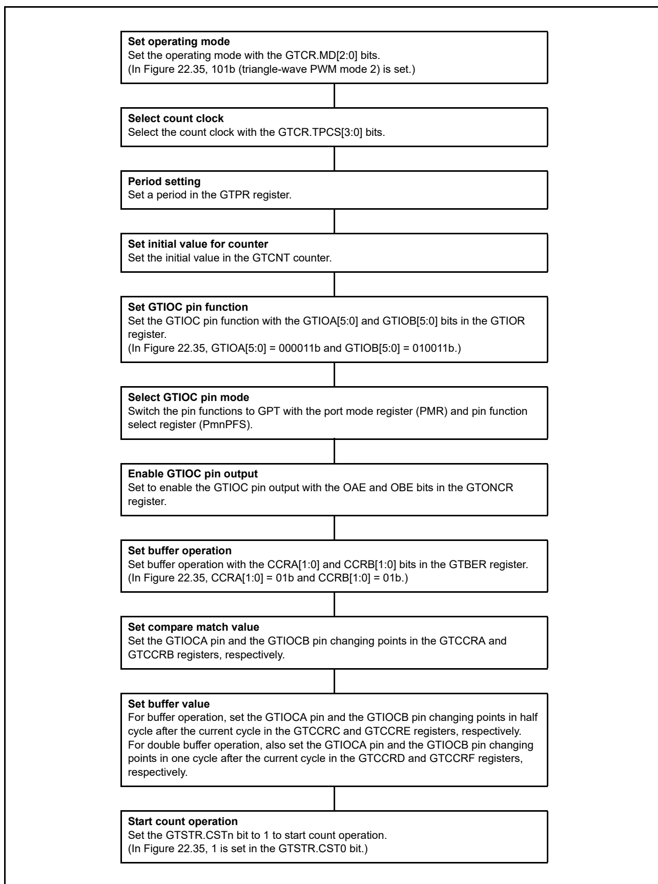
Figure 22.36 Example for Setting Triangle-Wave PWM Mode 2
