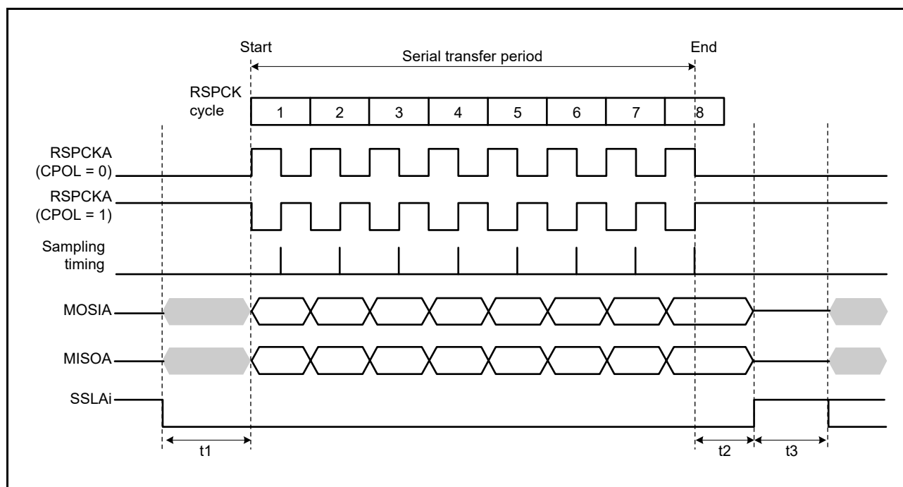
Figure 29.23 RSPI Transfer Format (CPHA = 1)
