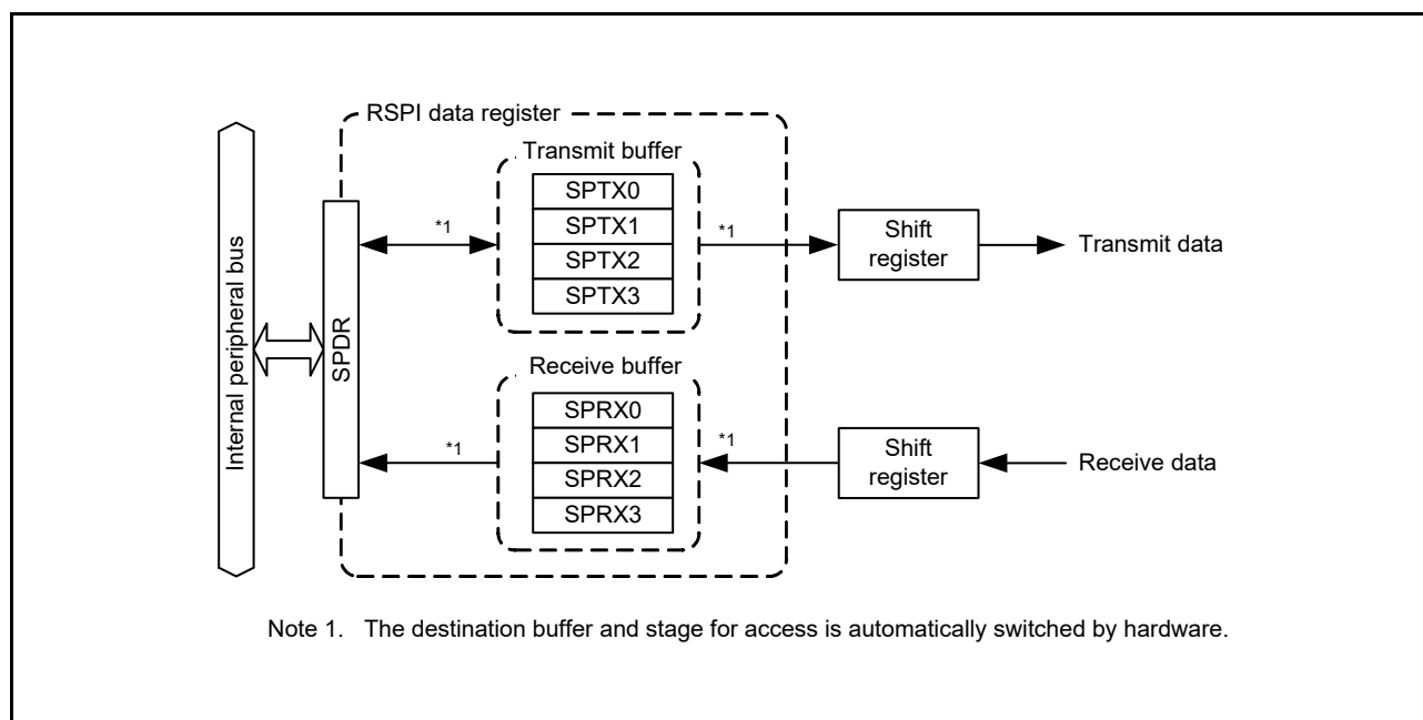
Figure 29.2 Configuration of SPDR
