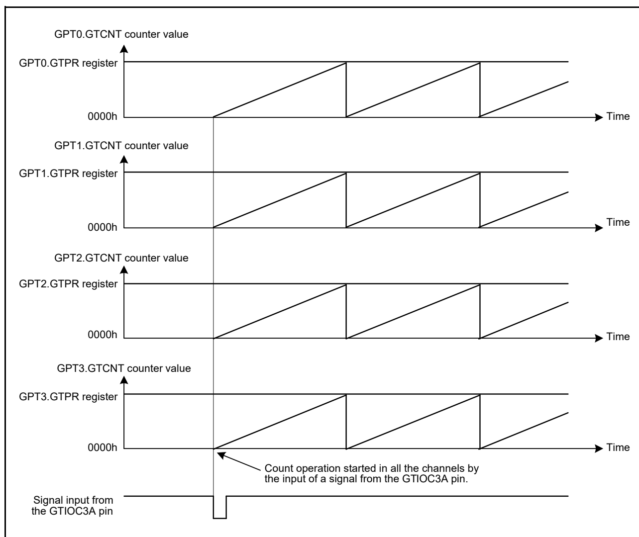
Figure 22.62 Example of Simultaneous Start Operation by Hardware Source (with Same Count Period (GTPR Value))
