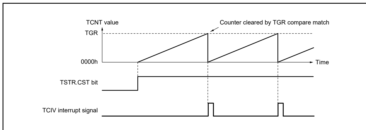
Figure 20.7 Periodic Counter Operation
