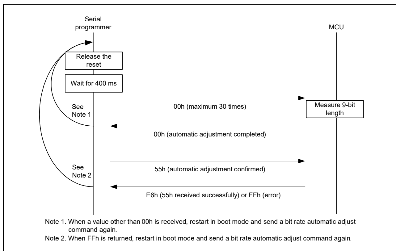
Figure 36.31 Bit Rate Automatic Adjustment Procedure
