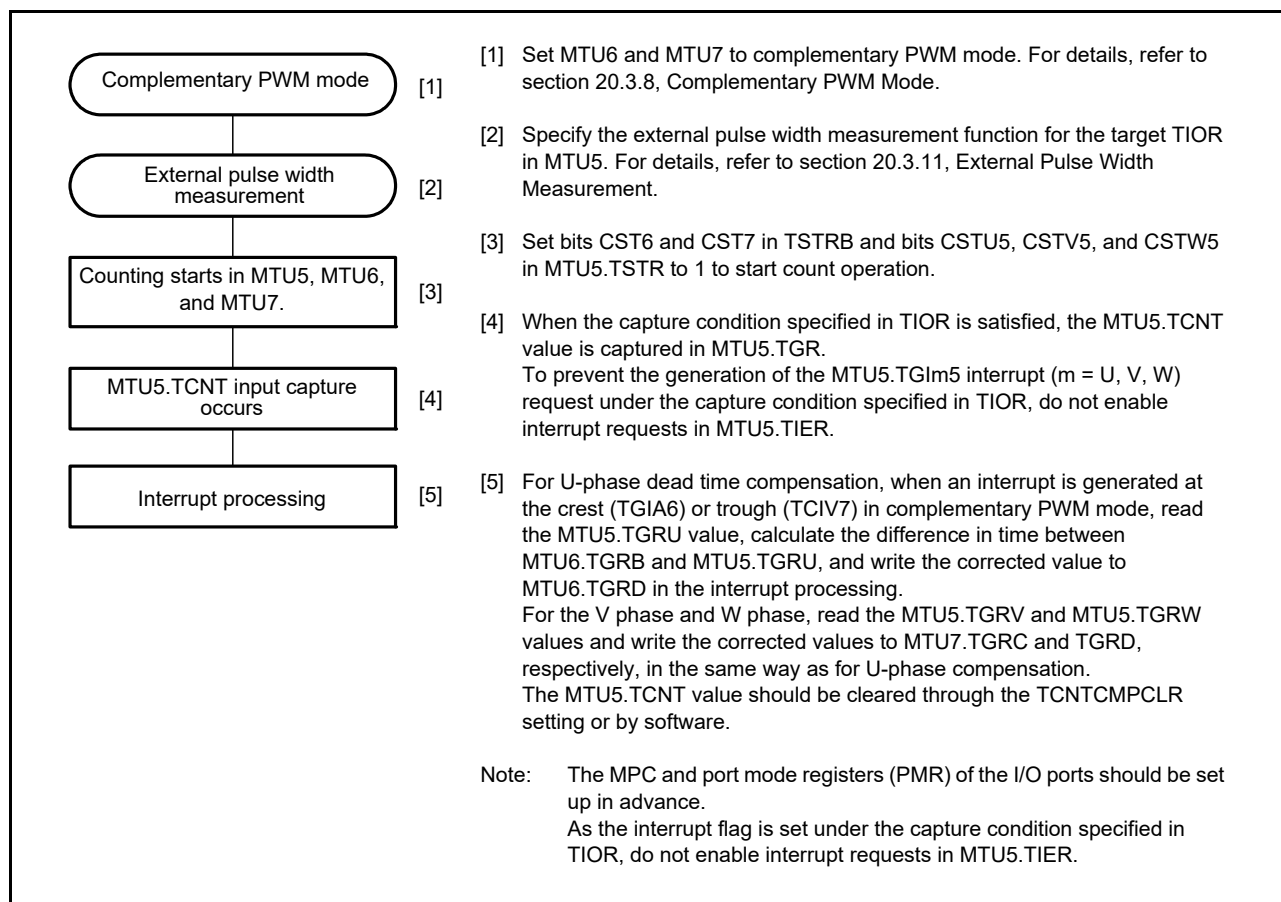
Figure 20.107 Example of Dead Time Compensation Setting Procedure
