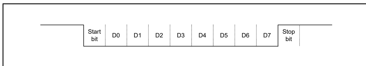
Figure 36.23 Communication Format
