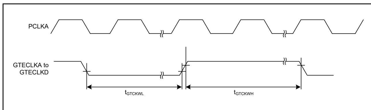
Figure 37.42 GPT Clock Input Timing
