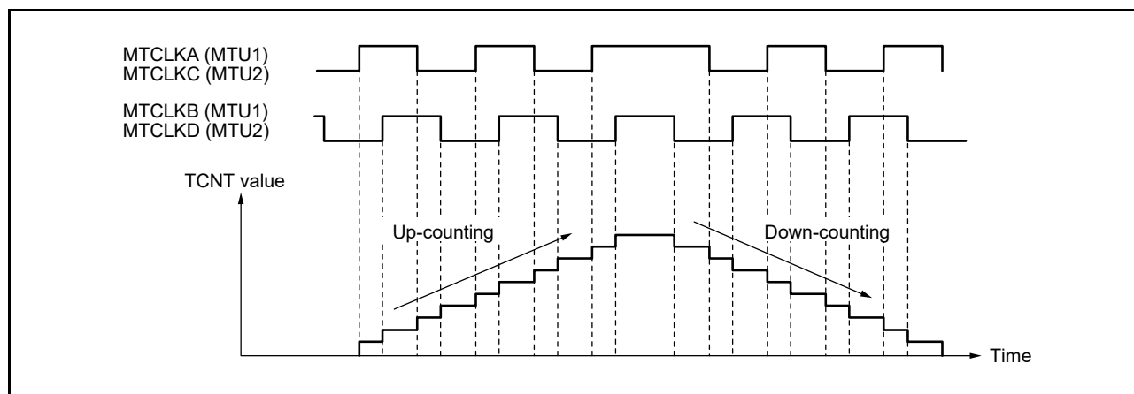
Figure 20.31 Example of Operation in Phase Counting Mode 1
