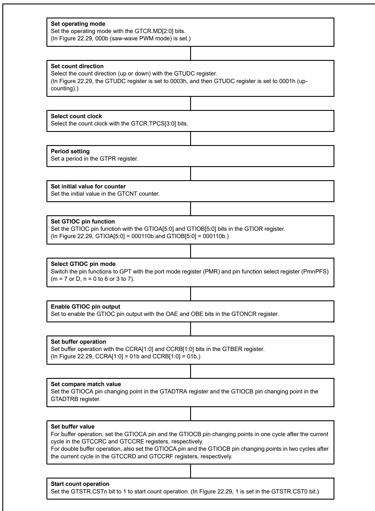
Figure 22.30 Example for Setting Saw-Wave PWM Mode
