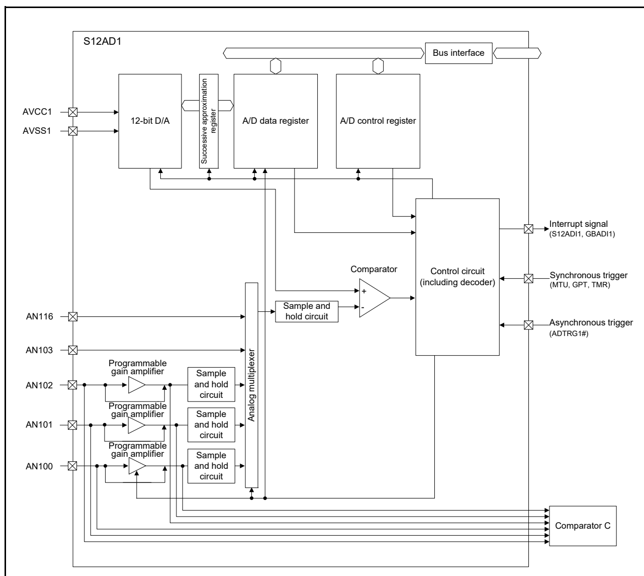
Figure 31.2 Block Diagram of 12-Bit A/D Converter (Unit 1)
