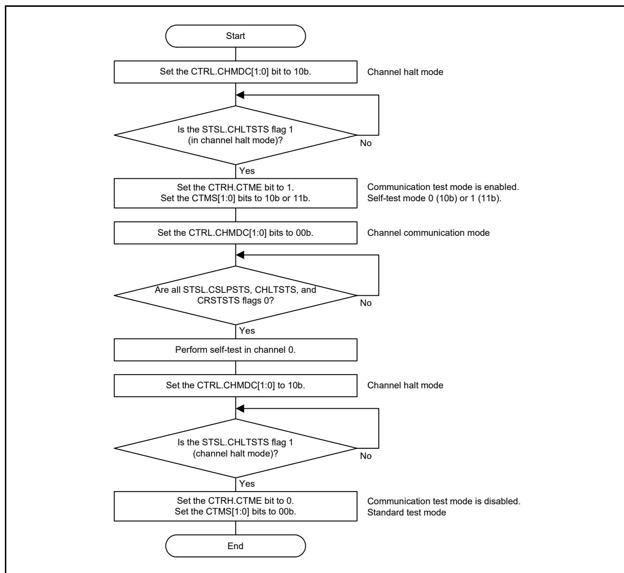
Figure 28.33 Self-Test Mode Setting Procedure
