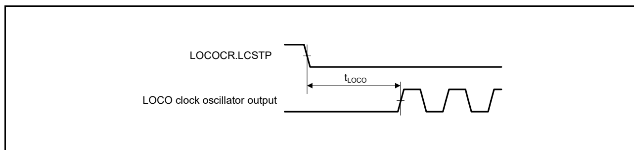
Figure 37.24 LOCO Clock Oscillation Start Timing
