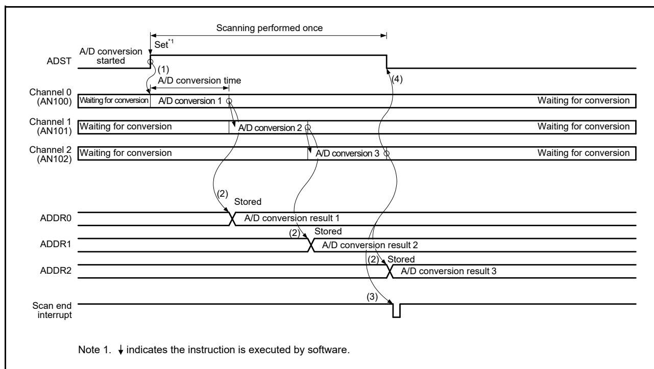
Figure 31.5 Example of Operation in Single Scan Mode (Basic Operation: AN100, AN101, AN102 Selected)
