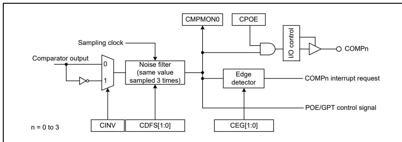
Figure 33.4 Noise Filter and Edge Detector Configuration
