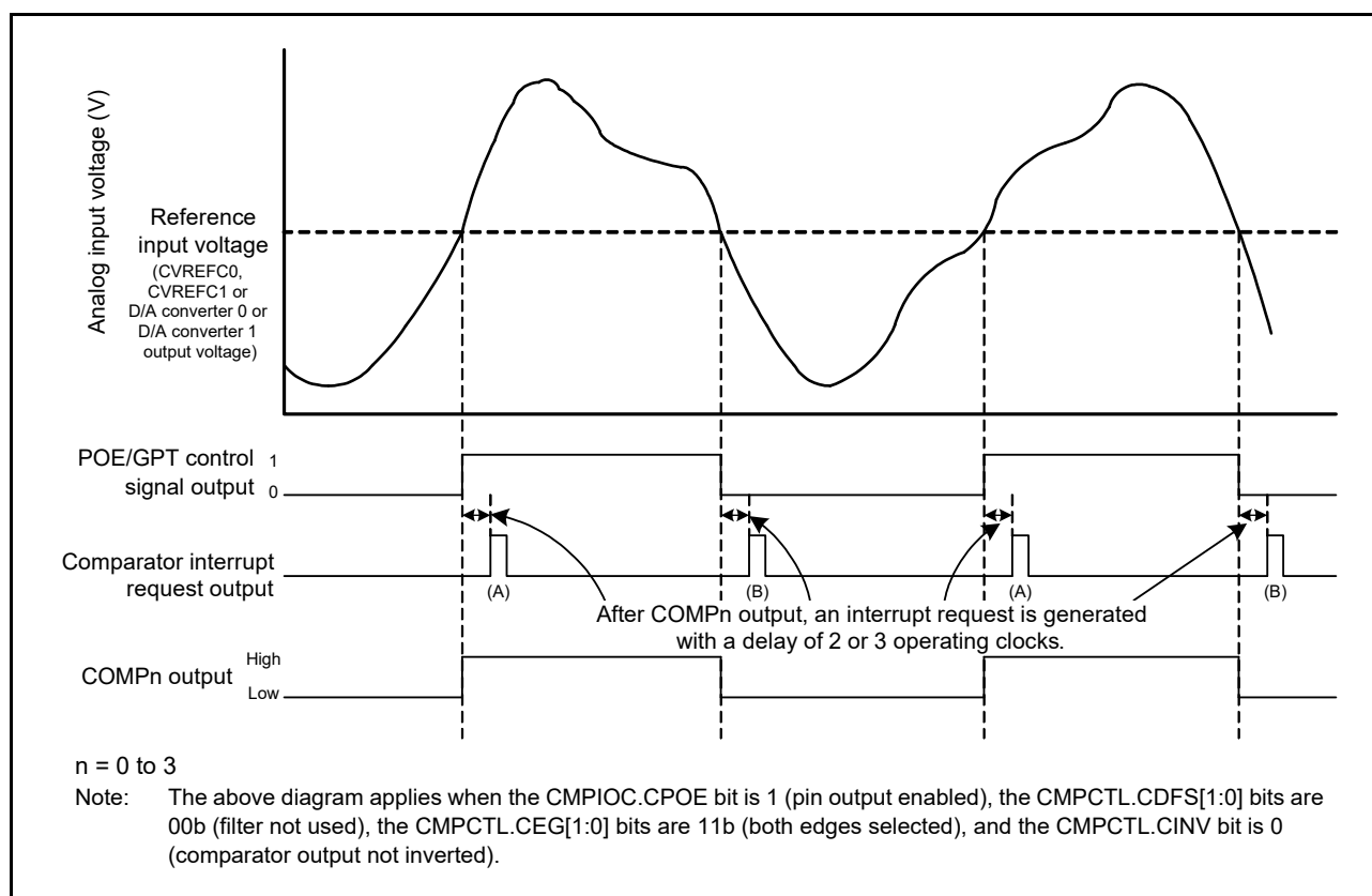
Figure 33.3 Comparator Operation Example
