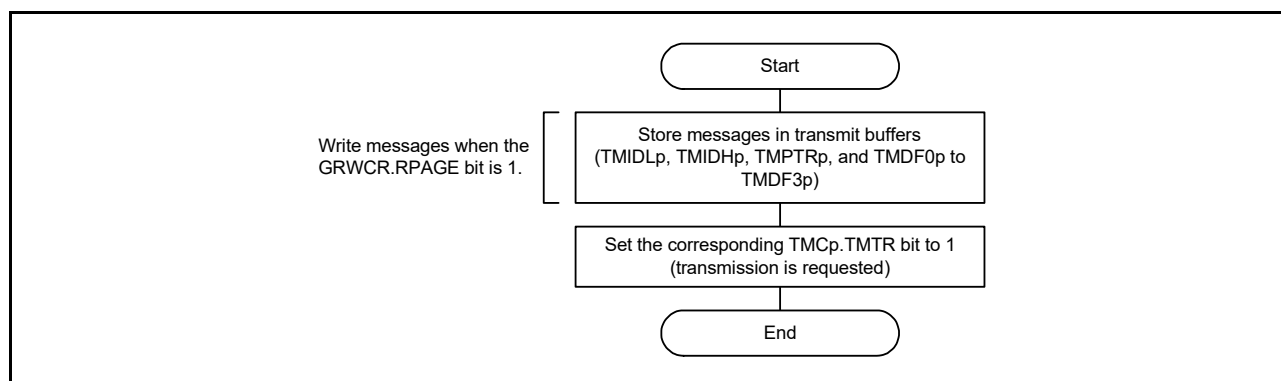
Figure 28.26 Procedure for Transmission from Transmit Buffers
