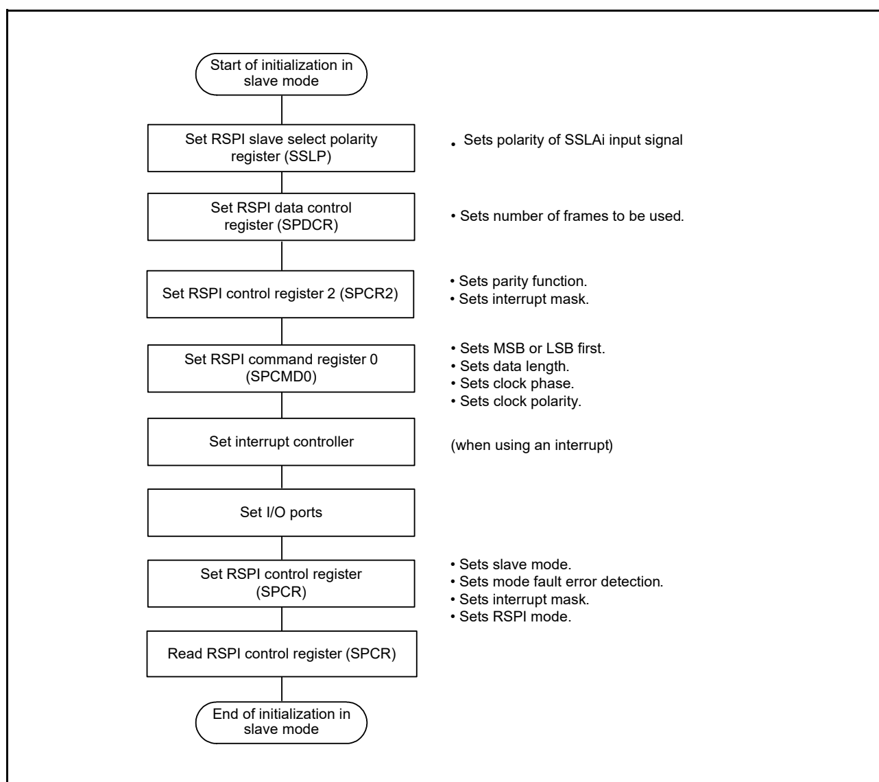
Figure 29.39 Example of Initialization Flowchart in Slave Mode (SPI Operation)
