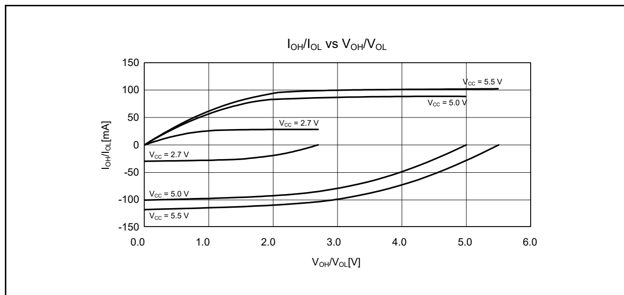
Figure 37.10 V_{OH}/V_{OL} and I_{OH}/I_{OL} Voltage Characteristics at T_a = 25^\circ\text{C} When Normal Output is Selected (Reference Data)
