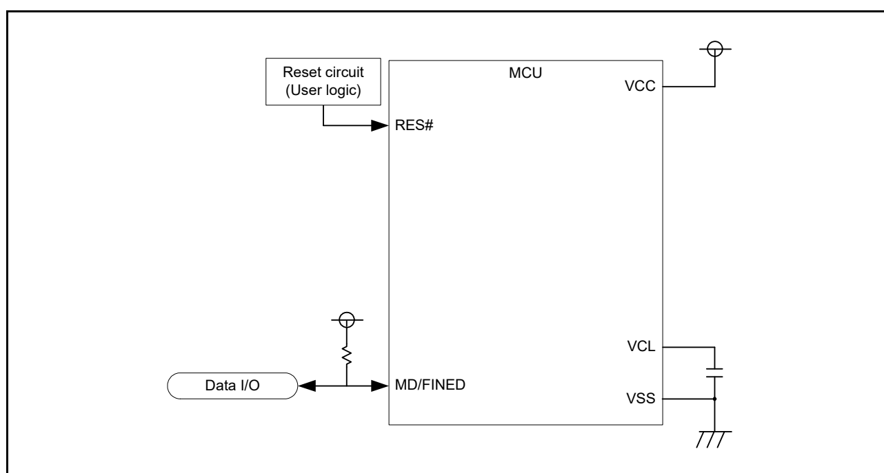
Figure 36.25 Example of Pin Connections in Boot Mode (FINE Interface)
