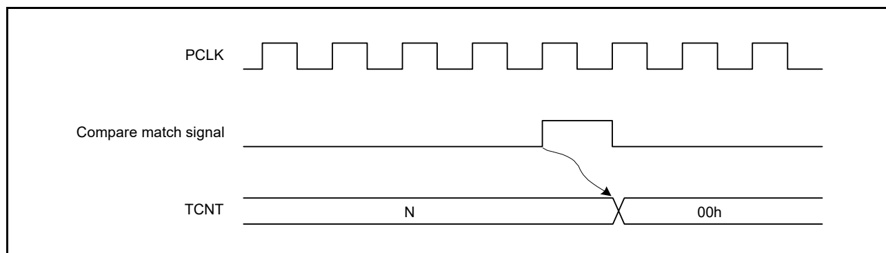
Figure 23.11 Timing of Counter Clear by Compare Match
