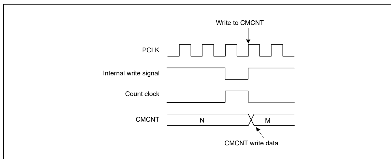
Figure 24.6 Conflict between CMCNT Counter Writing and Incrementing
