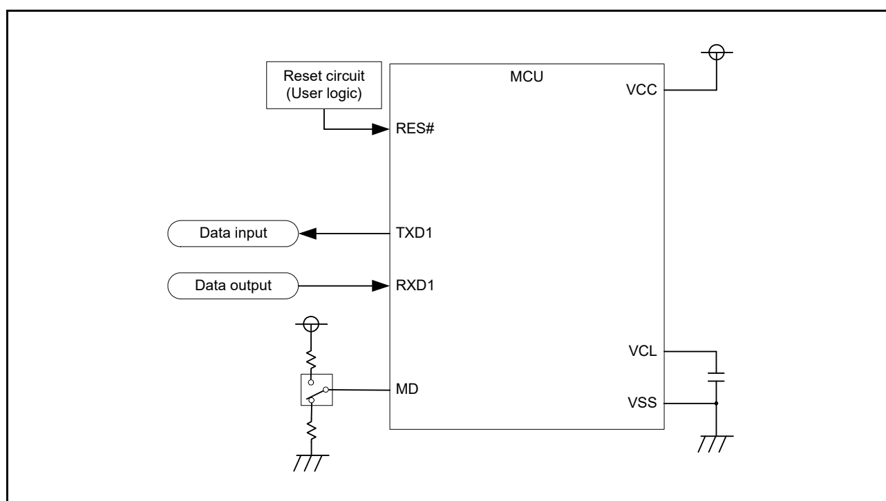
Figure 36.22 Example of Pin Connections in Boot Mode (SCI)
