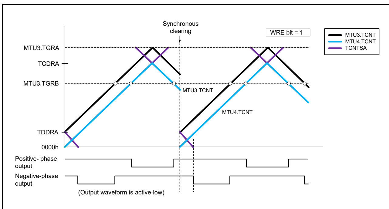
Figure 20.69 Example of Synchronous Clearing in Dead Time during Down-Counting (Timing (8) in Figure 20.65; TWCRA.WRE Bit is 1)
