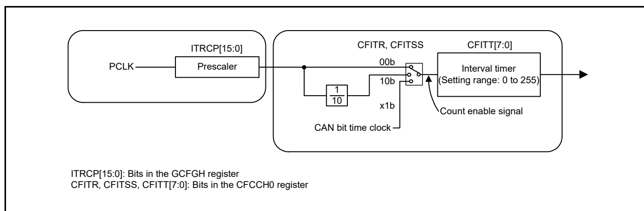
Figure 28.8 Interval Timer Block Diagram
