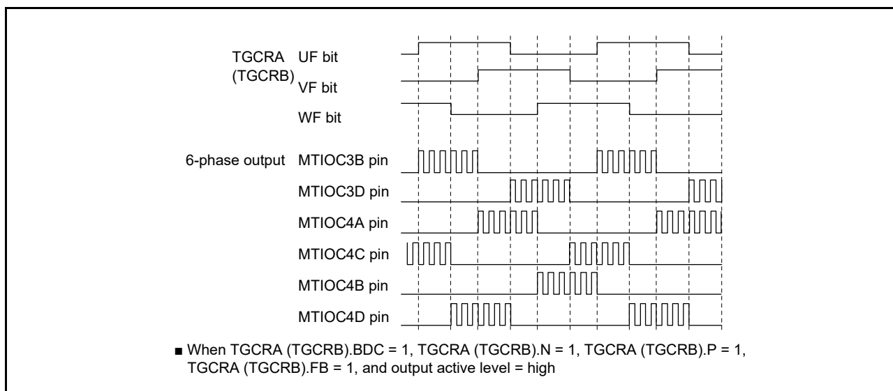
Figure 20.81 Example of Output Phase Switching through UF, VF, and WF Bit Settings (2)
