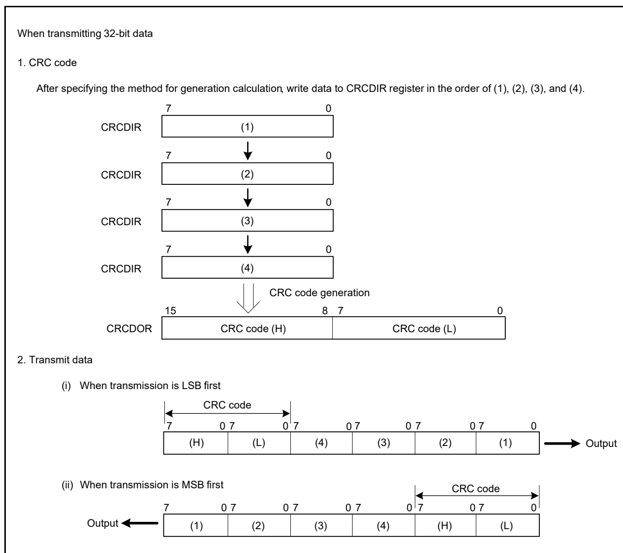
Figure 30.6 LSB First and MSB First Data Transmission
