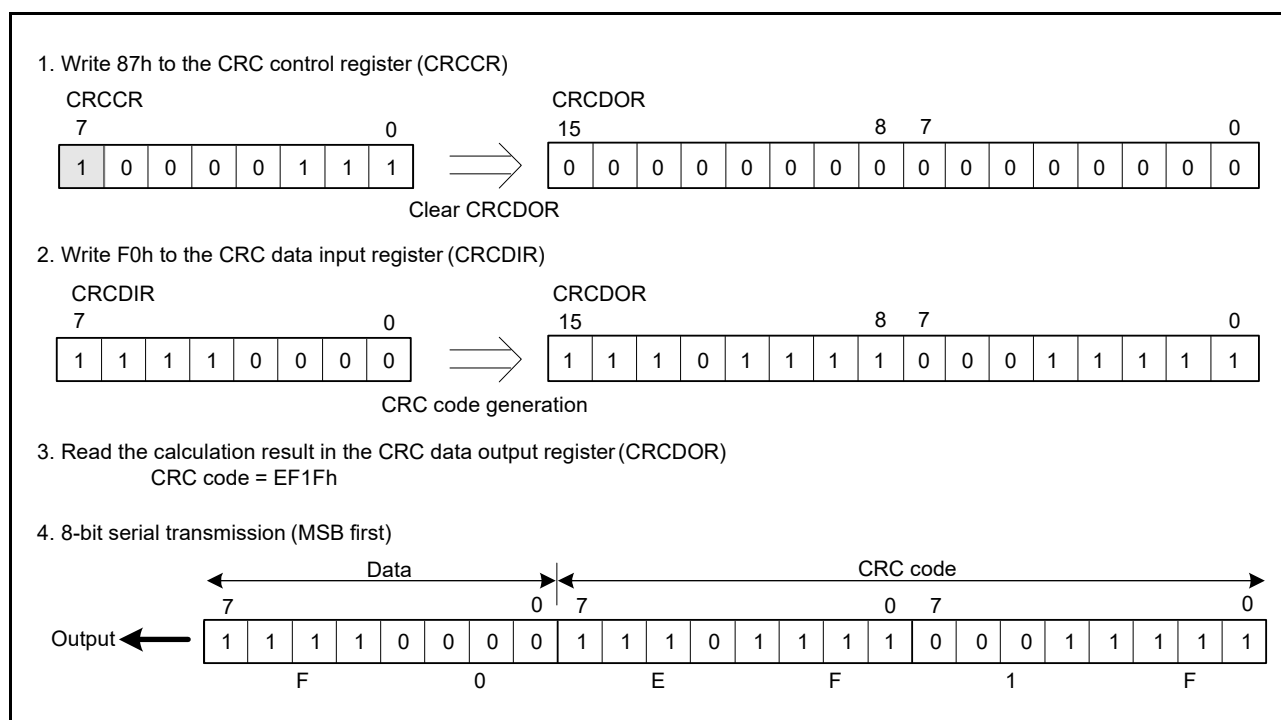
Figure 30.3 MSB First Data Transmission
