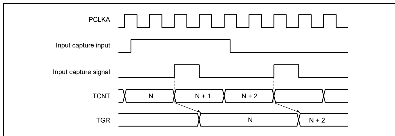
Figure 20.117 Input Capture Input Signal Timing
