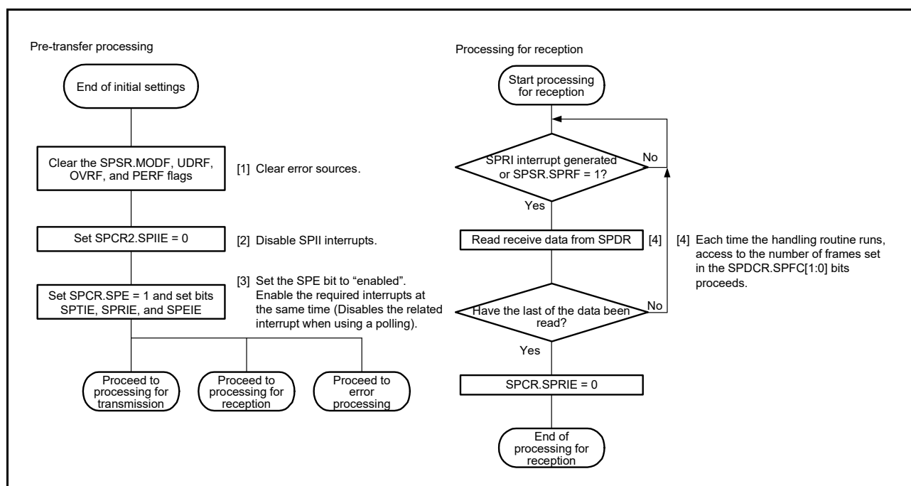
Figure 29.41 Flowchart in Slave Mode (Reception)
