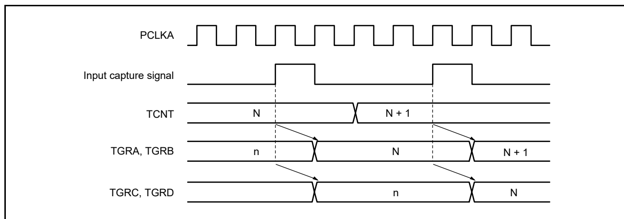
Figure 20.122 Buffer Operation Timing (Input Capture)
