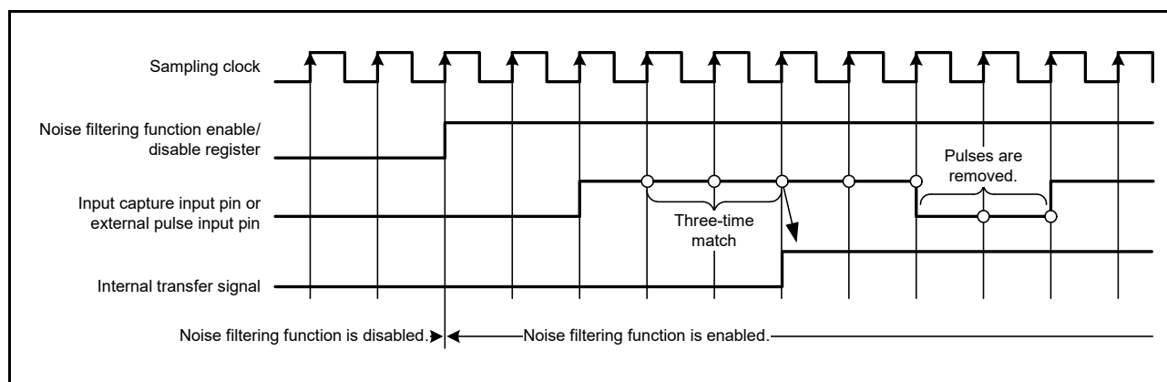
Figure 20.109 Timing of Noise Filtering
