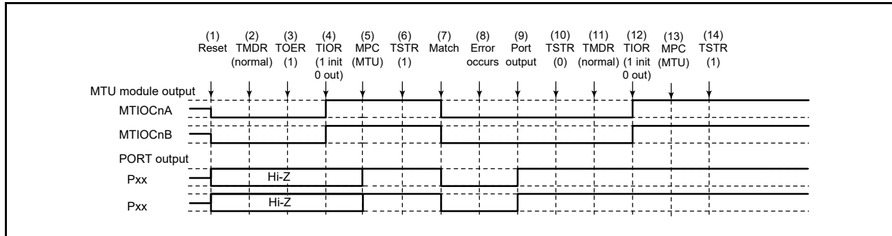
Figure 20.154 Error Occurrence in Normal Mode, Recovery in Normal Mode
