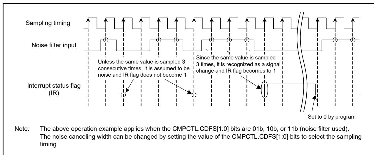
Figure 33.5 Comparator Noise Filter and Interrupt Operation Example
