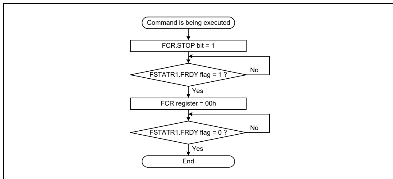
Figure 36.21 Procedure for Forced Stop of Software Commands
