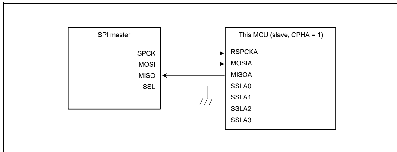
Figure 29.7 Single-Master/Single-Slave Configuration Example (This MCU = Slave, CPHA = 1)
