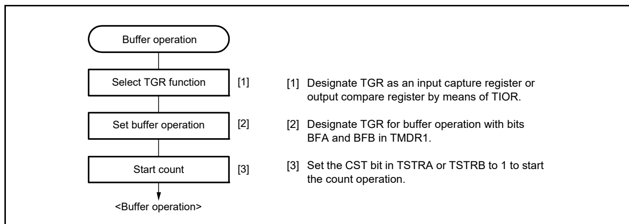
Figure 20.17 Example of Buffer Operation Setting Procedure
