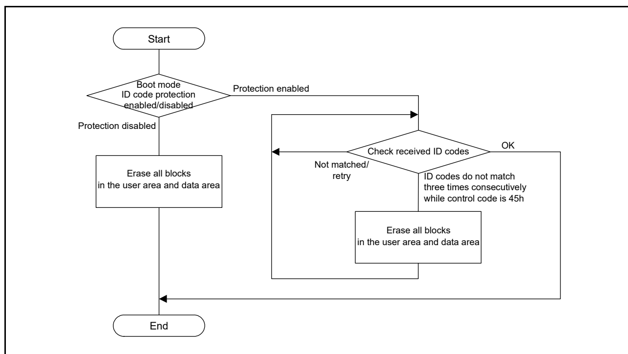
Figure 36.27 Authentication for Boot Mode ID Code Protection
