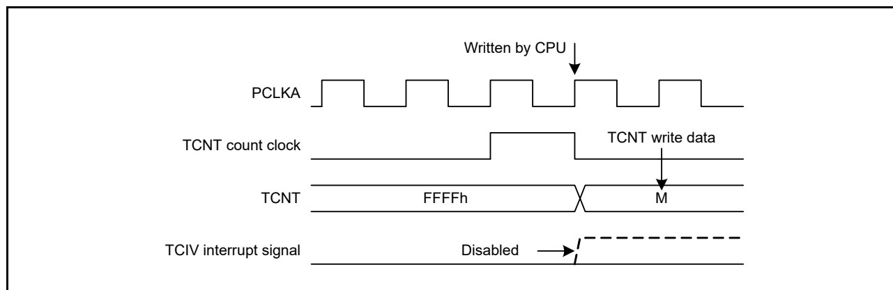
Figure 20.148 Contention between TCNT Write Operation and Overflow
