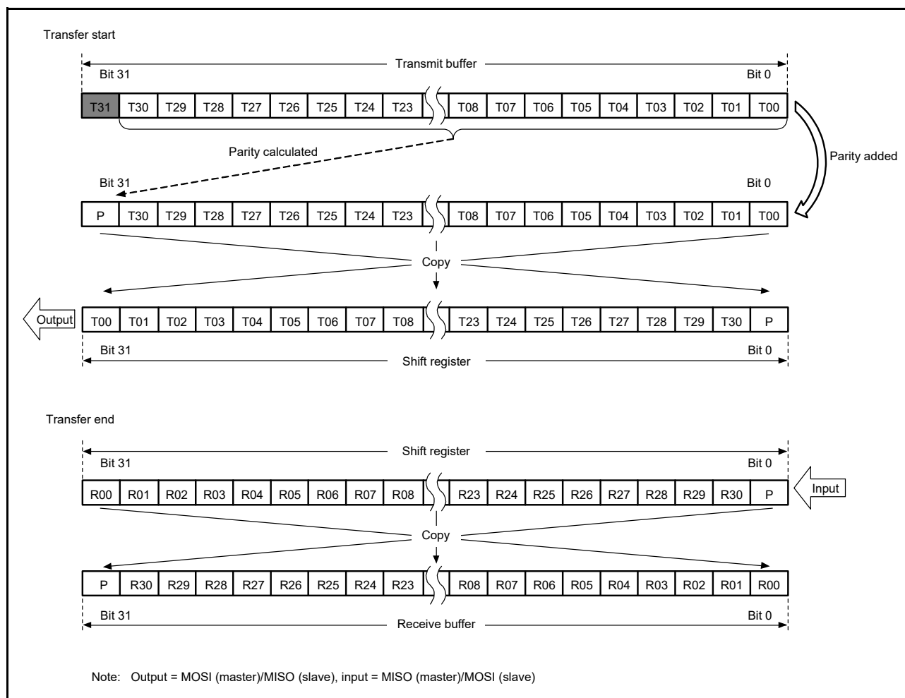
Figure 29.20 LSB First Transfer (32-Bit Data, Parity Enabled)
