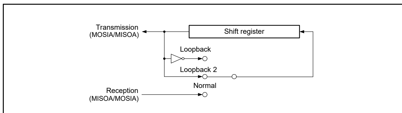
Figure 29.48 Configuration of Shift Register I/O Paths in Loopback Mode (Master Mode)
