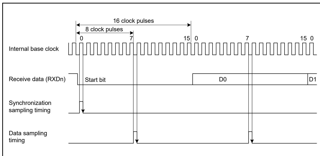
Figure 26.5 Receive Data Sampling Timing in Asynchronous Mode
