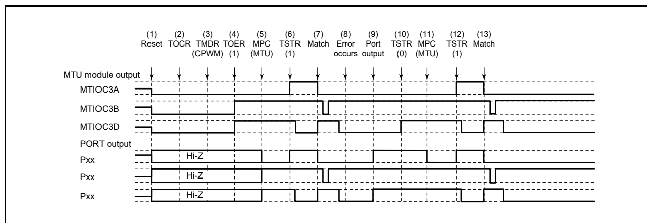
Figure 20.176 Error Occurrence in Complementary PWM Mode, Recovery in Complementary PWM Mode (1)
