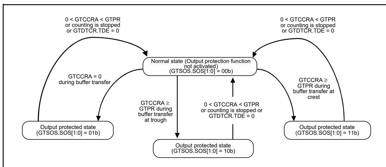
Figure 22.83 Output Protection Function
