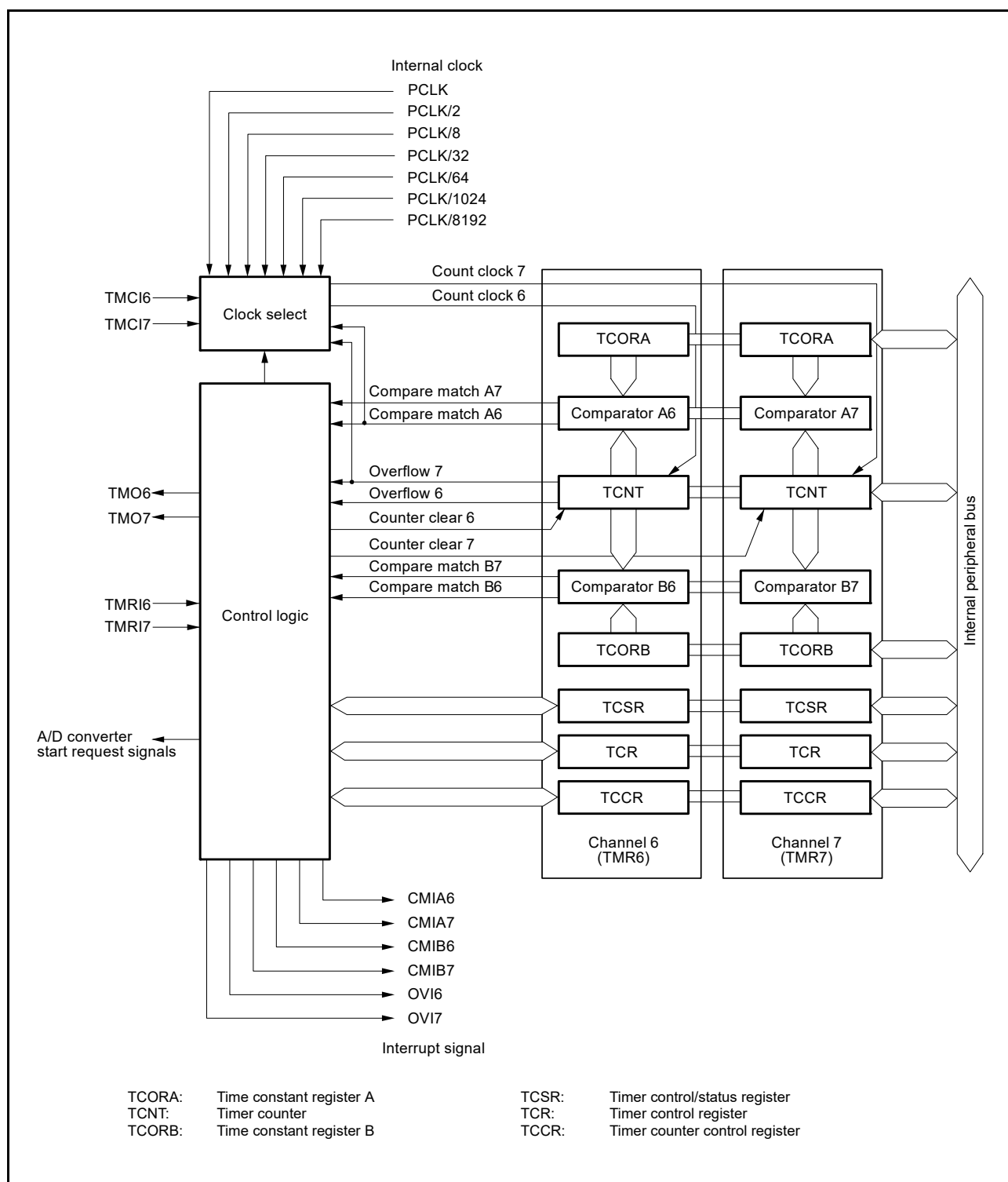
Figure 23.4 Block Diagram of TMR (Unit 3)
