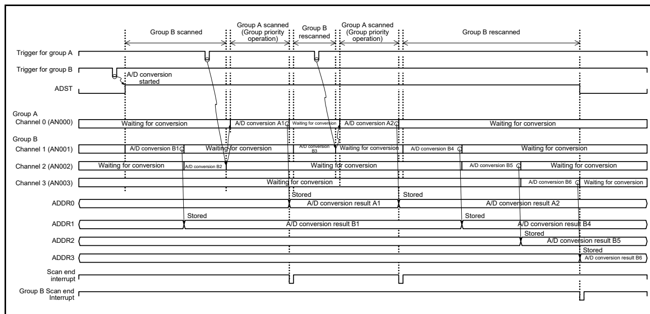
Figure 31.20 Example 2 of Group Priority Operation: Group A Trigger Input during Group B Rescan, With Rescan Setting (ADGSPCR.GBRSCN = 1, ADGSPCR.GBRP = 0, ADGSPCR.LGRRS = 0)
