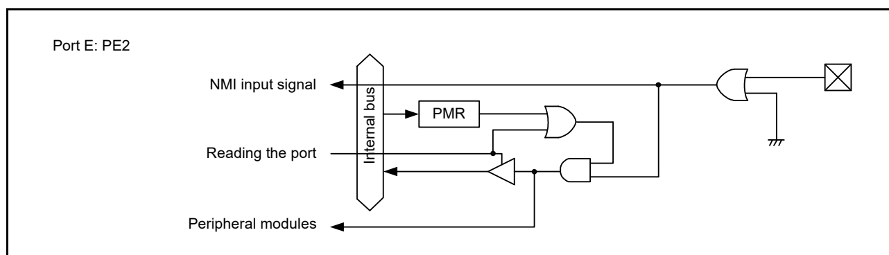
Figure 18.2 I/O Port Configuration (2)
