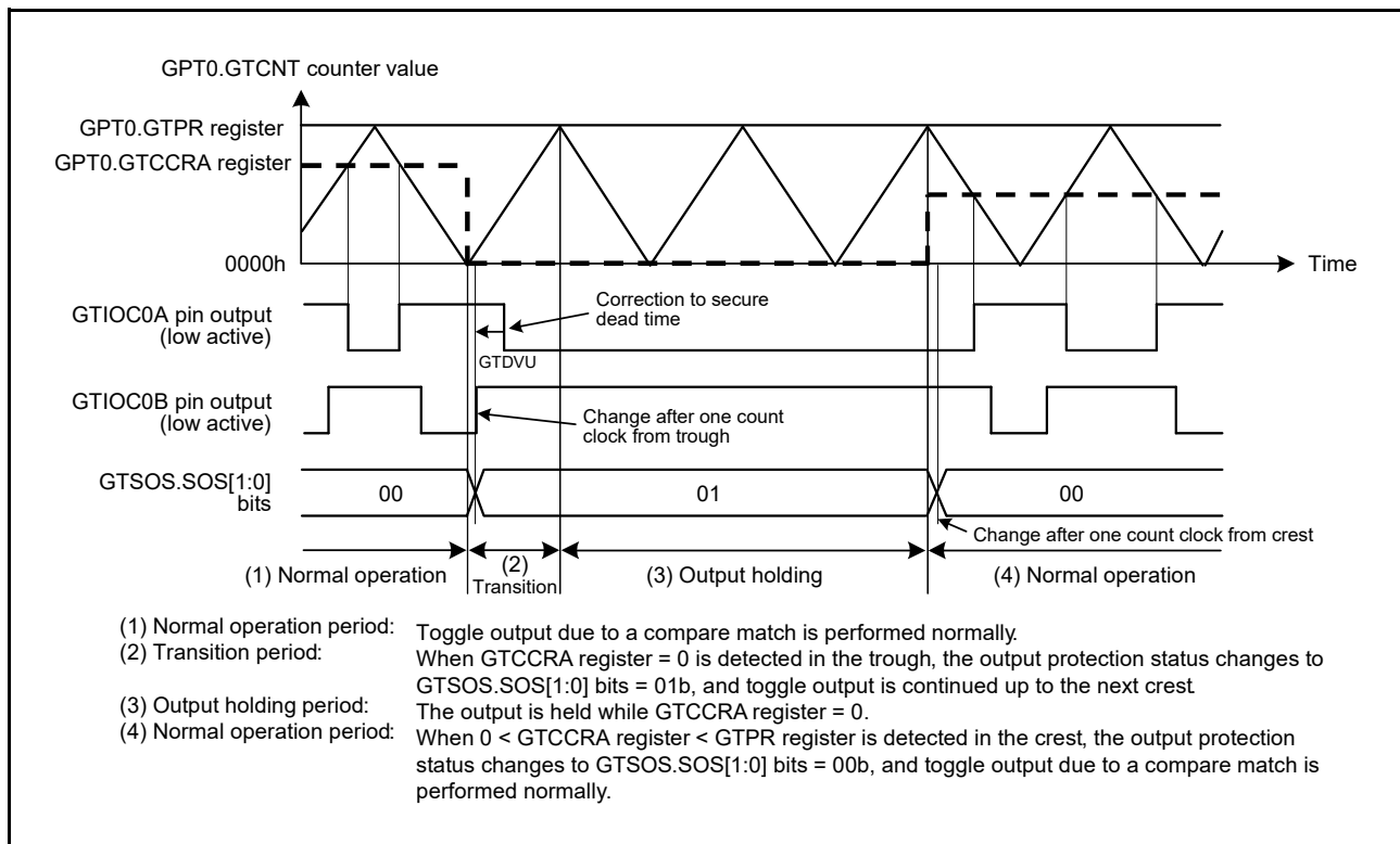
Figure 22.85 Example of Output Protection Function Operation When the GTCCRA Register is Set to 0000h during Buffer Transfer at Troughs (Restored to 0 < \text{GTCCRA} < \text{GTPR} during Buffer Transfer at Crests, Active Level: Low)
