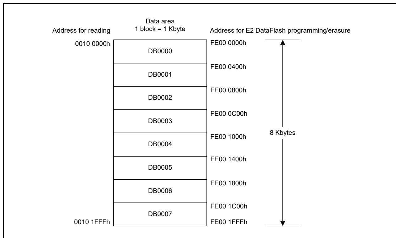
Figure 36.2 E2 DataFlash Area and Block Configuration
