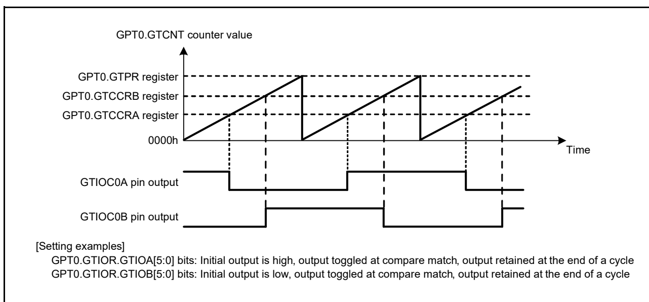
Figure 22.9 Example of Toggled Output Operation (1)
