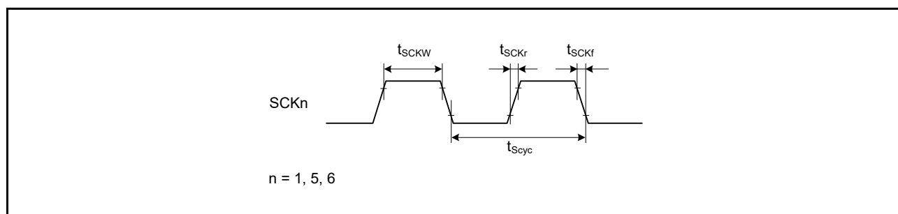
Figure 37.44 SCK Clock Input Timing
