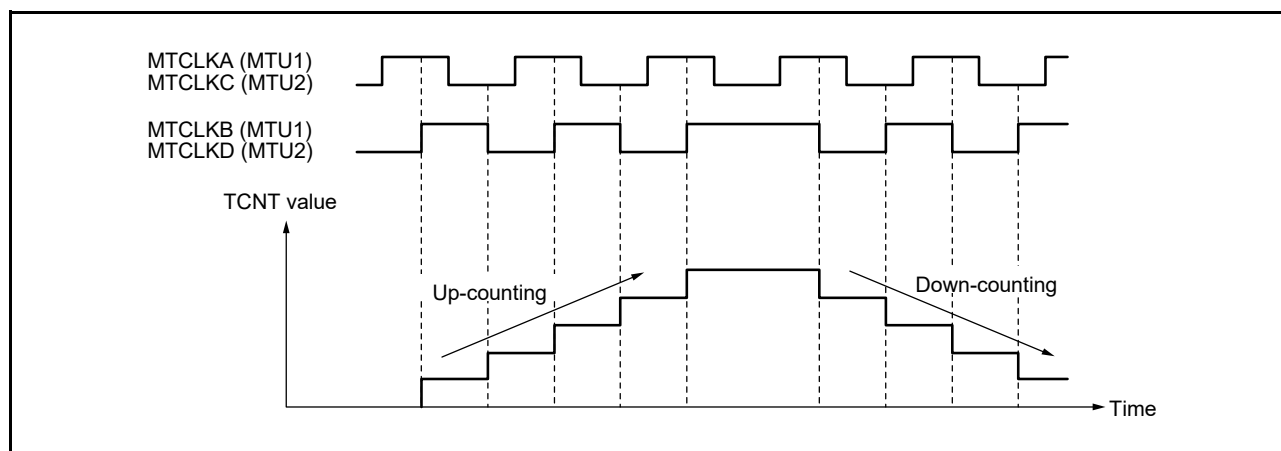
Figure 20.38 Example of Operation in Phase Counting Mode 4
