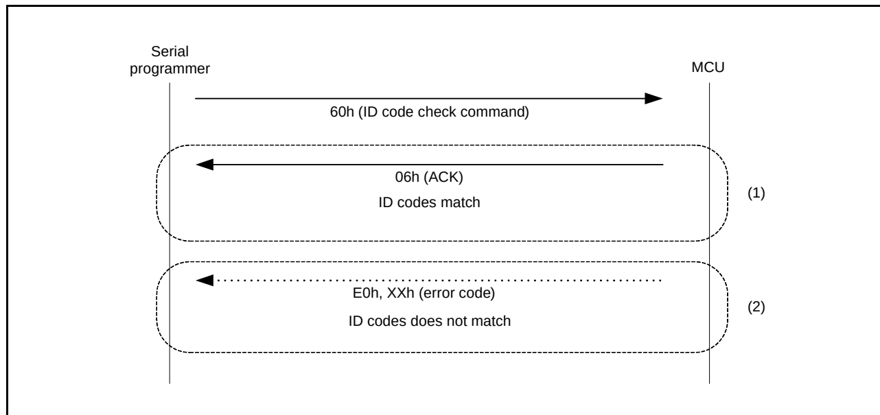
Figure 34.26 Procedure to Unlock ID Code Protection
