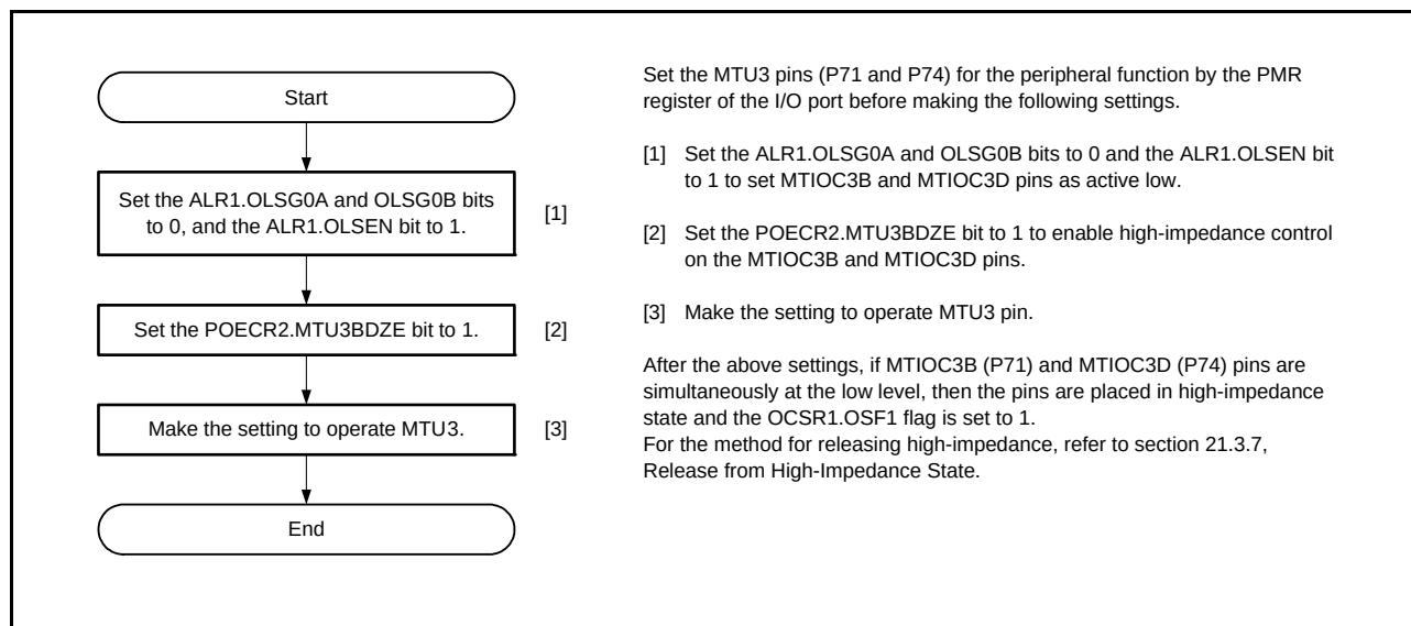
Figure 21.6 Procedure for Setting the POE
