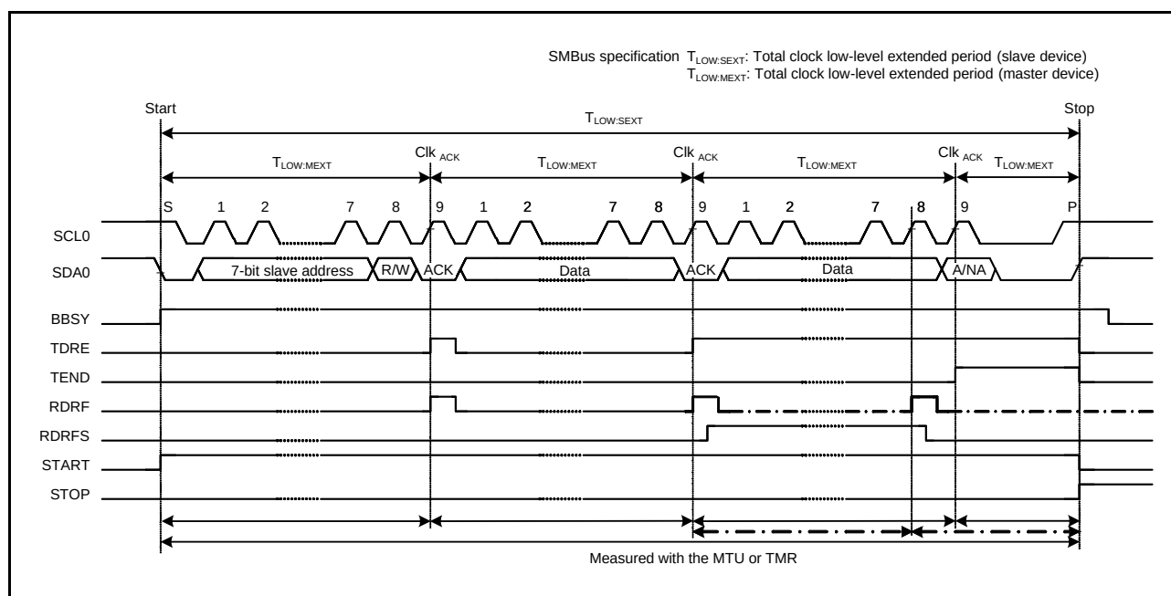
Figure 26.41 SMBus Timeout Measurement
