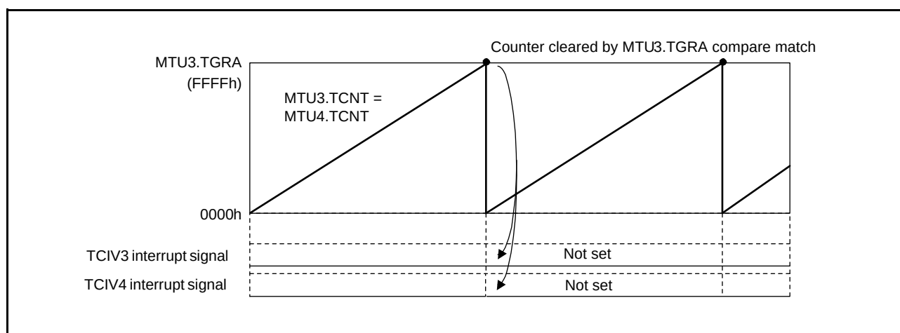
Figure 20.135 Overflow in Reset-Synchronized PWM Mode
