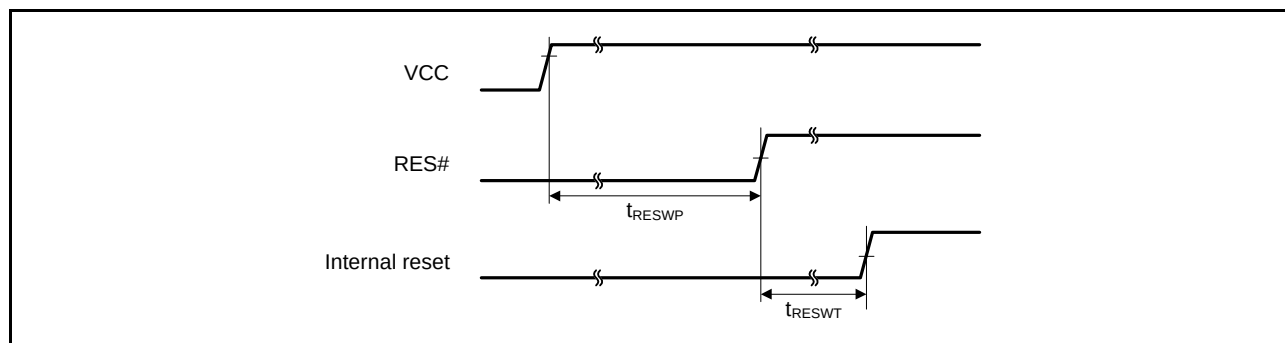
Figure 35.27 Reset Input Timing at Power-On
