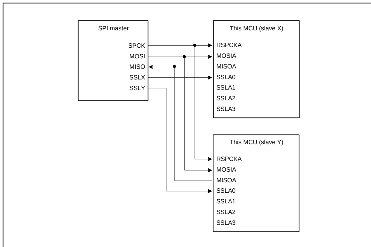
Figure 27.9 Single-Master/Multi-Slave Configuration Example (This MCU = Slave)
