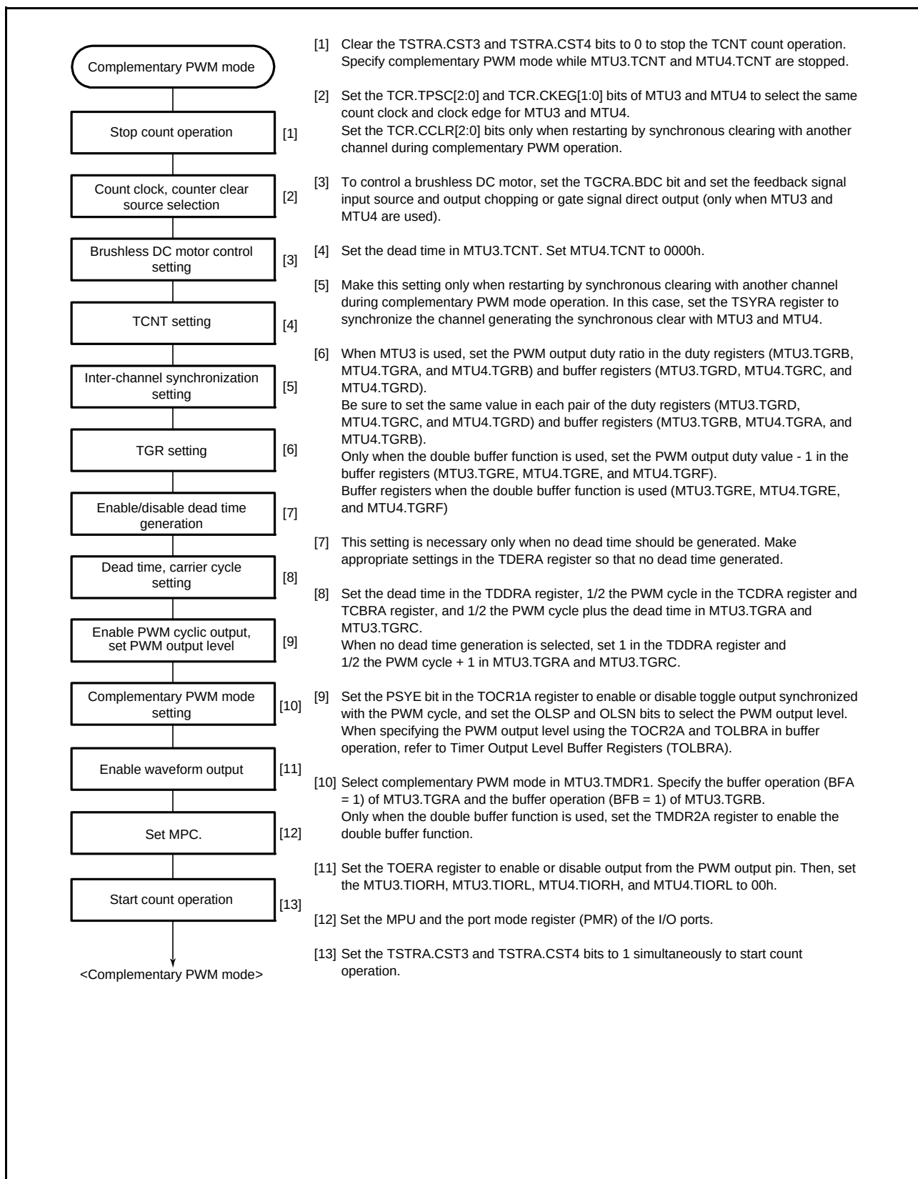
Figure 20.45 Example of Complementary PWM Mode Setting Procedure
