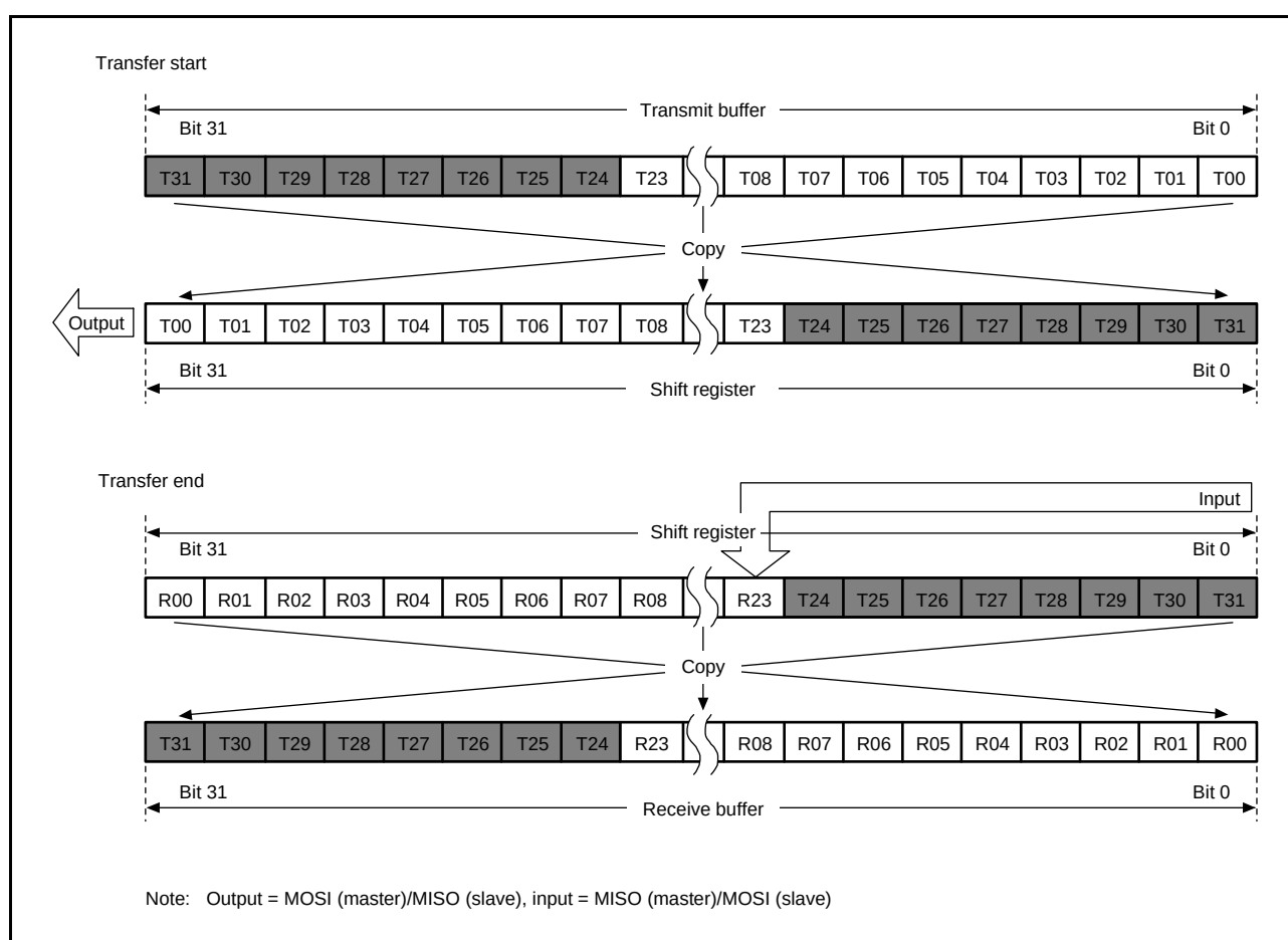
Figure 27.17 LSB First Transfer (24-Bit Data, Parity Disabled)
