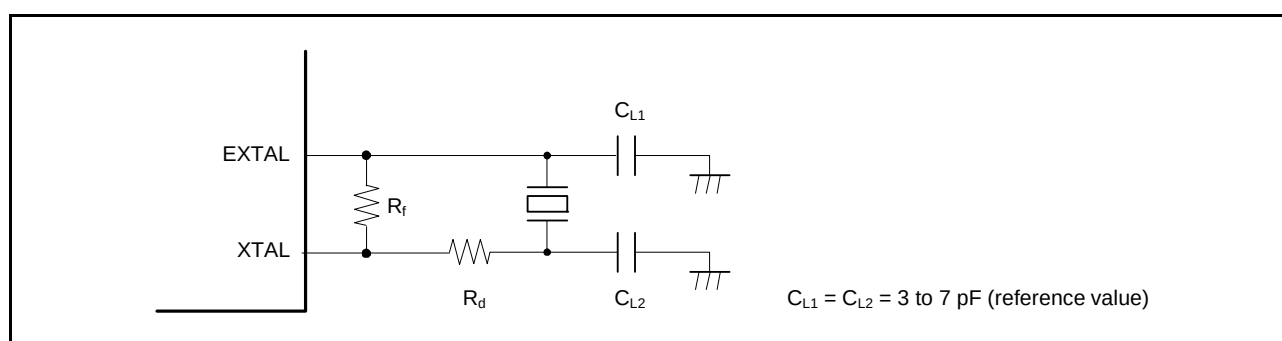
Figure 9.4 Example of Crystal Connection
