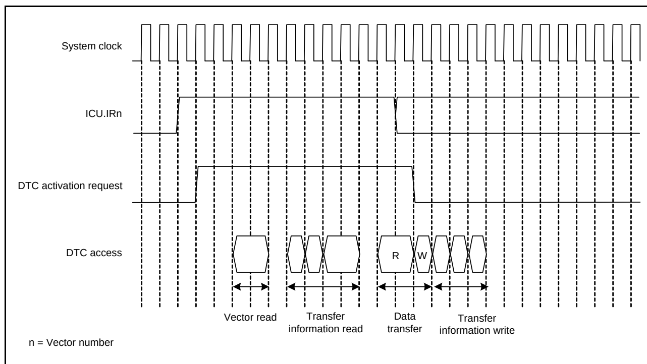
Figure 17.9 Example (1) of DTC Operation Timing (Short-Address Mode, Normal Transfer Mode, Repeat Transfer Mode)
