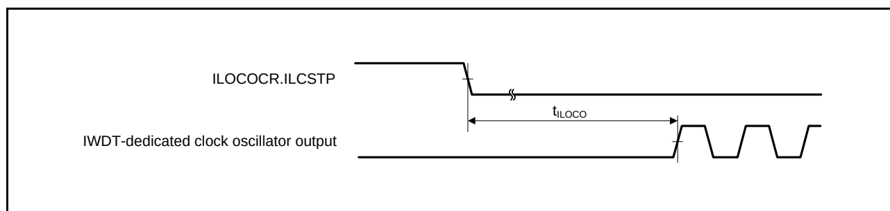
Figure 35.23 IWDt-Dedicated Clock Oscillation Start Timing
