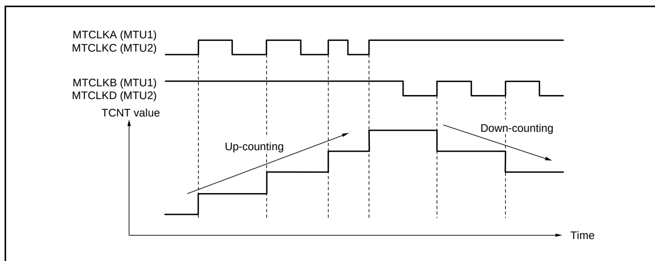
Figure 20.35 Example of Operation in Phase Counting Mode 3 (When MTUn.TCR2.PCB[1:0] = 01b ( n = 1, 2 ))
