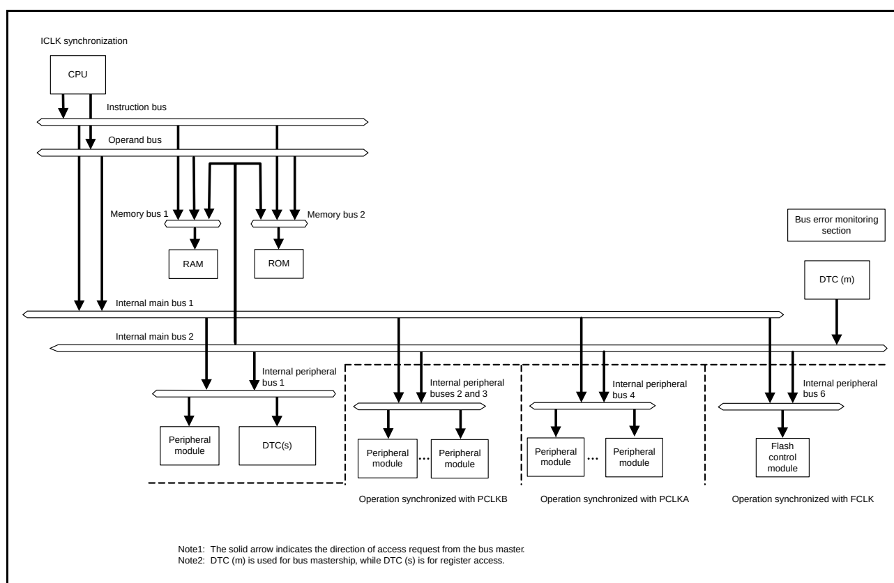
Figure 15.1 Bus Configuration
