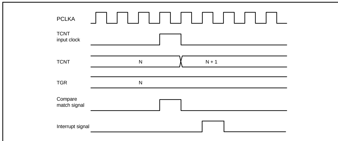
Figure 20.116 TGI Interrupt Timing (Compare Match) (MTU0 to MTU4)
