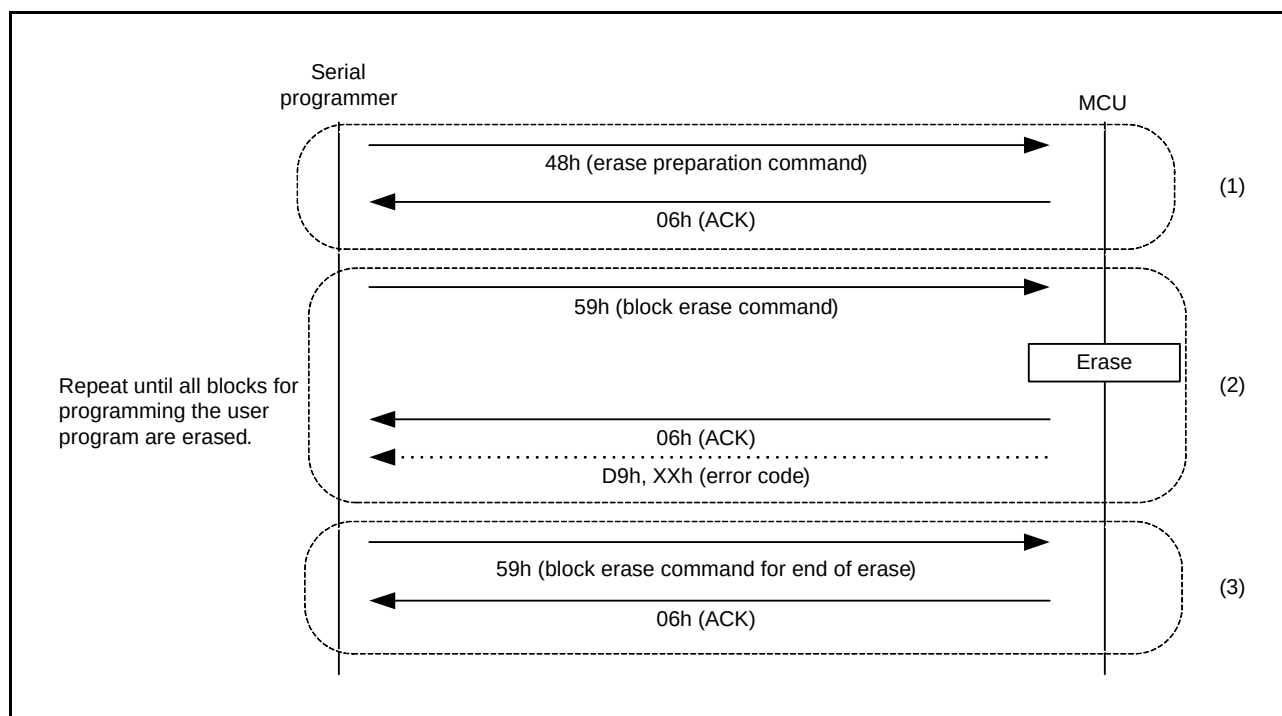
Figure 34.27 Procedure to Erase the User Area
