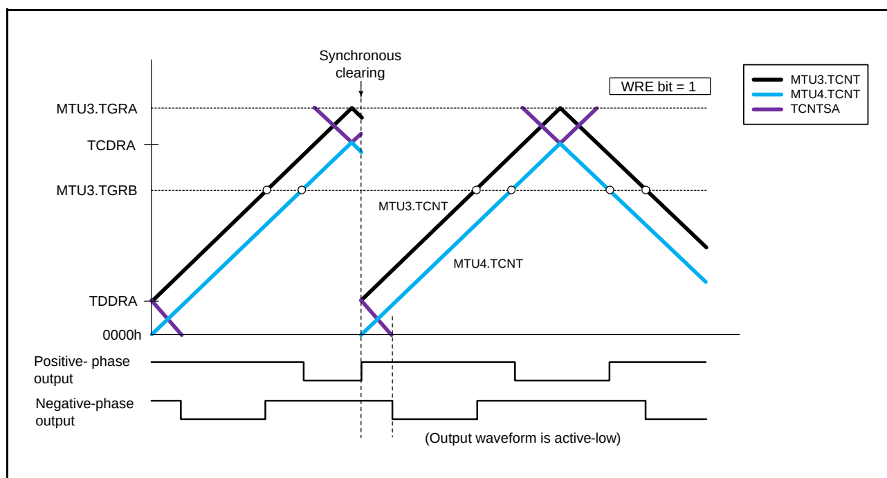
Figure 20.66 Example of Synchronous Clearing in Tb1 interval (Timing (6) in Figure 20.63; TWCRA.WRE Bit is 1)
