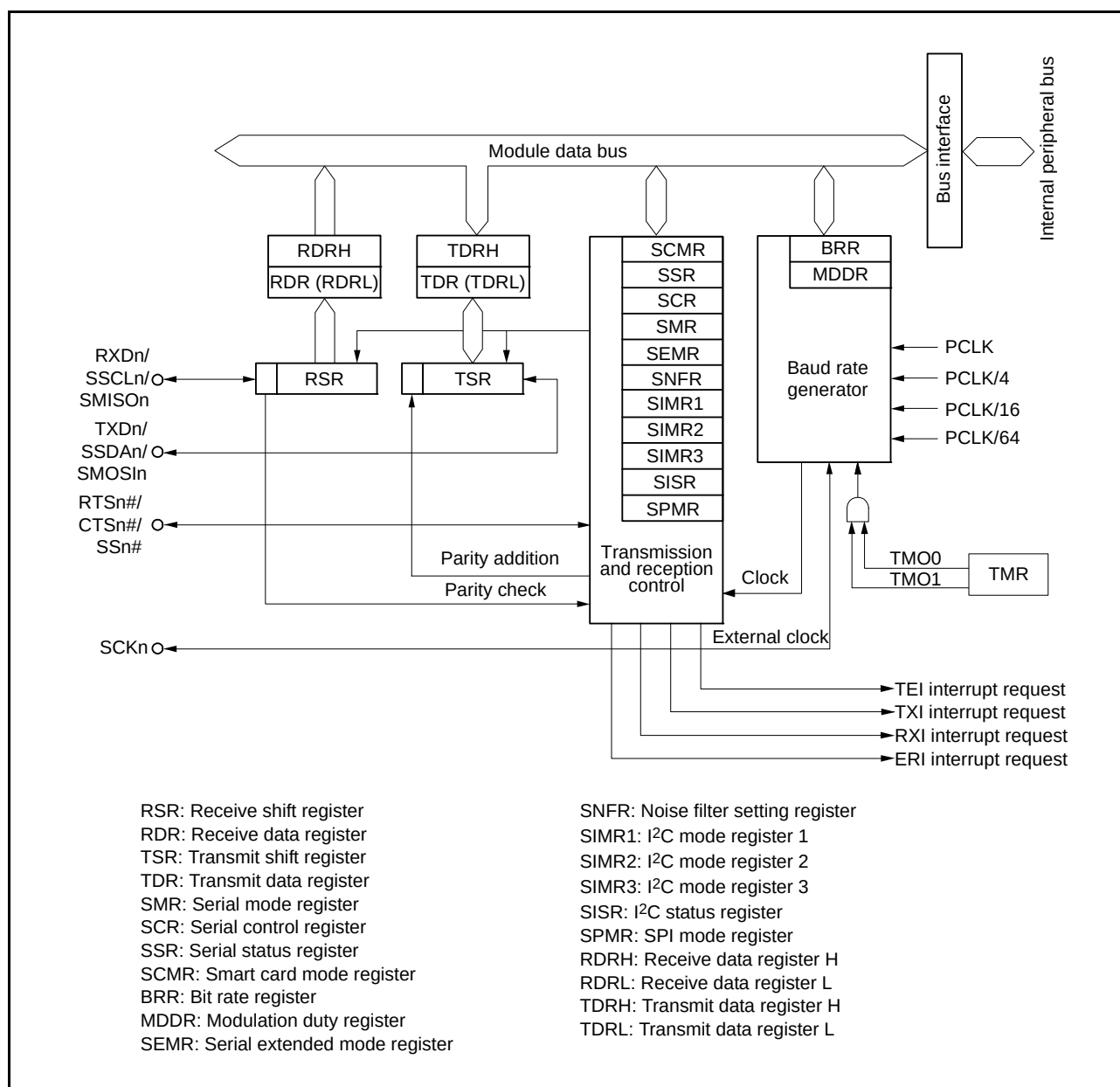
Figure 25.2 Block Diagram of SCIg (SCI5)
