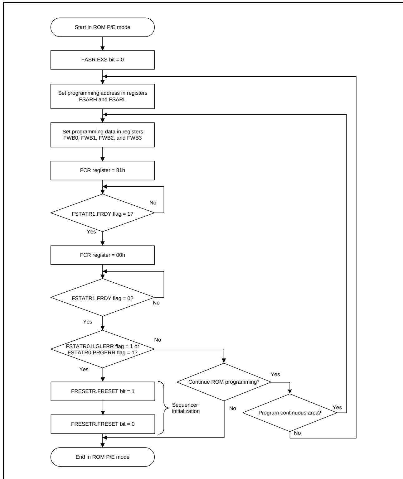
Figure 34.8 Procedure to Issue the Program Command
