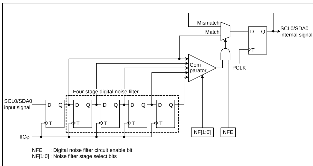
Figure 26.23 Block Diagram of Digital Noise Filter Circuit
