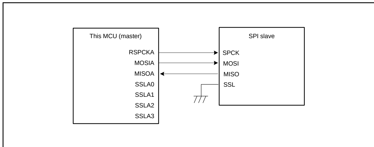
Figure 27.5 Single-Master/Single-Slave Configuration Example (This MCU = Master)
