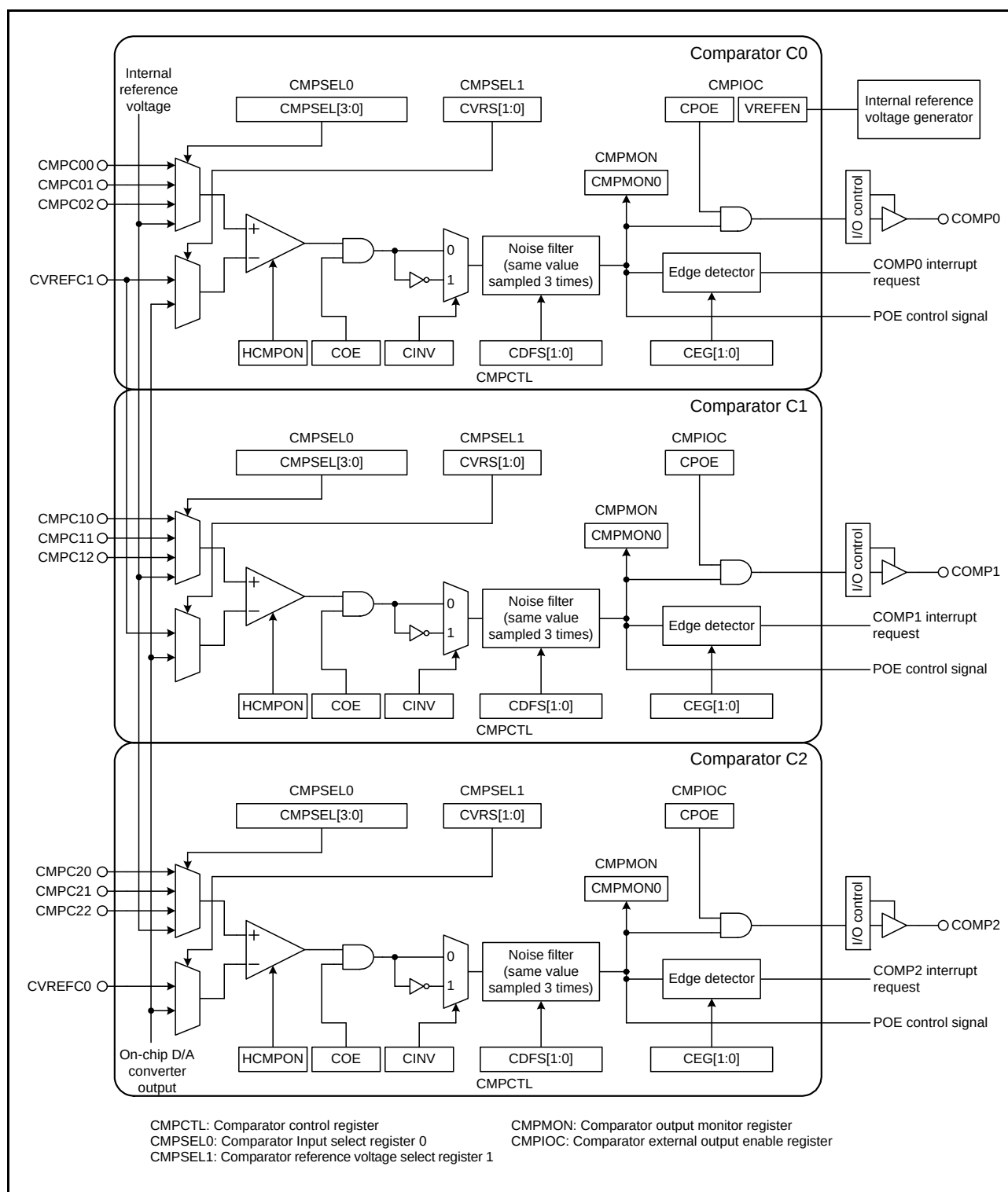
Figure 31.1 Comparator C Block Diagram
