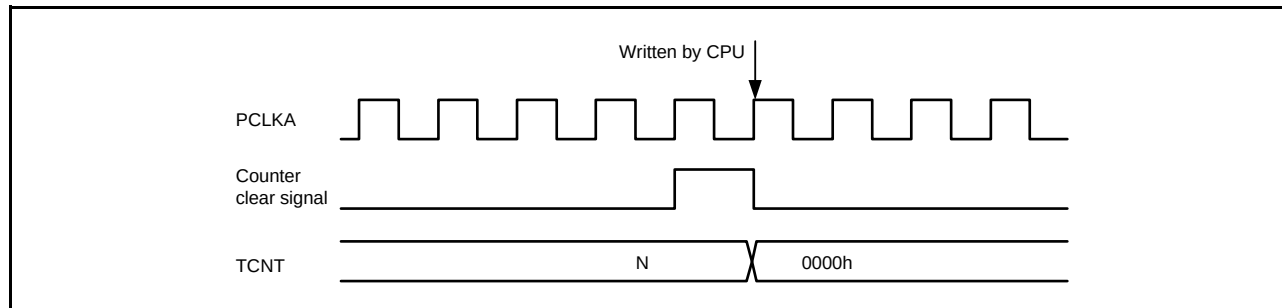
Figure 20.123 Contention between TCNT Write and Clear Operations
