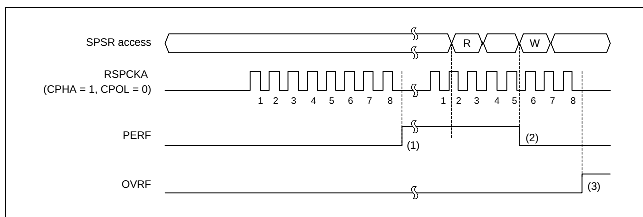
Figure 27.30 Operation Example of PERF Flag
