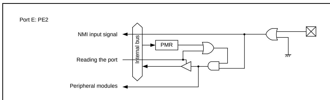
Figure 18.2 I/O Port Configuration (2)
