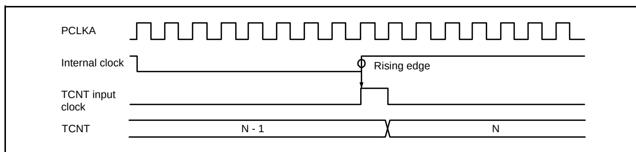
Figure 20.101 Count Timing in Internal Clock Operation (MTU5)
