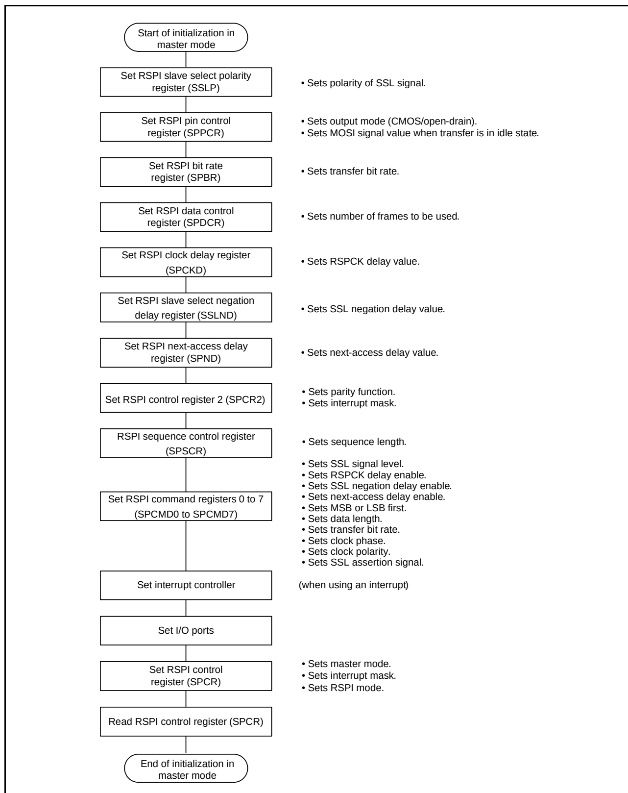
Figure 27.35 Example of Initialization Flowchart in Master Mode (SPI Operation)
