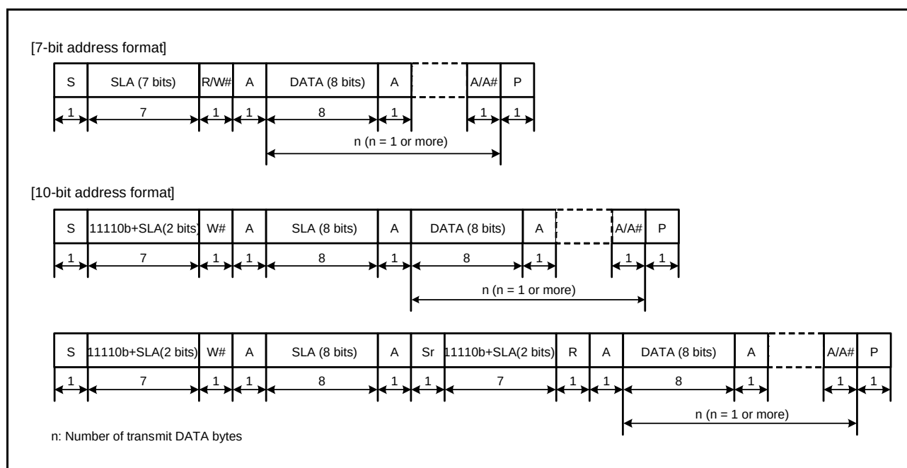
Figure 26.3 I 2 C-bus Format
