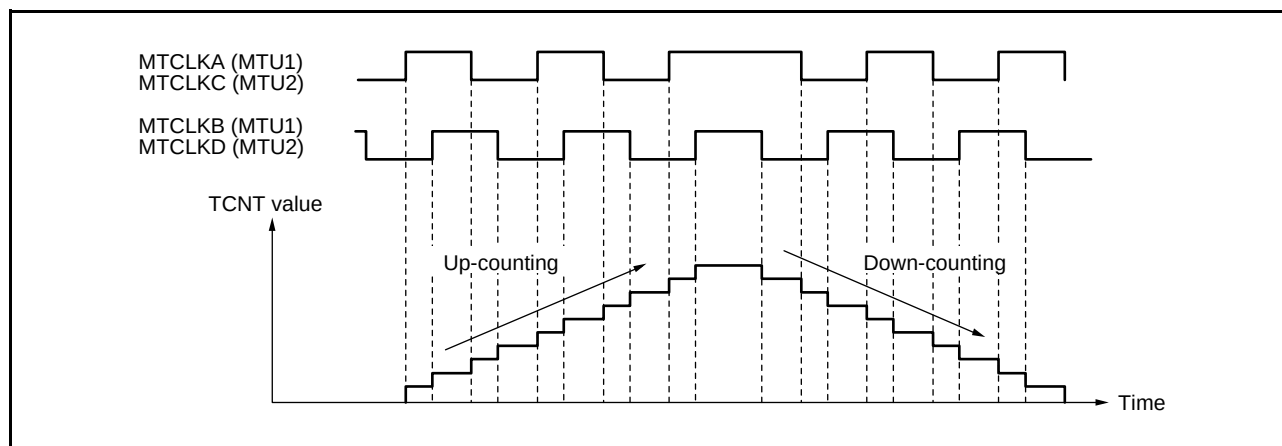
Figure 20.30 Example of Operation in Phase Counting Mode 1
