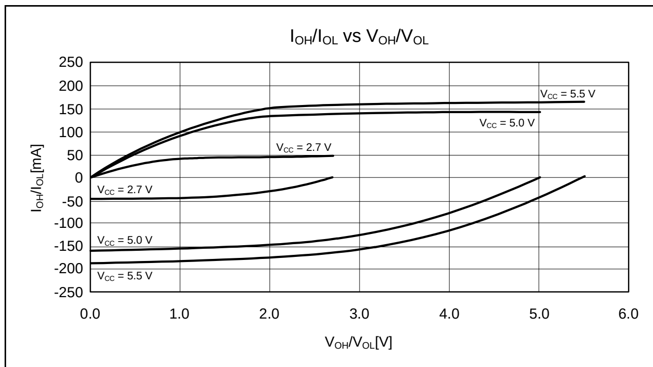
Figure 35.12 V_{OH}/V_{OL} and I_{OH}/I_{OL} Voltage Characteristics of Large Current Ports (Ports 71 to 76, Port B5, Port D3) at T_a = 25^\circ\text{C} (Reference Data)
