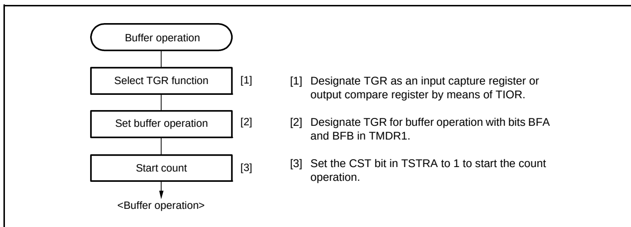
Figure 20.16 Example of Buffer Operation Setting Procedure
