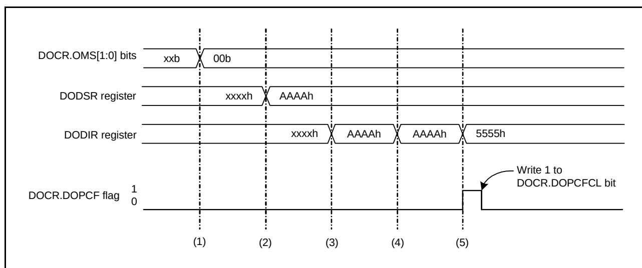
Figure 32.2 Example of Operation in Data Comparison Mode
