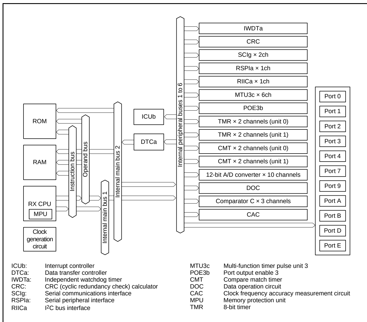
Figure 1.2 Block Diagram
