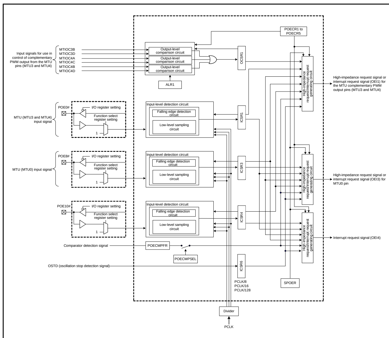
Figure 21.1 POE Block Diagram
