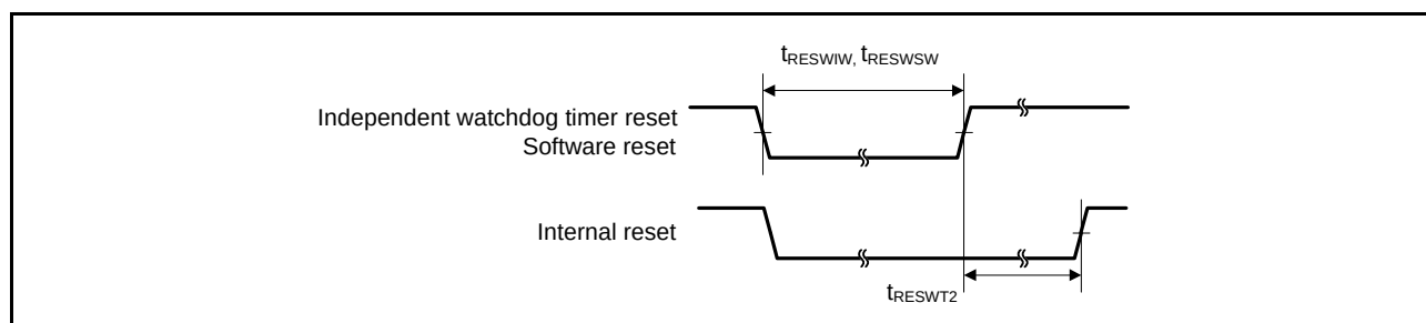
Figure 35.29 Reset Input Timing (2)
