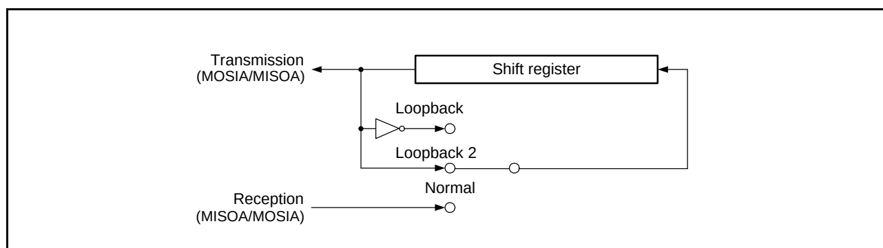
Figure 27.48 Configuration of Shift Register I/O Paths in Loopback Mode (Master Mode)
