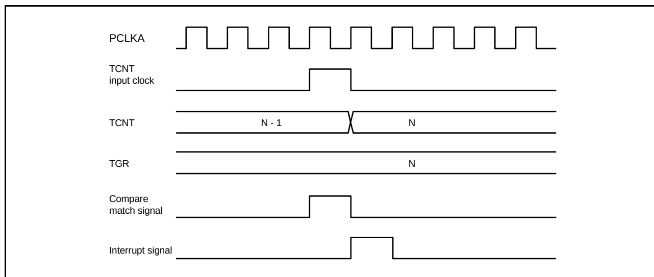
Figure 20.117 TGI Interrupt Timing (Compare Match) (MTU5)
