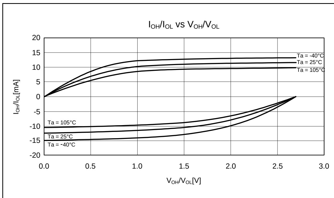
Figure 35.5 V_{OH}/V_{OL} and I_{OH}/I_{OL} Temperature Characteristics at V_{CC} = 2.7 V when Normal Output is Selected (Reference Data)
