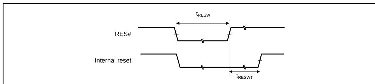
Figure 35.28 Reset Input Timing (1)
