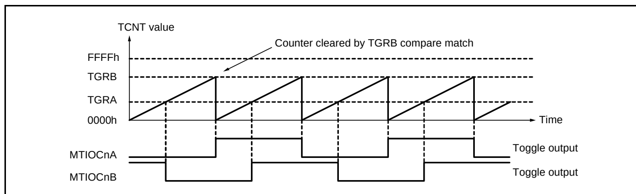
Figure 20.9 Example of Toggle Output Operation (n = 0 to 4)
