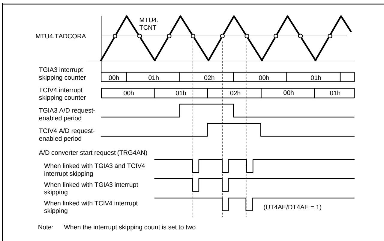
Figure 20.86 Example of A/D Converter Start Request Signal (TRG4AN) Operation Linked with Interrupt Skipping Function 1 (UT4AE and DT4AE = 1)
