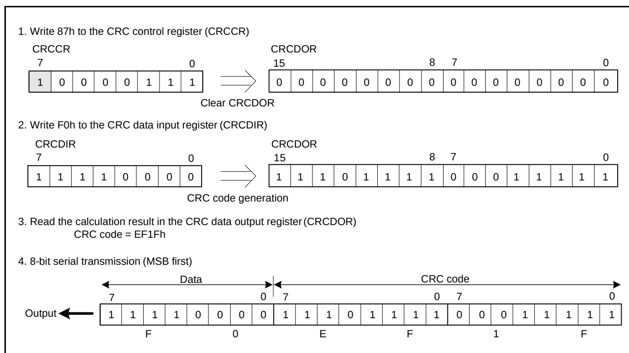
Figure 28.3 MSB First Data Transmission
