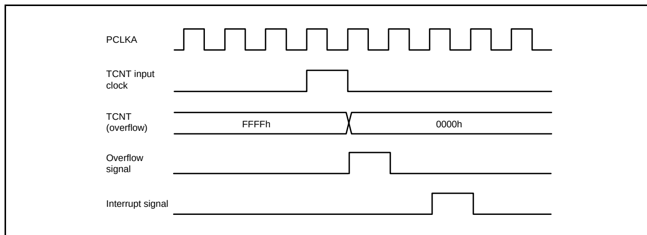
Figure 20.120 TCIV Interrupt Timing
