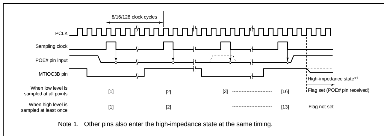
Figure 21.4 Low-Level Detection Operation
