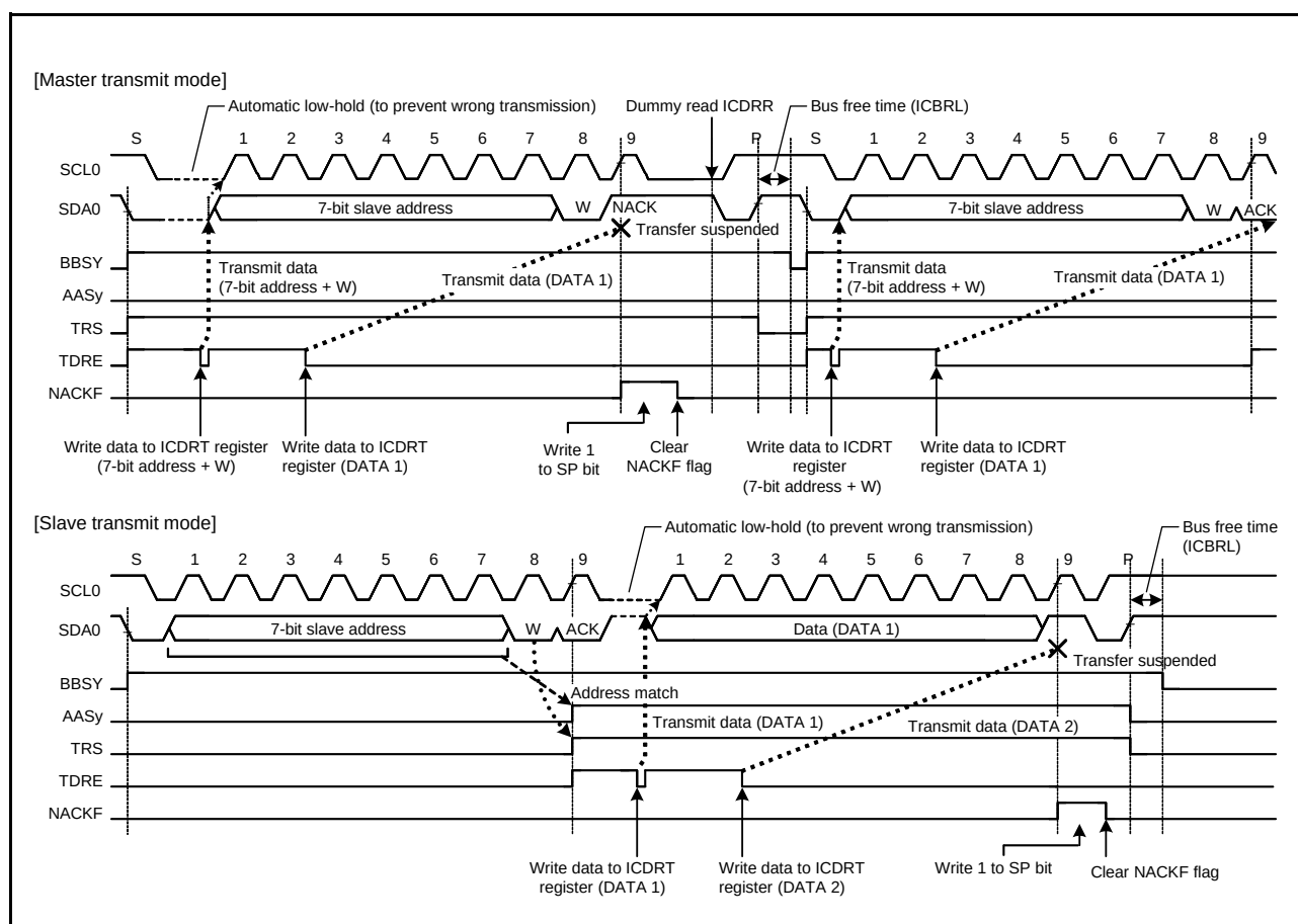
Figure 26.31 Suspension of Data Transfer When NACK is Received (NACKF = 1)
