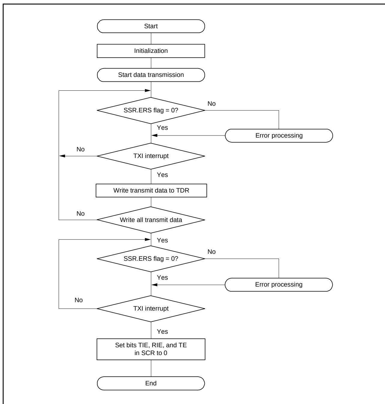
Figure 25.39 Sample Smart Card Interface Transmission Flowchart
