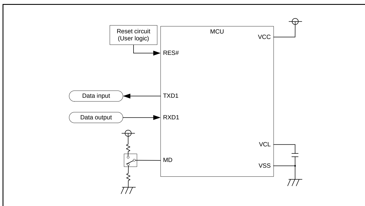
Figure 34.14 Example of Pin Connections in Boot Mode (SCI)
