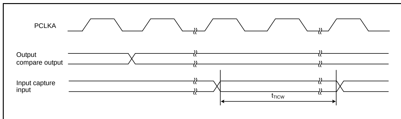
Figure 35.35 MTU3 Input/Output Timing
