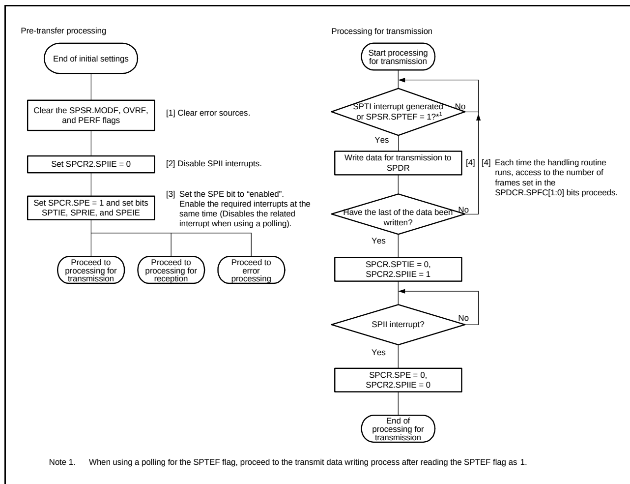
Figure 27.36 Flowchart in Master Mode (Transmission)
