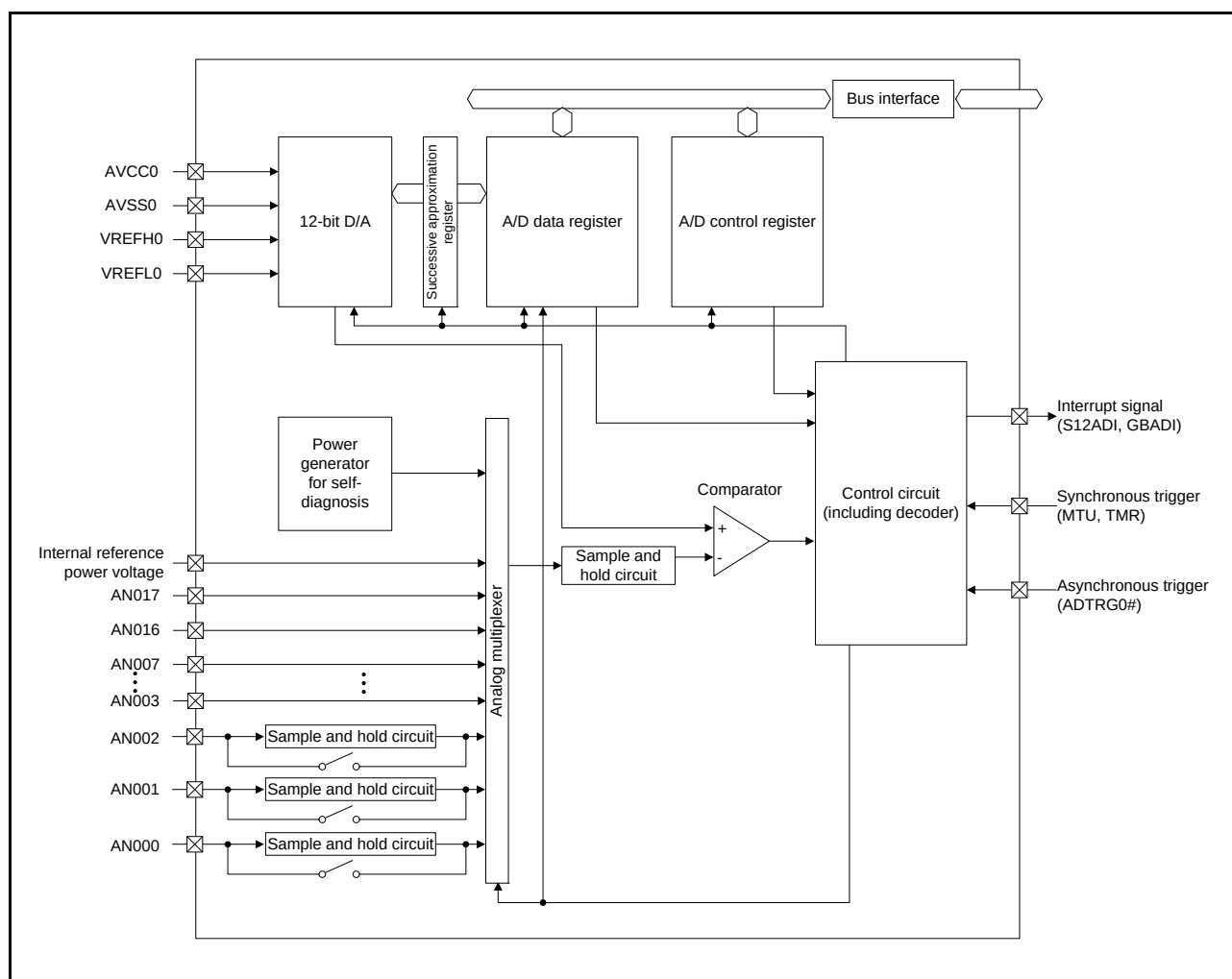
Figure 29.1 Block Diagram of 12-Bit A/D Converter
