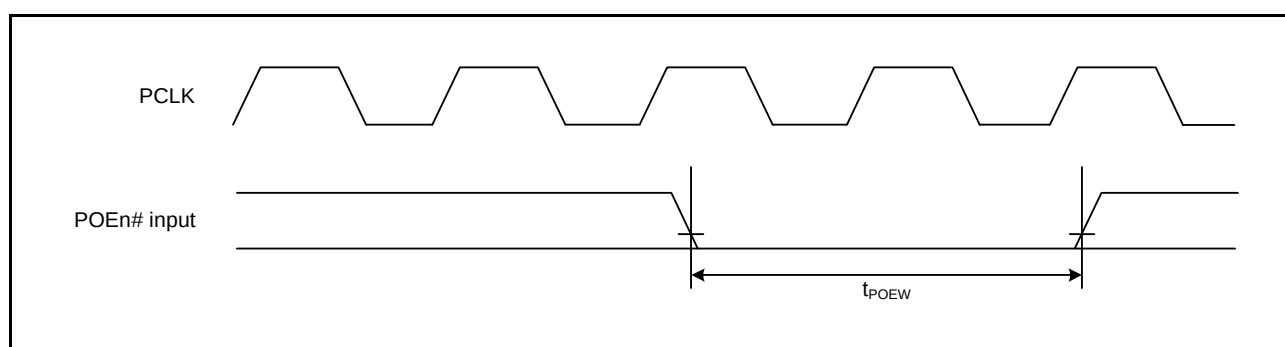
Figure 35.37 POE# Input Timing
