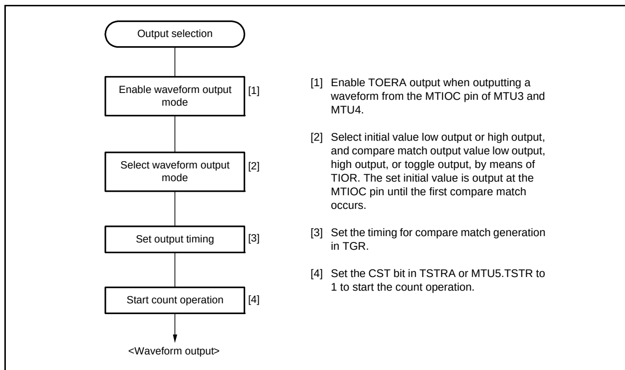
Figure 20.7 Example of Procedure for Setting Waveform Output by Compare Match
