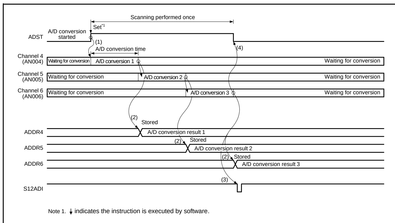
Figure 29.3 Example of Operation in Single Scan Mode (Basic Operation: AN004, AN005, AN006 Selected)
