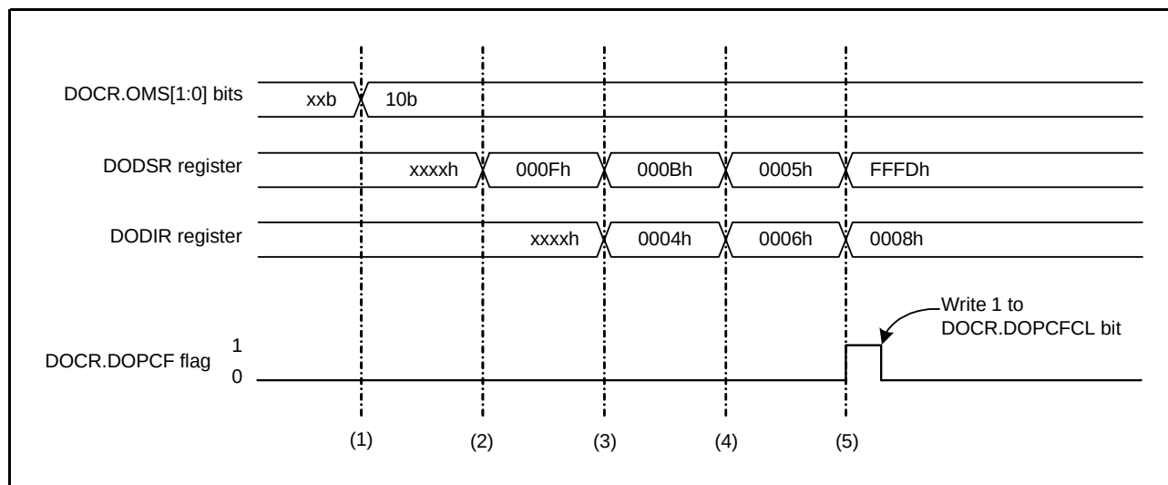
Figure 32.4 Example of Operation in Data Subtraction Mode
