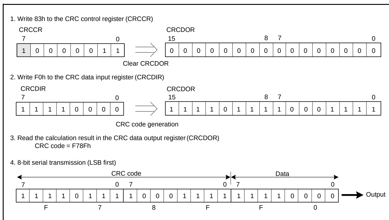
Figure 28.2 LSB First Data Transmission
