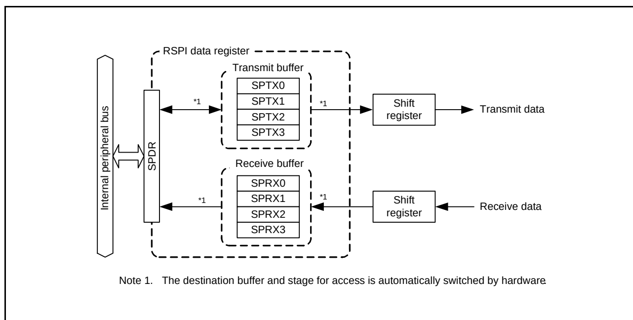
Figure 27.2 Configuration of SPDR
