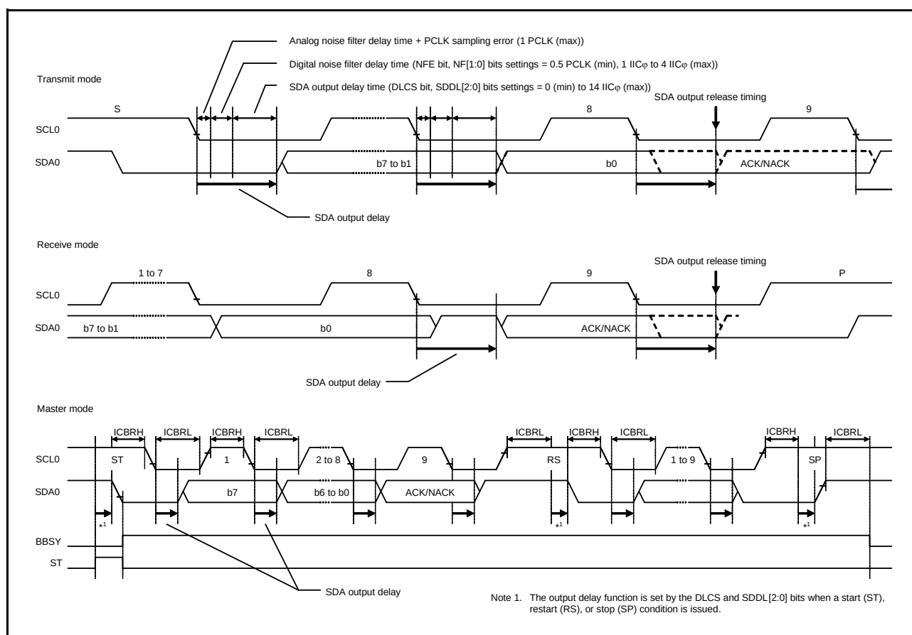
Figure 26.22 SDA Output Delay Function
