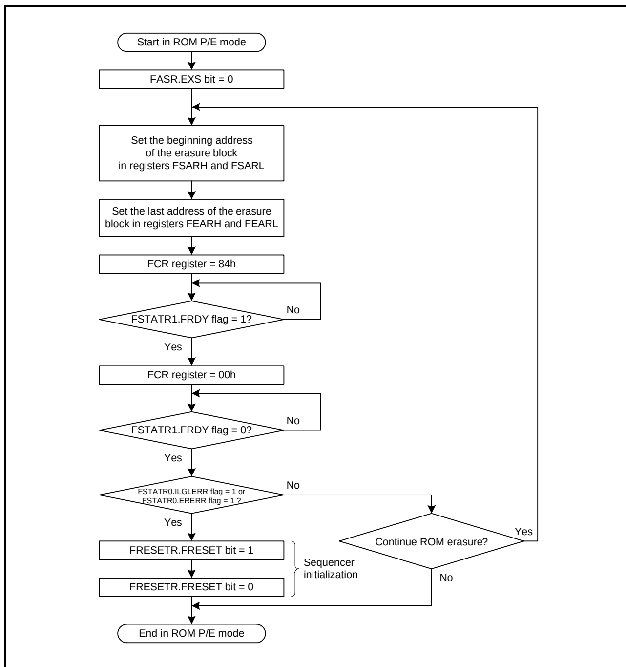
Figure 34.9 Procedure to Issue the Block Erase Command
