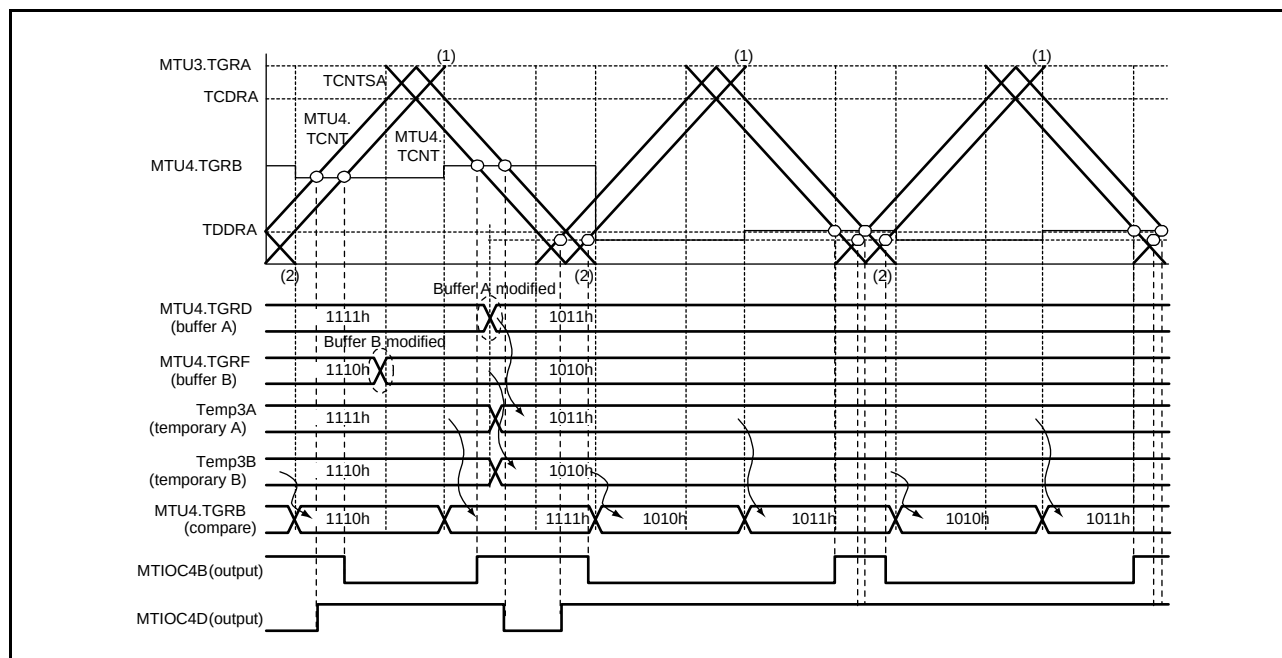
Figure 20.75 Example of Double Buffer Operation (Buffer Write Value is Smaller than TDDRA)
