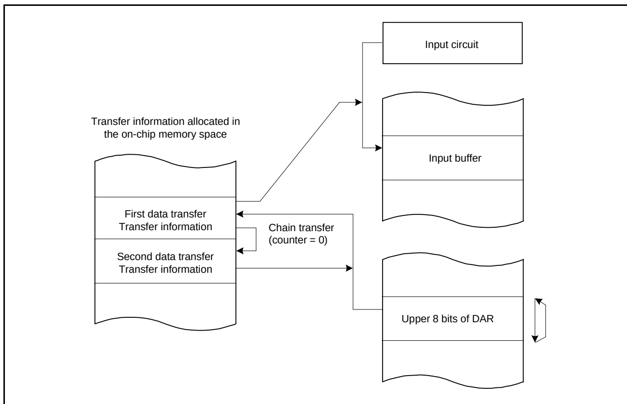
Figure 17.15 Chain Transfer When the Counter = 0
