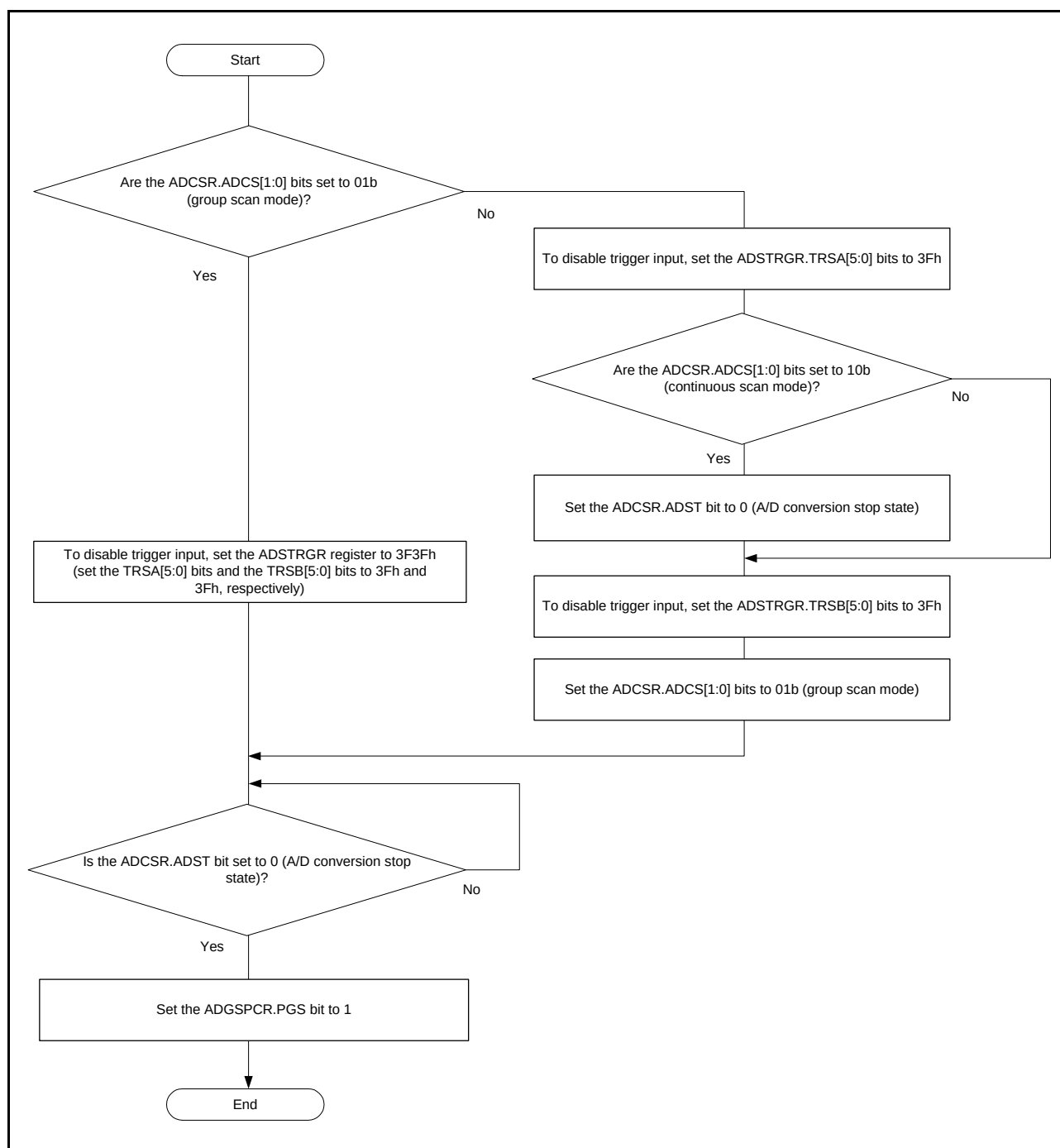
Figure 29.14 Flow of Setting the ADGSPCR.PGS Bit
