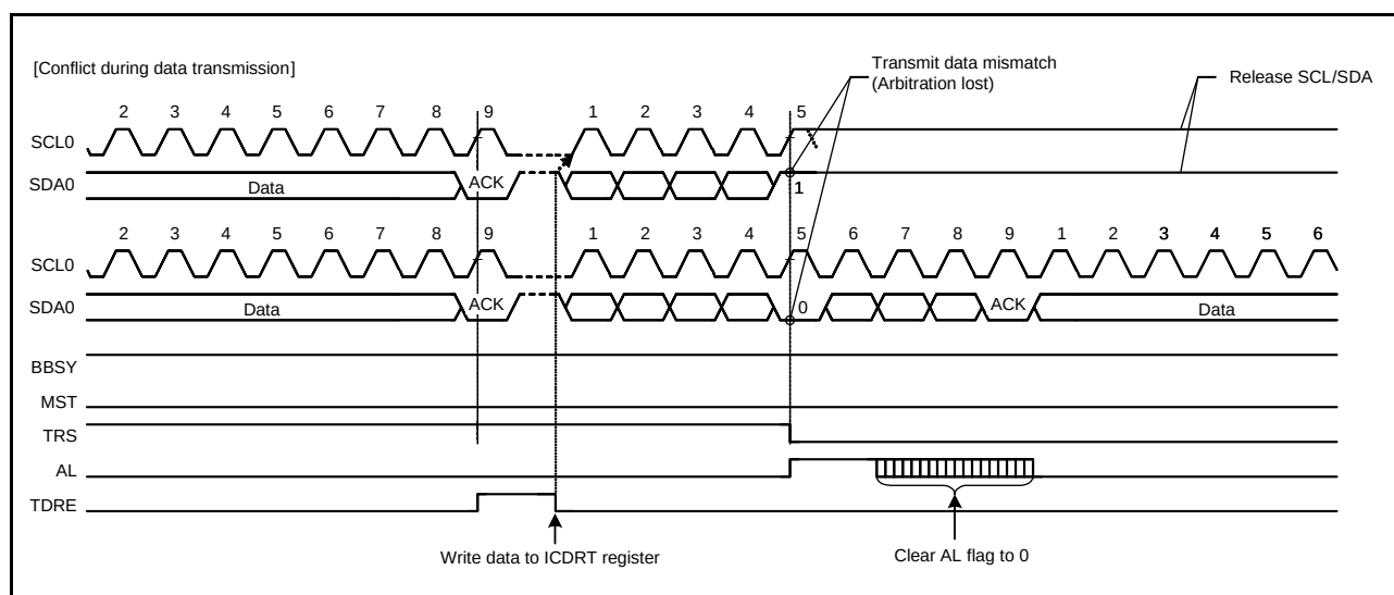
Figure 26.36 Example of Slave Arbitration-Lost Detection (SALE = 1)
