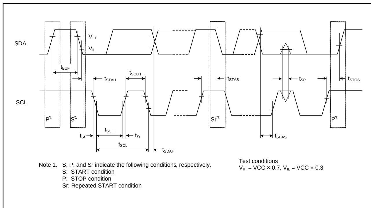
Figure 35.47 IIC Bus Interface Input/Output Timing and Simple I 2 C Bus Interface Input/Output Timing
