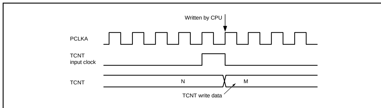
Figure 20.124 Contention between TCNT Write and Increment Operations
