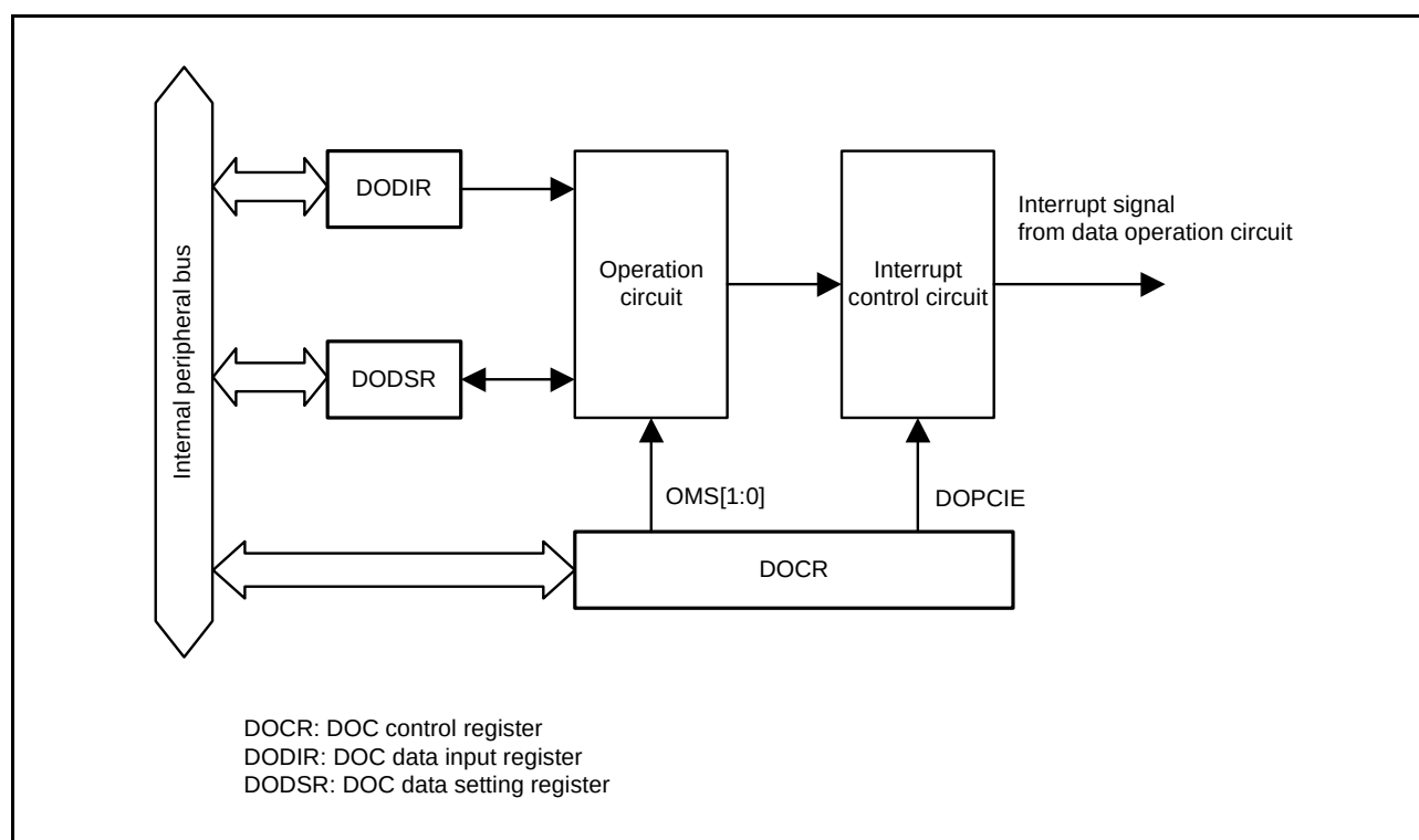
Figure 32.1 DOC Block Diagram
