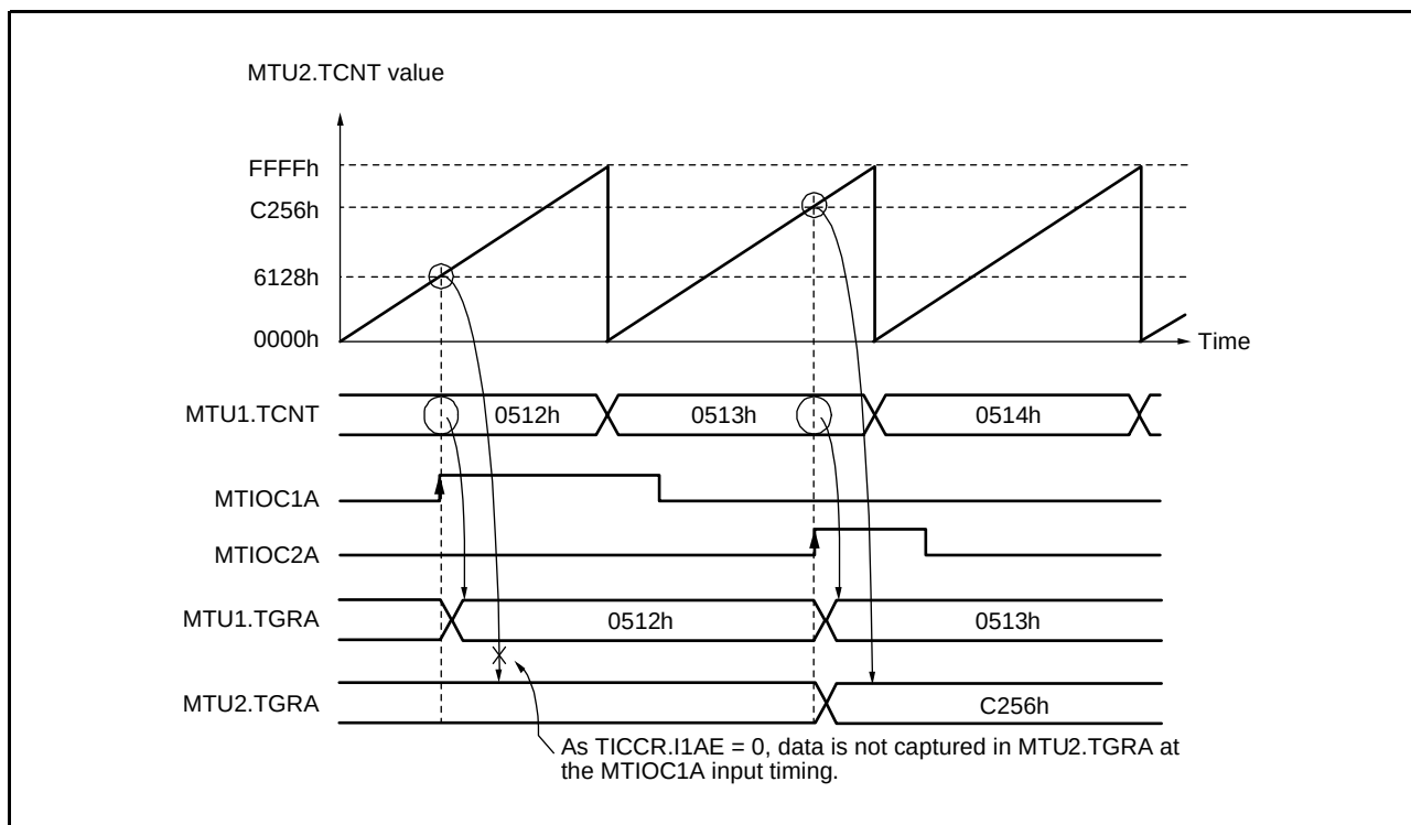
Figure 20.22 Cascaded Operation Example (b)
