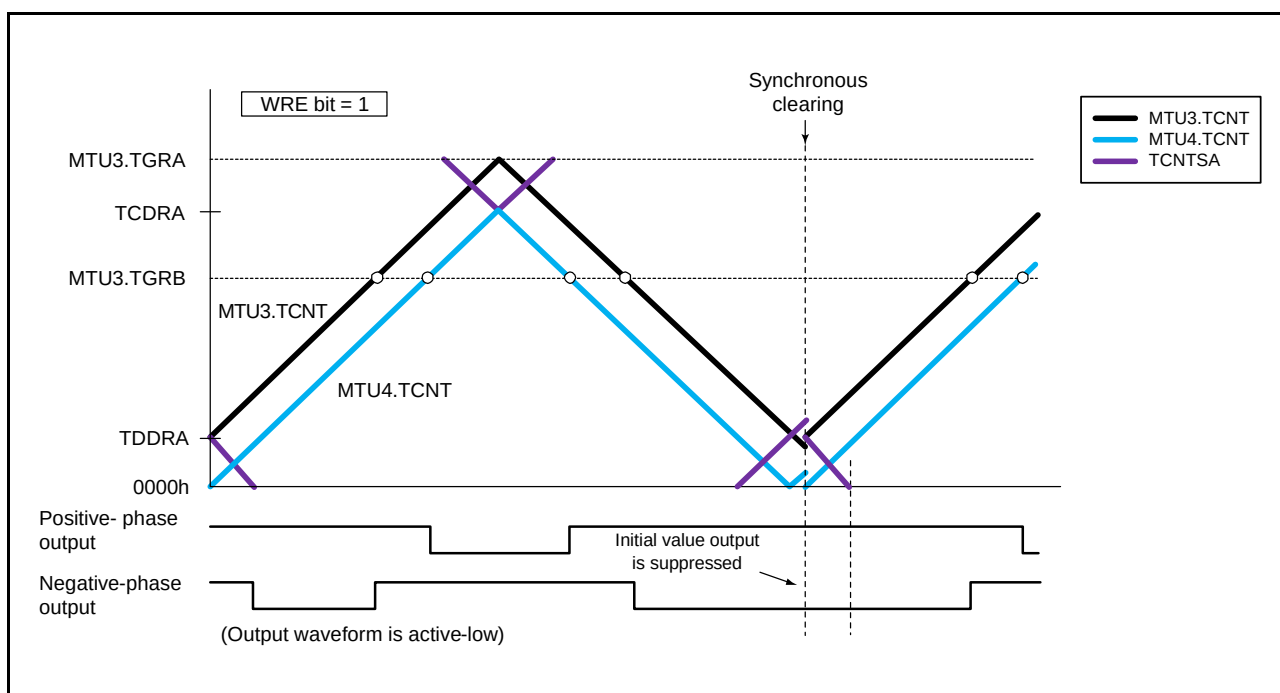
Figure 20.68 Example of Synchronous Clearing in Tb2 interval (Timing (11) in Figure 20.63; TWCRA.WRE Bit is 1)
