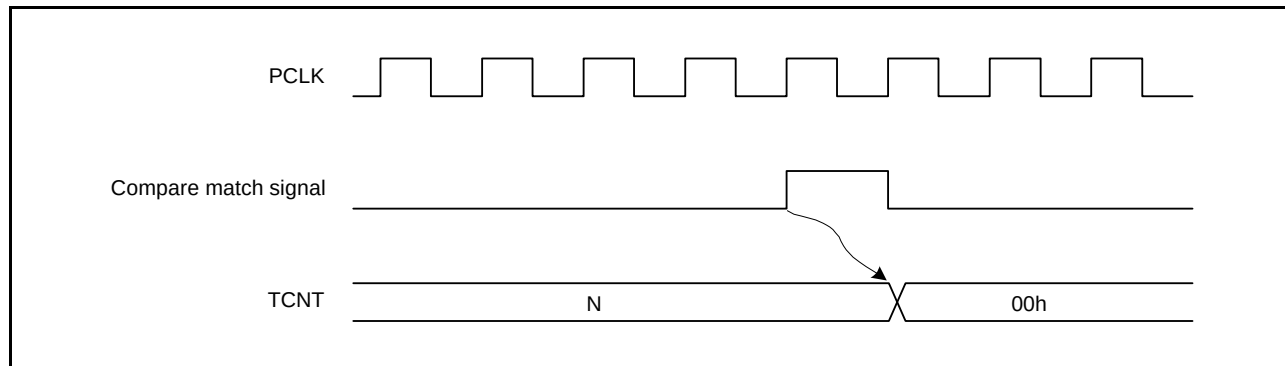
Figure 22.9 Timing of Counter Clear by Compare Match
