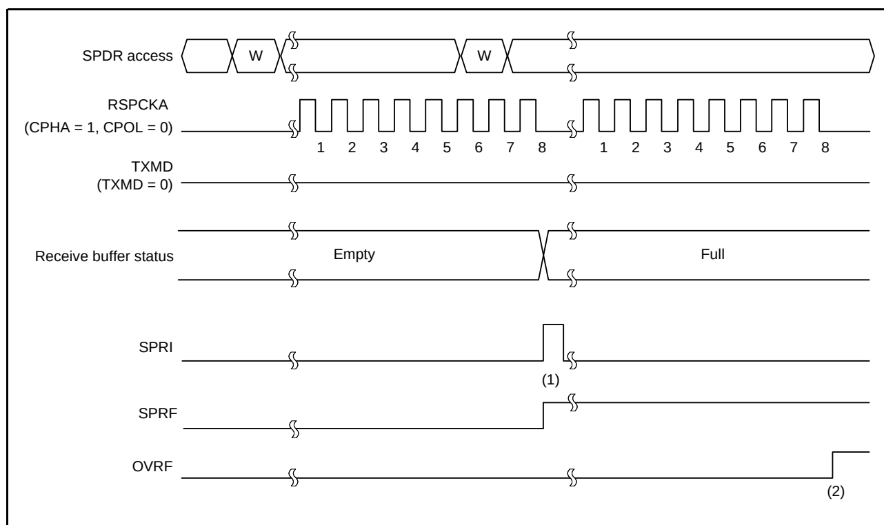
Figure 27.24 Operation Example of SPCR.TXMD = 0
