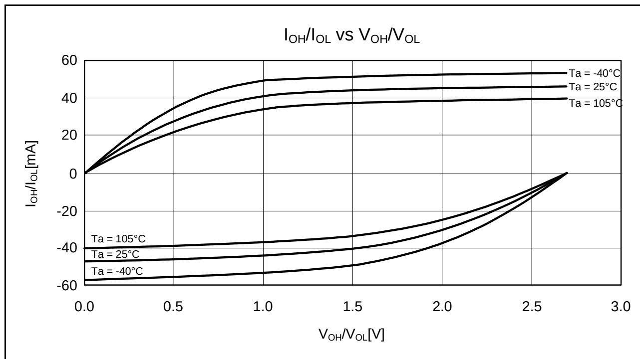
Figure 35.13 V_{OH}/V_{OL} and I_{OH}/I_{OL} Temperature Characteristics of Large Current Ports (Ports 71 to 76, Port B5, Port D3) at V_{CC} = 2.7\text{ V} (Reference Data)
