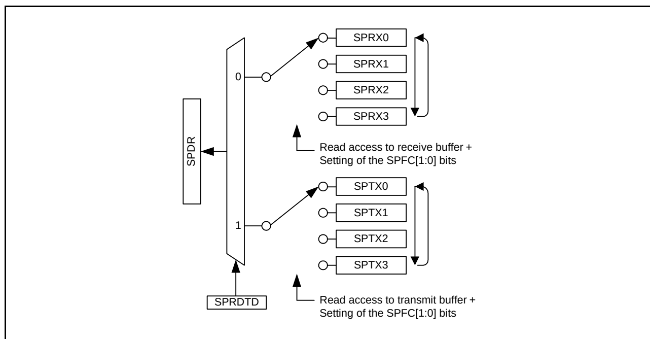
Figure 27.4 Configuration of SPDR (Reading)
