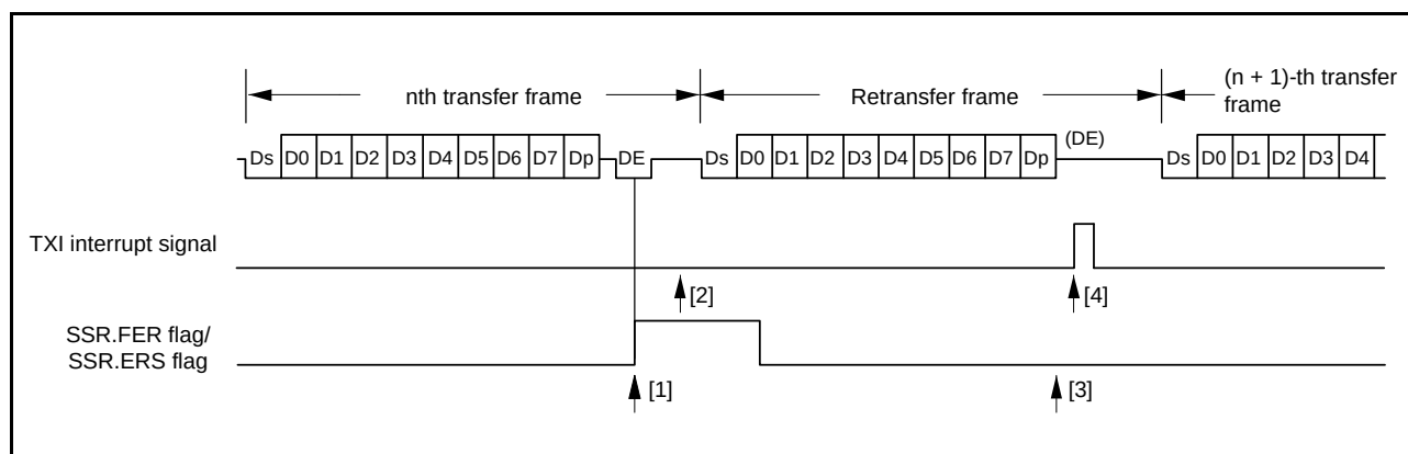
Figure 25.37 Data Retransfer Operation in SCI Transmission Mode
