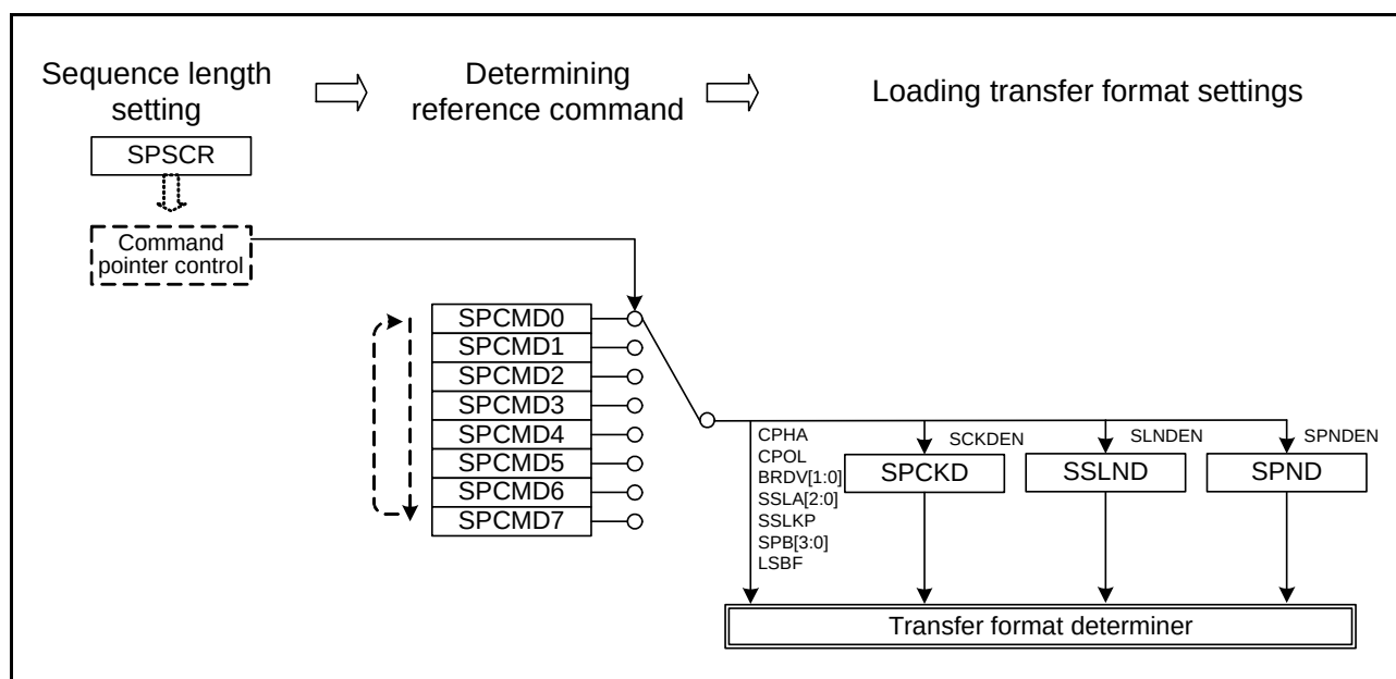
Figure 27.43 Procedure for Determining the Form of Serial Transmission in Master Mode
