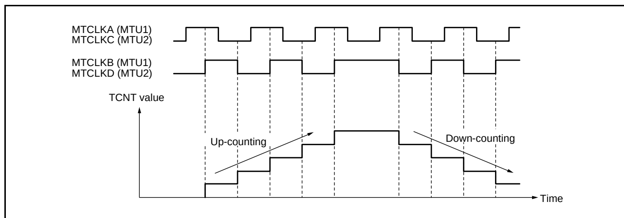
Figure 20.37 Example of Operation in Phase Counting Mode 4
