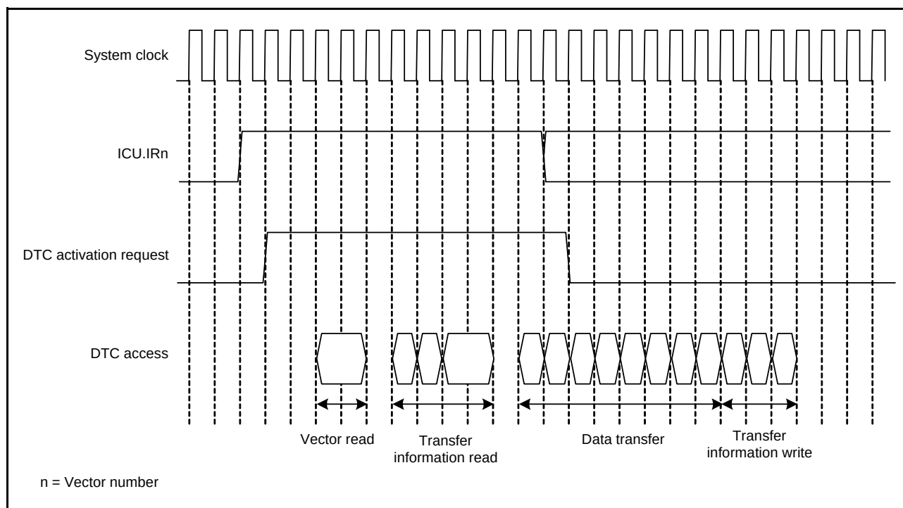
Figure 17.10 Example (2) of DTC Operation Timing (Short-Address Mode, Block Transfer Mode, Block Size = 4)
