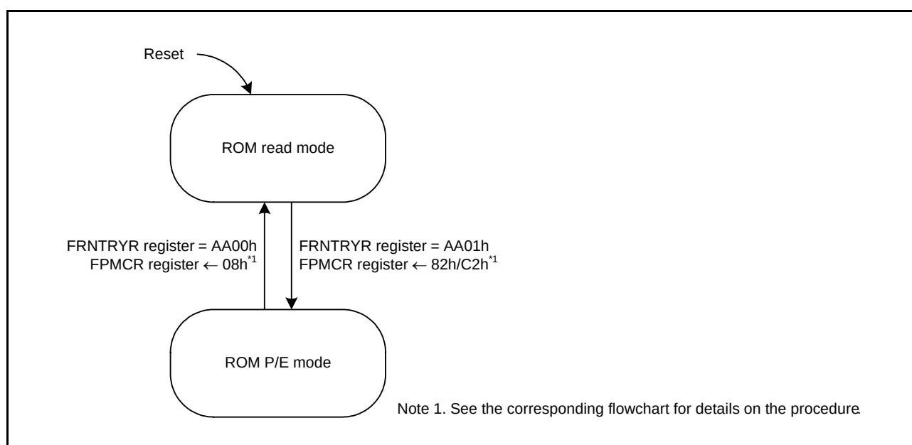
Figure 34.5 Mode Transitions of the Flash Memory
