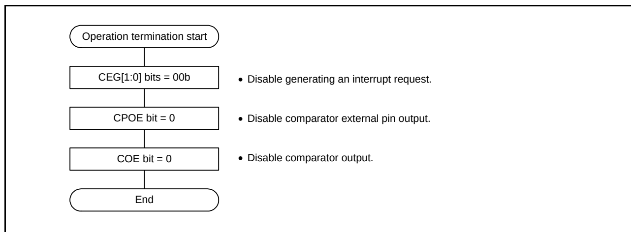
Figure 31.6 Comparator Operation Termination Flowchart
