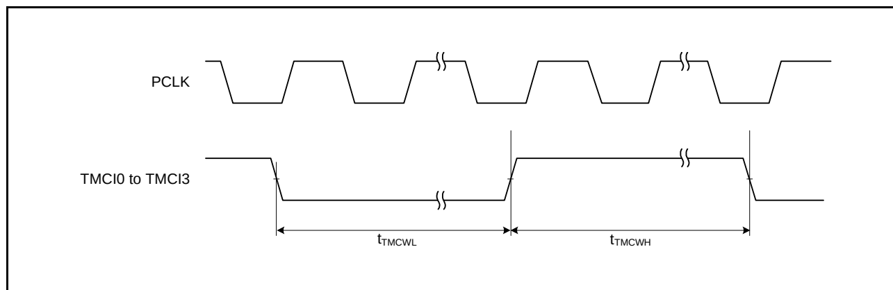
Figure 35.38 TMR Clock Input Timing
