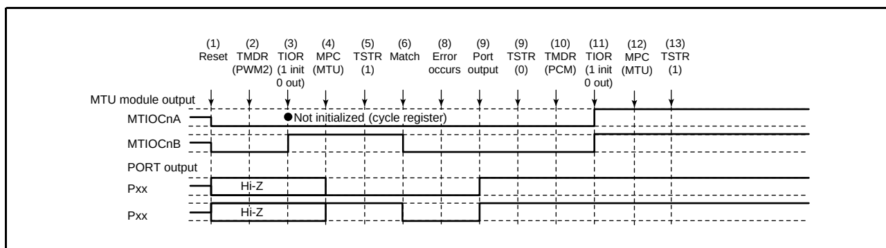
Figure 20.158 Error Occurrence in PWM Mode 2, Recovery in Phase Counting Mode
