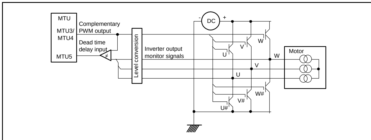
Figure 20.94 Motor Control Circuit Example
