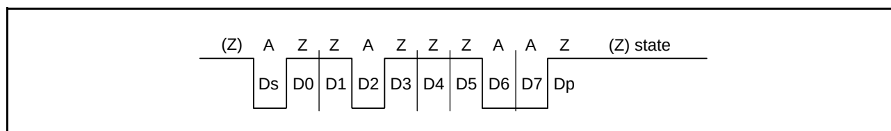
Figure 25.33 Direct Convention (SDIR in SCMR = 0, SINV in SCMR = 0, PM in SMR = 0)
