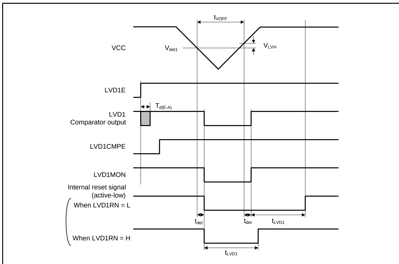
Figure 35.53 Voltage Detection Circuit Timing (V det1 )
