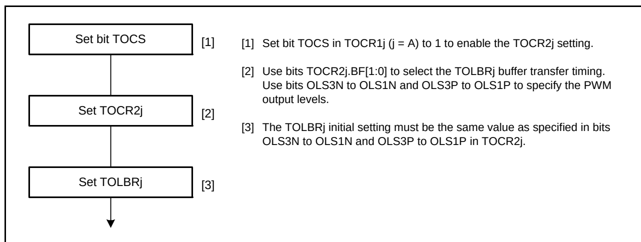
Figure 20.3 Example of PWM Output Level Setting Procedure in Buffer Operation
