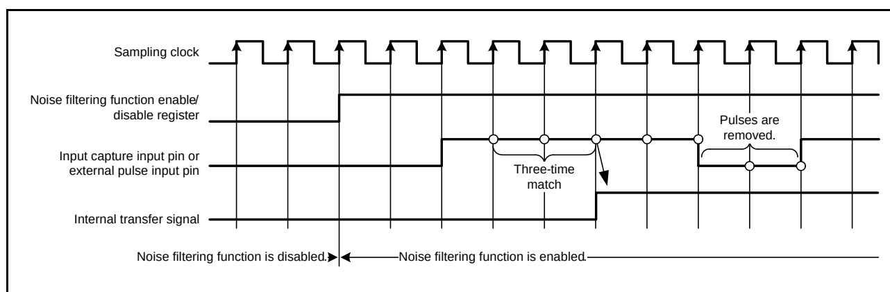
Figure 20.98 Timing of Noise Filtering
