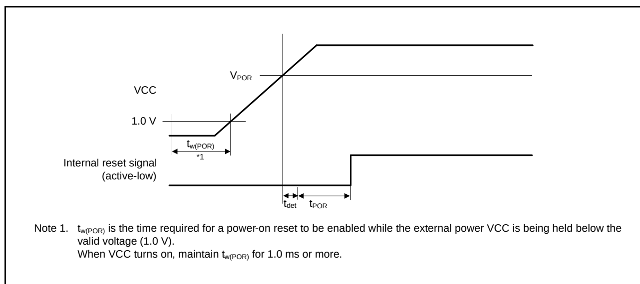
Figure 35.51 Power-On Reset Timing
