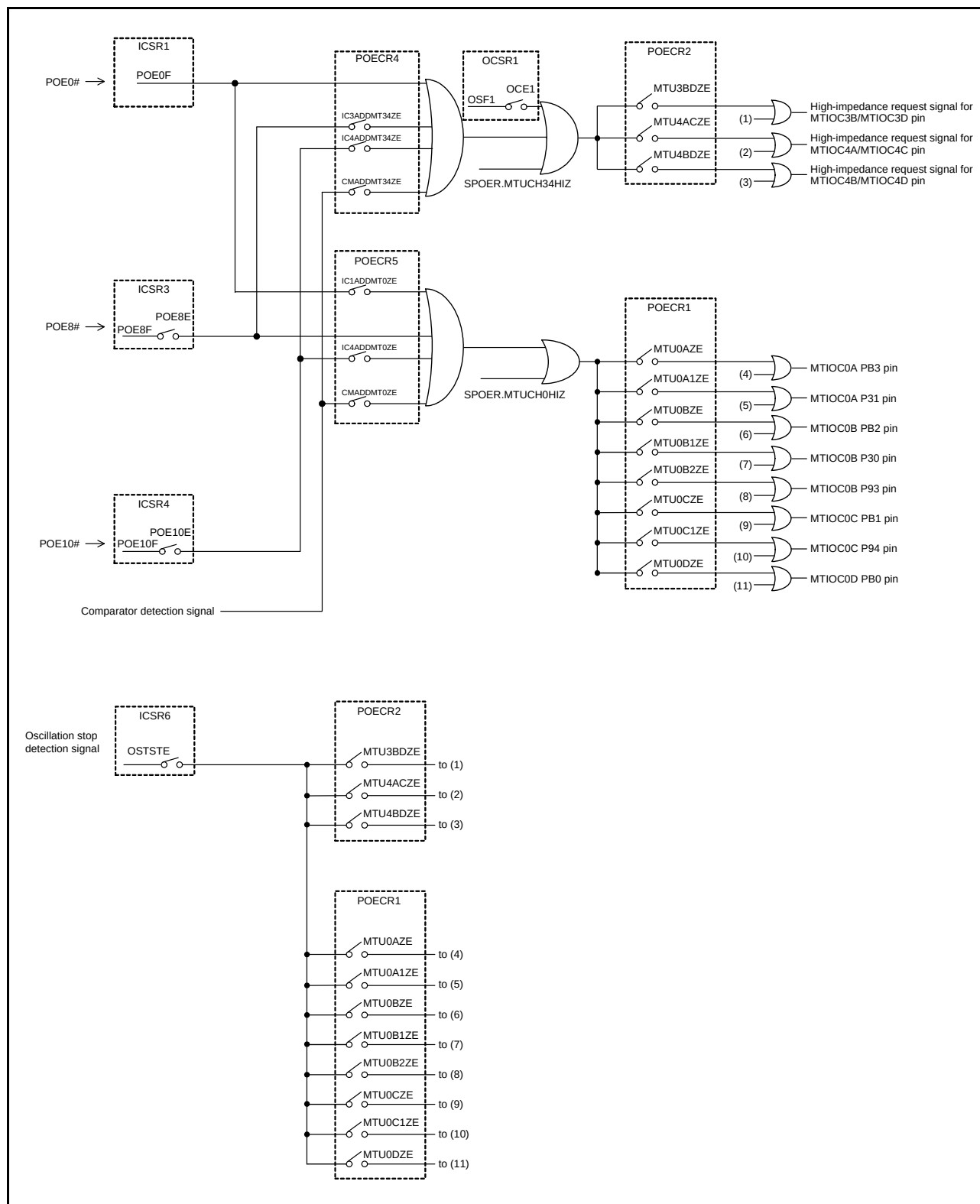
Figure 21.2 Target Pins and Conditions for High-Impedance Control
