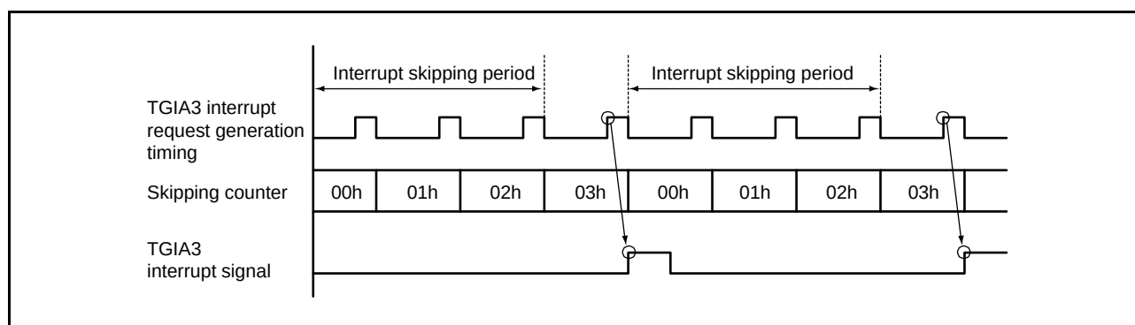
Figure 20.79 Example of Interrupt Skipping Function 1
