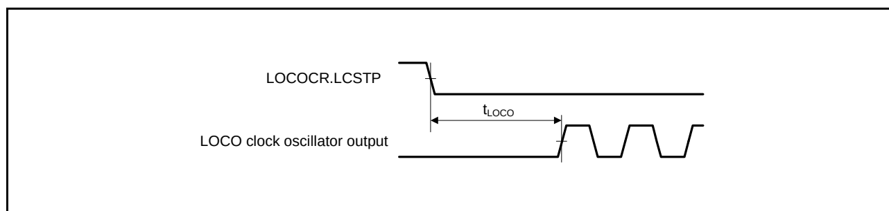
Figure 35.22 LOCO Clock Oscillation Start Timing
