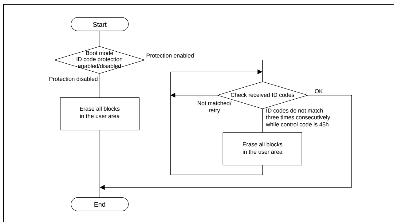
Figure 34.19 Authentication for Boot Mode ID Code Protection
