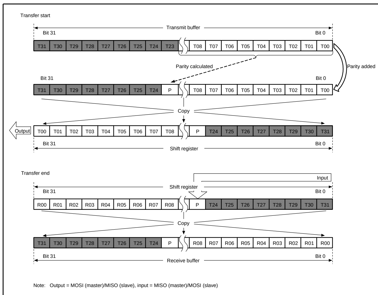
Figure 27.21 LSB First Transfer (24-Bit Data, Parity Enabled)
