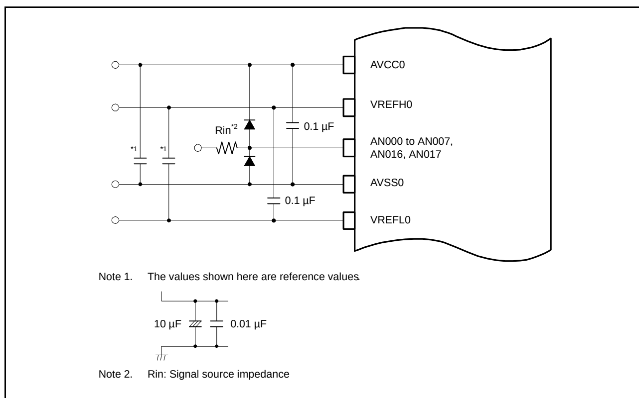
Figure 29.30 Sample Protection Circuit for Analog Inputs
