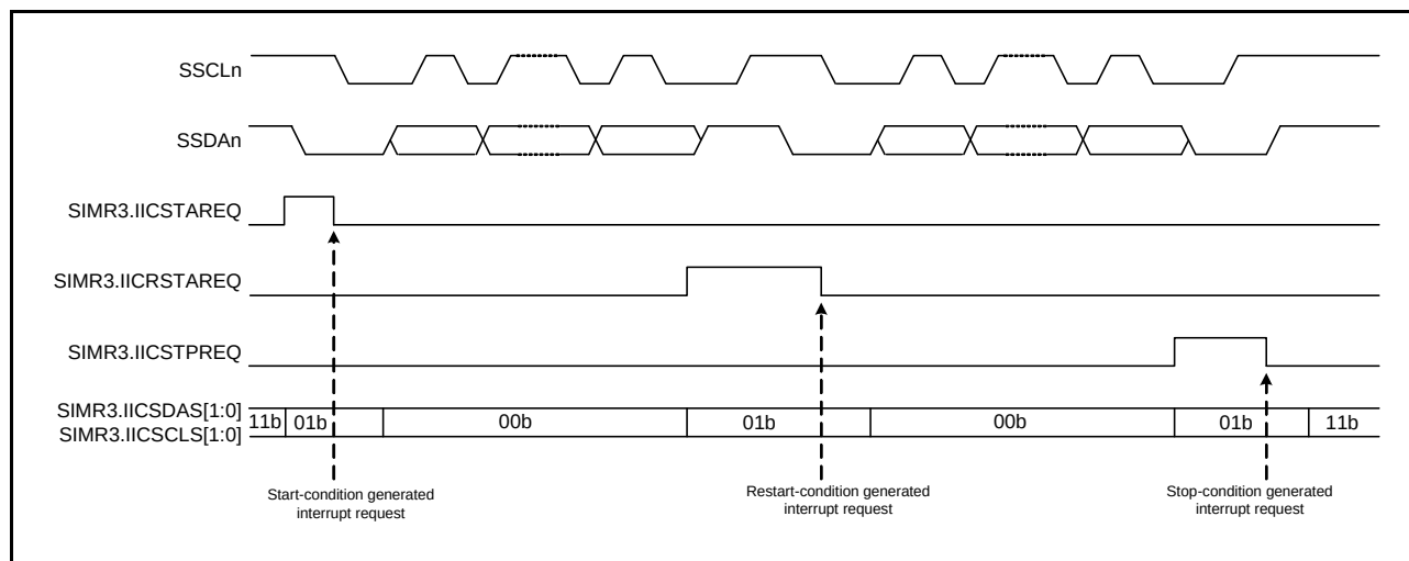
Figure 25.45 Timing of Operations in the Generation of Start, Restart, and Stop Conditions
