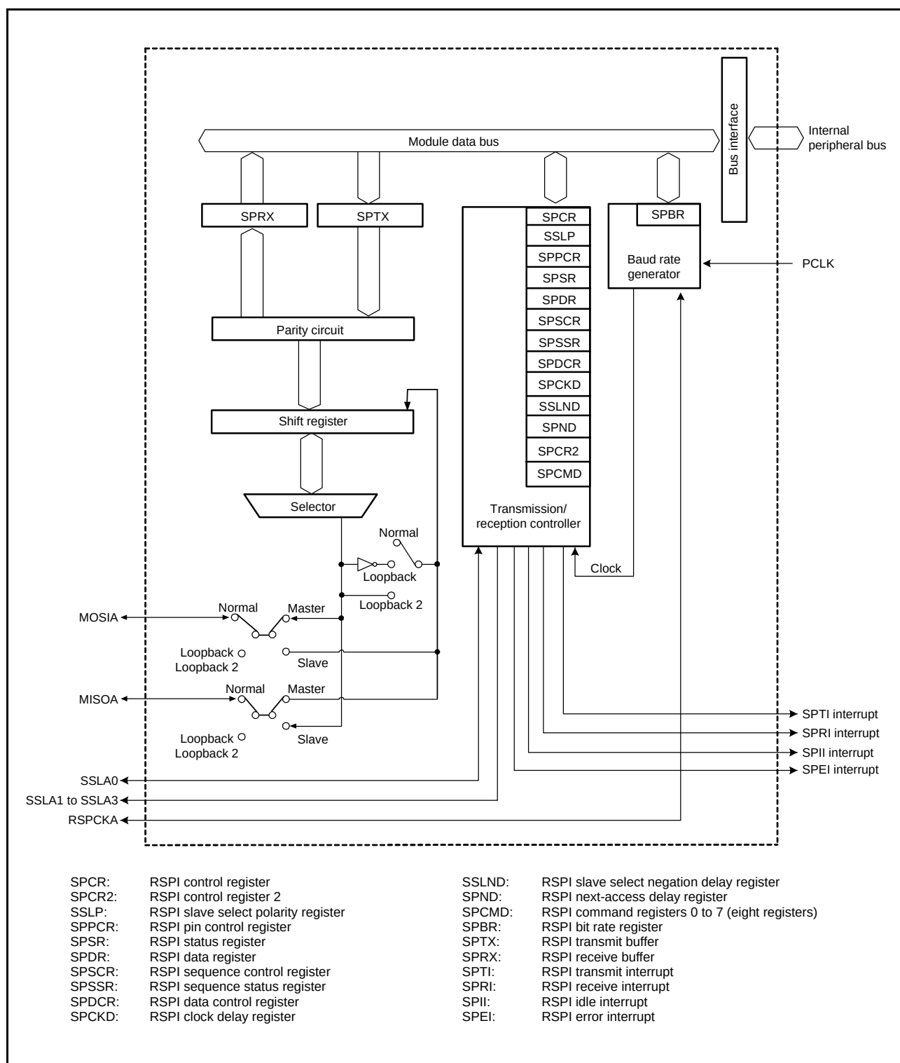
Figure 27.1 RSPI Block Diagram
