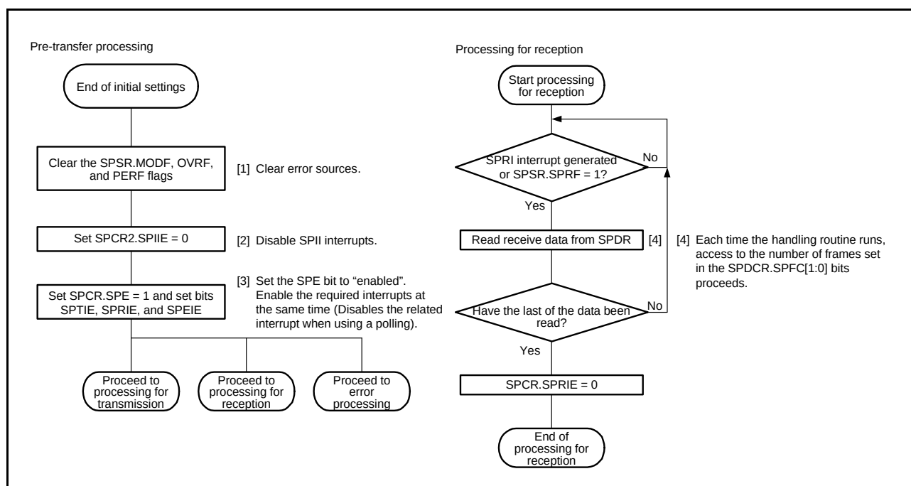
Figure 27.41 Flowchart in Slave Mode (Reception)
