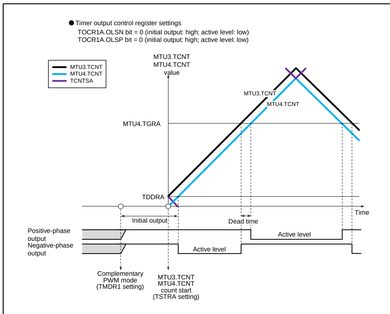
Figure 20.51 Example of Initial Output in Complementary PWM Mode (MTU3 and MTU4) (1)
