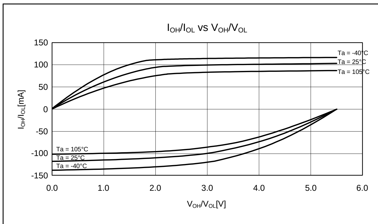
Figure 35.11 V OH /V OL and I OH /I OL Temperature Characteristics at VCC = 5.5 V when Normal Output is Selected (Reference Data)
