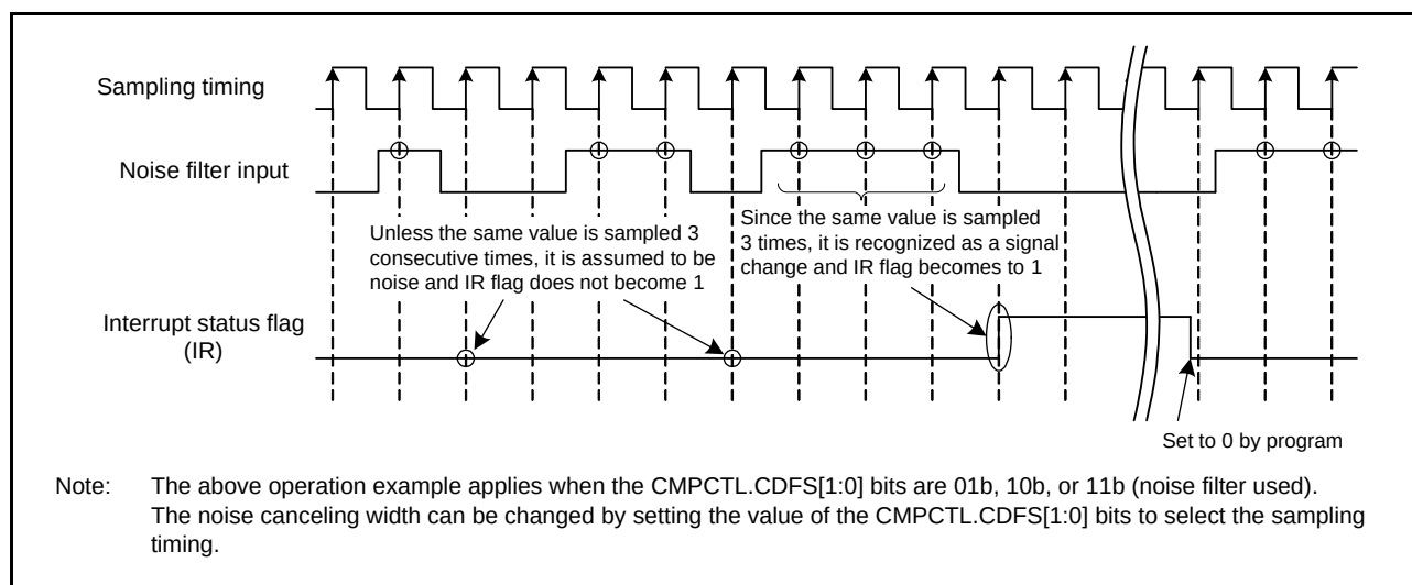
Figure 31.4 Comparator Noise Filter and Interrupt Operation Example
