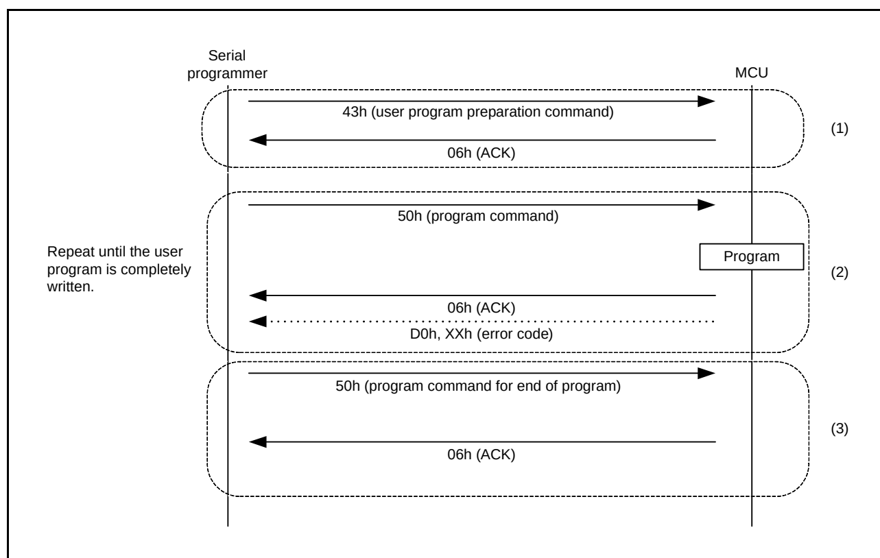
Figure 34.28 Procedure to Program the User Area
