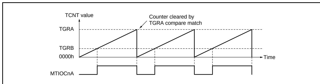
Figure 20.26 Example of PWM Mode 1 Operation (n = 0 to 4)
