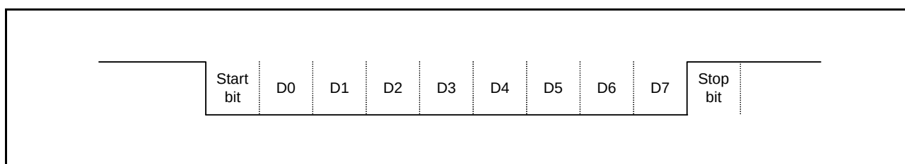
Figure 34.15 Communication Format
