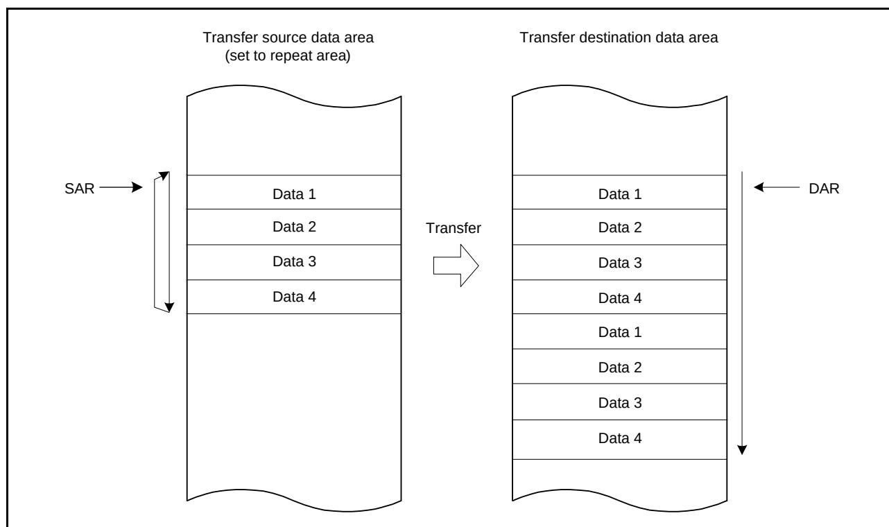
Figure 17.6 Memory Map of Repeat Transfer Mode (Transfer Source: Repeat Area)
