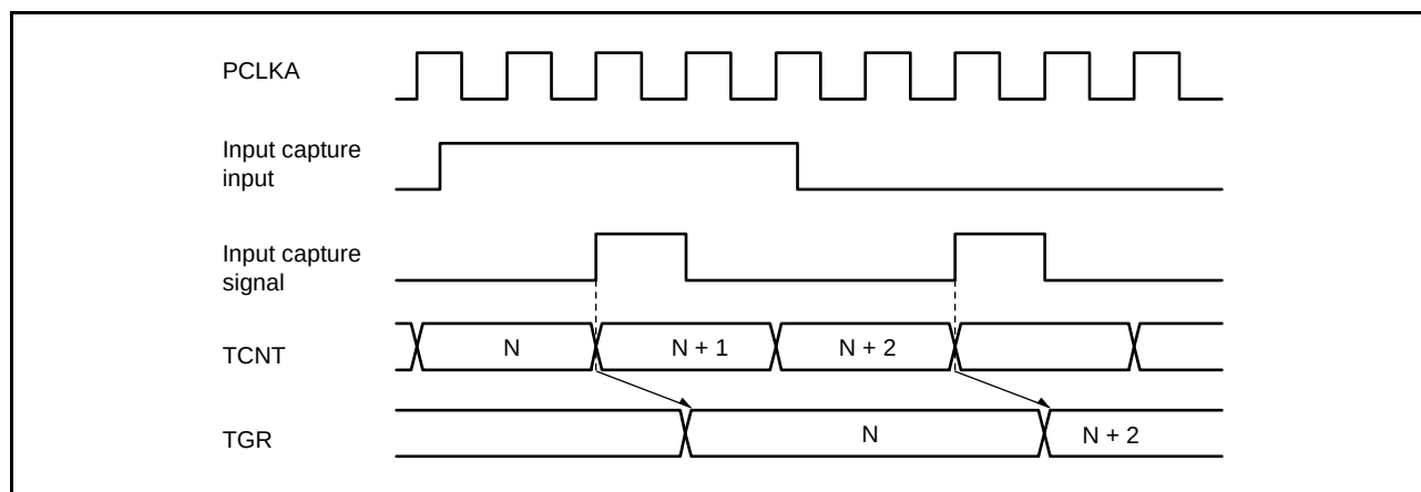
Figure 20.106 Input Capture Input Signal Timing
