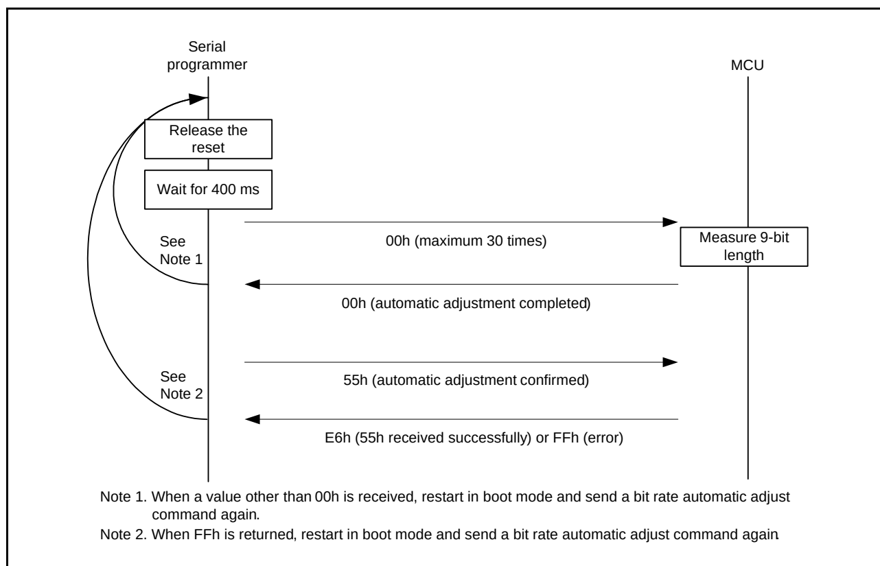
Figure 34.22 Bit Rate Automatic Adjustment Procedure
