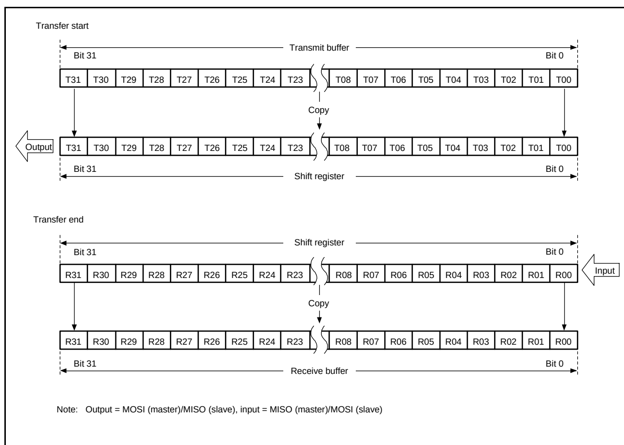
Figure 27.14 MSB First Transfer (32-Bit Data, Parity Disabled)
