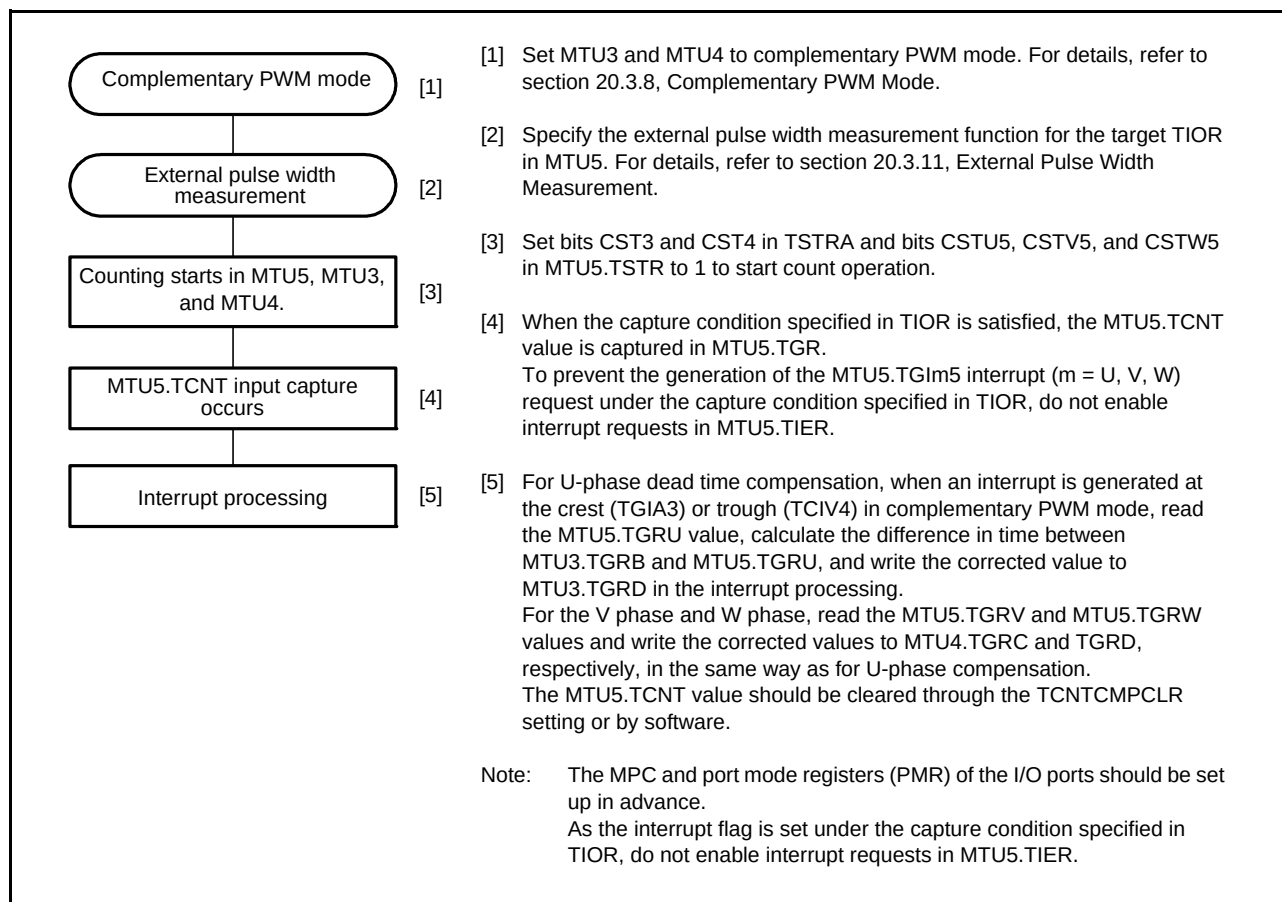
Figure 20.96 Example of Dead Time Compensation Setting Procedure
