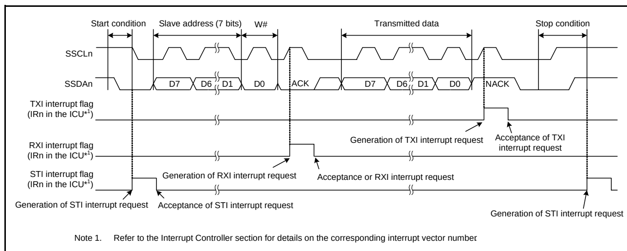
Figure 25.50 Example 2 of Operations for Master Transmission in Simple I 2 C-bus Mode (with 7-Bit Slave Addresses, ACK Interrupts, and NACK Interrupts in Use)
