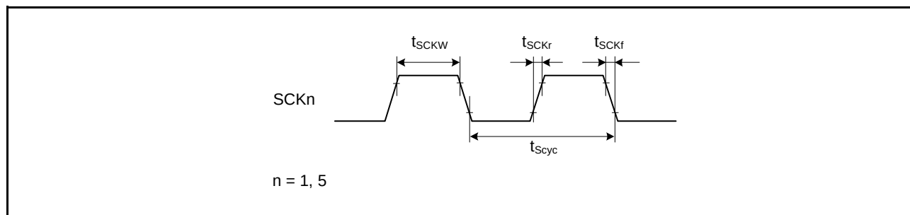
Figure 35.39 SCK Clock Input Timing
