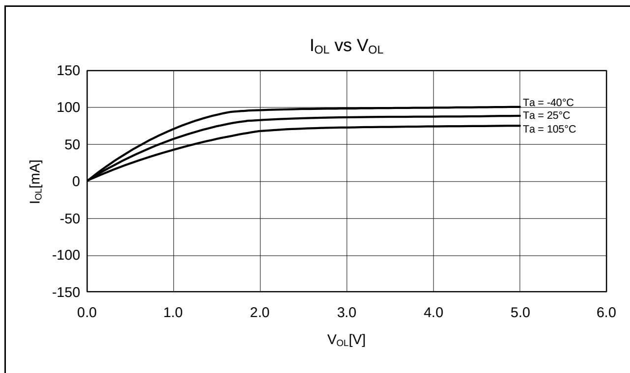
Figure 35.18 V OL and I OL Temperature Characteristics of RIIC Output Pin at VCC = 5.0 V (Reference Data)
