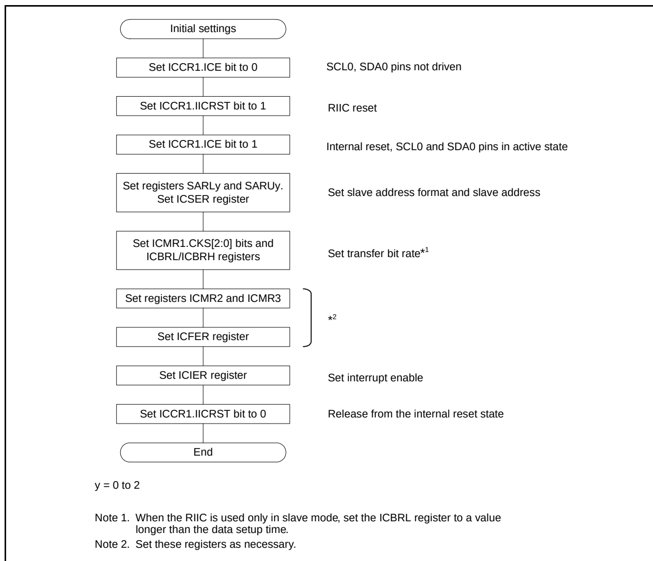
Figure 26.5 Example of RIIC Initialization Flowchart
