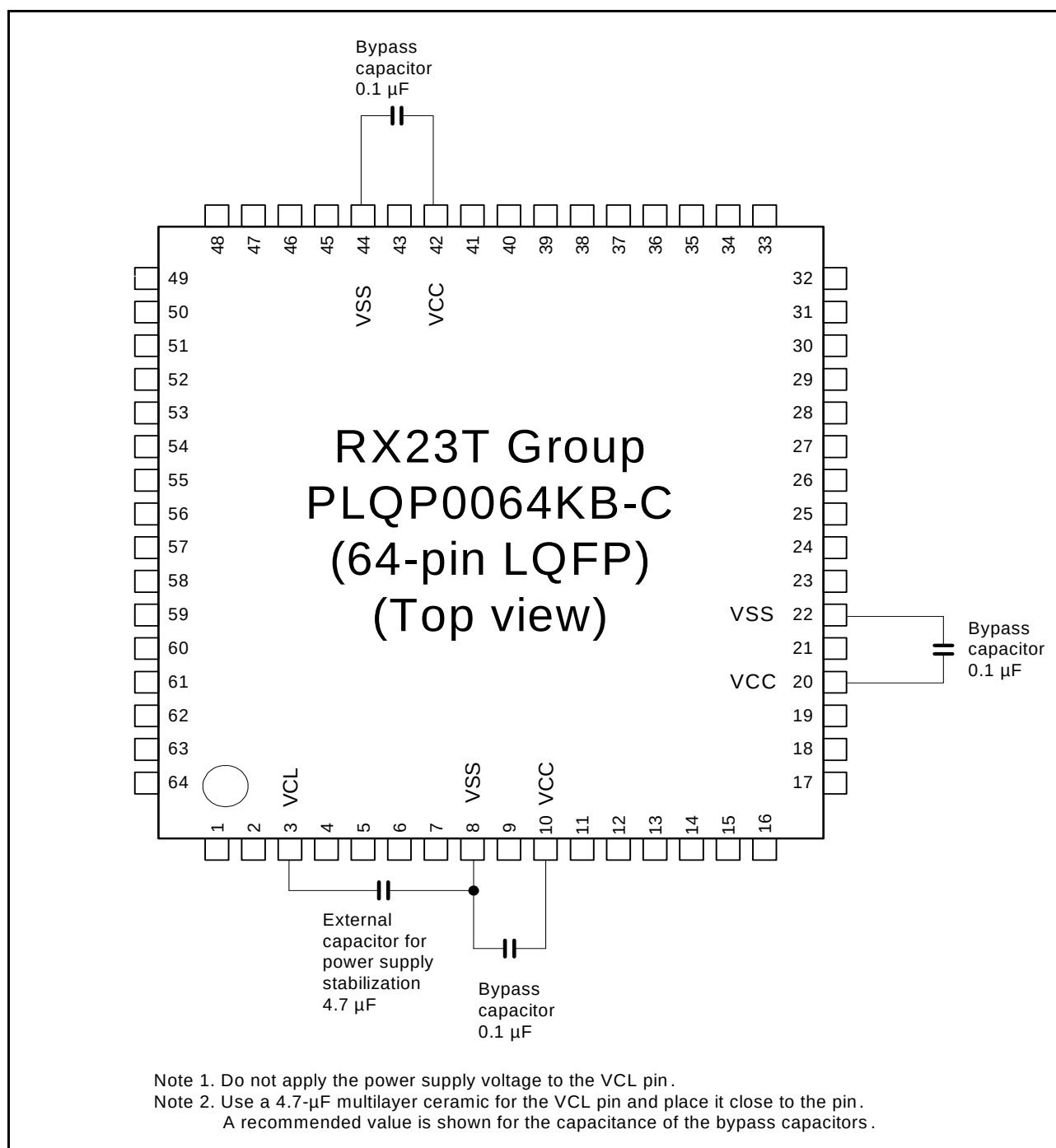
Figure 35.56 Connecting Capacitors (64 Pins)
