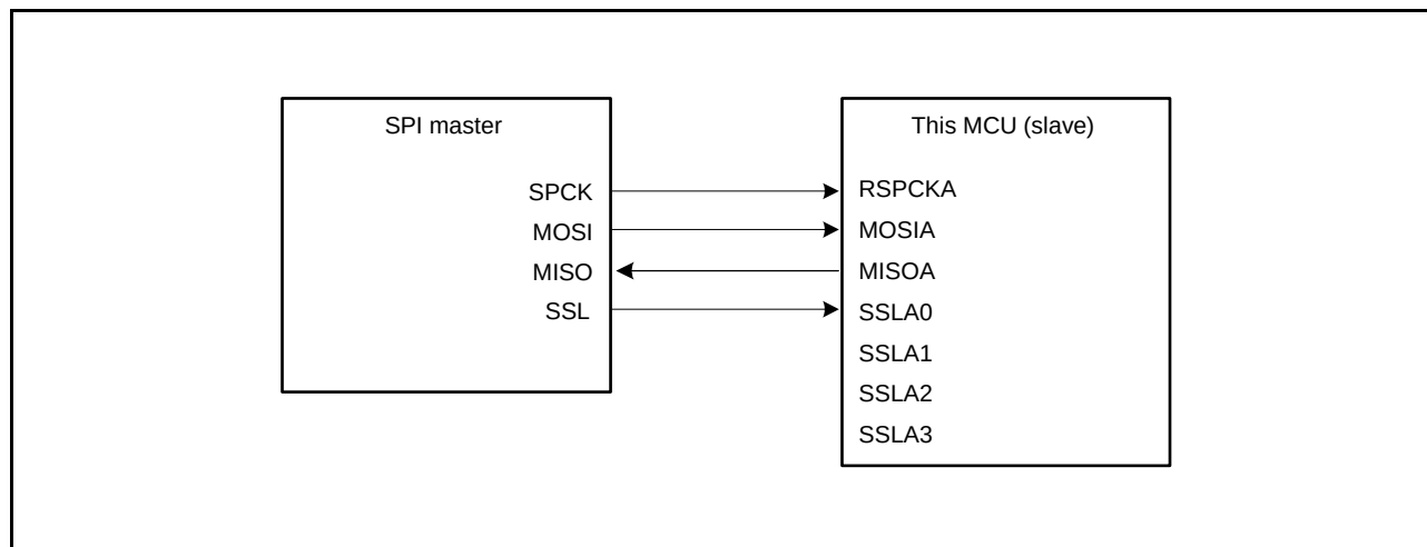
Figure 27.6 Single-Master/Single-Slave Configuration Example (This MCU = Slave, CPHA = 0)
