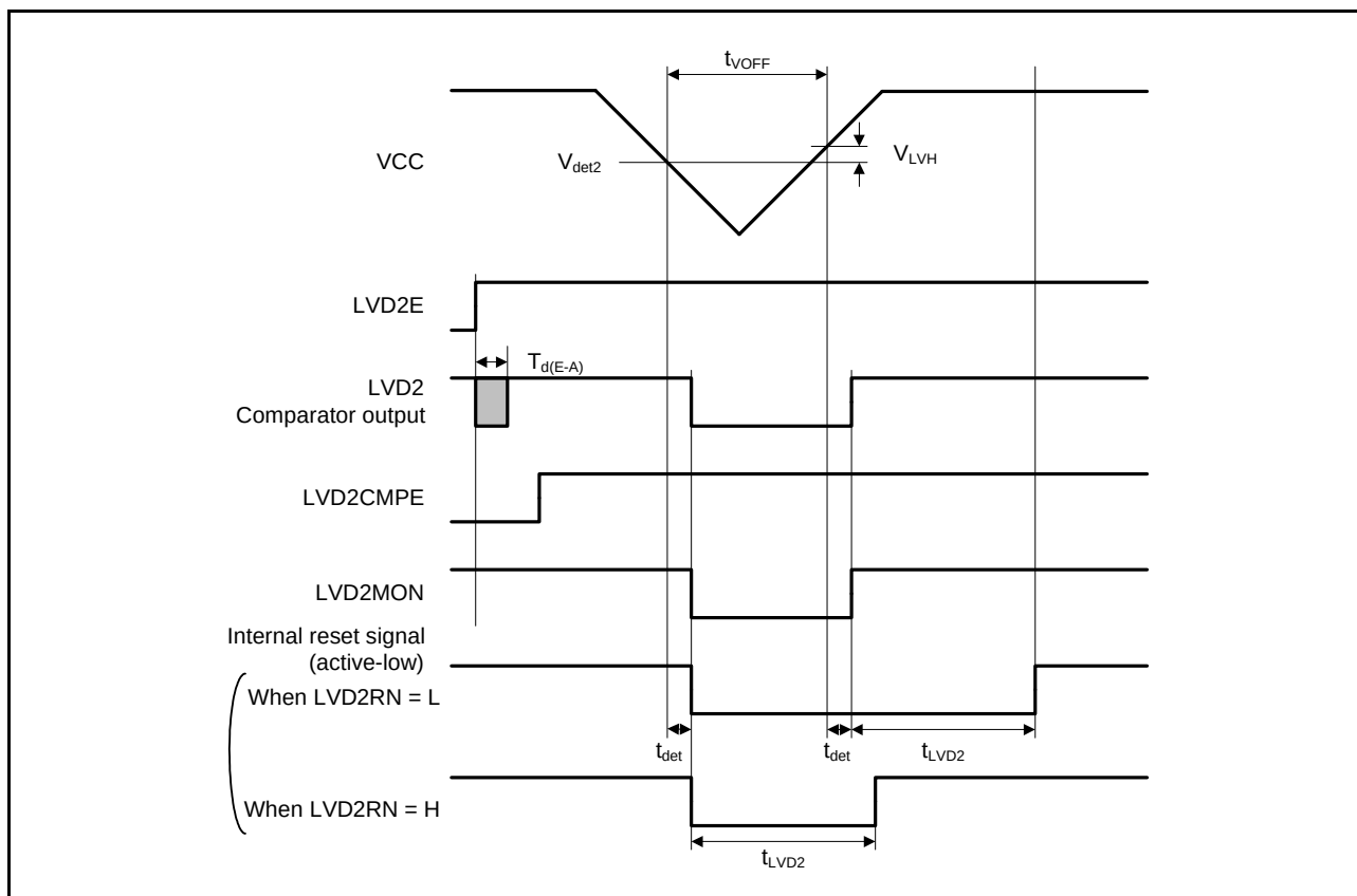
Figure 35.54 Voltage Detection Circuit Timing (V det2 )
