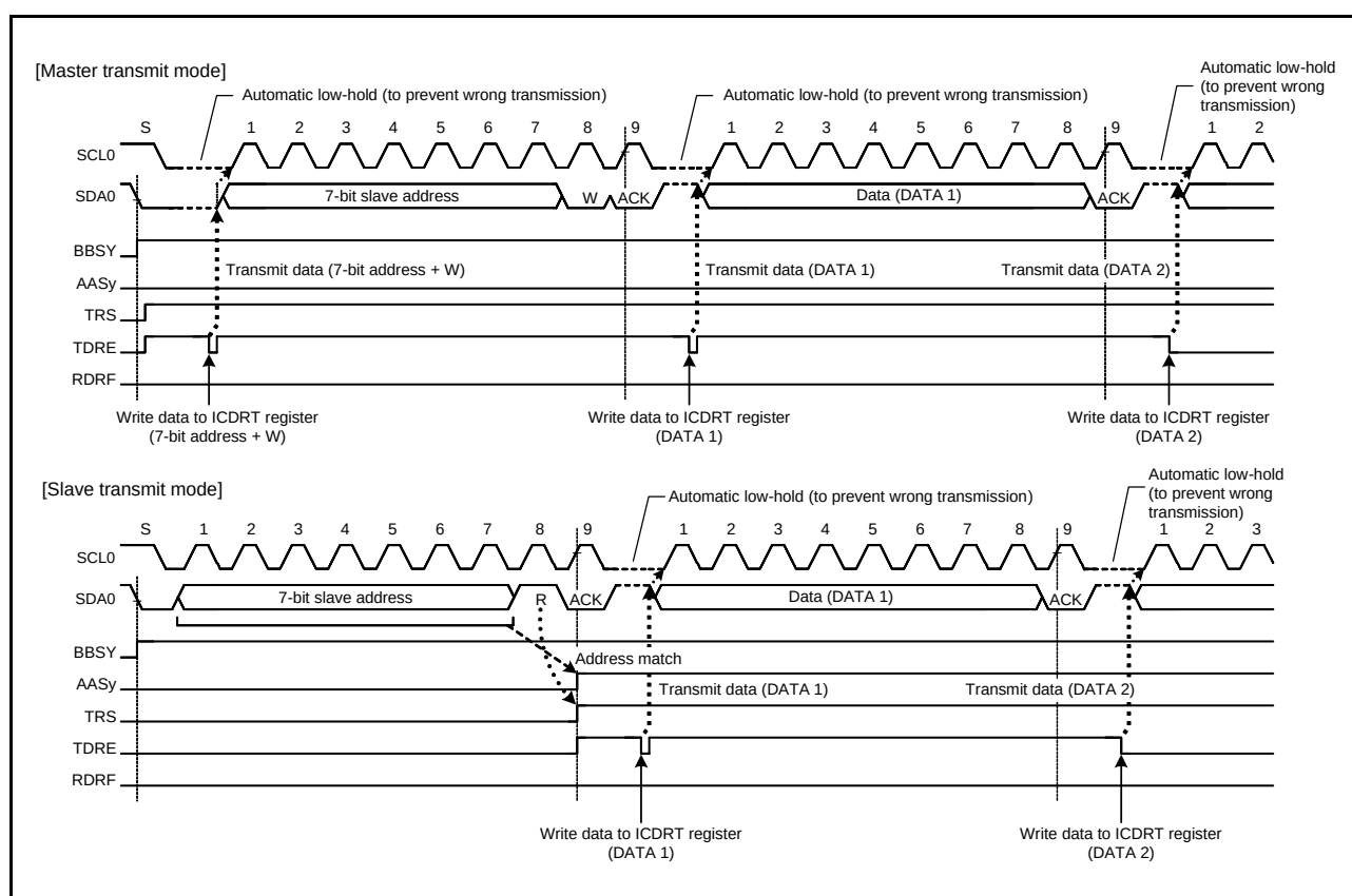
Figure 26.30 Automatic Low-Hold Operation in Transmit Mode
