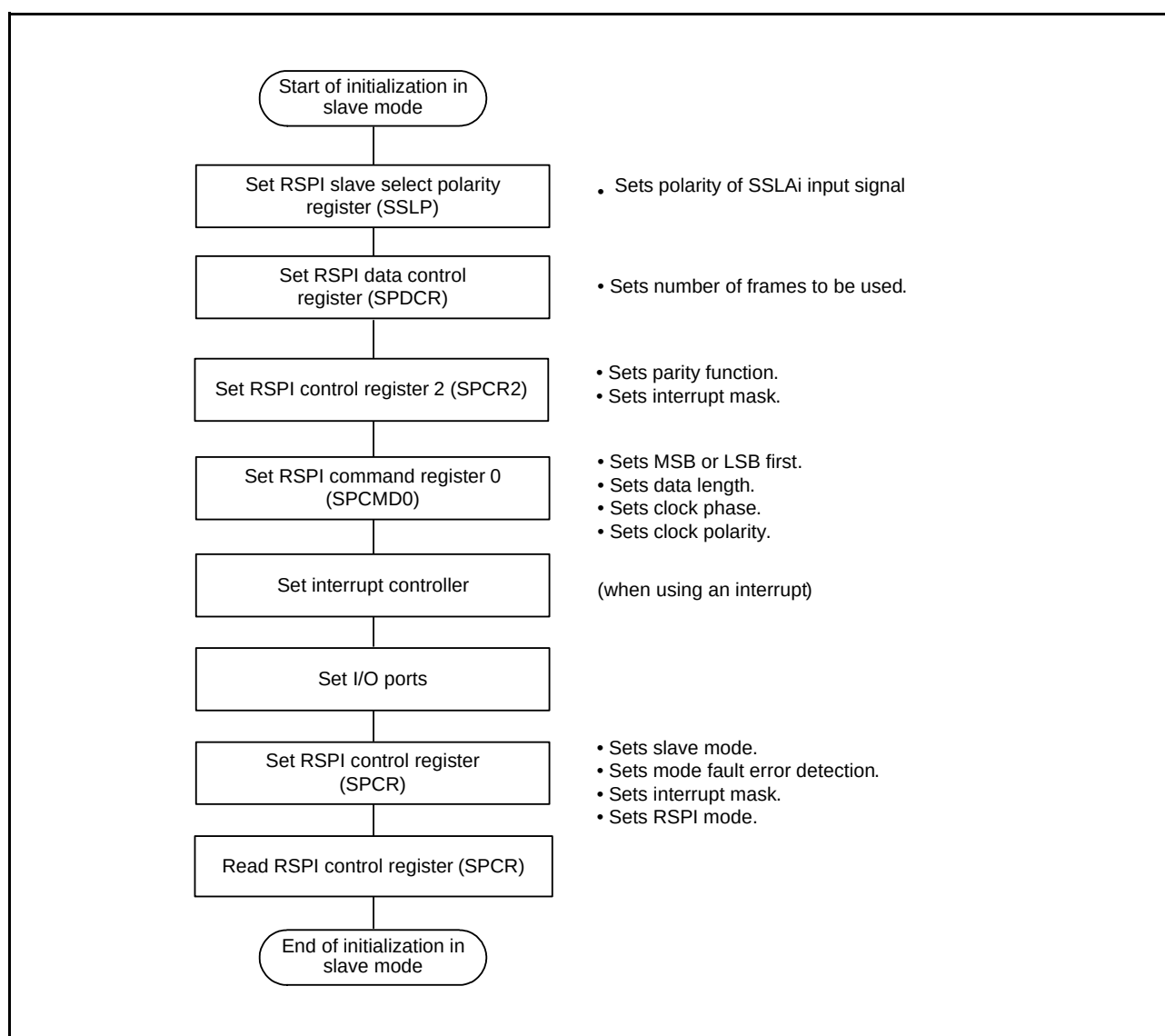
Figure 27.39 Example of Initialization Flowchart in Slave Mode (SPI Operation)
