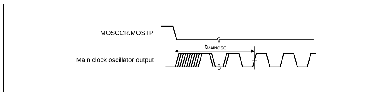
Figure 35.21 Main Clock Oscillation Start Timing
