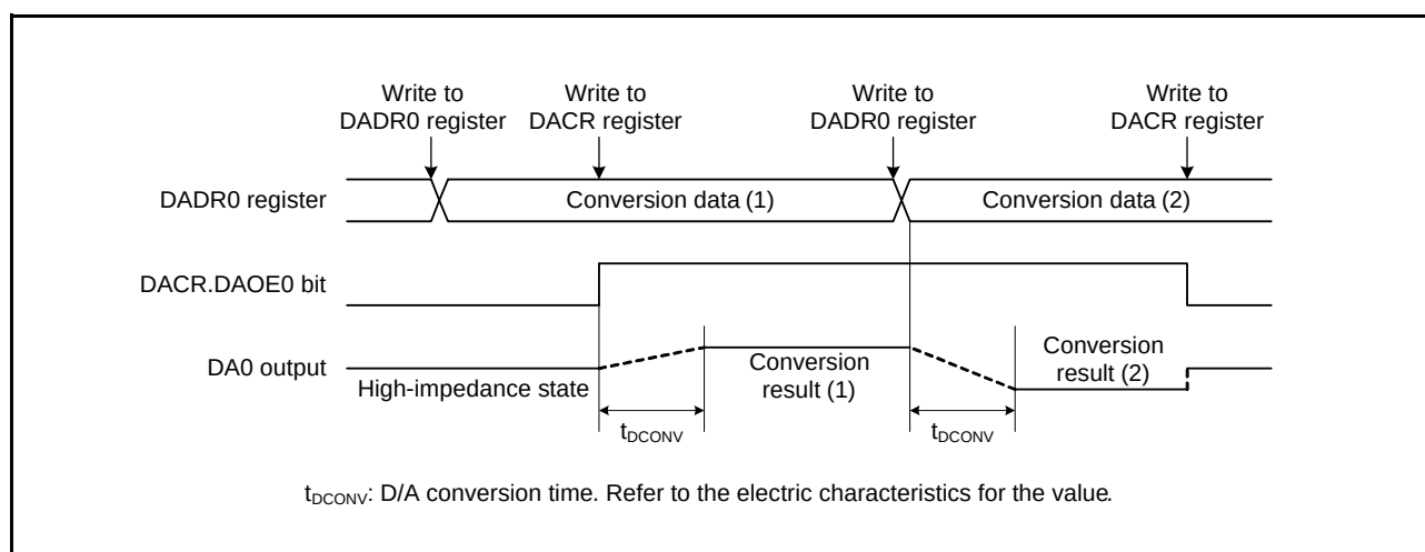
Figure 30.2 Example of 8-Bit D/A Converter Operation
