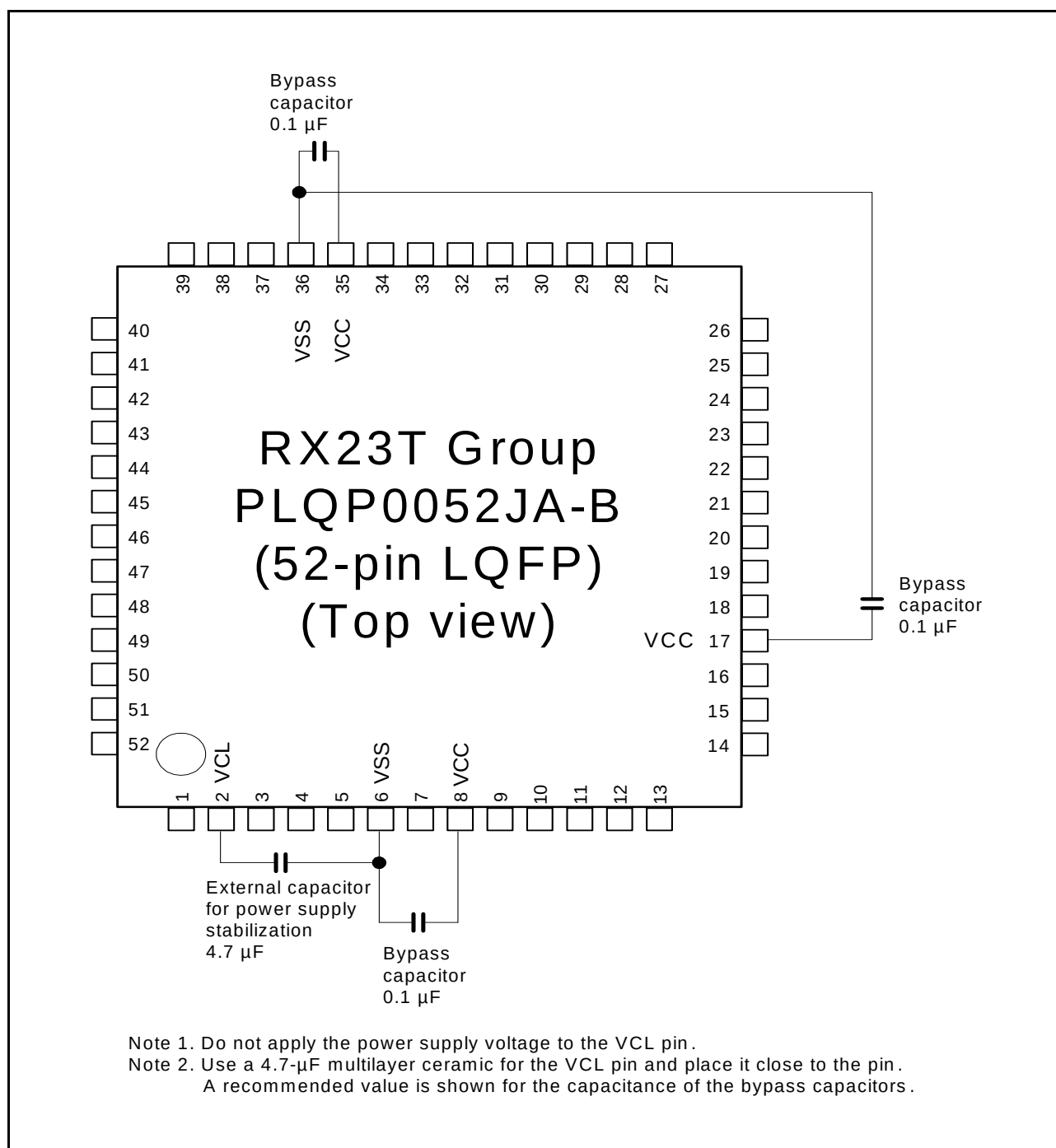
Figure 35.57 Connecting Capacitors (52 Pins)
