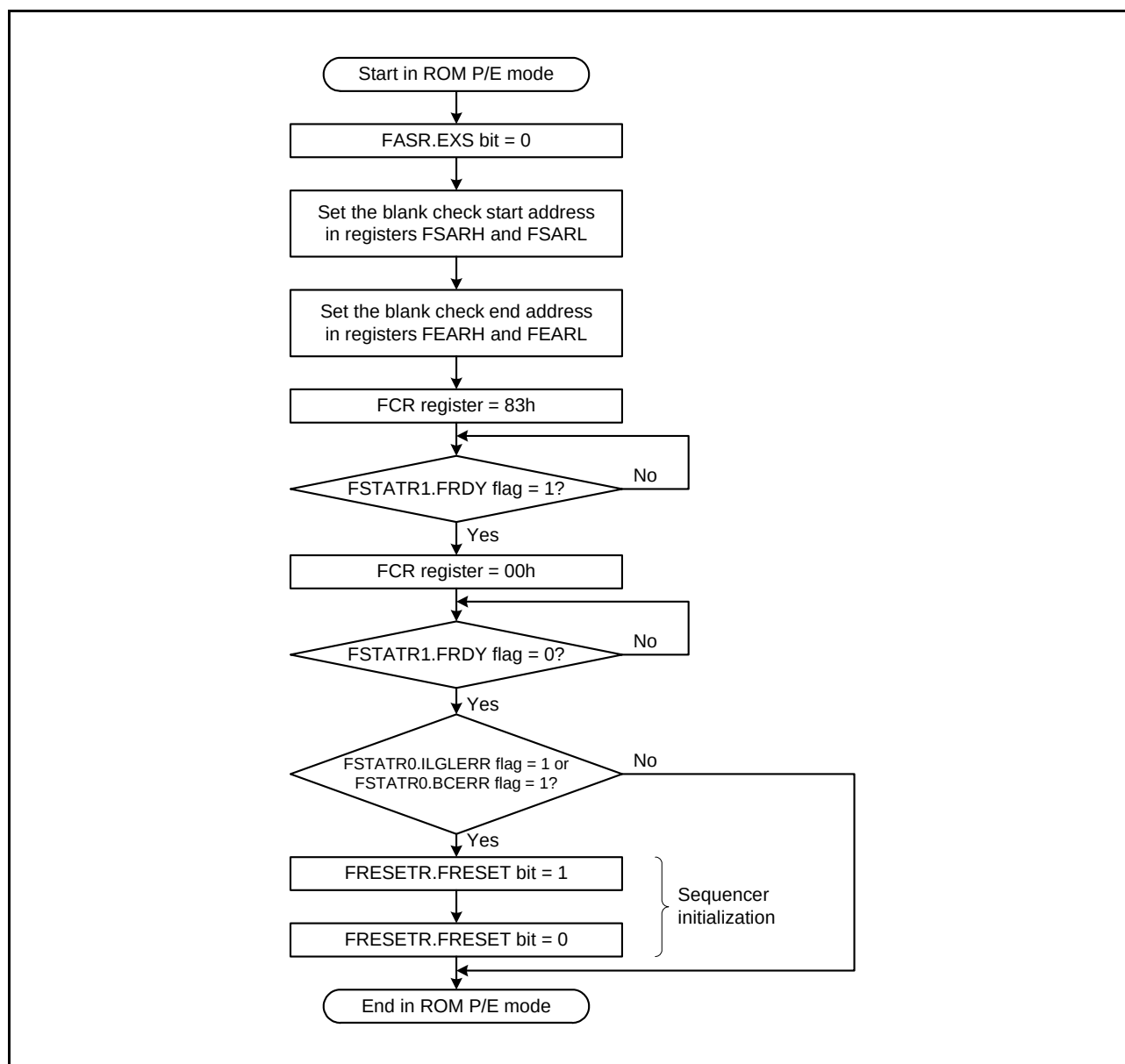
Figure 34.11 Procedure to Issue the Blank Check Command
