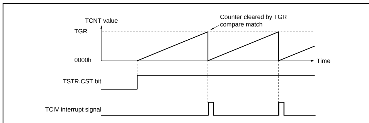
Figure 20.6 Periodic Counter Operation
