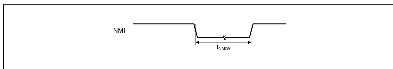
Figure 35.32 NMI Interrupt Input Timing
