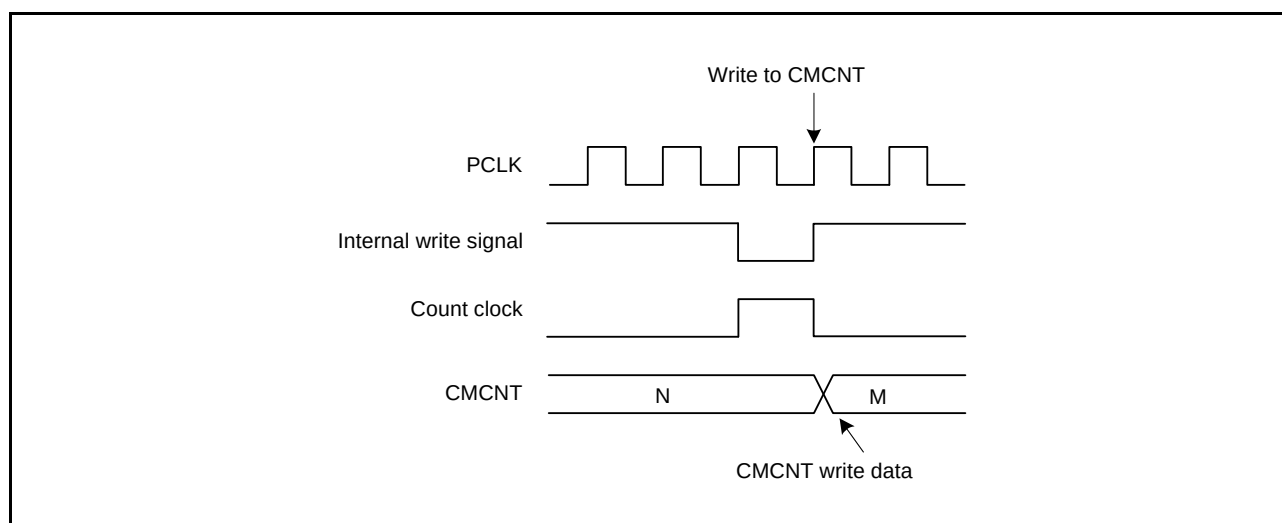
Figure 23.6 Conflict between CMCNT Counter Writing and Incrementing
