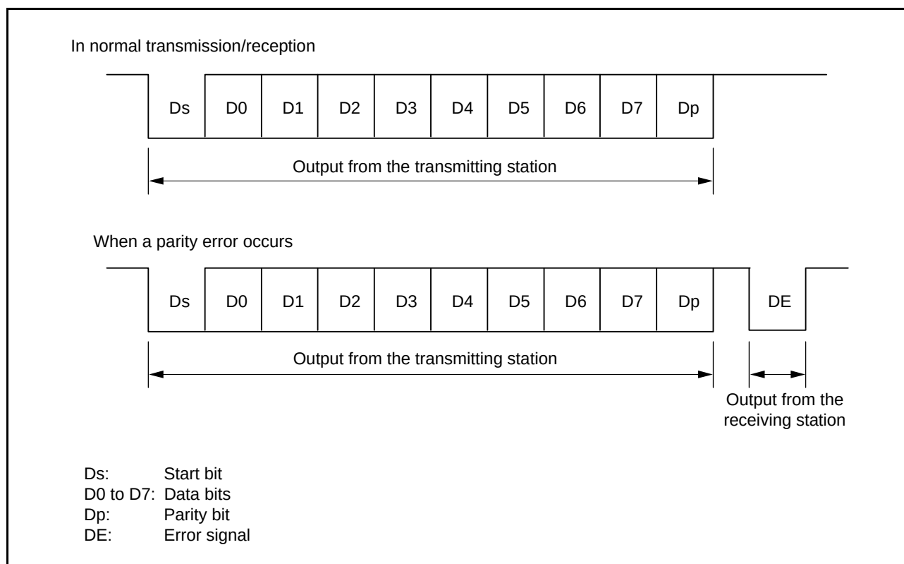
Figure 25.32 Data Formats in Smart Card Interface Mode
