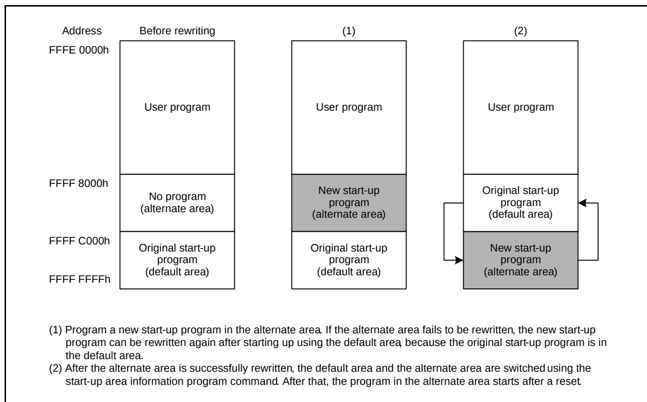
Figure 34.3 Overview of the Start-Up Program Protection
