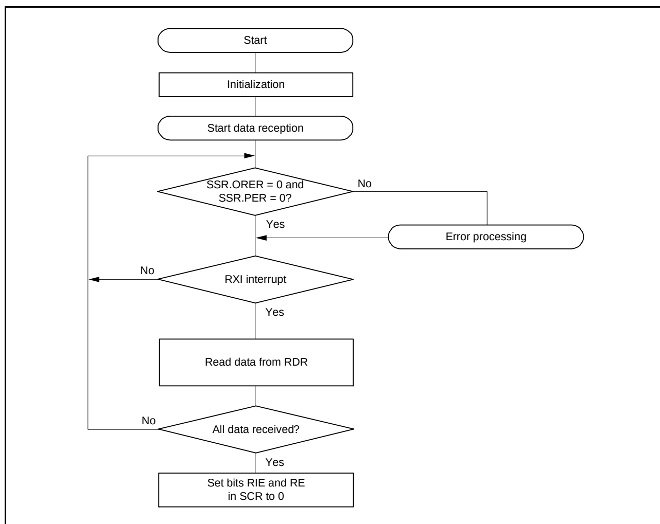
Figure 25.41 Sample Smart Card Interface Reception Flowchart
