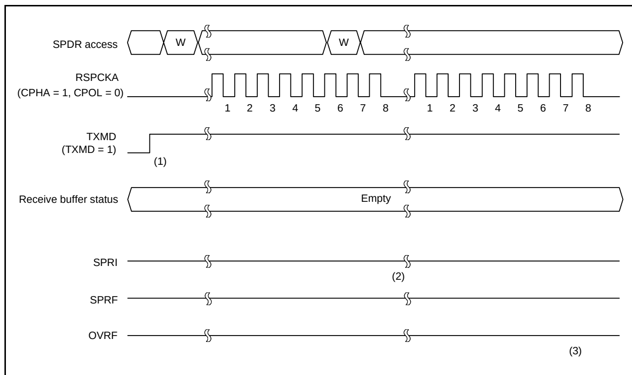
Figure 27.25 Operation Example of SPCR.TXMD = 1
