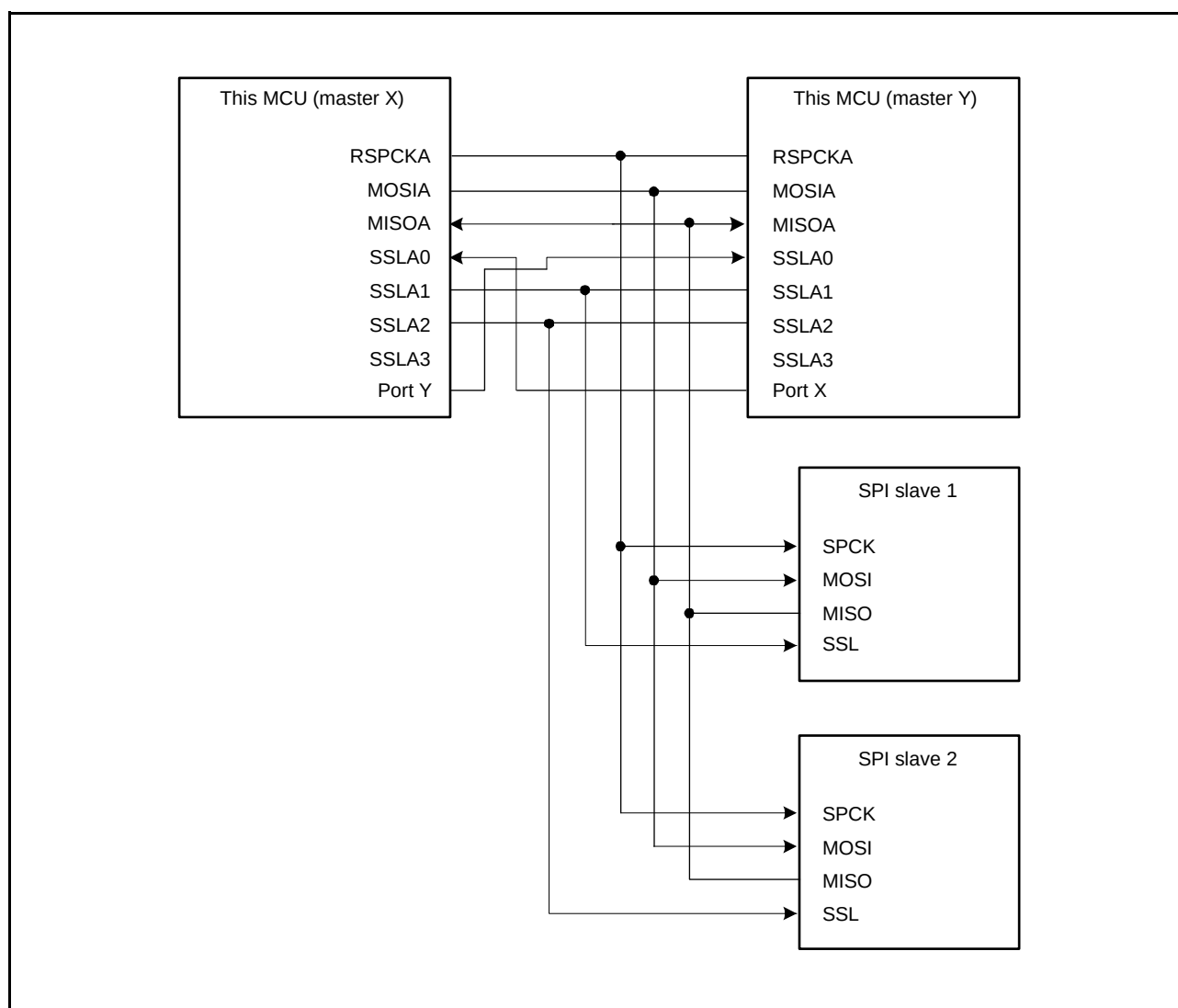
Figure 27.10 Multi-Master/Multi-Slave Configuration Example (This MCU = Master)
