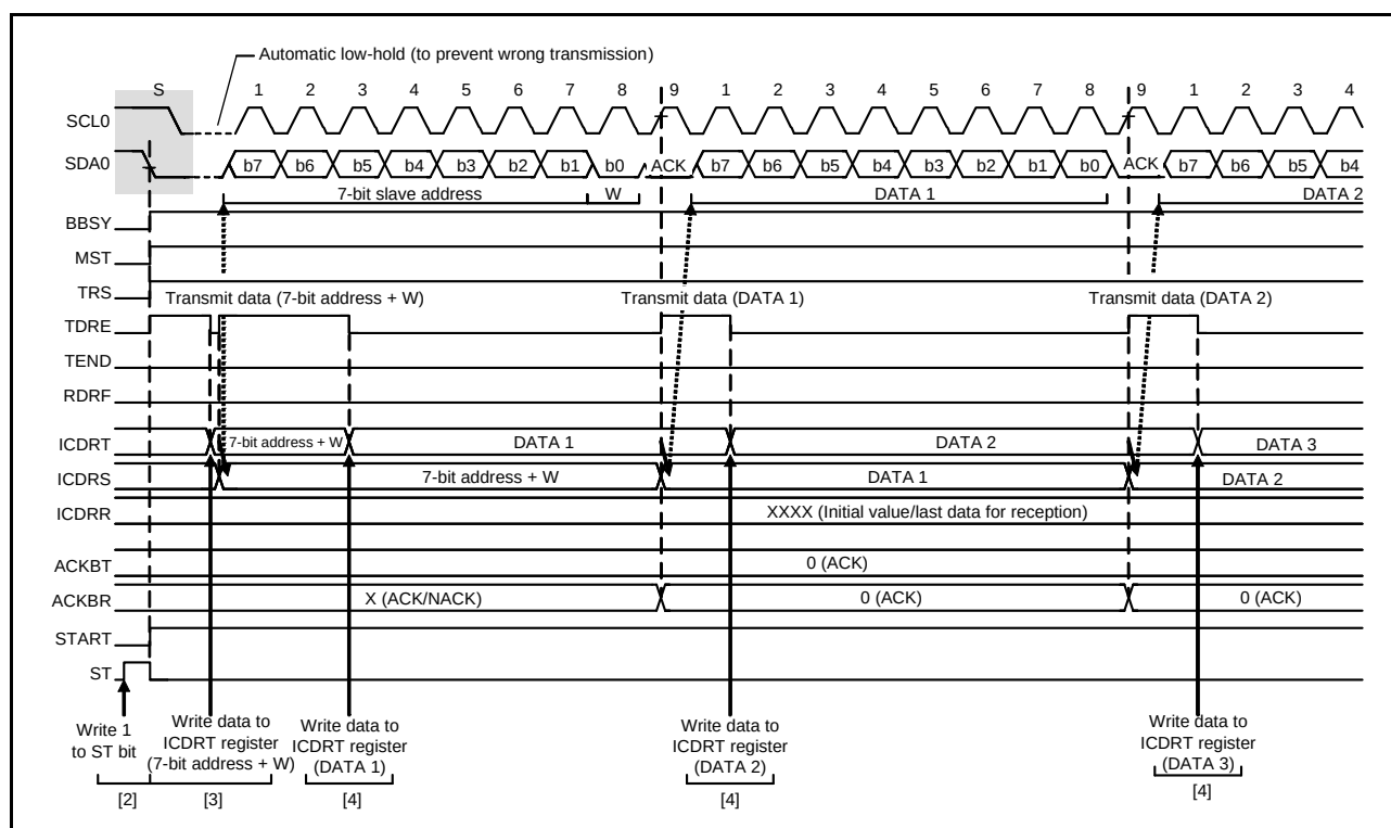
Figure 26.7 Master Transmit Operation Timing (1) (7-Bit Address Format)
