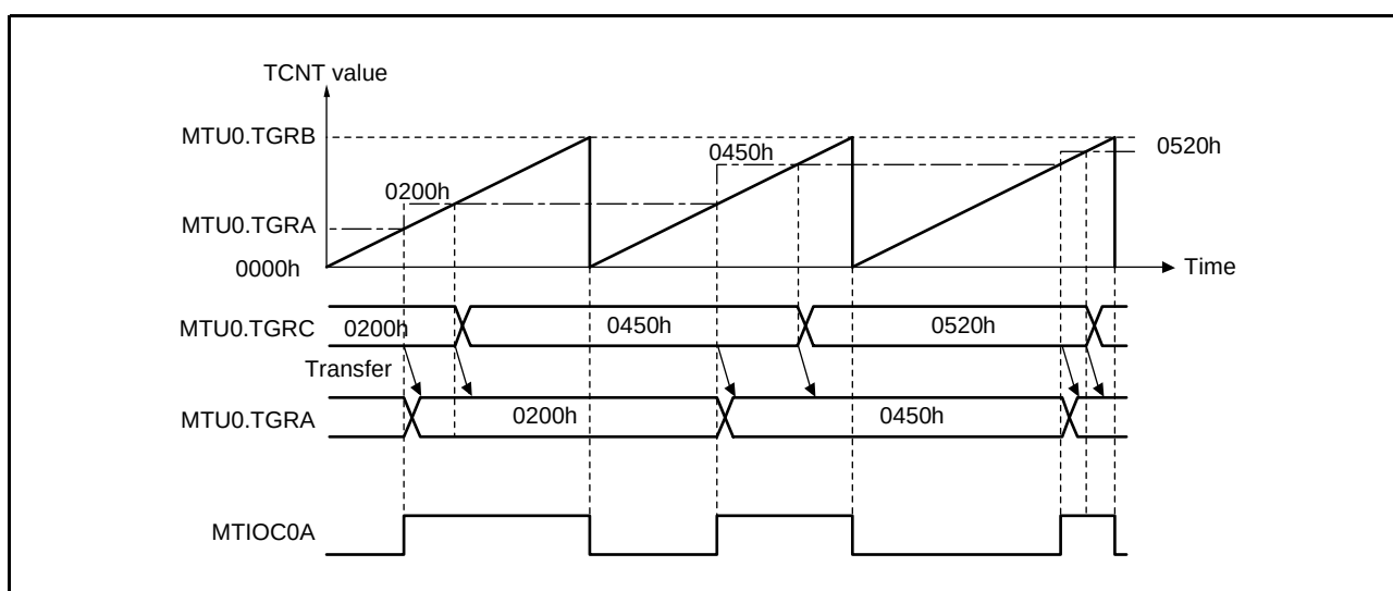
Figure 20.17 Example of Buffer Operation (1)
