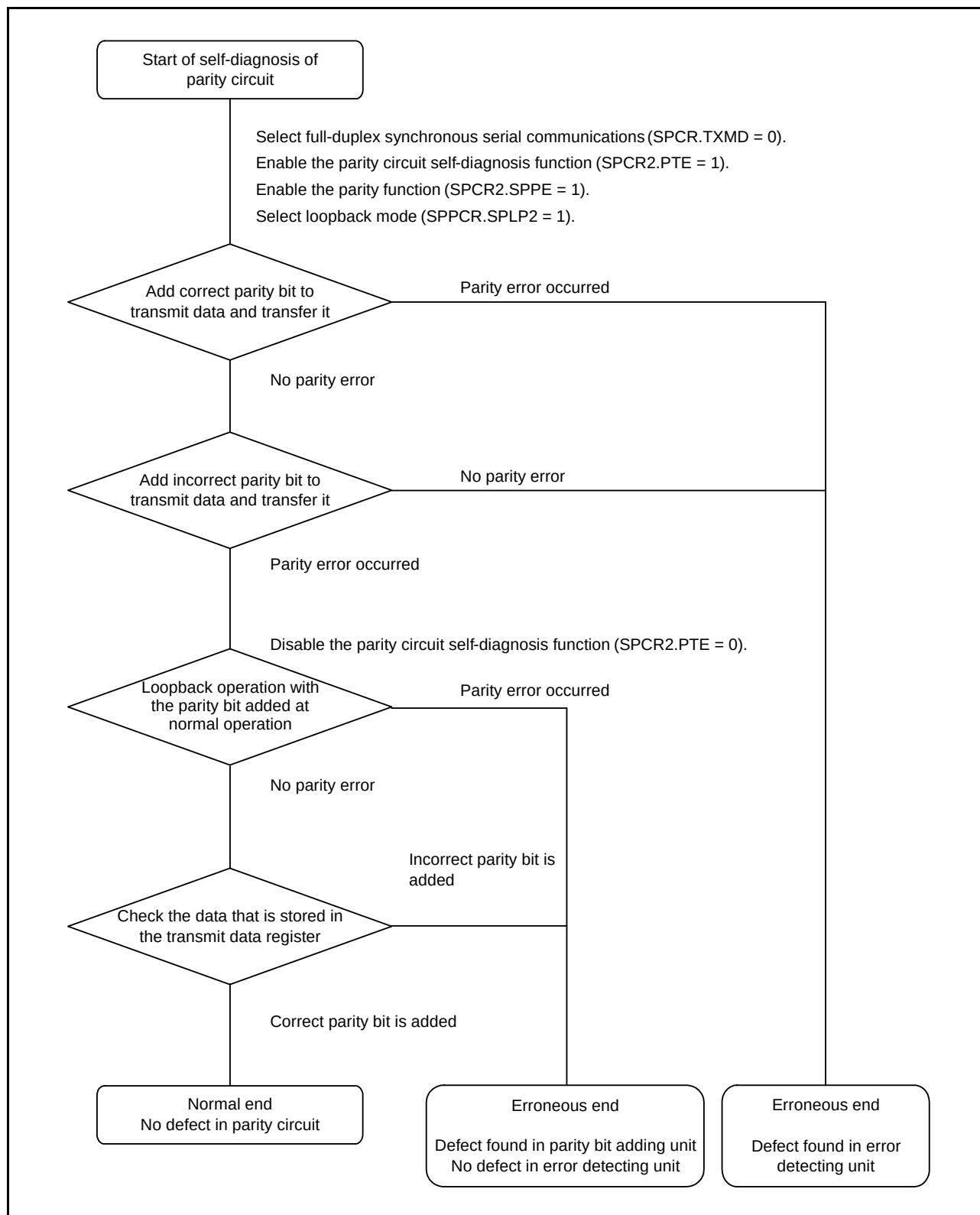
Figure 27.49 Flowchart for Self-Diagnosis of Parity Circuit
