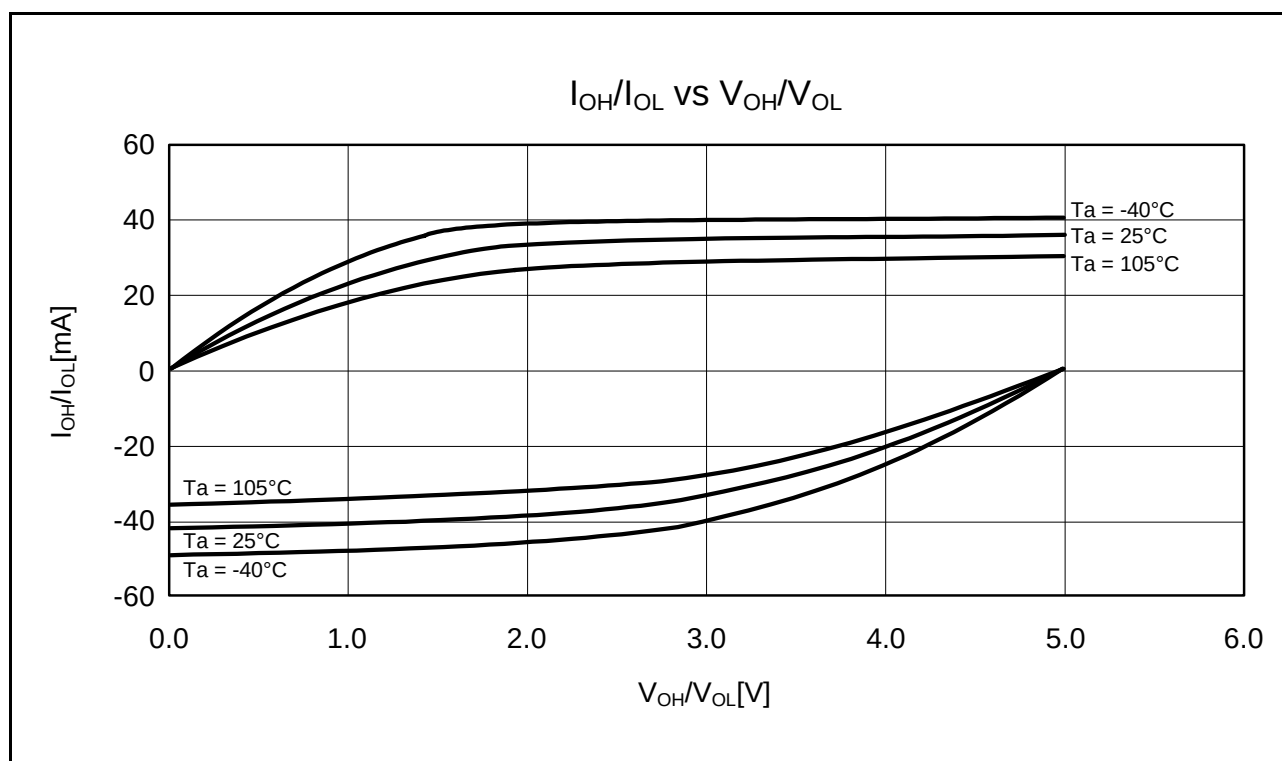
Figure 35.6 V_{OH}/V_{OL} and I_{OH}/I_{OL} Temperature Characteristics at V_{CC} = 5.0 V when Normal Output is Selected (Reference Data)
