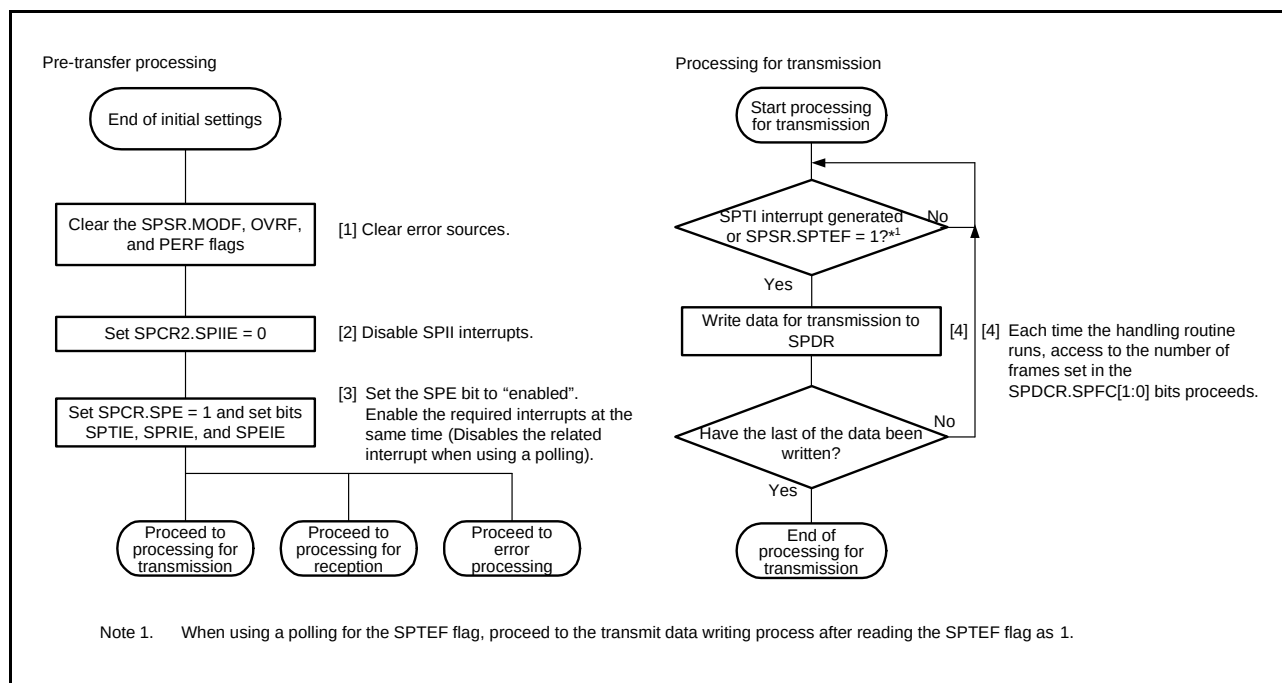
Figure 27.40 Flowchart in Slave Mode (Transmission)
