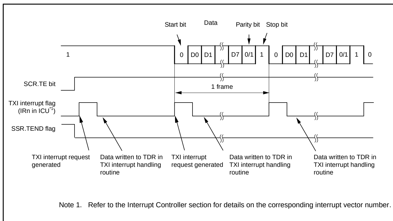
Figure 25.8 Example of Operation for Serial Transmission in Asynchronous Mode (1) (with 8-Bit Data, Parity, 1 Stop Bit, CTS Function Not Used, at the Beginning of Transmission)
