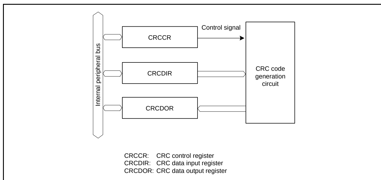
Figure 28.1 CRC Block Diagram
