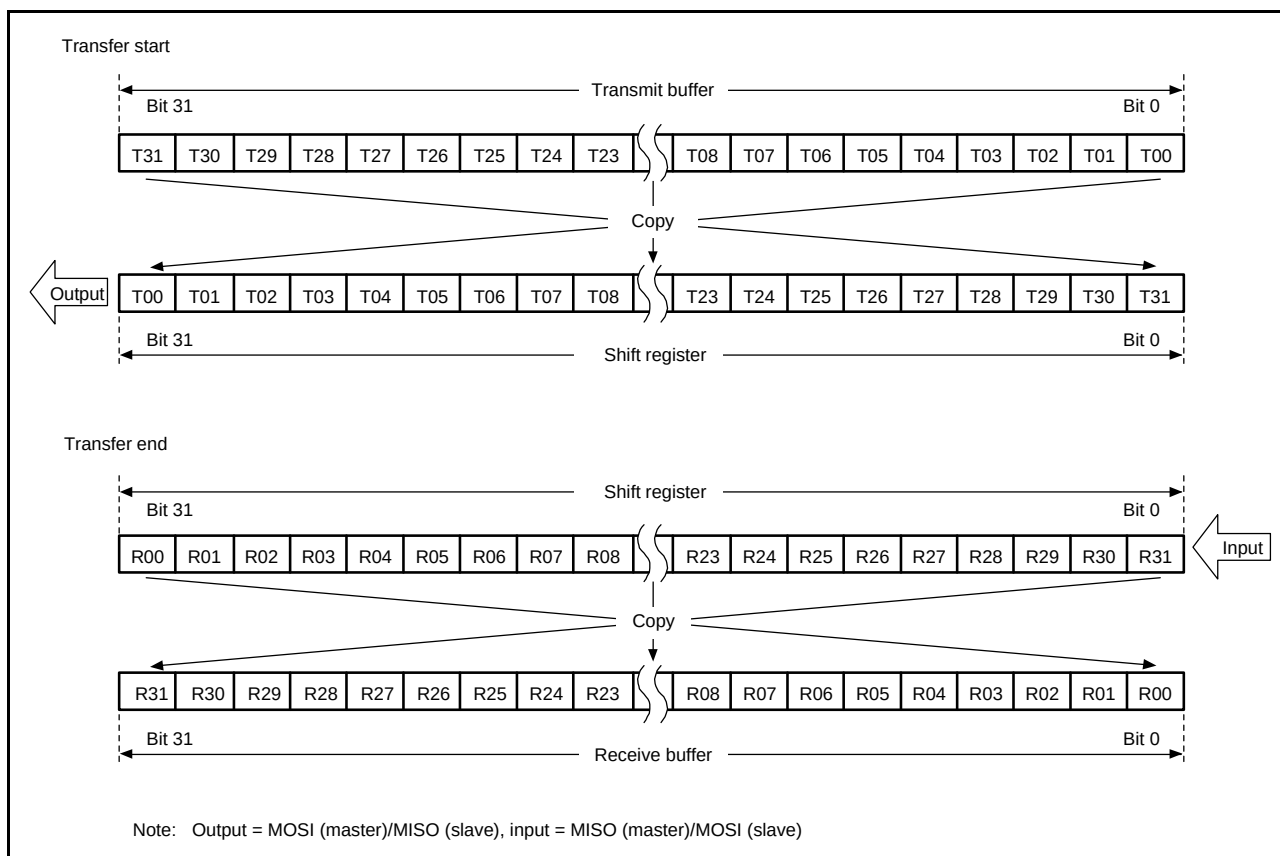
Figure 27.16 LSB First Transfer (32-Bit Data, Parity Disabled)
