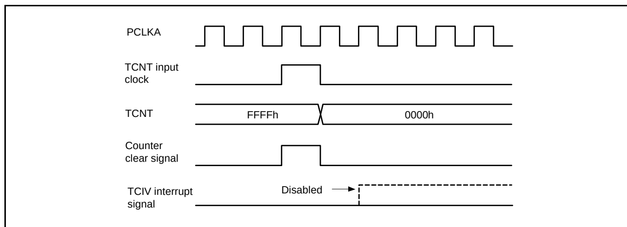
Figure 20.136 Contention between Overflow and Counter Clearing
