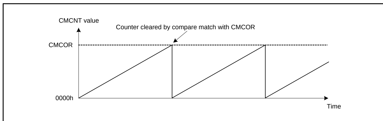
Figure 23.2 CMCNT Counter Operation
