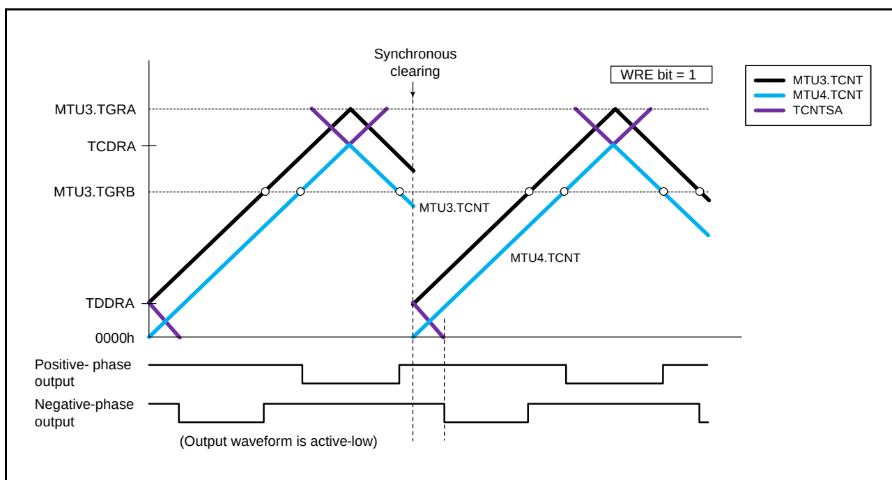
Figure 20.67 Example of Synchronous Clearing in Dead Time during Down-Counting (Timing (8) in Figure 20.63; TWCRA.WRE Bit is 1)
