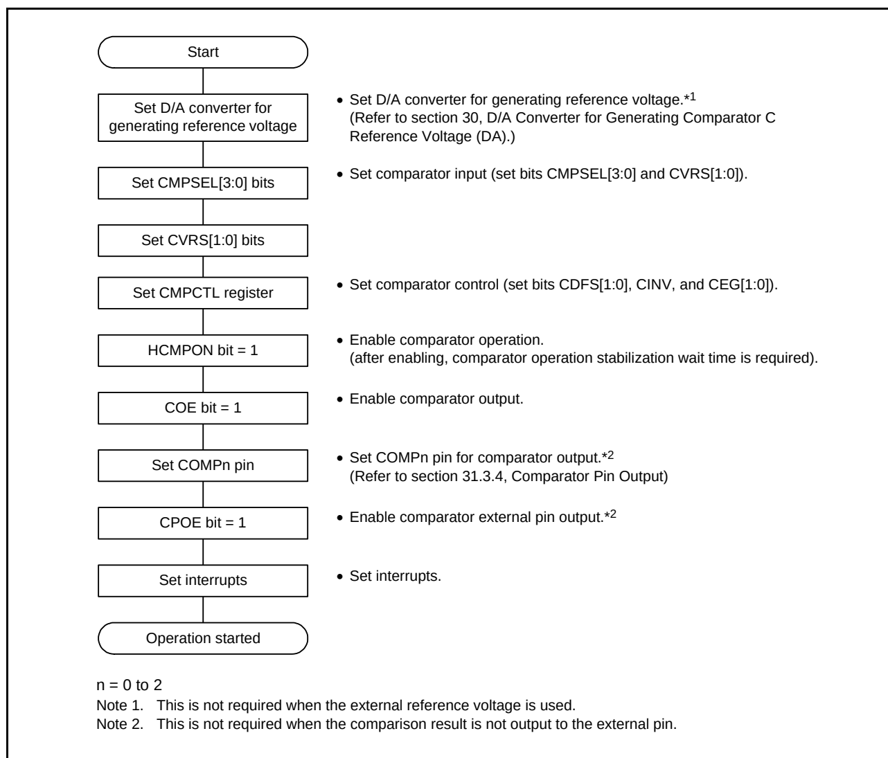
Figure 31.5 Comparator Operation Setting Flowchart
