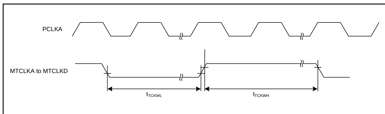
Figure 35.36 MTU3 Clock Input Timing
