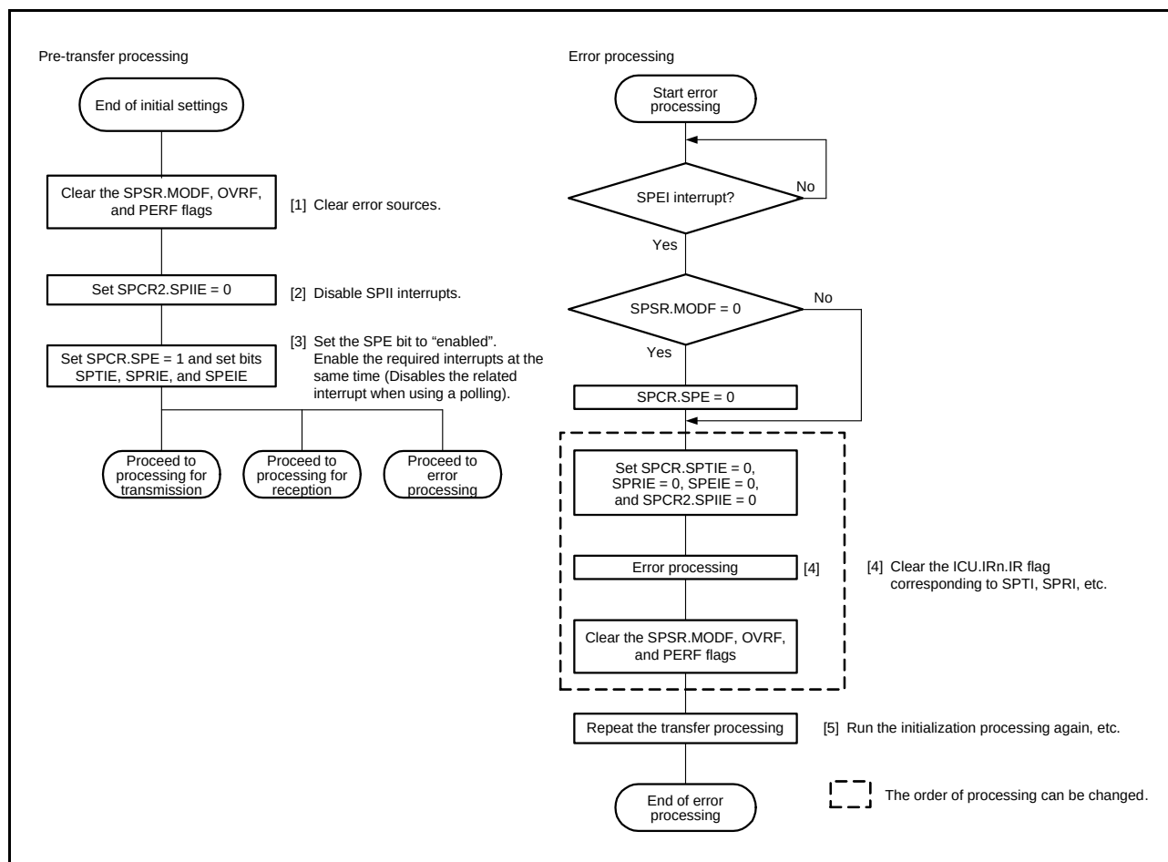
Figure 27.42 Flowchart for Slave Mode (Error Processing)
