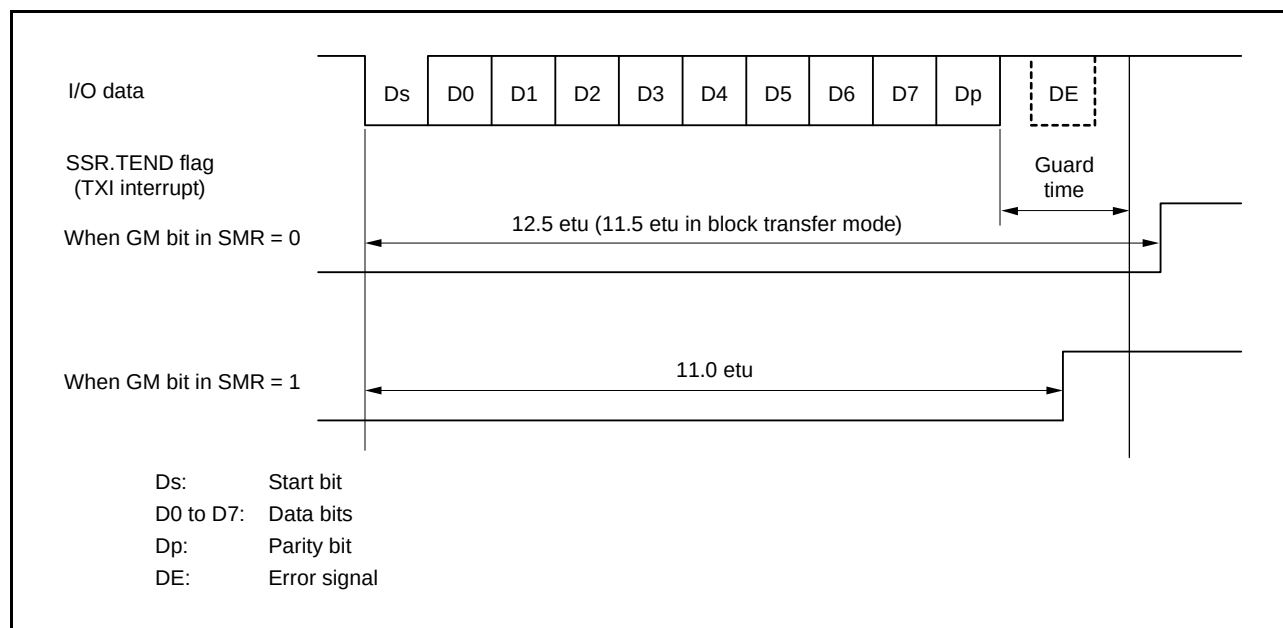
Figure 25.38 SSR.TEND Flag Generation Timing during Transmission
