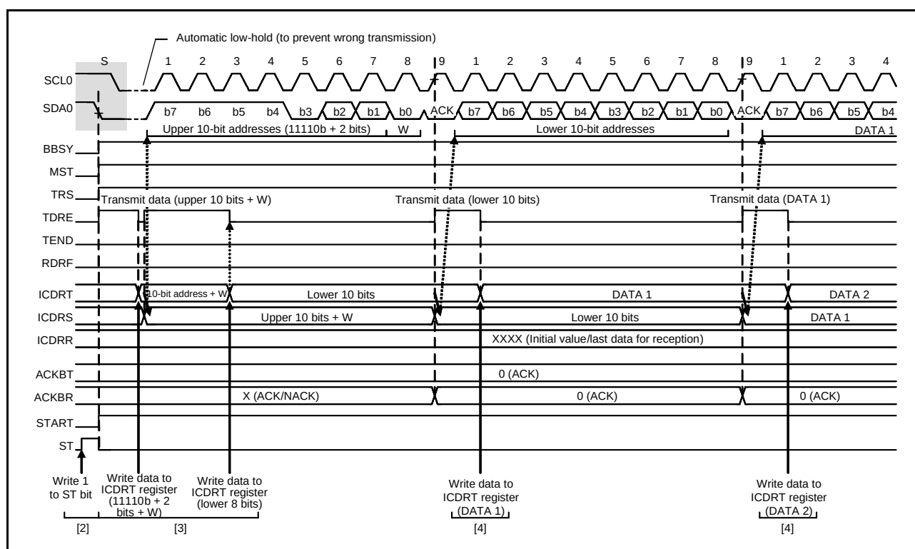
Figure 26.8 Master Transmit Operation Timing (2) (10-Bit Address Format)
