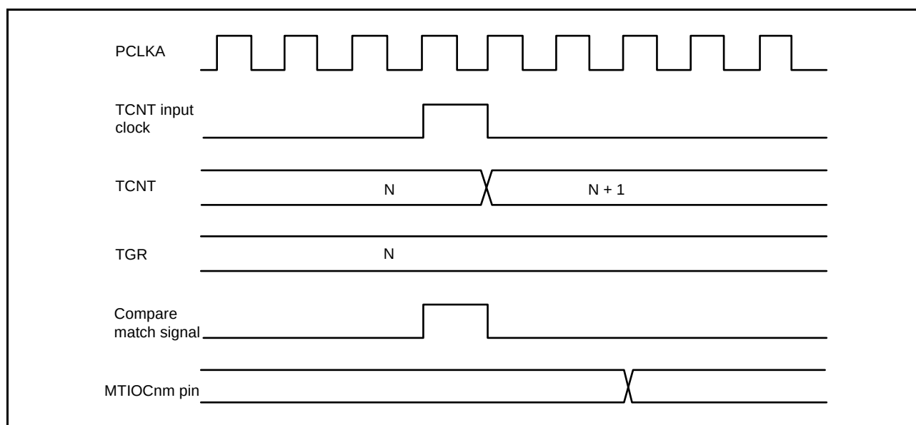
Figure 20.105 Output Compare Output Timing (Complementary PWM Mode or Reset-Synchronized PWM Mode) ( n = 0 to 4 ; m = A to D )
