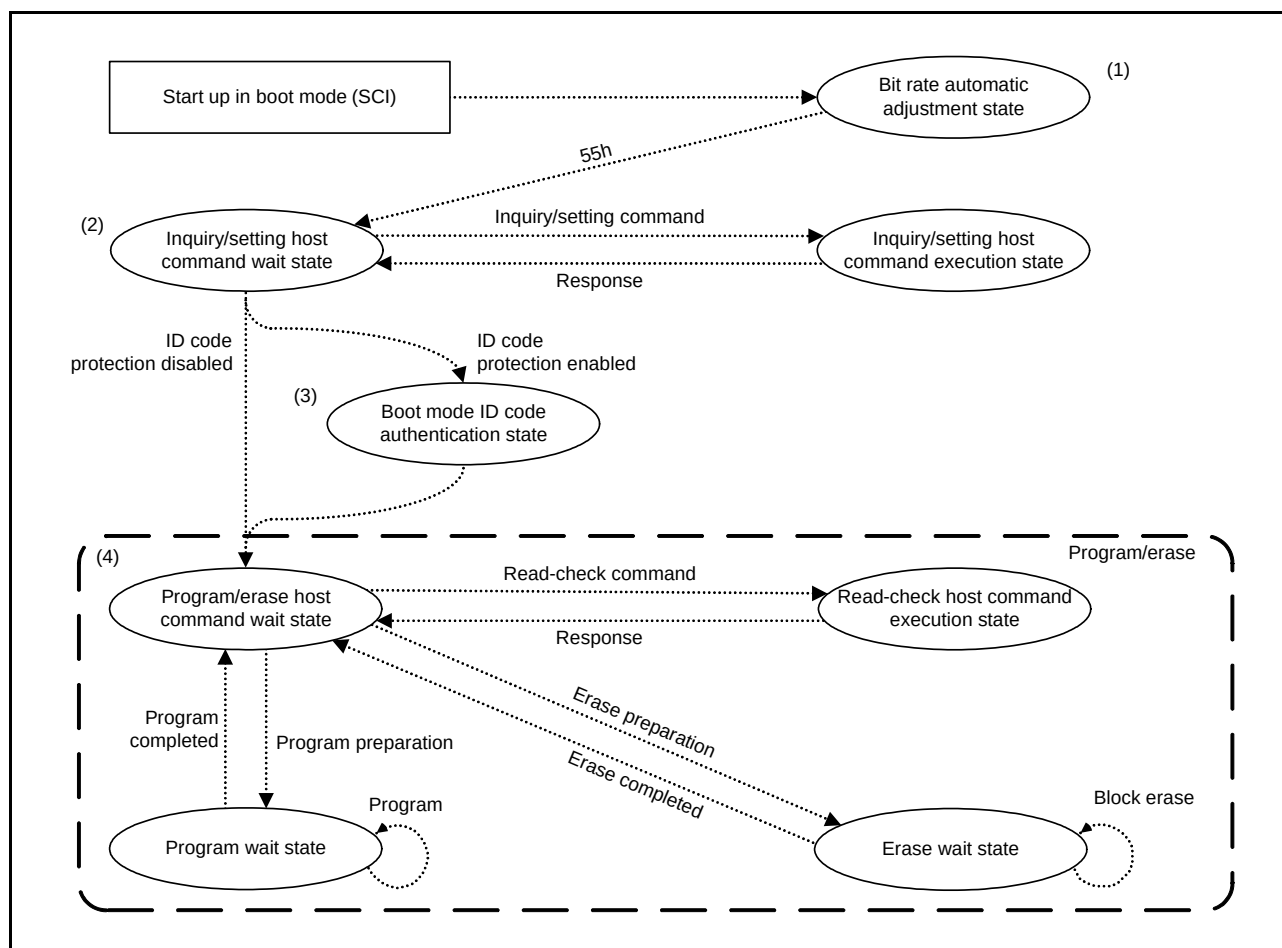
Figure 34.20 Boot Mode (SCI) State Transition
