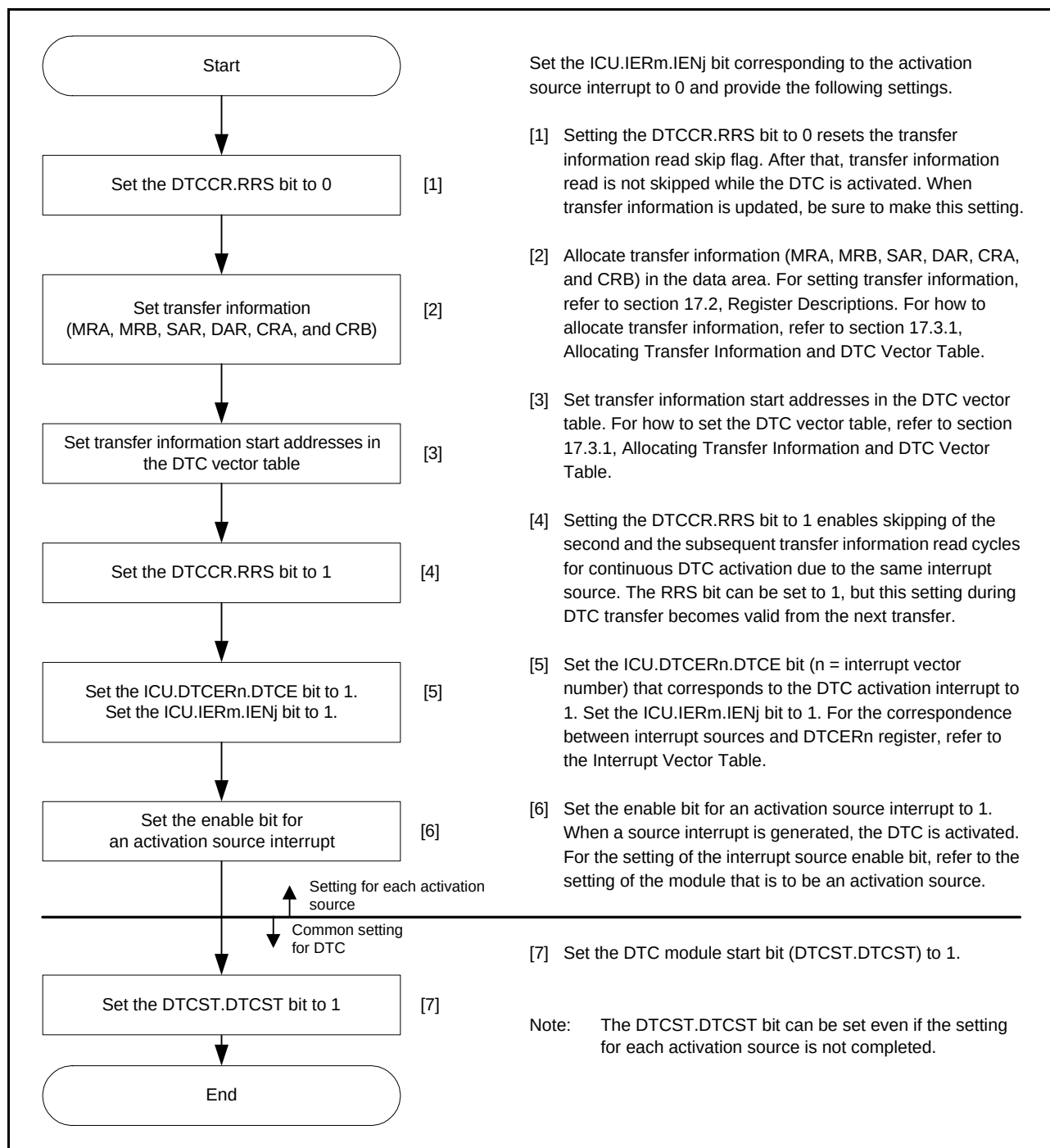
Figure 17.14 Procedure to Set the DTC
