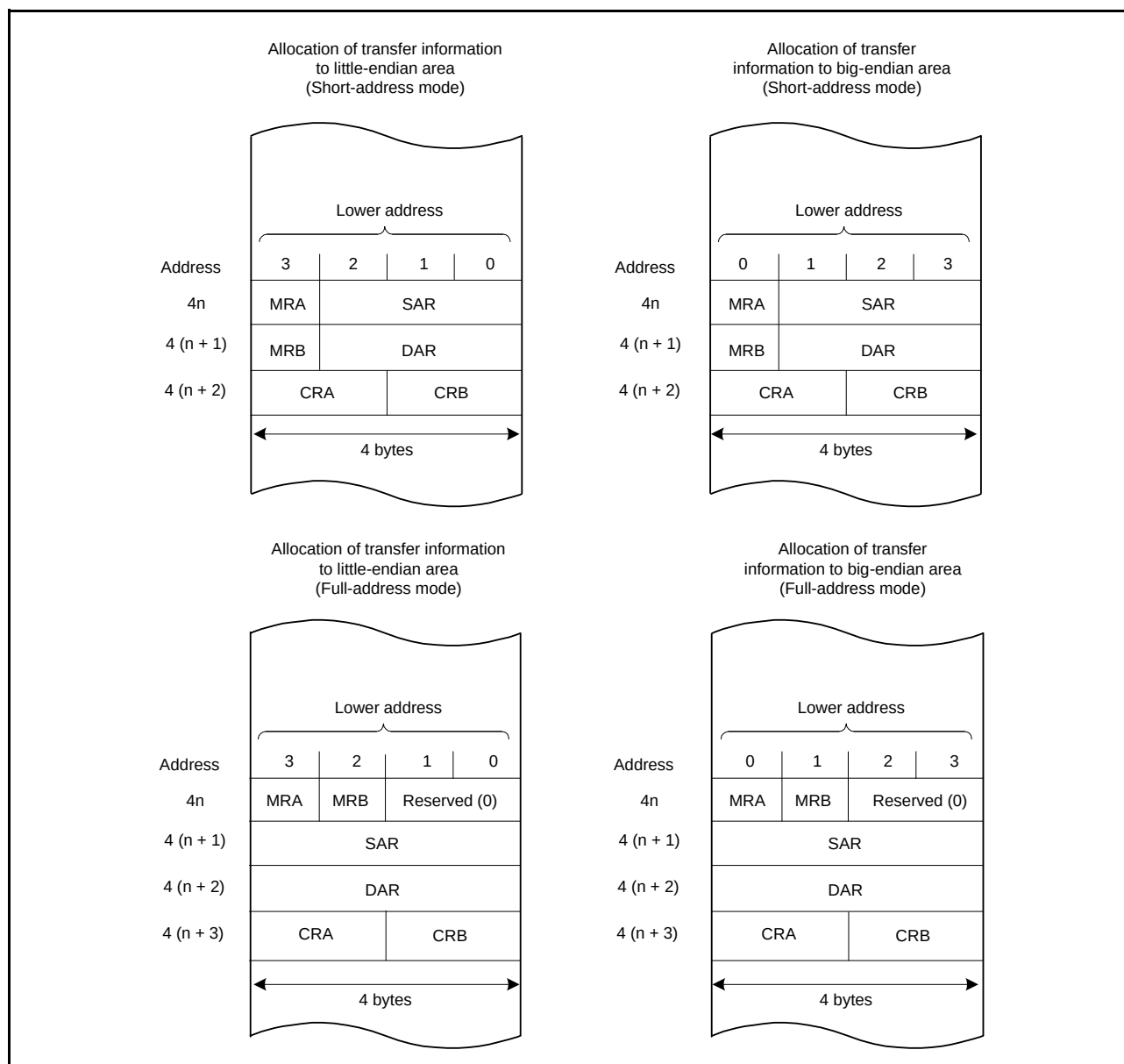
Figure 17.16 Allocation of Transfer Information
