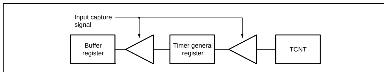
Figure 20.15 Input Capture Buffer Operation
