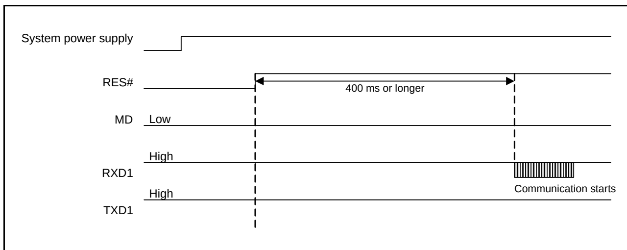
Figure 34.16 Pin States until Communication Becomes Possible in Boot Mode (SCI)
