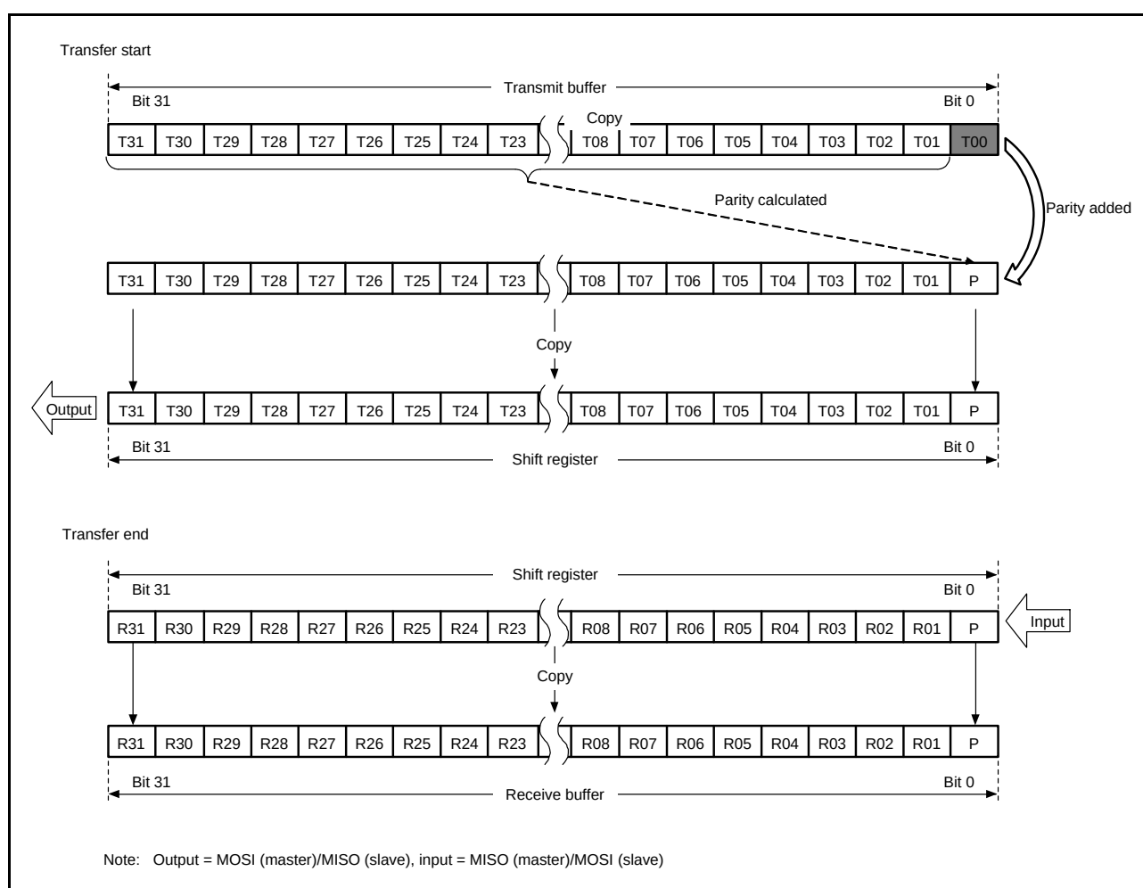
Figure 27.18 MSB First Transfer (32-Bit Data, Parity Enabled)
