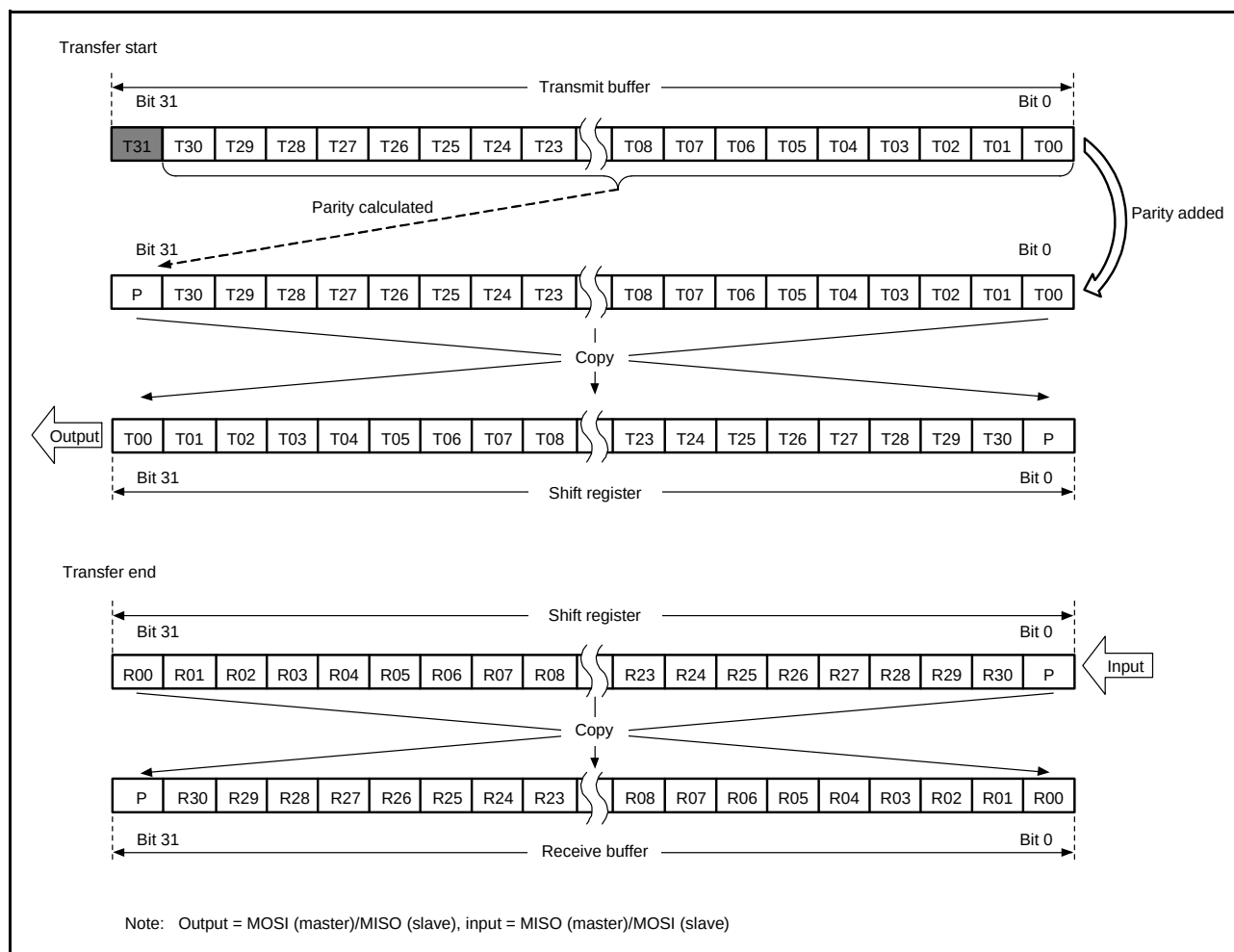
Figure 27.20 LSB First Transfer (32-Bit Data, Parity Enabled)
