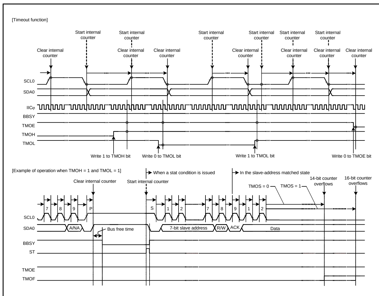
Figure 26.39 Timeout Function
