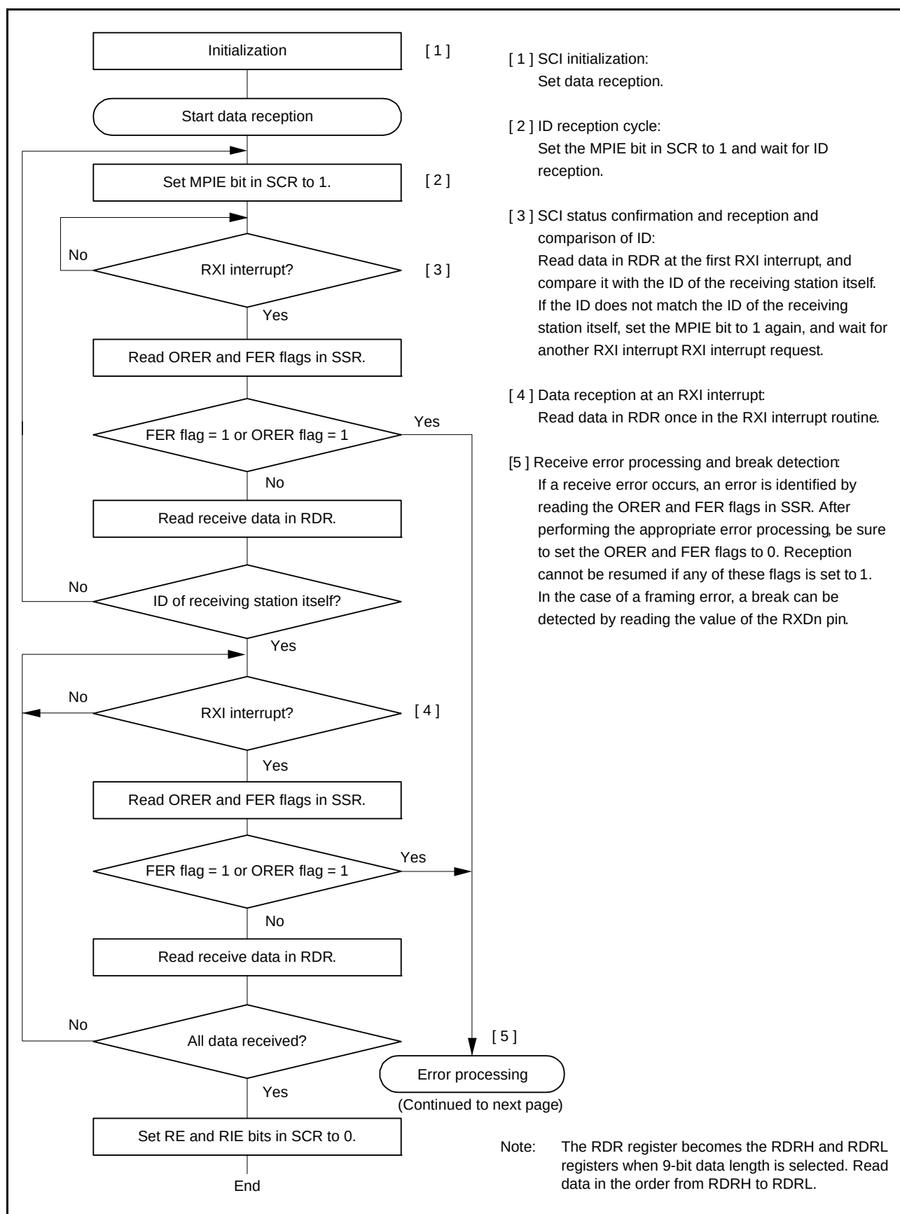
Figure 25.19 Example of Multi-Processor Serial Reception Flowchart (1)
