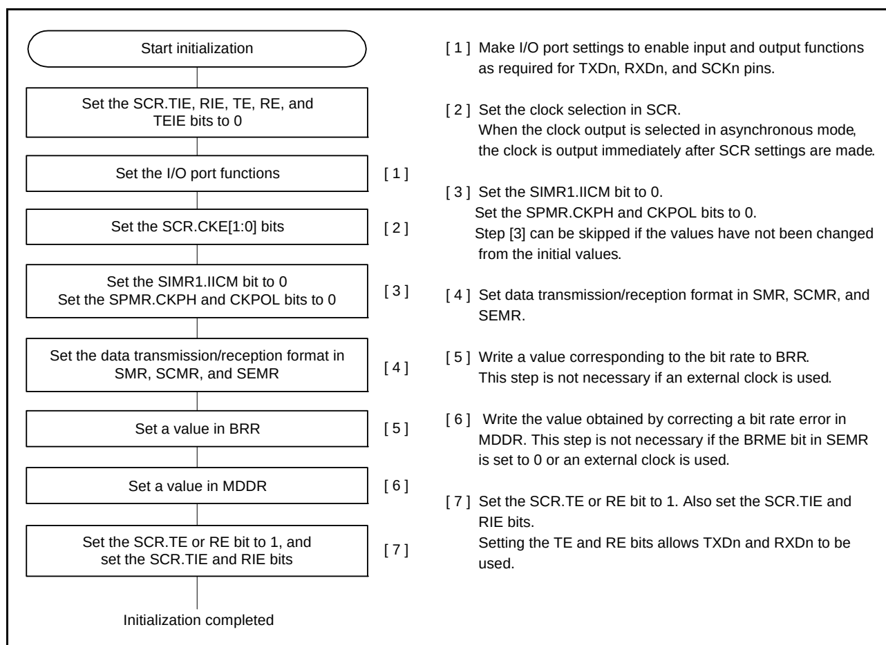
Figure 25.7 Sample SCI Initialization Flowchart (Asynchronous Mode)
