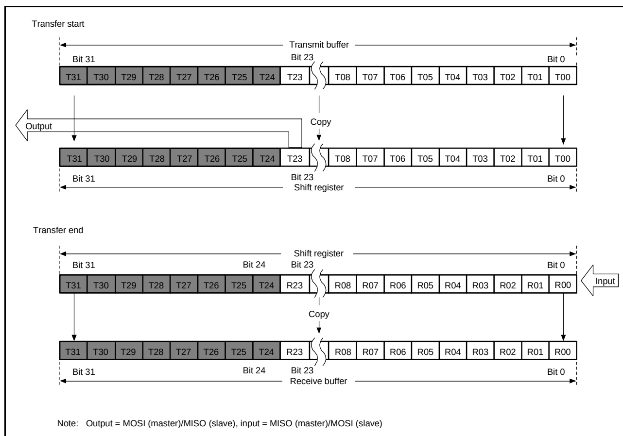
Figure 27.15 MSB First Transfer (24-Bit Data, Parity Disabled)
