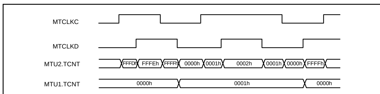
Figure 20.21 Cascaded Operation Example (a)
