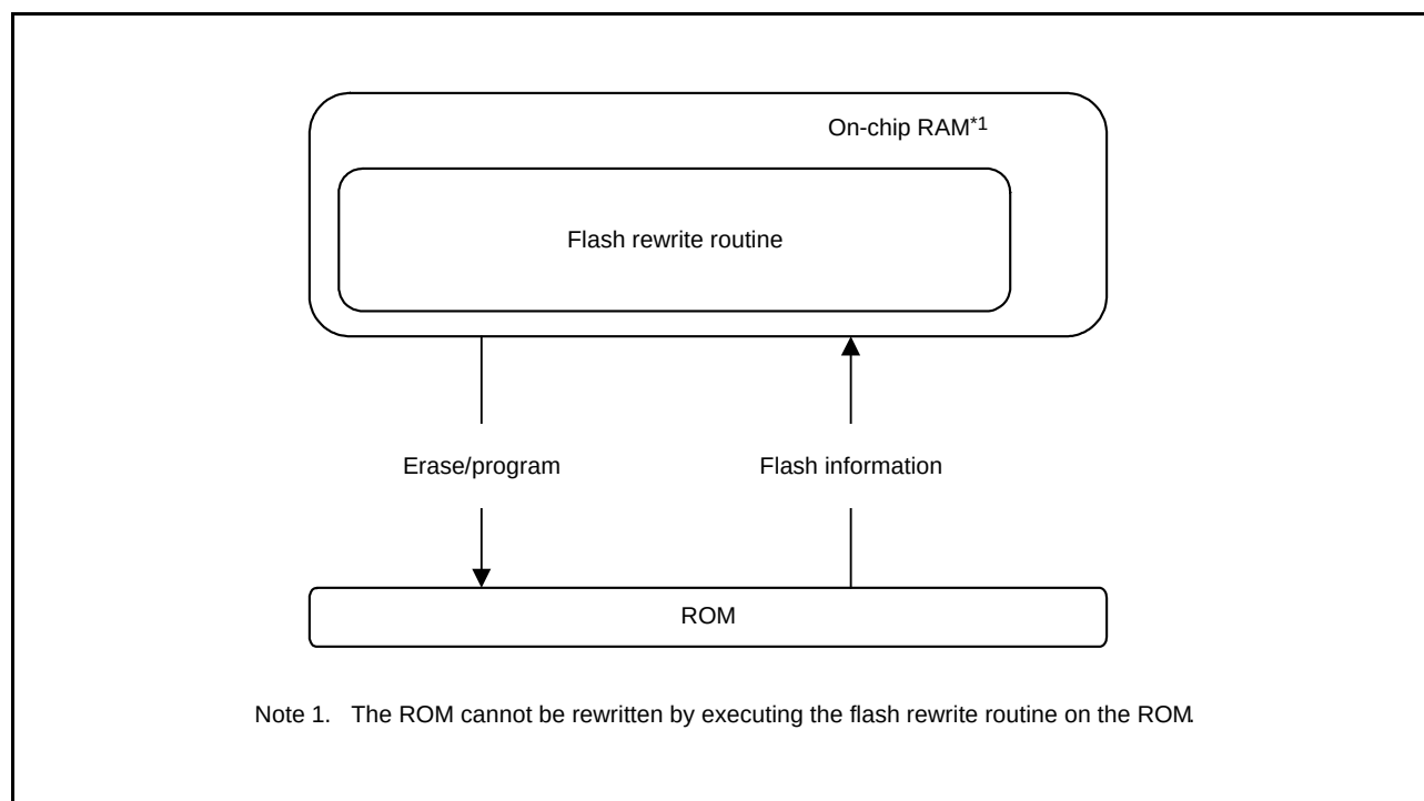
Figure 34.31 Self-Programming Overview
