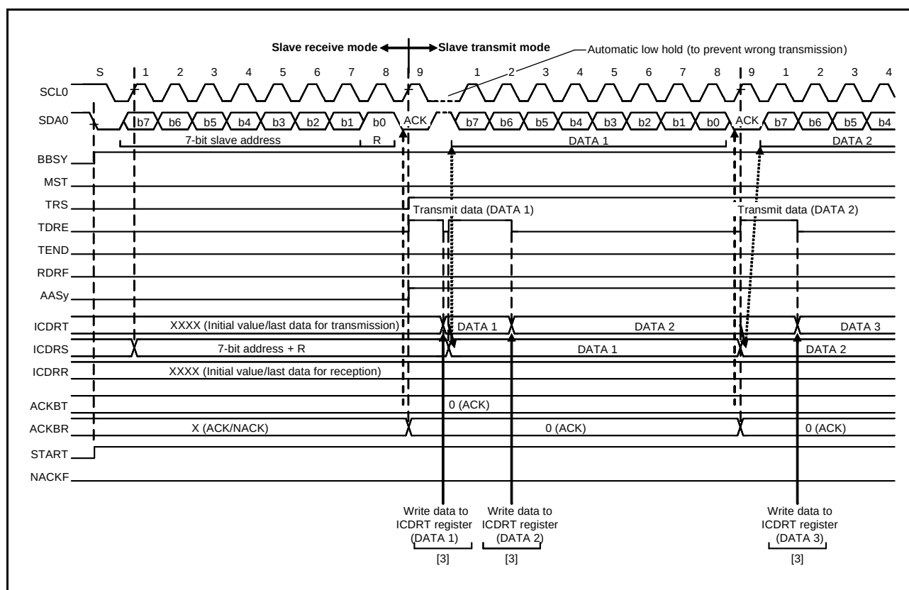
Figure 26.16 Slave Transmit Operation Timing (1) (7-Bit Address Format)
