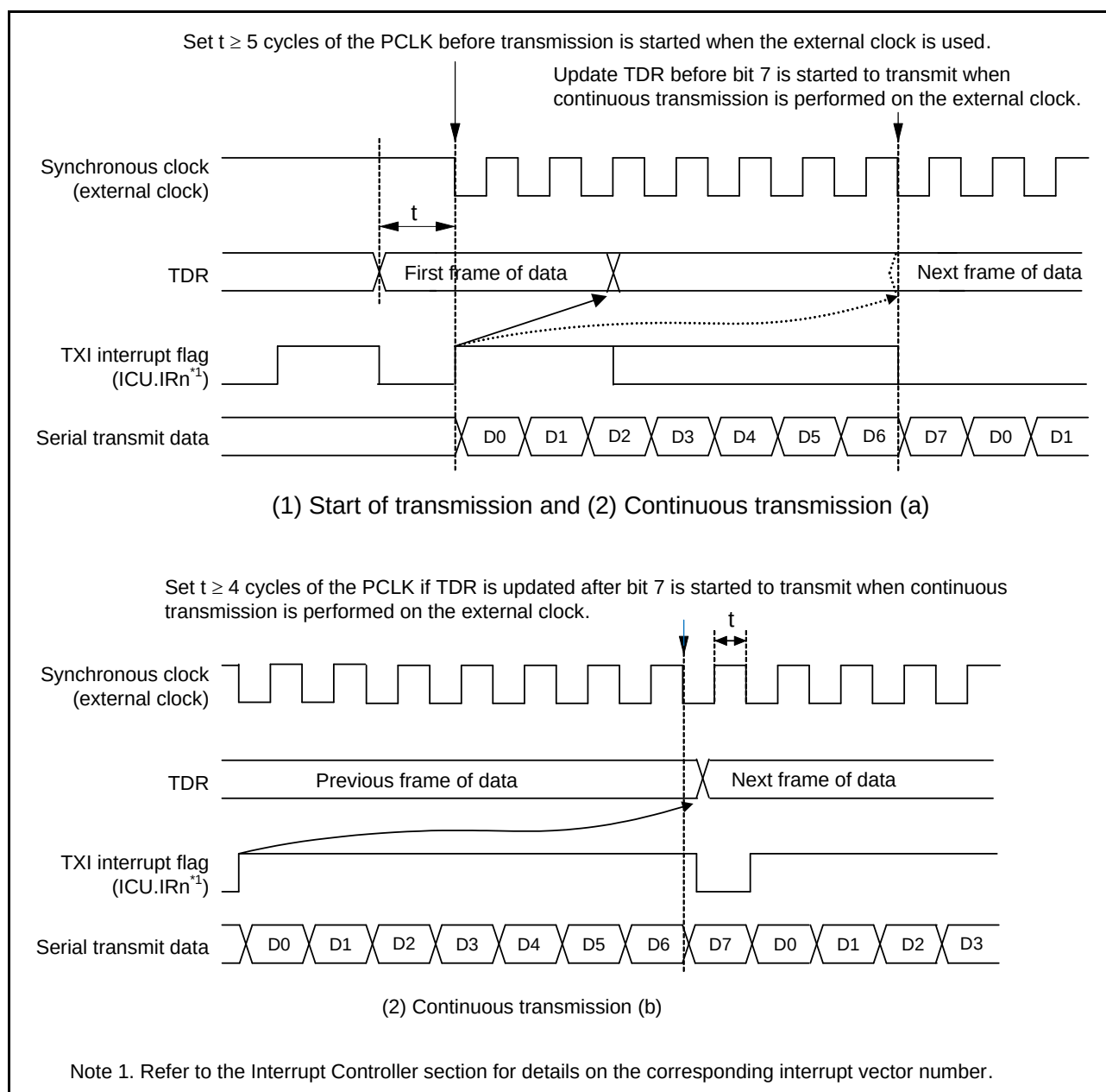
Figure 25.58 Restrictions on Use of External Clock in Clock Synchronous Transmission
