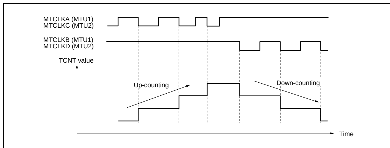
Figure 20.34 Example of Operation in Phase Counting Mode 3 (When MTUn.TCR2.PCB[1:0] = 00b ( n = 1, 2 ))
