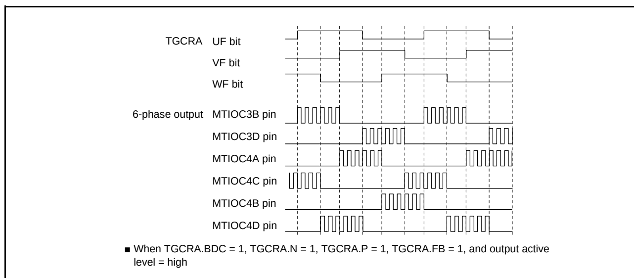
Figure 20.73 Example of Output Phase Switching through UF, VF, and WF Bit Settings (2)
