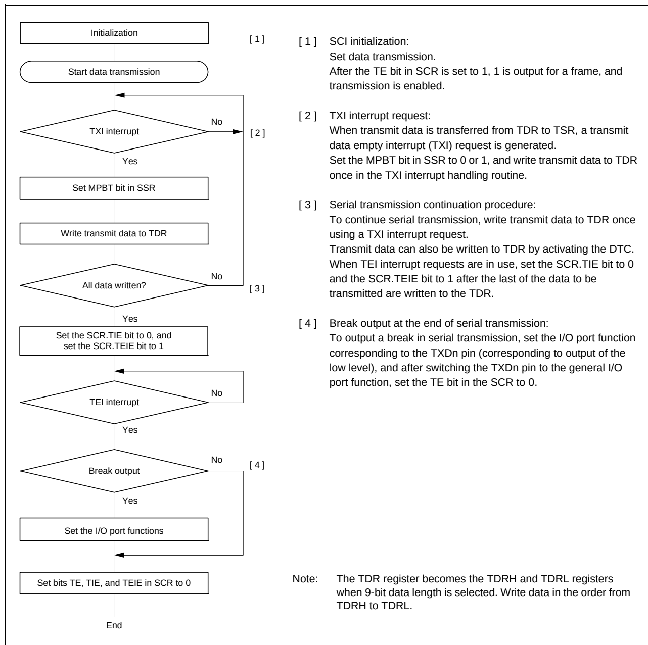
Figure 25.17 Example of Multi-Processor Serial Transmission Flowchart
