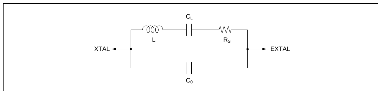
Figure 9.5 Equivalent Circuit of Crystal
