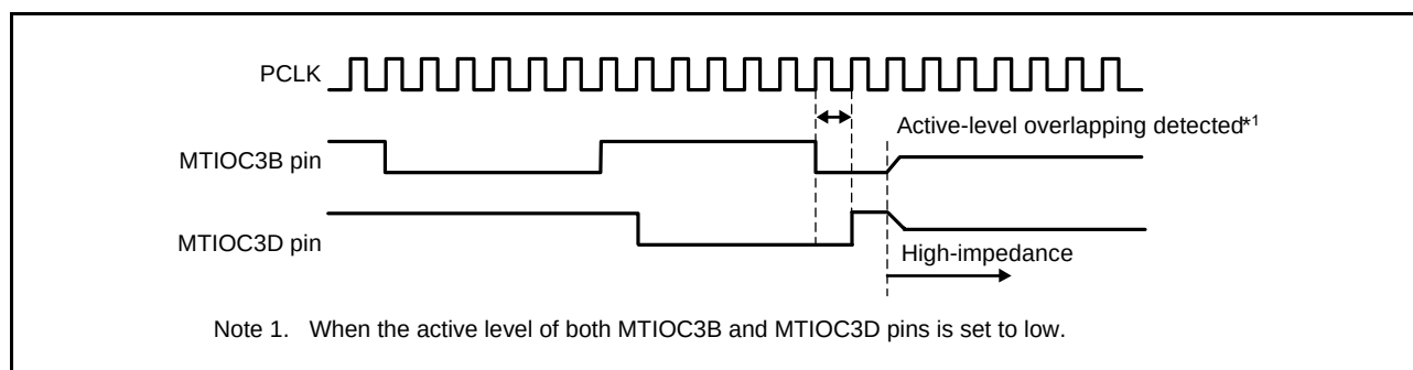
Figure 21.5 Output-Level Compare Operation
