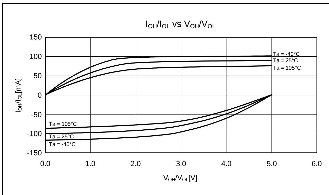
Figure 35.10 V OH /V OL and I OH /I OL Temperature Characteristics at VCC = 5.0 V when Normal Output is Selected (Reference Data)
