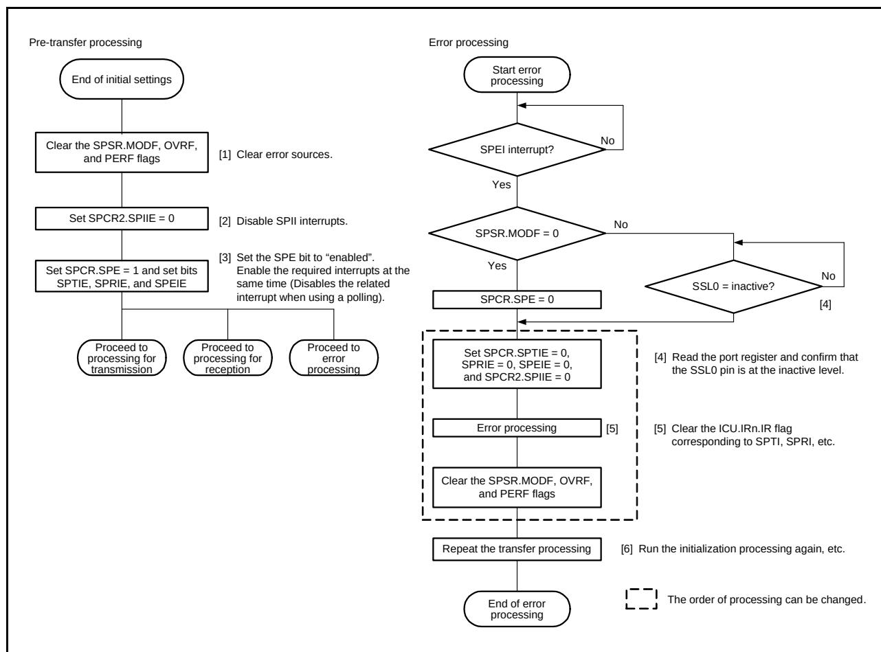
Figure 27.38 Flowchart for Master Mode (Error Processing)
