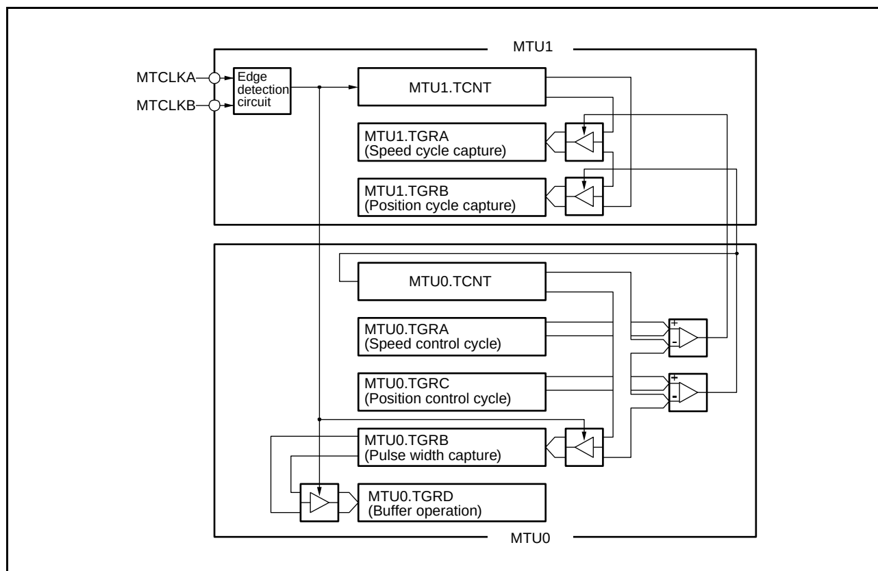
Figure 20.40 16-Bit Phase Counting Mode Application Example
