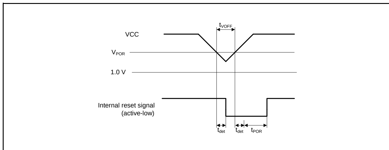
Figure 35.50 Voltage Detection Reset Timing
