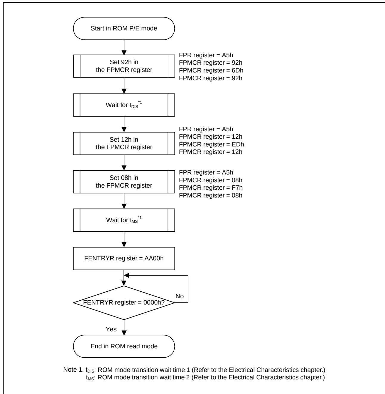
Figure 34.7 Procedure for Transition from ROM P/E Mode to ROM Read Mode
