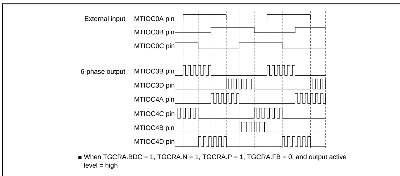
Figure 20.71 Example of Output Phase Switching by External Input (2)
