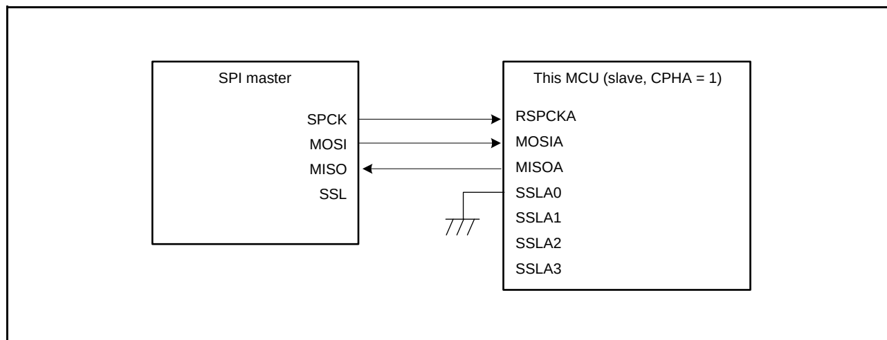
Figure 27.7 Single-Master/Single-Slave Configuration Example (This MCU = Slave, CPHA = 1)
