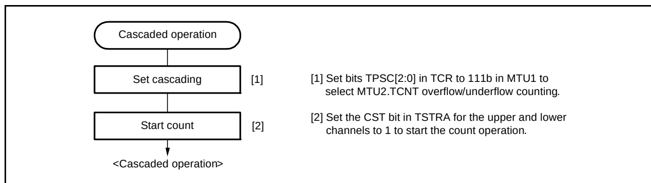
Figure 20.20 Cascaded Operation Setting Procedure
