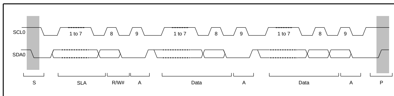
Figure 26.4 I 2 C-bus Timing (SLA = 7 Bits)
