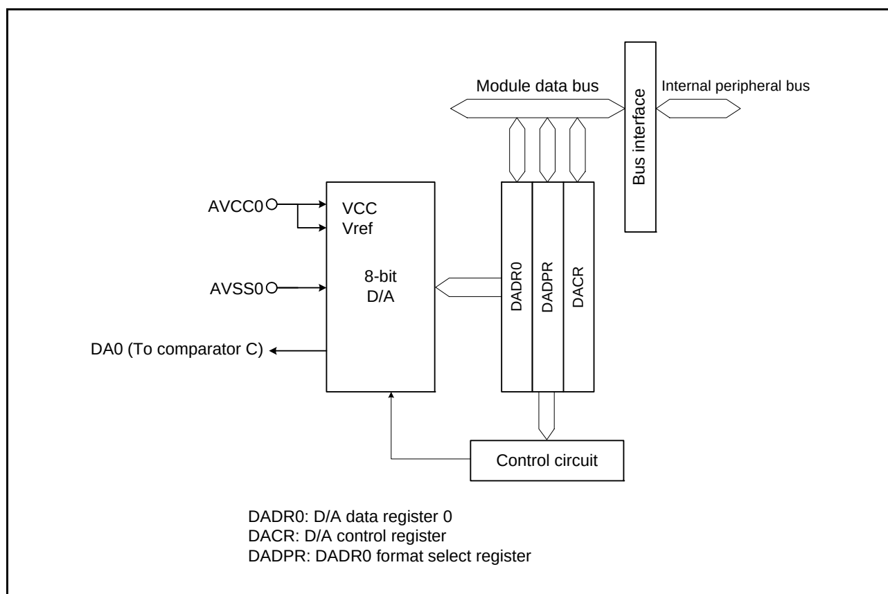
Figure 30.1 Block Diagram of 8-Bit D/A Converter
