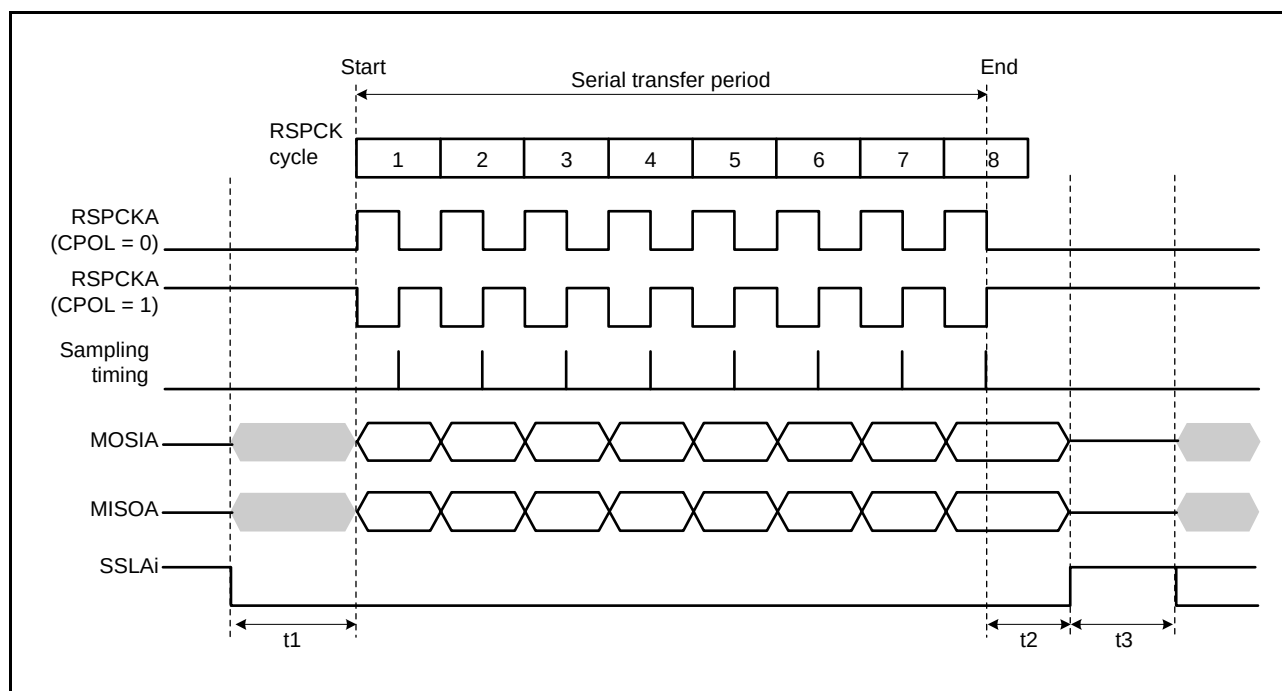
Figure 27.23 RSPI Transfer Format (CPHA = 1)
