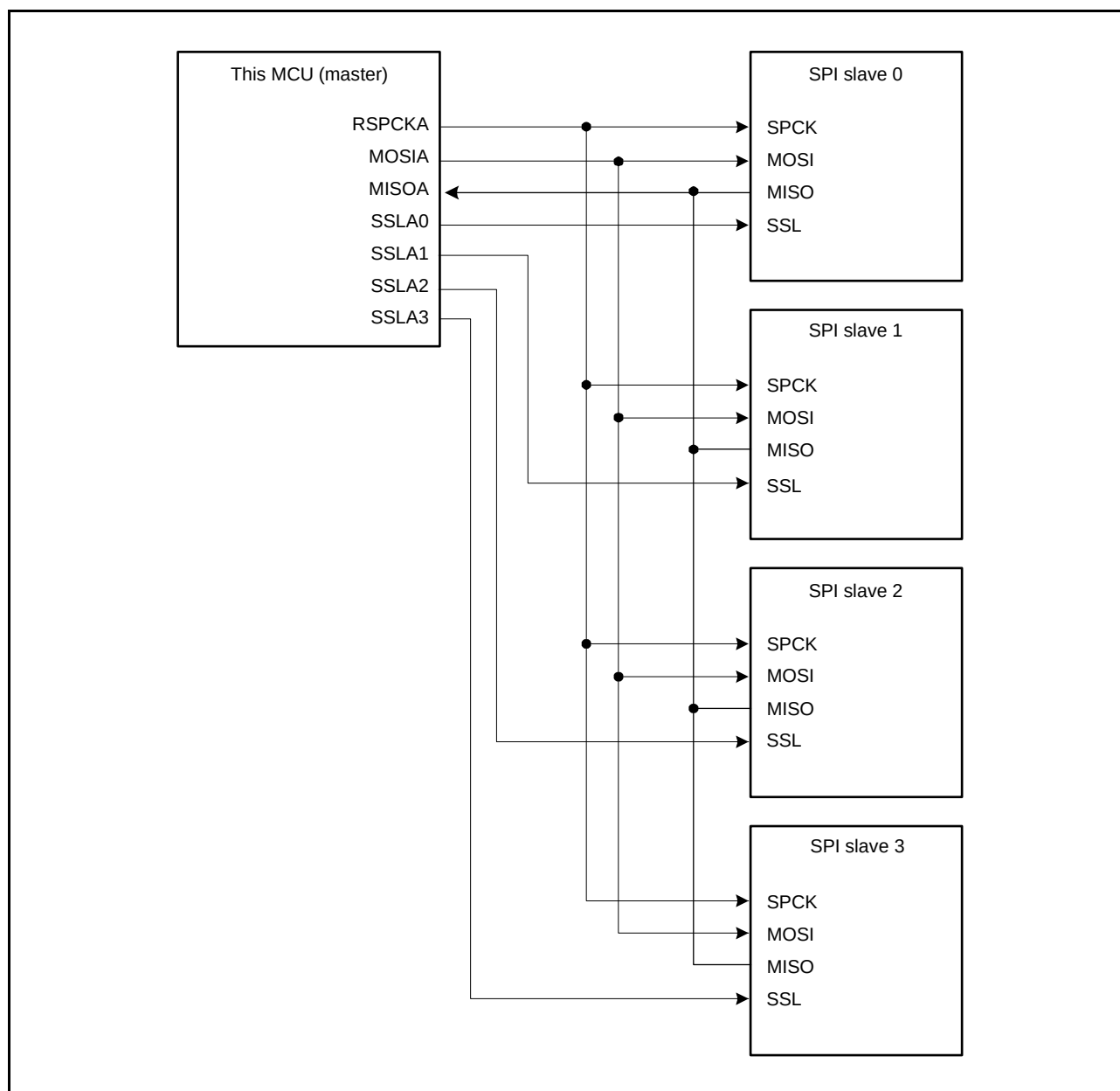
Figure 27.8 Single-Master/Multi-Slave Configuration Example (This MCU = Master)
