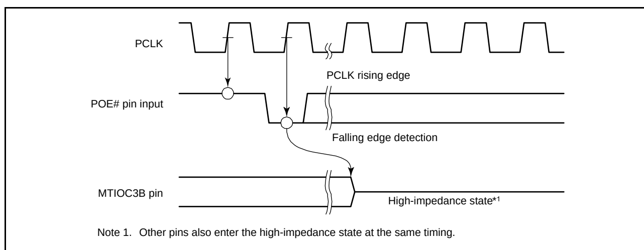
Figure 21.3 Falling Edge Detection
