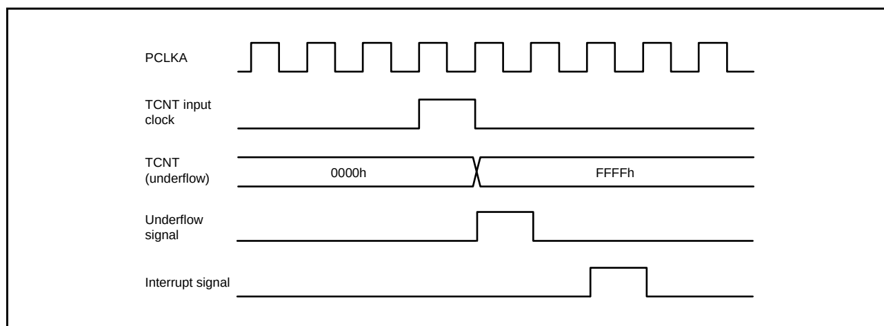
Figure 20.121 TCIU Interrupt Timing
