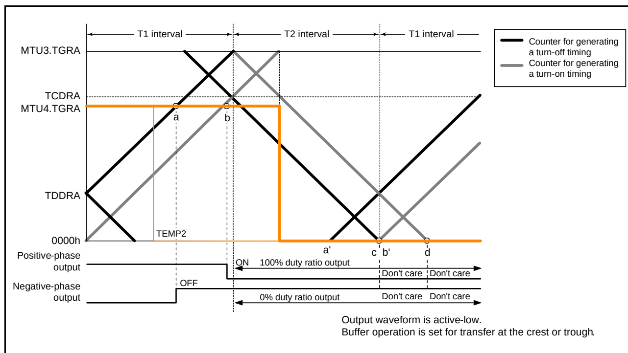
Figure 20.59 Example of 0% and 100% Waveform Output in Complementary PWM Mode (MTU3 and MTU4) (4)
