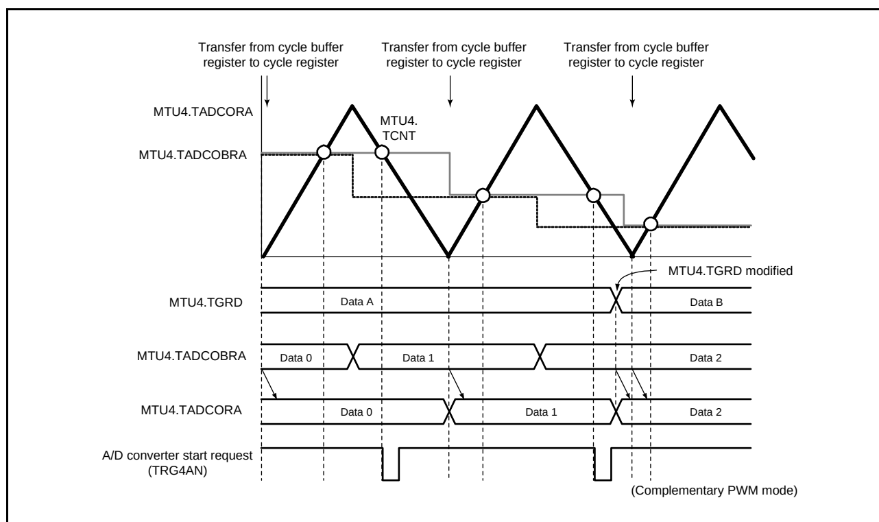
Figure 20.85 Example of A/D Converter Start Request Signal (TRG4AN) and Buffer Transfer Operation
