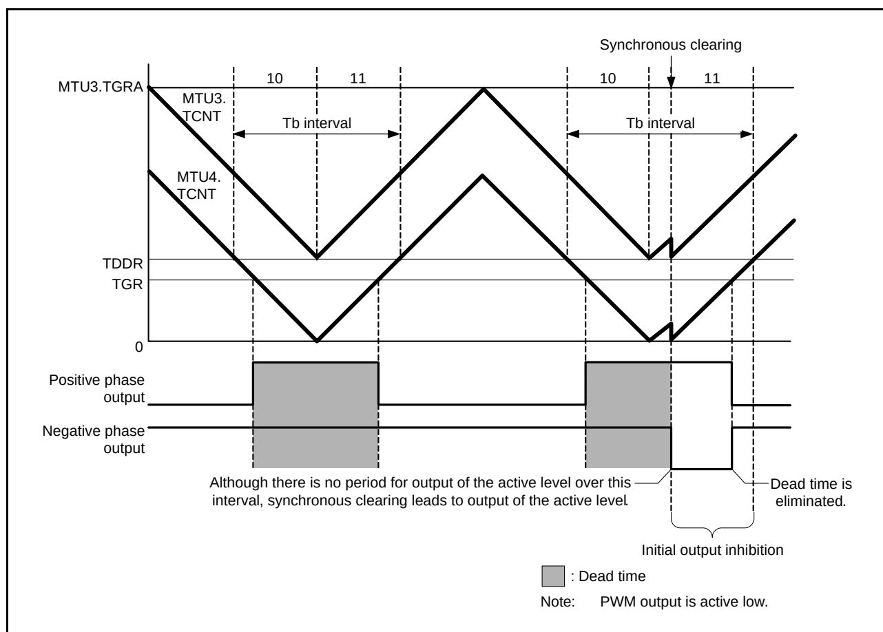
Figure 20.139 Example of Synchronous Clearing (When Condition 2 Applies)
