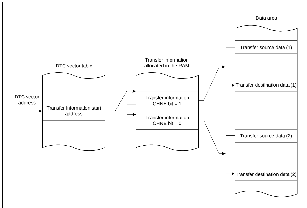
Figure 17.8 Chain Transfer Operation
