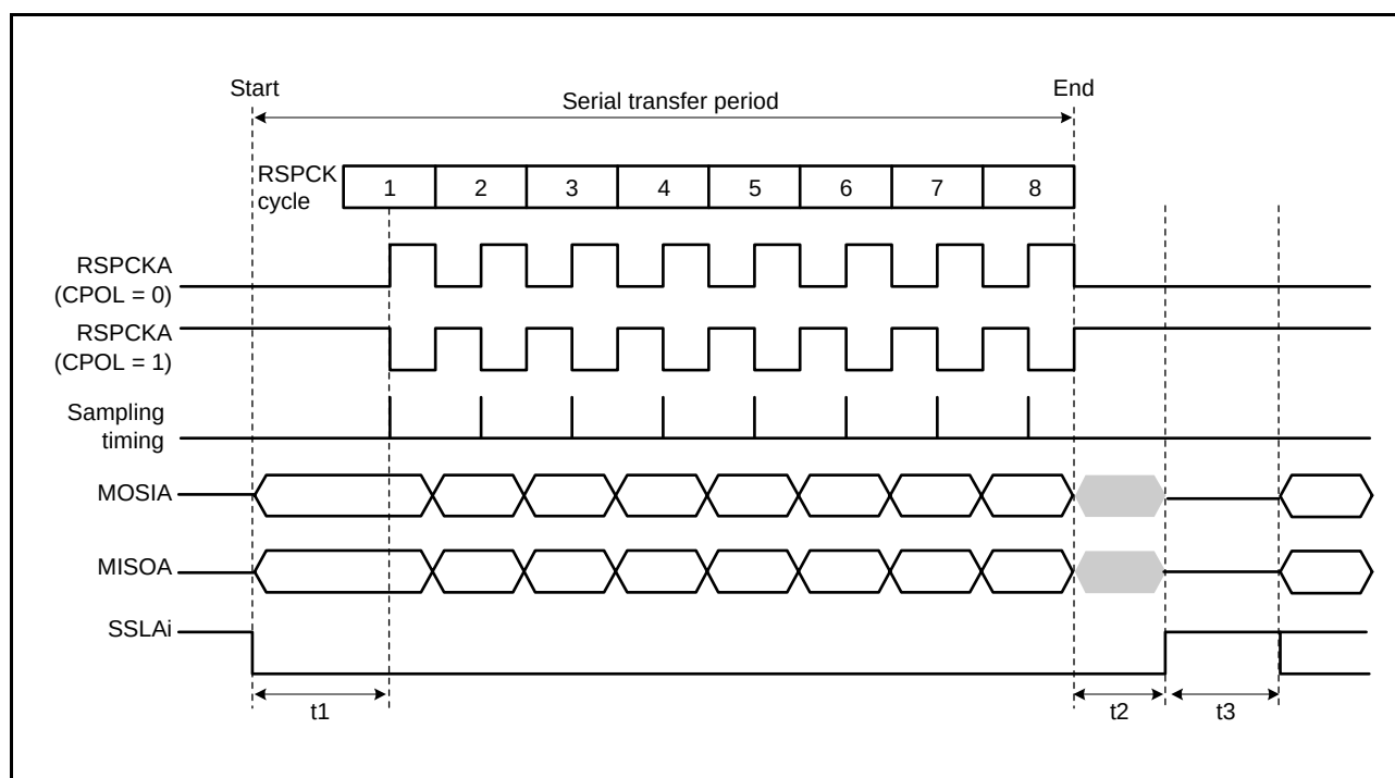
Figure 27.22 RSPI Transfer Format (CPHA = 0)
