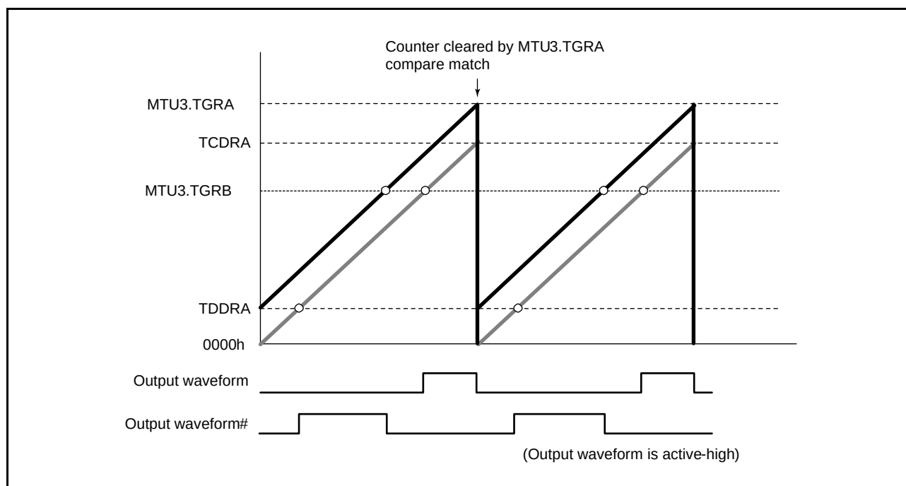
Figure 20.69 Example of Counter Clearing Operation by MTU3.TGRA Compare Match
