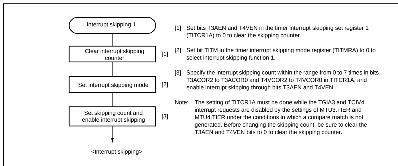
Figure 20.77 Example of Interrupt Skipping Function 1 Setting Procedure
