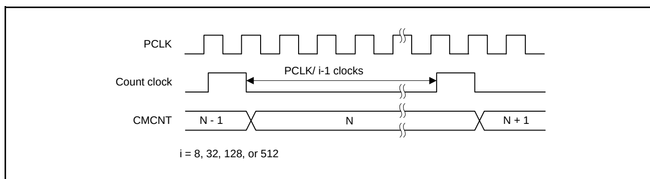
Figure 23.3 CMCNT Count Timing
