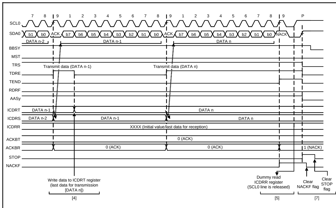
Figure 26.17 Slave Transmit Operation Timing (2)
