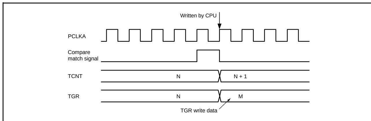
Figure 20.125 Contention between TGR Write Operation and Compare Match
