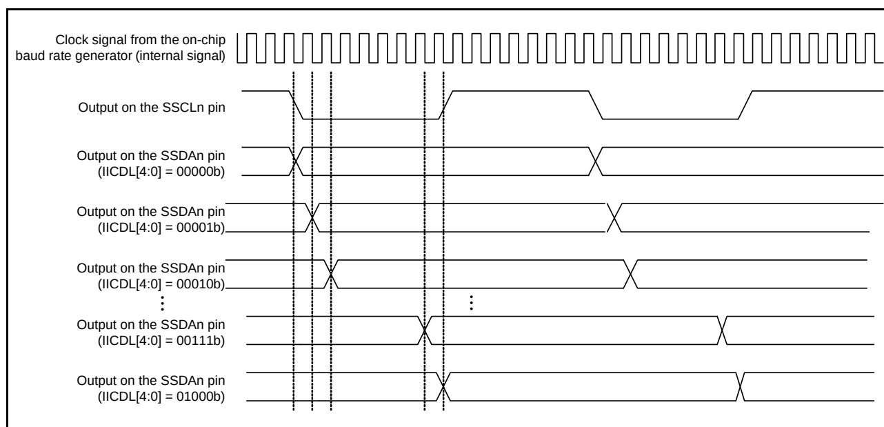
Figure 25.47 Timing of Delays in SSDA Output
