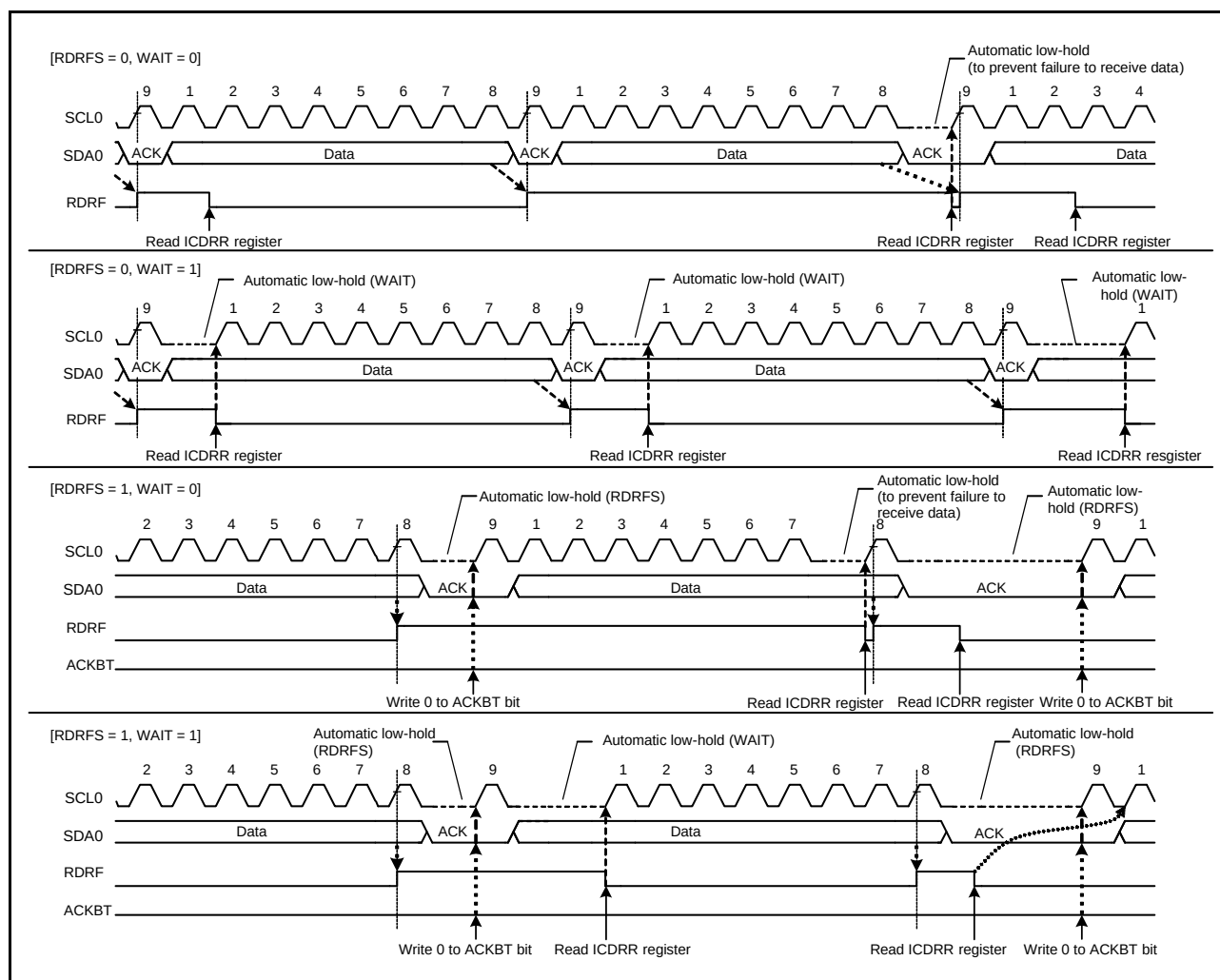
Figure 26.32 Automatic Low-Hold Operation in Receive Mode (Using RDRFS and WAIT Bits)
