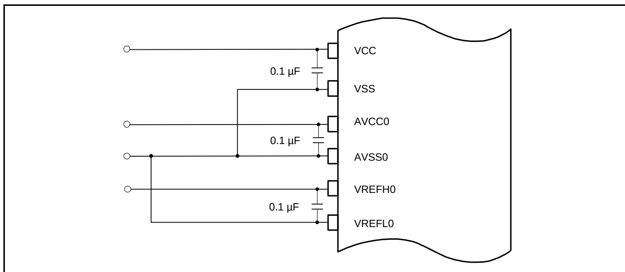
Figure 29.29 Power Supply Pin Connection Example
