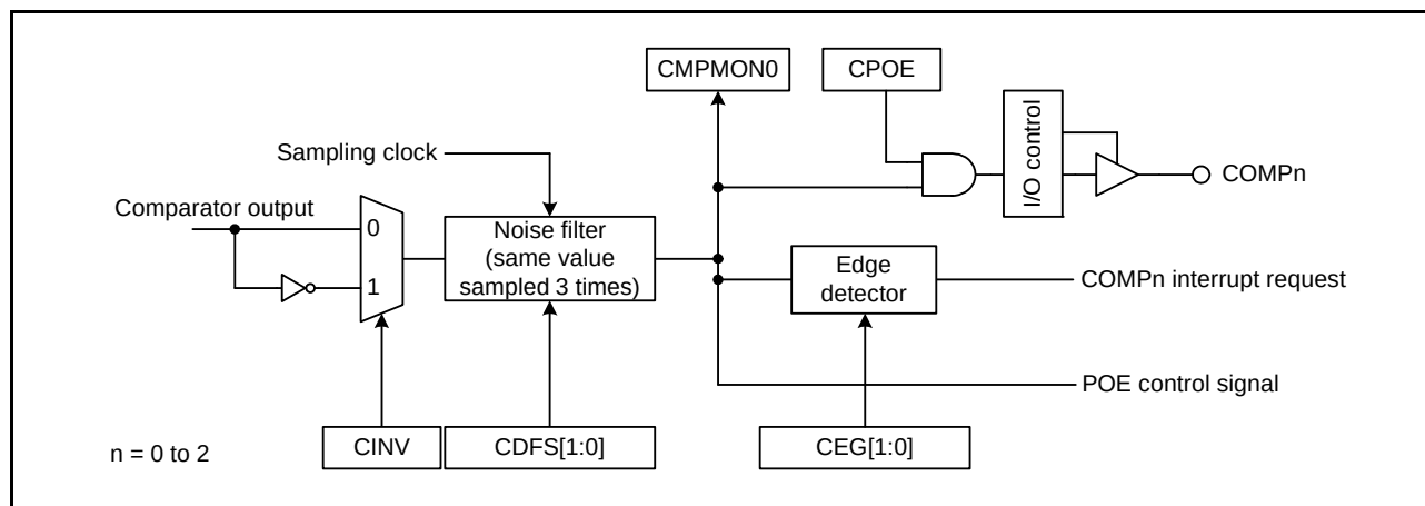
Figure 31.3 Noise Filter and Edge Detector Configuration
