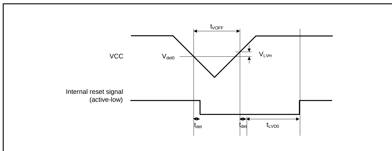
Figure 35.52 Voltage Detection Circuit Timing (Vdet0)
