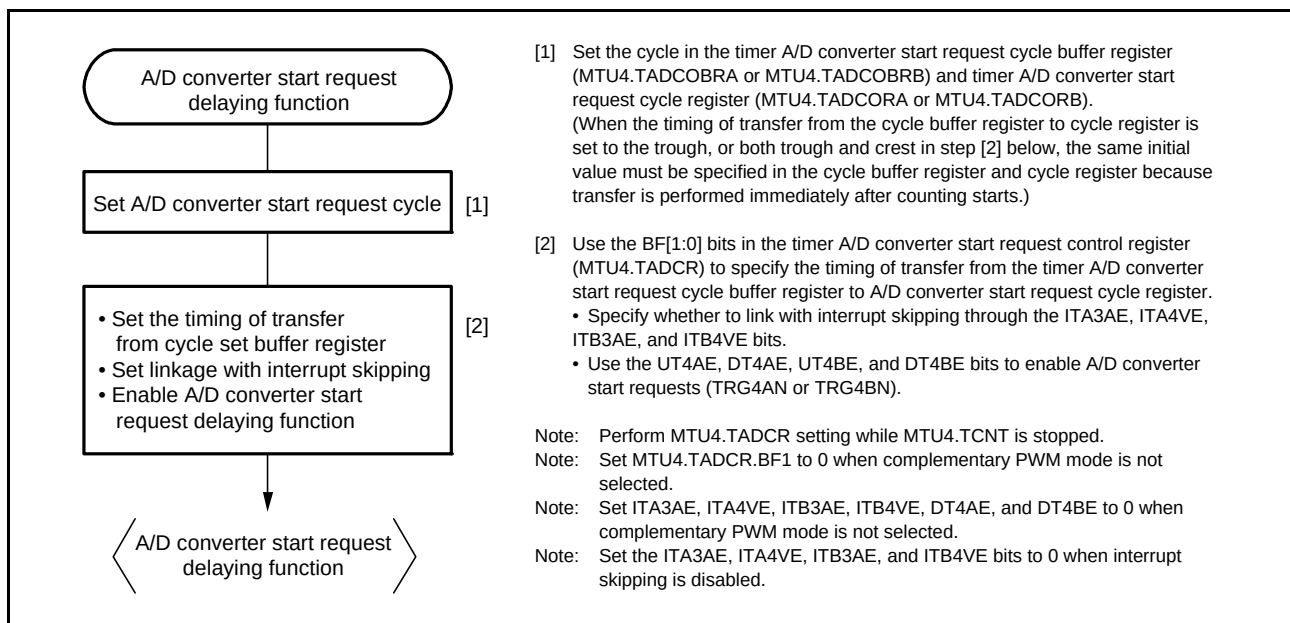
Figure 20.83 Example of Procedure for Specifying A/D Converter Start Request Delaying Function (MTU3 and MTU4)
