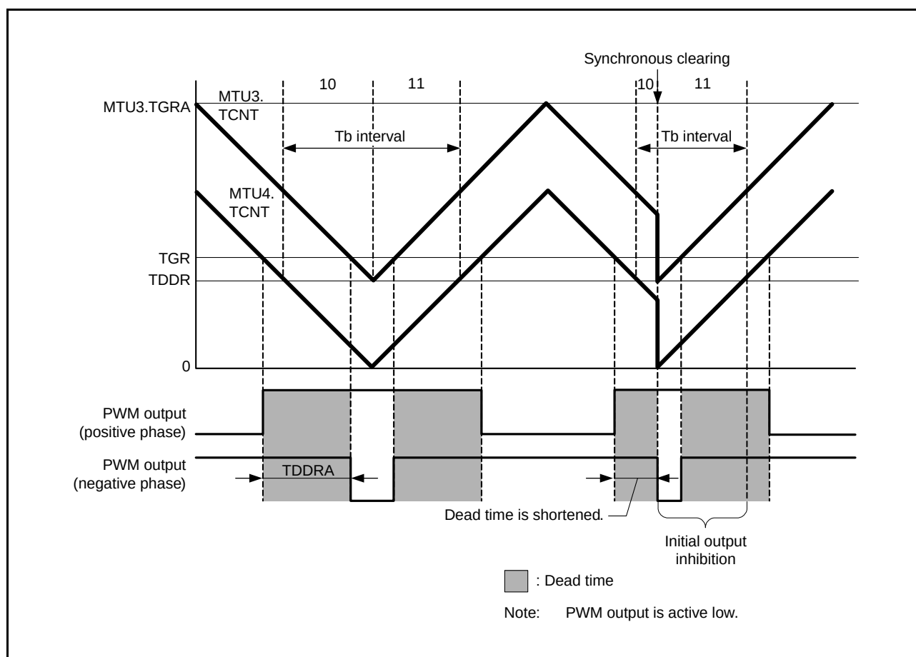
Figure 20.138 Example of Synchronous Clearing (When Condition 1 Applies)
