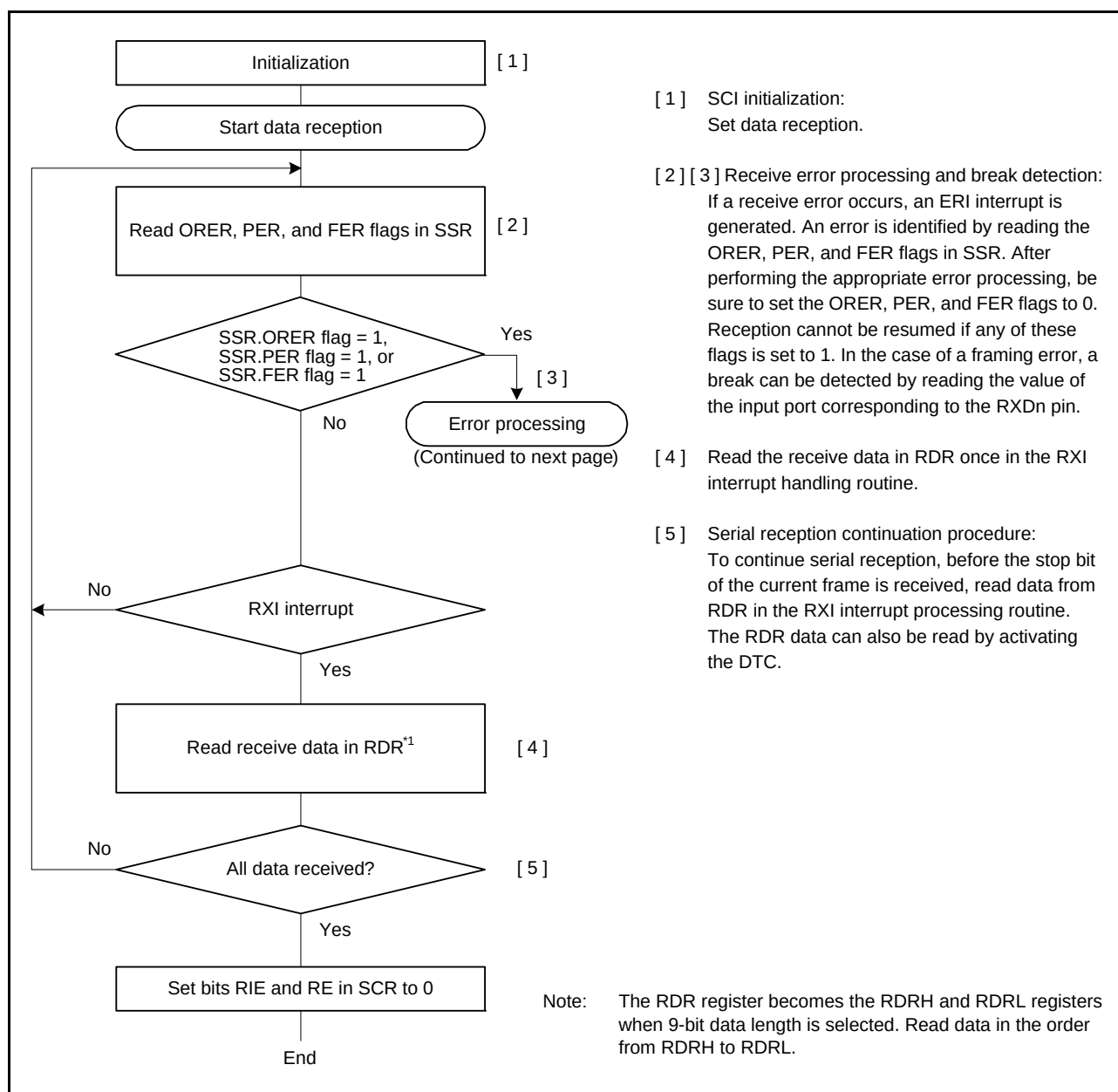
Figure 25.14 Example Flowchart of Serial Reception in Asynchronous Mode (1)
