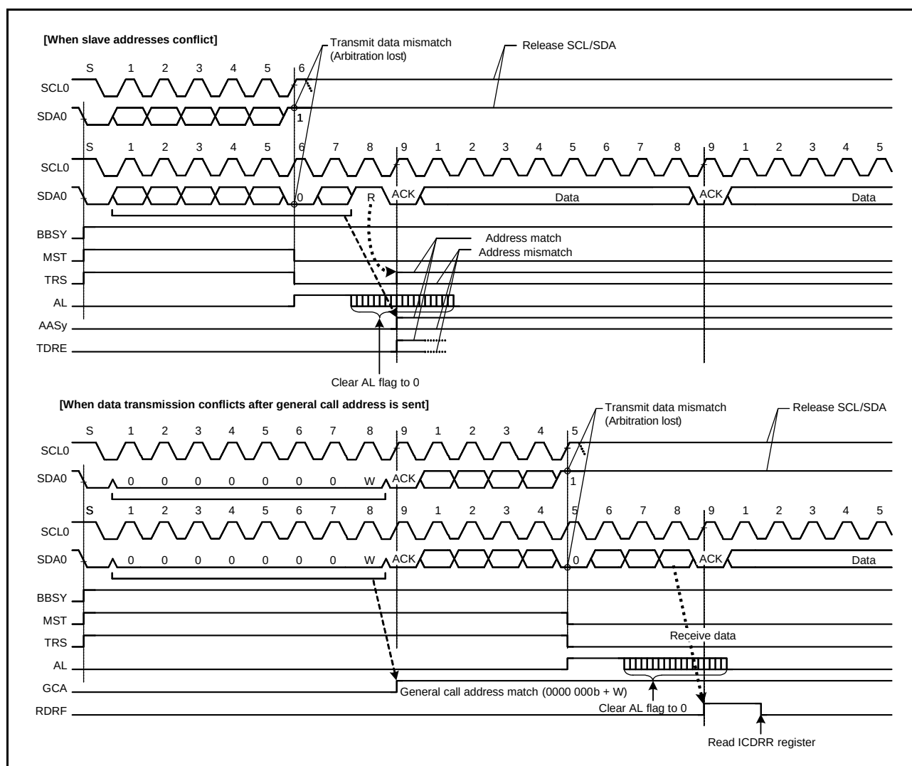
Figure 26.33 Examples of Master Arbitration-Lost Detection (MALE = 1)
