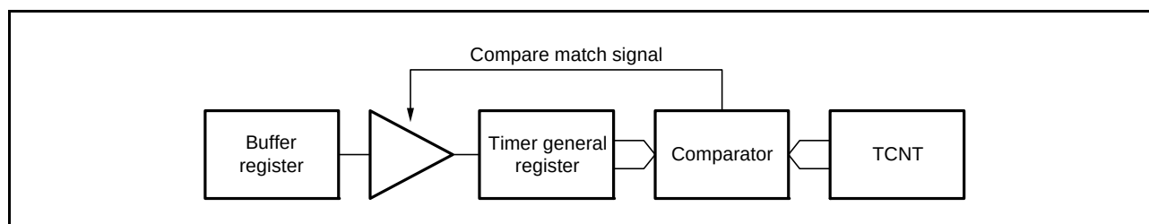
Figure 20.14 Compare Match Buffer Operation
