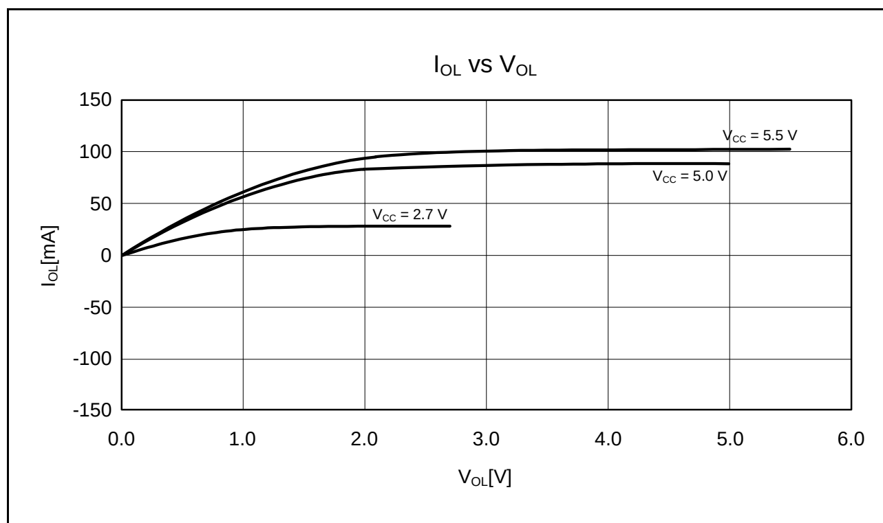
Figure 35.16 V OL and I OL Voltage Characteristics of RIIC Output Pin at T a = 25°C (Reference Data)
