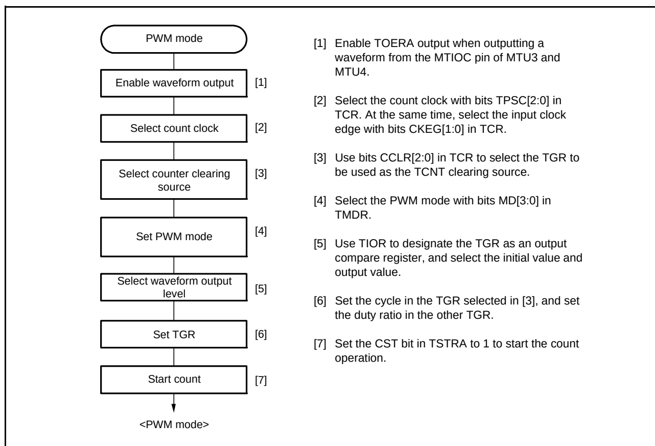
Figure 20.25 Example of PWM Mode Setting Procedure
