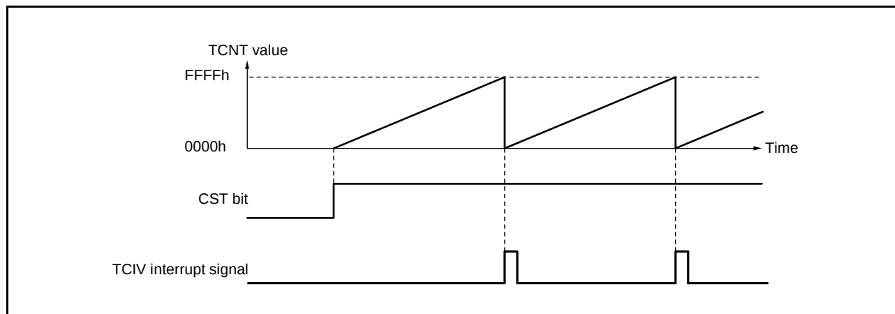
Figure 20.5 Free-Running Counter Operation
