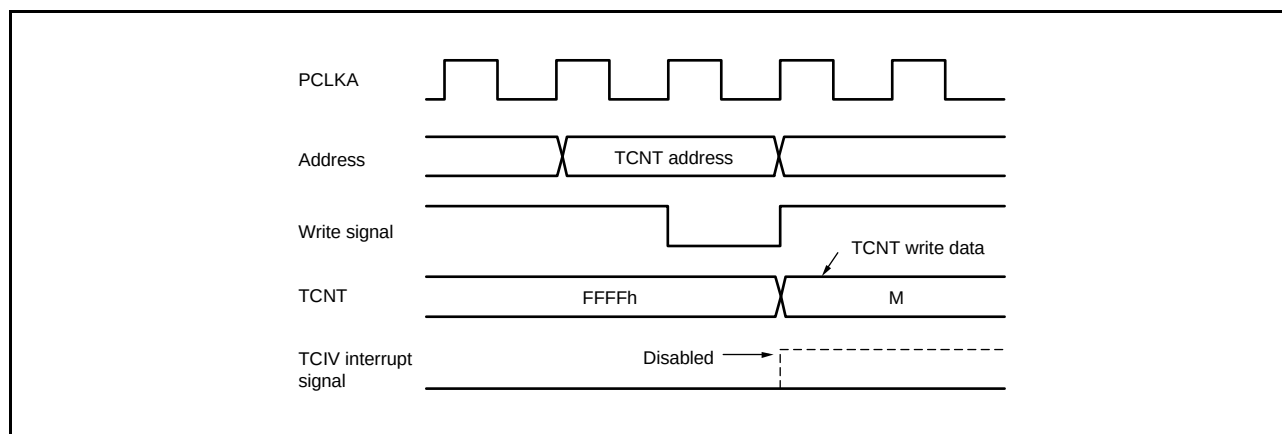
Figure 20.137 Contention between TCNT Write Operation and Overflow
