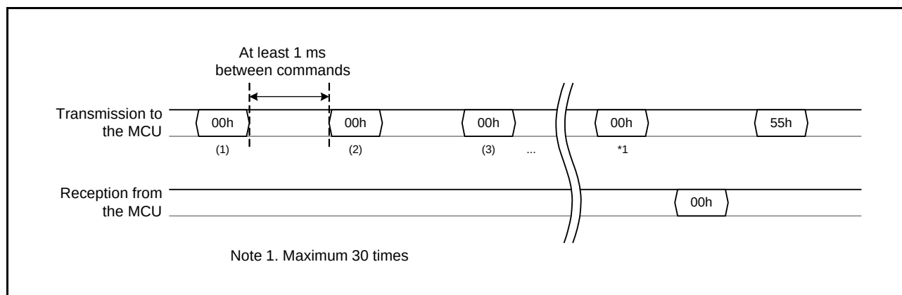
Figure 34.21 Transmit/Receive Data for Bit Rate Automatic Adjustment
