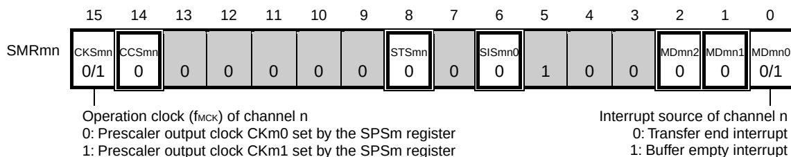
Figure 18-34. Example of Contents of Registers for Master Reception of 3-Wire Serial I/O (CSI00, CSI10, CSI30) (1/2)
