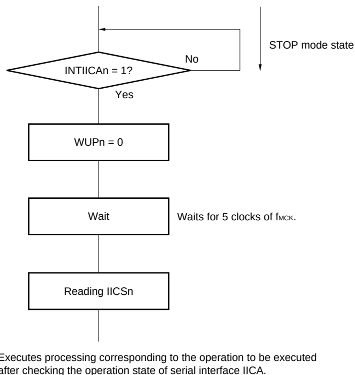
Figure 19-24. Flow When Setting WUPn = 0 upon Address Match (Including Extension Code Reception)
