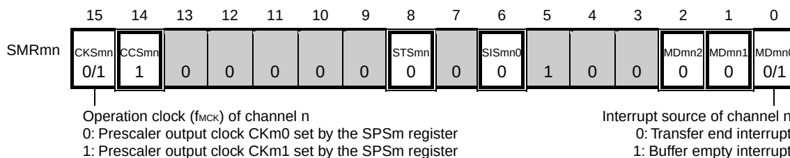
Figure 18-64. Example of Contents of Registers for Slave Transmission/Reception of 3-Wire Serial I/O (CSI00, CSI10, CSI30) (1/2)
