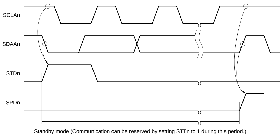
Figure 19-27. Timing for Accepting Communication Reservations
