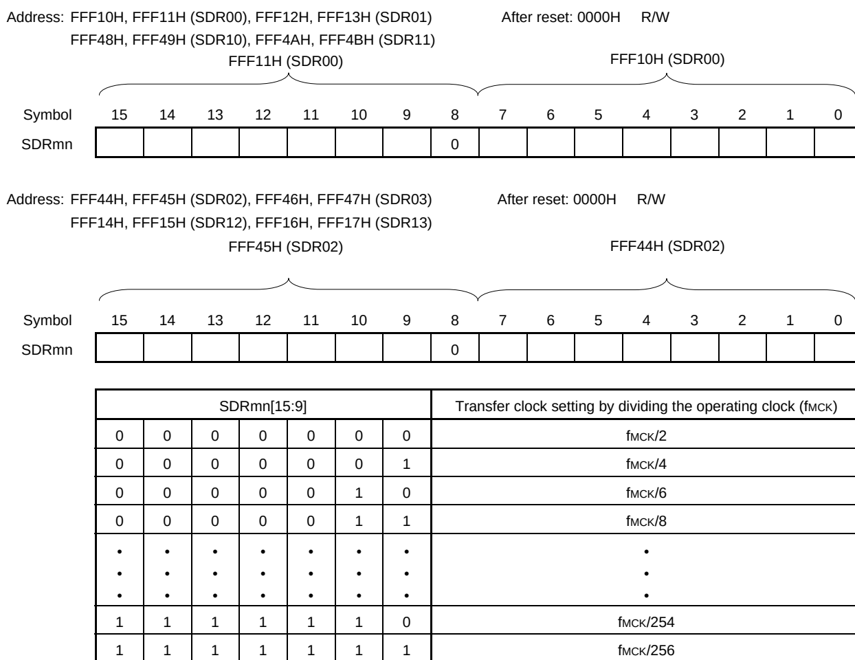
Figure 18-9. Format of Serial Data Register mn (SDRmn)
