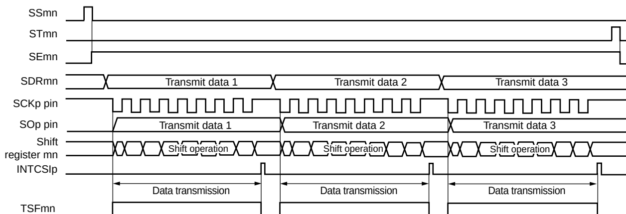
Figure 18-30. Timing Chart of Master Transmission (in Single-Transmission Mode) (Type 1: DAPmn = 0, CKPmn = 0)
