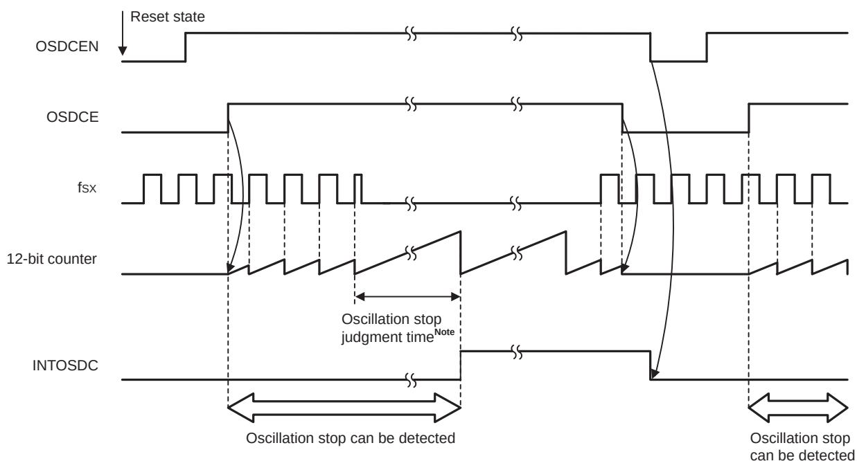
Figure 31-6. Timing of Oscillation Stop Detection by Oscillation Stop Detector
