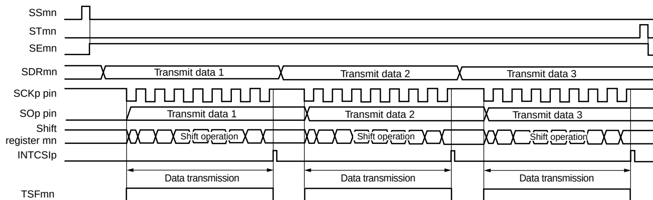
Figure 18-54. Timing Chart of Slave Transmission (in Single-Transmission Mode)
