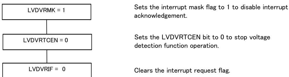
Figure 29 - 14 Setting procedure to disable VRTC voltage detection function
