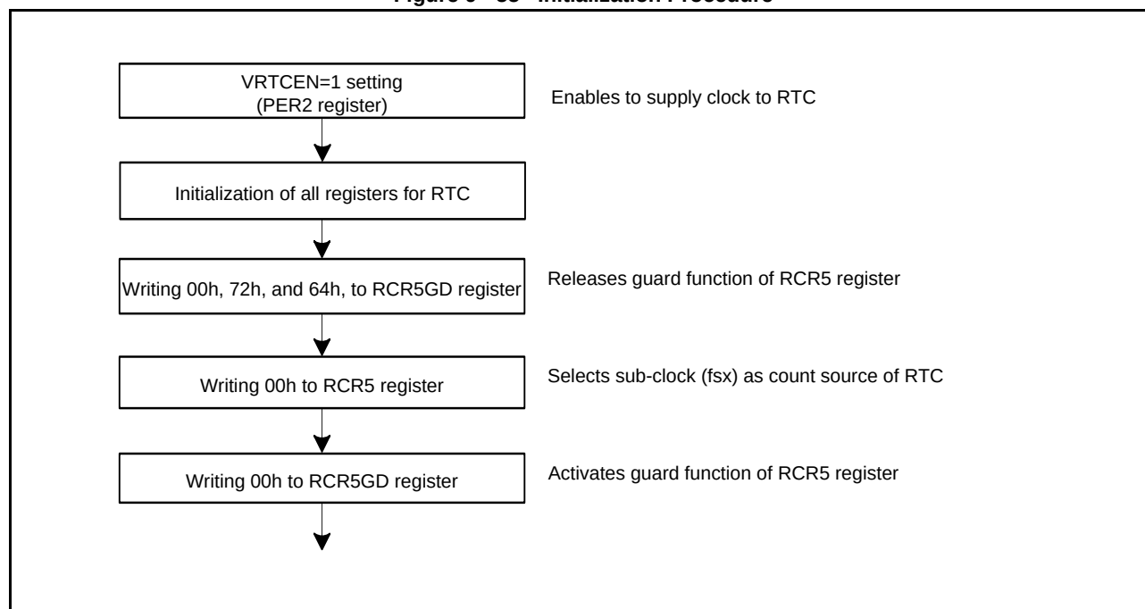
Figure 9 - 55 Initialization Procedure
