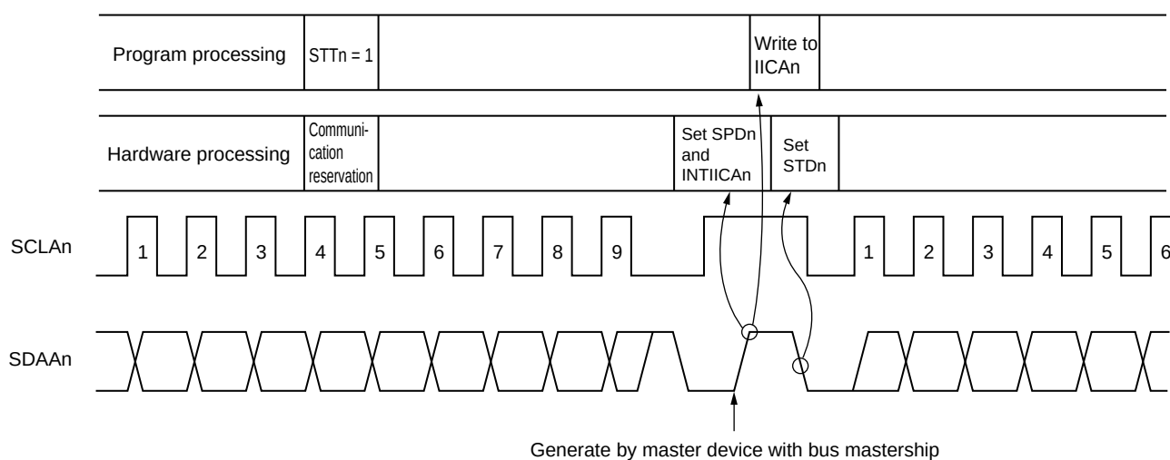
Figure 19-26. Communication Reservation Timing
