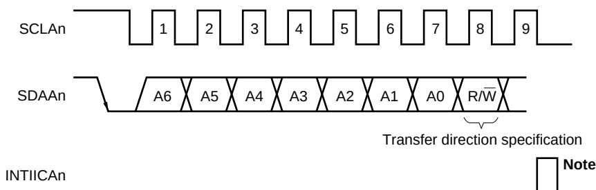
Figure 19-18. Transfer Direction Specification
