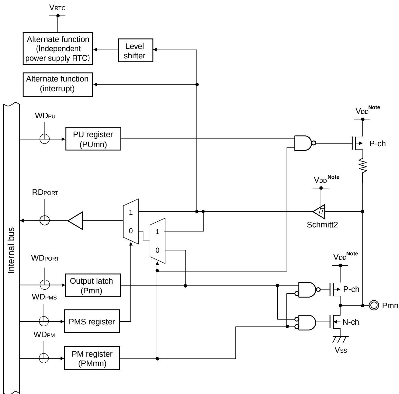
Figure 2-5. Pin Block Diagram for Pin Type 4-3-6
