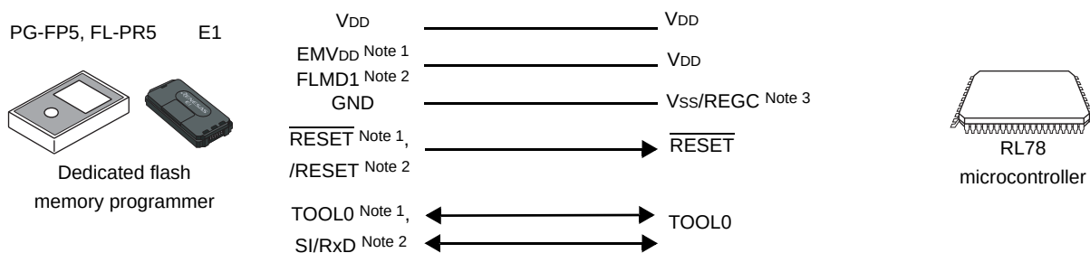
Figure 36 - 2 Communication with Dedicated Flash Memory Programmer
