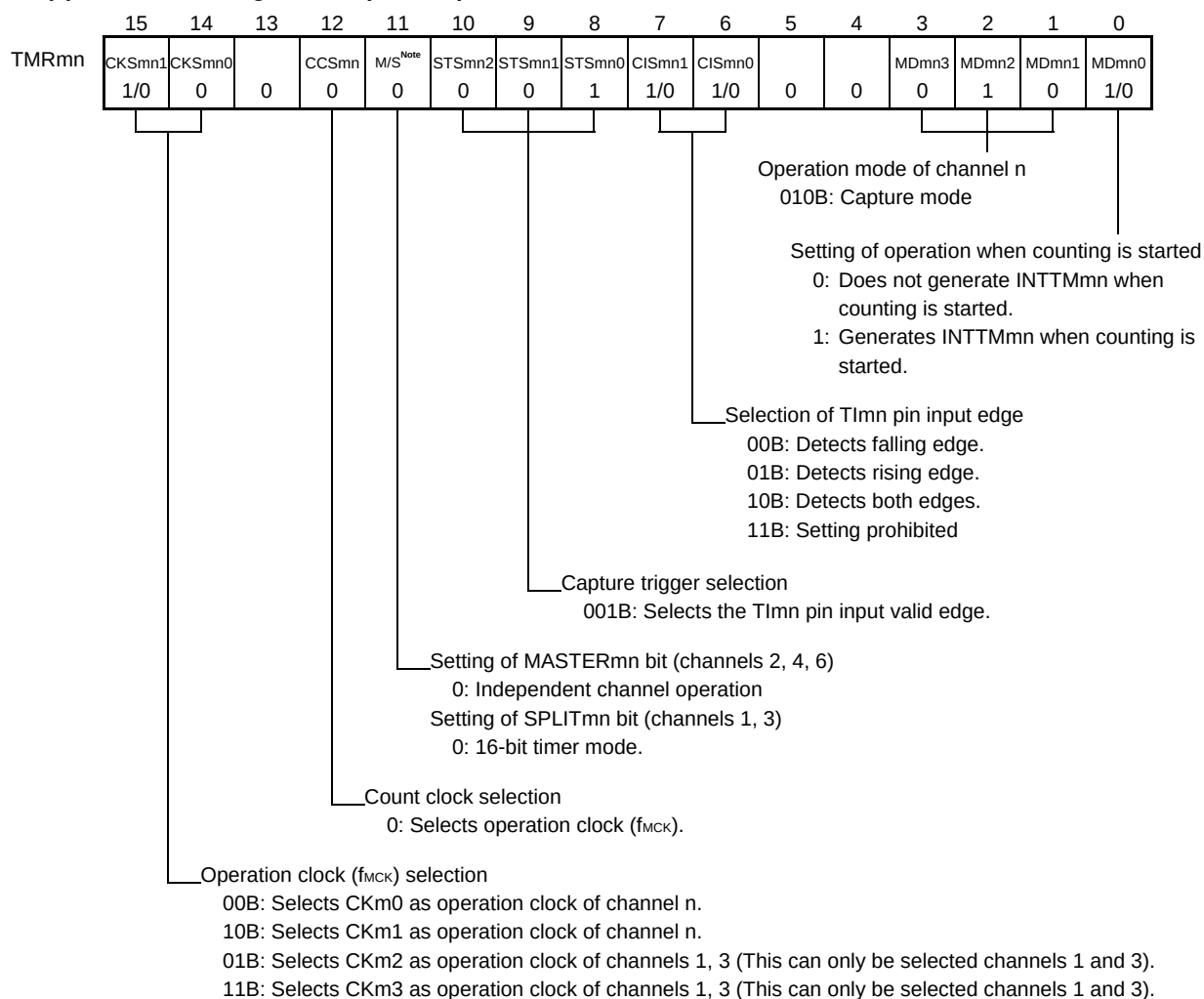
Figure 8-55. Example of Set Contents of Registers to Measure Input Pulse Interval
