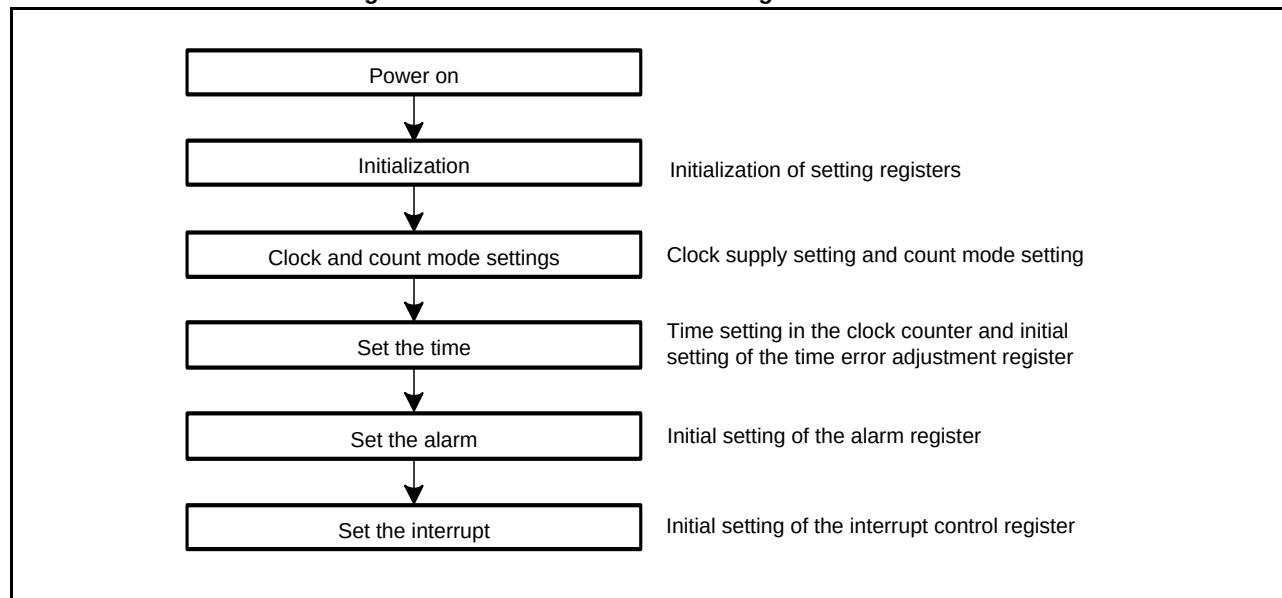
Figure 9 - 54 Outline of Initial Settings after Power On
