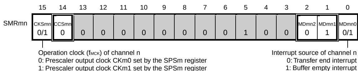
Figure 18-77. Example of Contents of Registers for UART Transmission of UART (UART0 to UART3) (1/2)
