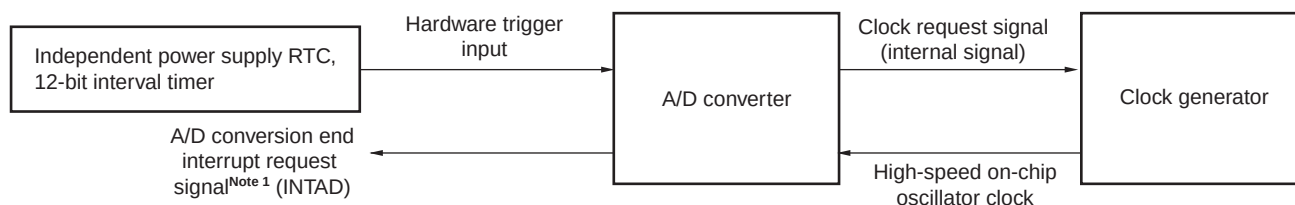
Figure 15-35. Block Diagram When Using SNOOZE Mode Function
