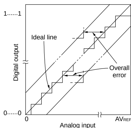
Figure 15-39. Overall Error
