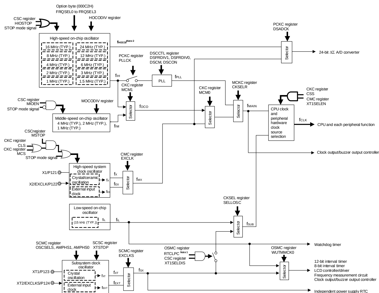
Figure 6 - 1 Block Diagram of Clock Generator
