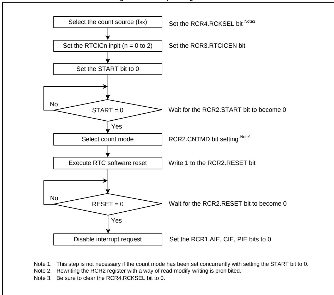
Figure 9 - 67 Stop Setting Procedure
