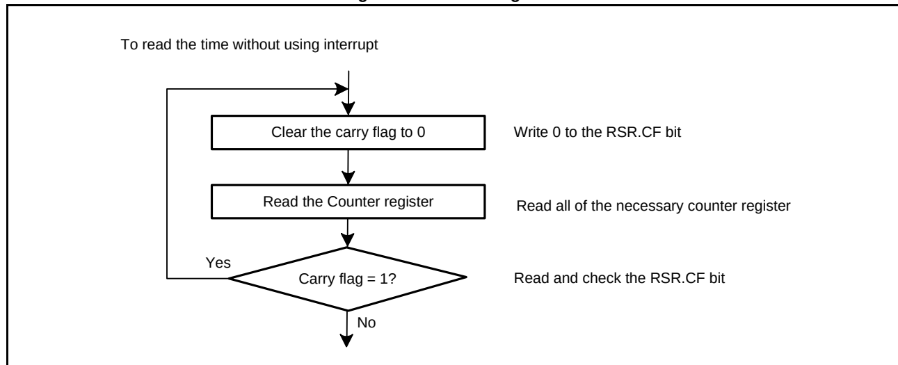
Figure 9 - 59 Reading Time
