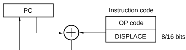
Figure 3-12. Outline of Relative Addressing
