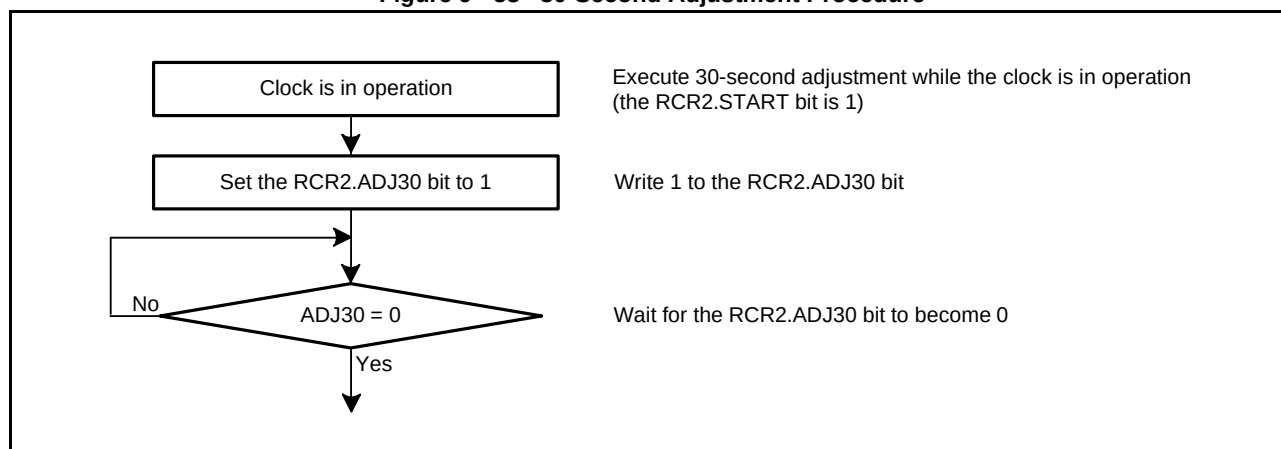
Figure 9 - 58 30-Second Adjustment Procedure
