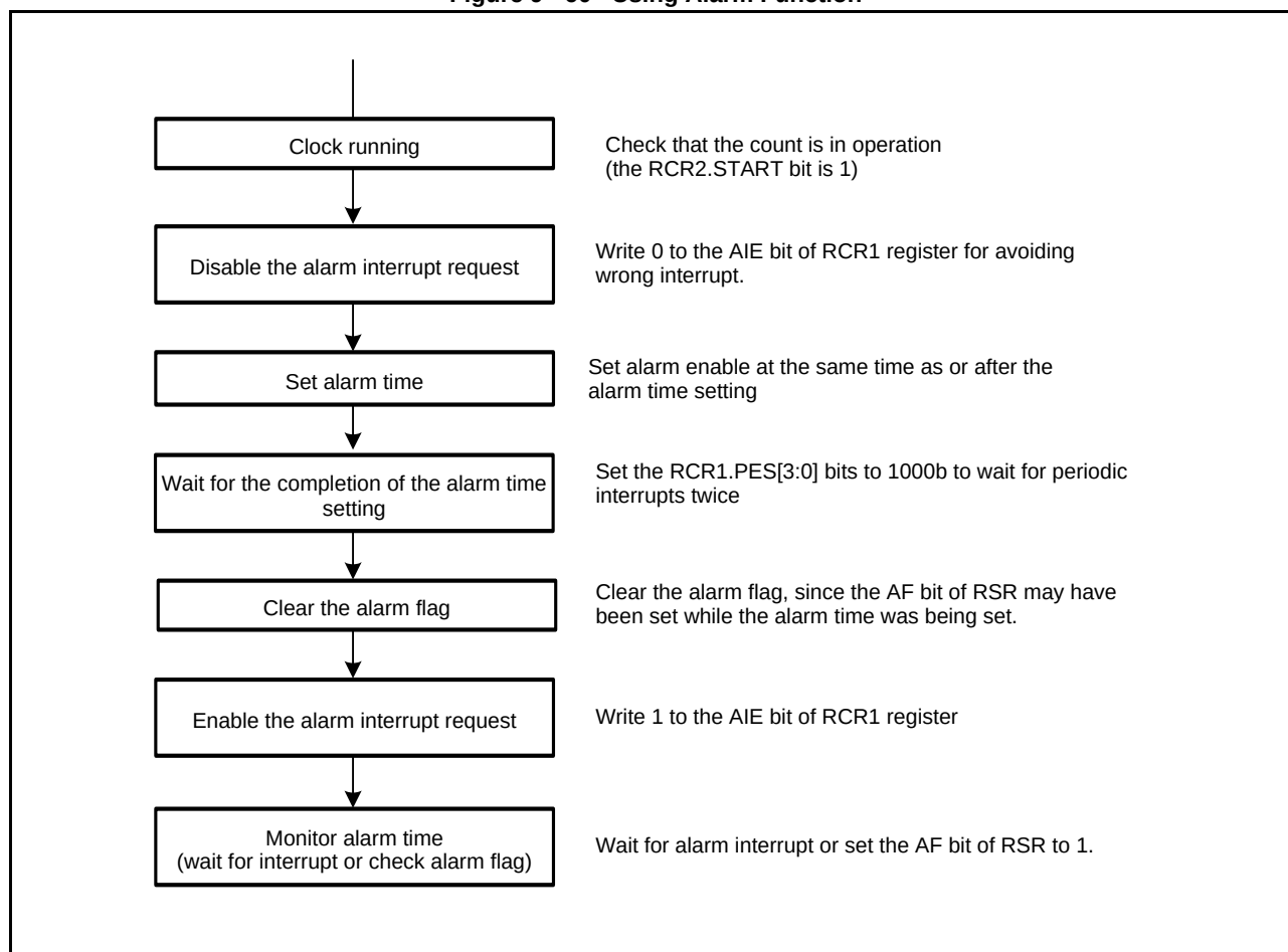
Figure 9 - 60 Using Alarm Function
