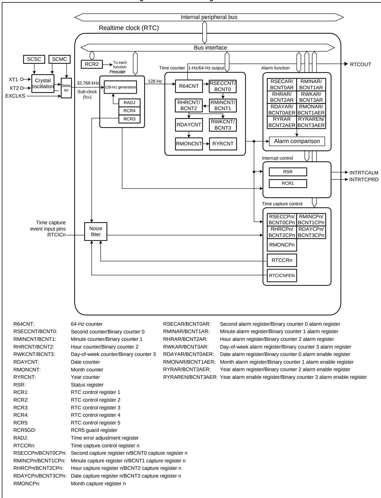
Figure 9 - 1 Block Diagram of RTC
