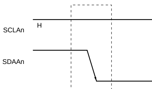
Figure 19-16. Start Conditions
