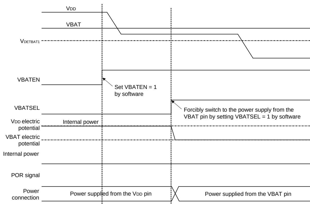
Figure 30-6. Battery Backup Operation (2) with VBATEN = 1 and VBATSEL = 1
