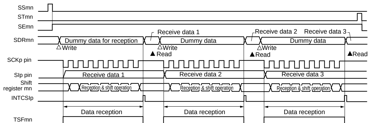
Figure 18-38. Timing Chart of Master Reception (in Single-reception Mode)
