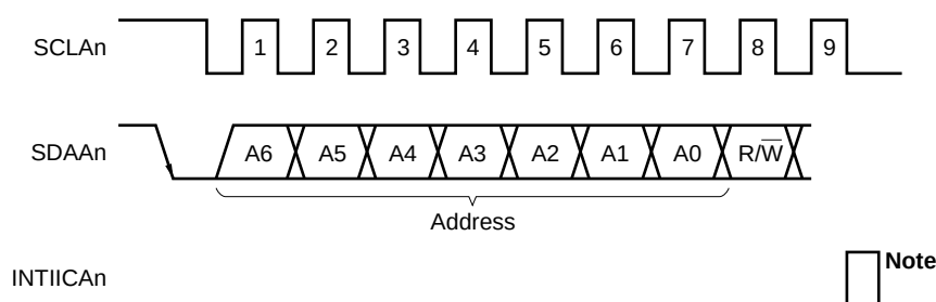
Figure 19-17. Address
