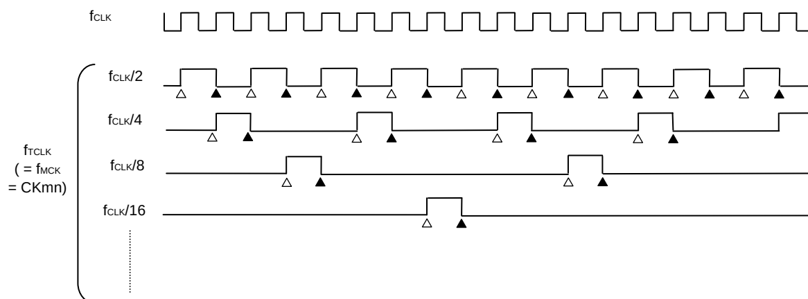
Figure 8-27. Timing of f_{\text{CLK}} and count clock ( f_{\text{CLK}} ) (When CCMn = 0)
