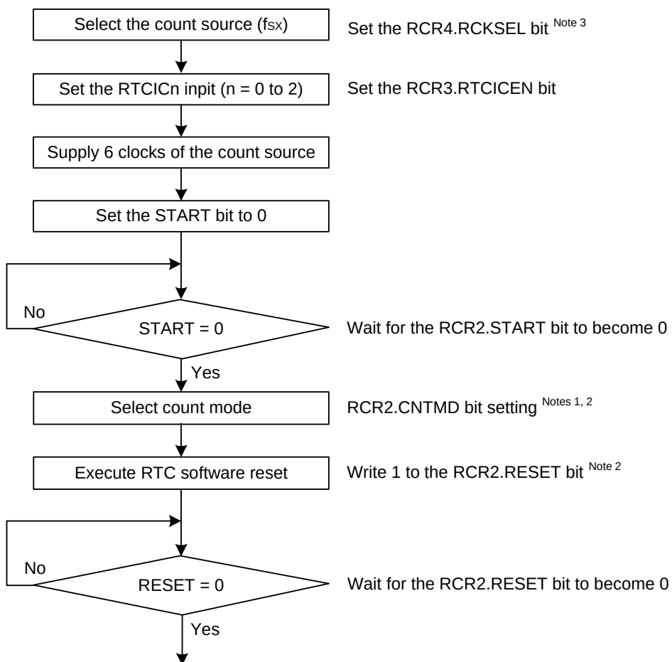
Figure 9 - 56 Clock and Count Mode Setting Procedure
