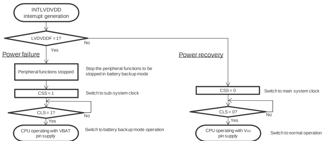
Figure 30-13. Setting Procedure for Power Supply Switching with Hardware
