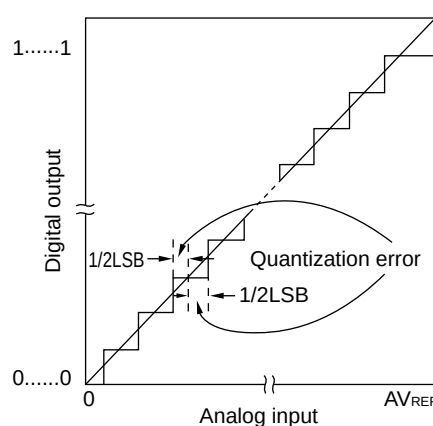
Figure 15-40. Quantization Error
