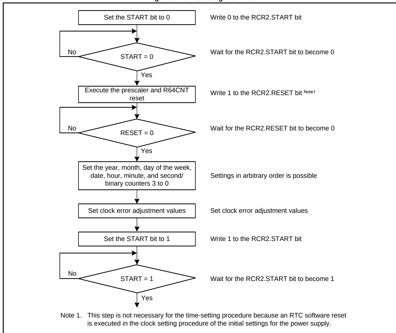
Figure 9 - 57 Setting the Time
