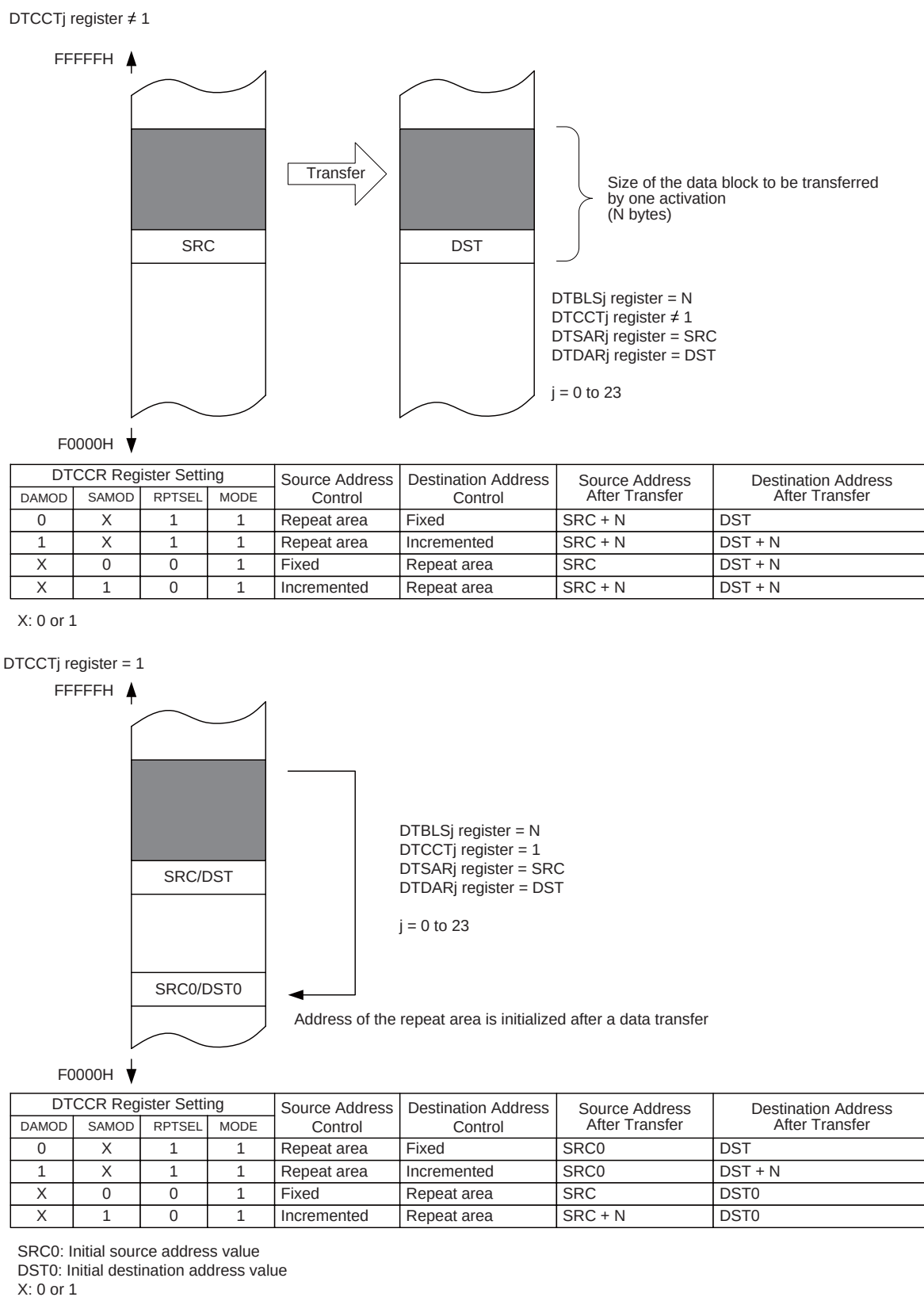
Figure 22-18. Data Transfers in Repeat Mode
