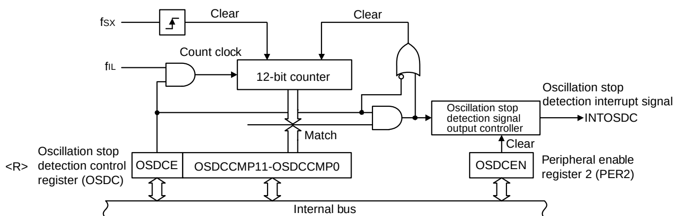
Figure 31-1. Block Diagram of Oscillation Stop Detector
