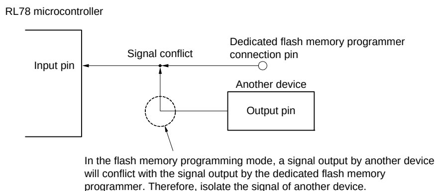
Figure 36 - 5 Signal Conflict ( RESET Pin)
