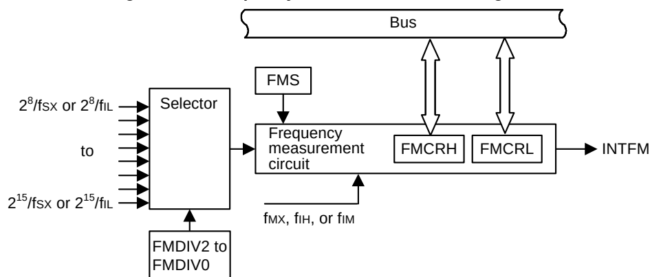
Figure 10 - 1 Frequency Measurement Circuit Diagram
