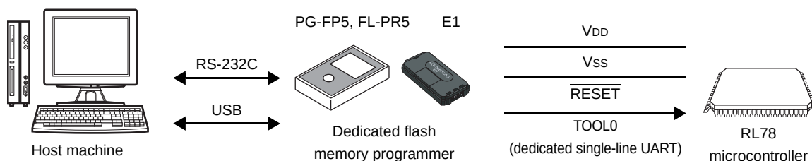
Figure 36 - 1 Environment for Writing Program to Flash Memory
