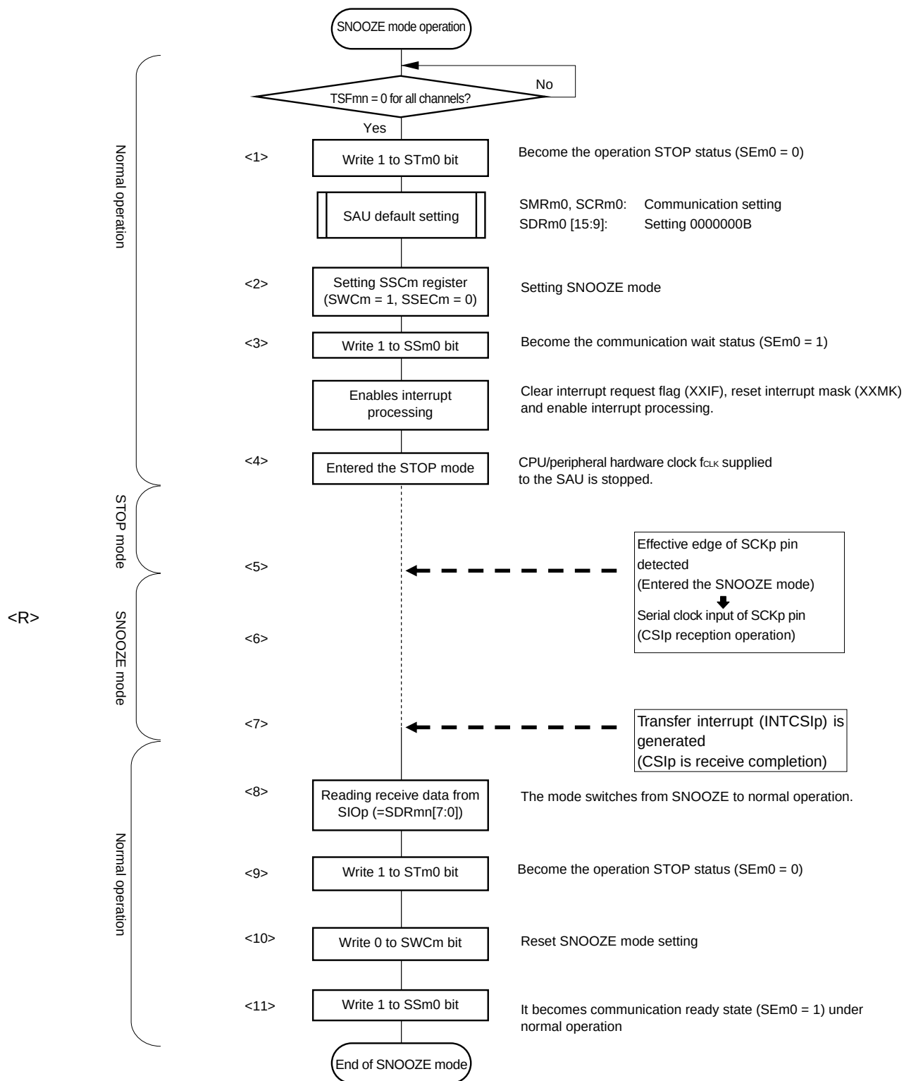
Figure 18-73. Flowchart of SNOOZE Mode Operation (Once Startup)
