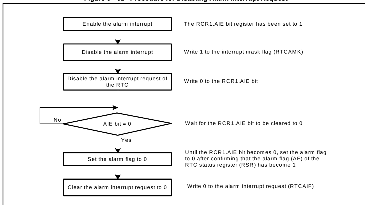
Figure 9 - 61 Procedure for Disabling Alarm Interrupt Request
