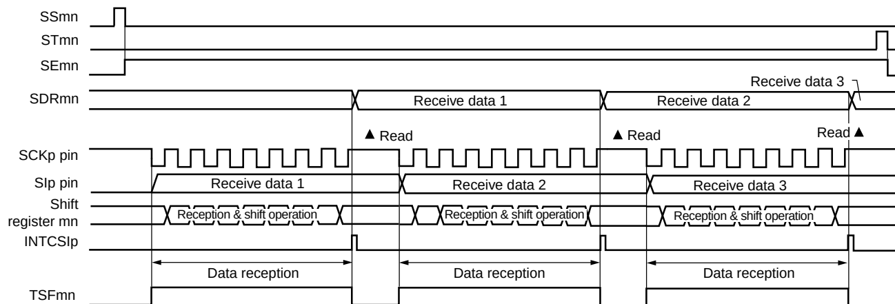
Figure 18-62. Timing Chart of Slave Reception (in Single-reception Mode)
