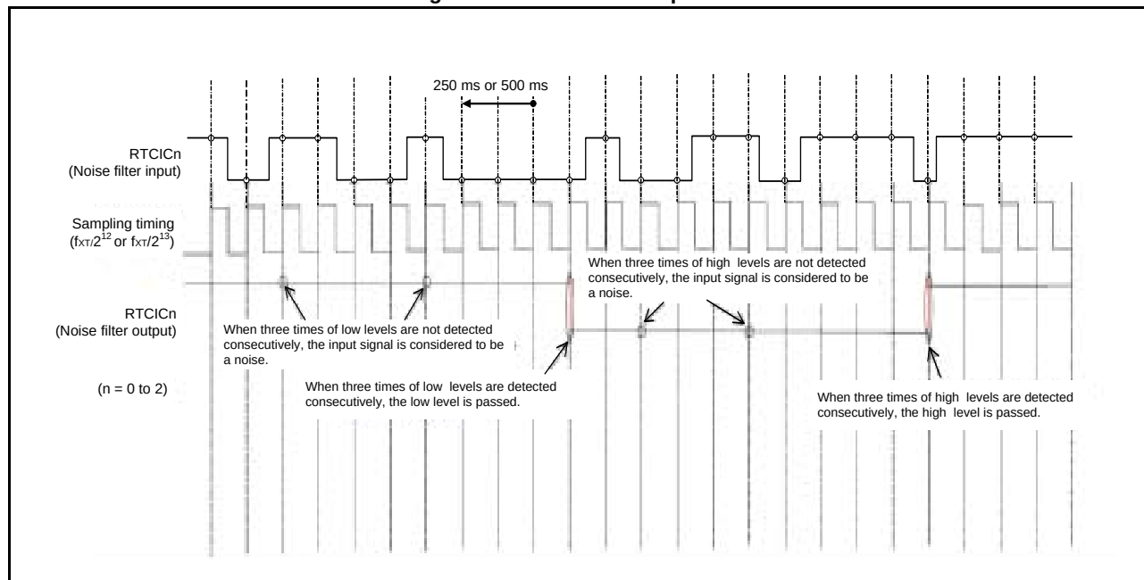
Figure 9 - 64 Noise filter operation
