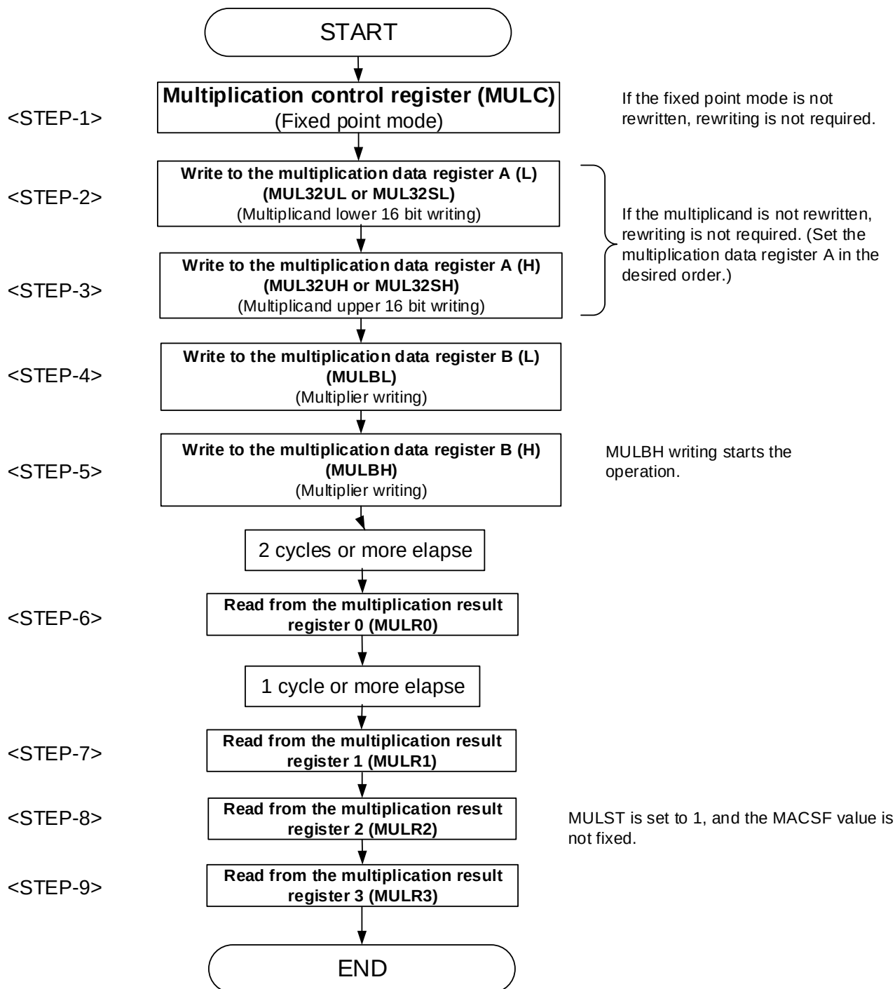
Figure 39-8. MACL Operation Flow (for Multiplication)
