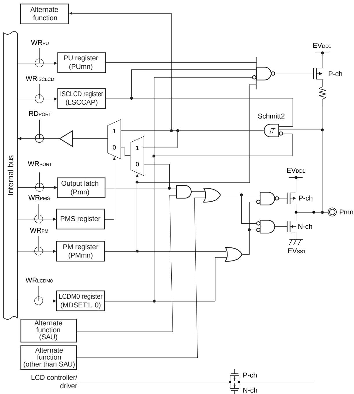
Figure 2-9. Pin Block Diagram for Pin Type 7-5-5
