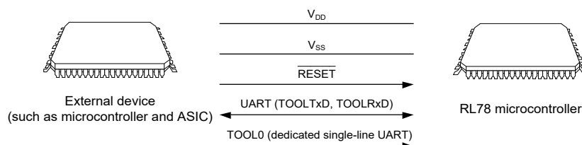
Figure 22-3. Environment for Writing Program to Flash Memory
