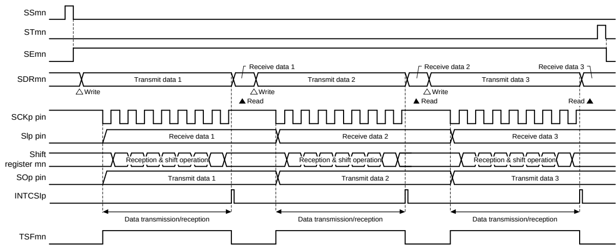
Figure 13-65. Timing Chart of Slave Transmission/Reception (in Single-Transmission/Reception Mode) (Type 1: DAPmn = 0, CKPmn = 0)
