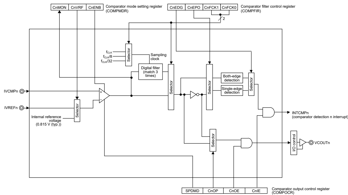
Figure 12-1. Block Diagram of the Comparator
