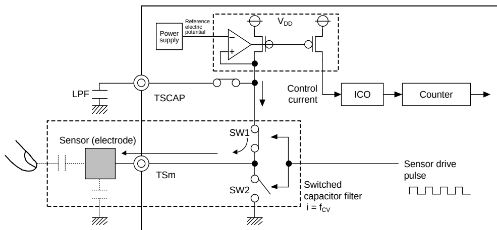
Figure 15-28. Charging Operation
