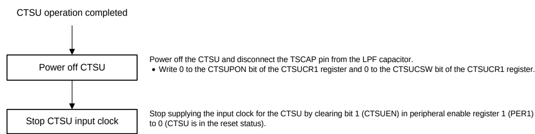
Figure 15-33. CTSU Stopping Flowchart
