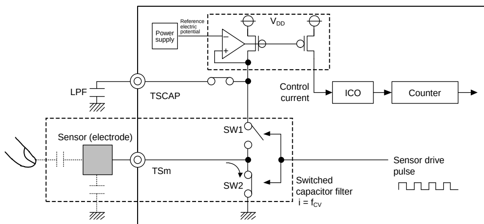
Figure 15-29. Discharging Operation
