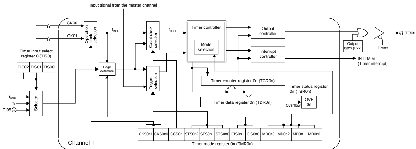
Figure 6-5. Internal Block Diagram of Channel 5 of Timer Array Unit
