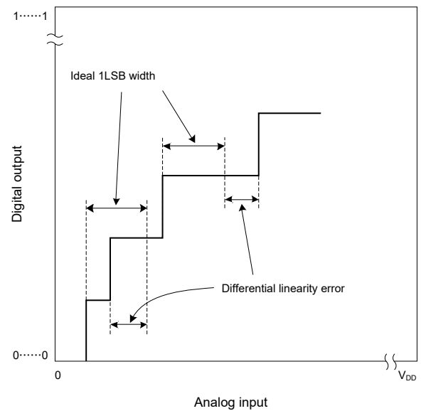
Figure 11-21. Differential Linearity Error
