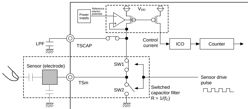
Figure 15-27. Measurement Circuit
