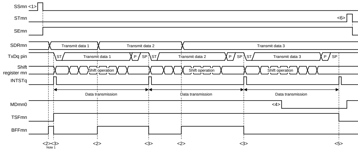
Figure 13-76. Timing Chart of UART Transmission (in Continuous Transmission Mode)
