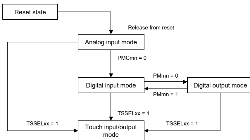
Figure 4-10. State Transition Diagram of ANLxx/TSxx/Port Pin Function
