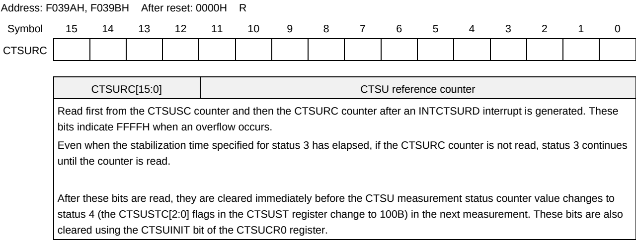
Figure 15-21. Format of CTSU Reference Counter (CTSURC)
