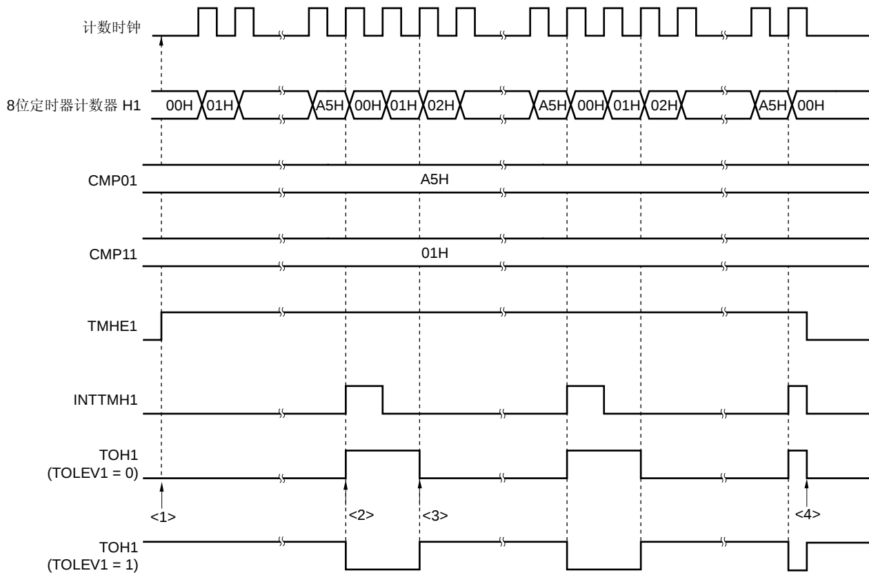
(a)基本操作 ( 00H < \text{CMP11} < \text{CMP01} < FFH )
